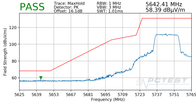
Plot 7-825. Antenna 4b (Pk, Ch.149, 802.11ax(SU), MCS11)
