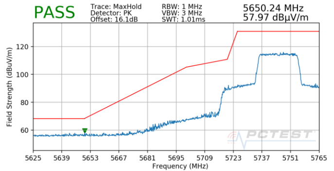
Plot 7-823. Antenna 4b (Pk, Ch.149, 802.11ax(SU), MCS0)
