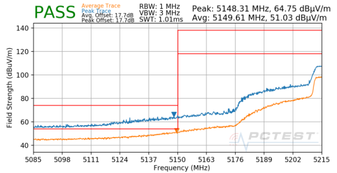
Plot 7-832. Antenna 4b (Pk & Avg, Ch.46, 802.11n, MCS0)
