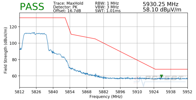
Plot 7-828. Antenna 4b (Pk, Ch.165, 802.11ax(SU), MCS11)
