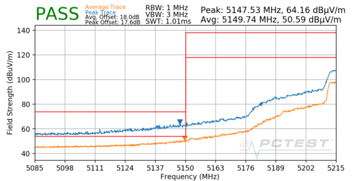
Plot 7-833. Antenna 4b (Pk & Avg, Ch.46, 802.11n, MCS3)
