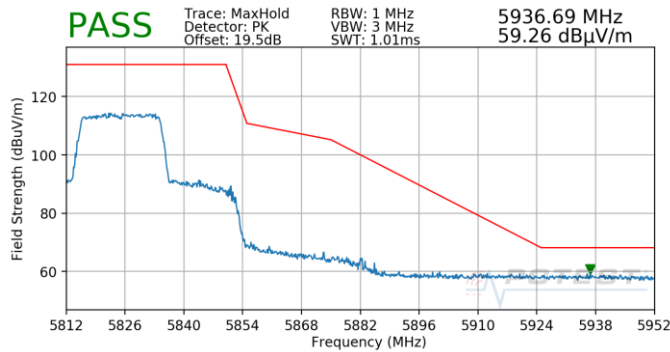
Plot 7-826. Antenna 4b (Pk, Ch.165, 802.11ax(SU), MCS0)
