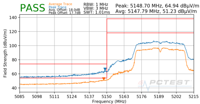
Plot 7-830. Antenna 4b (Pk & Avg, Ch.38, 802.11n, MCS3)
