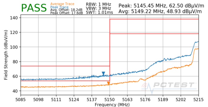
Plot 7-834. Antenna 4b (Pk & Avg, Ch.46, 802.11n, MCS5)
