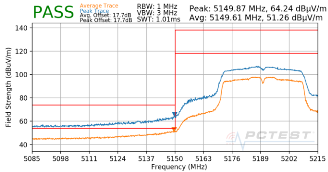
Plot 7-829. Antenna 4b (Pk & Avg, Ch.38, 802.11n, MCS0)
