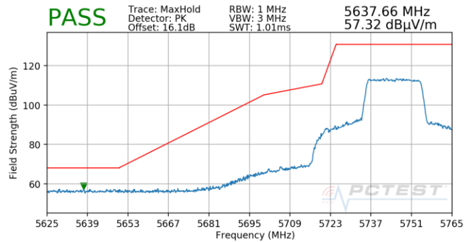
Plot 7-824. Antenna 4b (Pk, Ch.149, 802.11ax(SU), MCS3)
