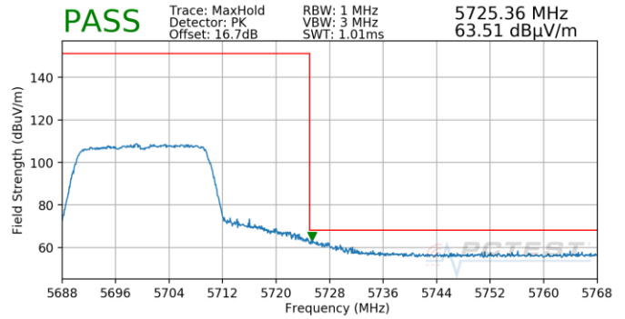
Plot 7-822. Antenna 4b (Pk, Ch.140, 802.11ax(SU), MCS11)
