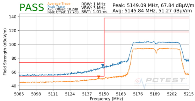
Plot 7-831. Antenna 4b (Pk & Avg, Ch.38, 802.11n, MCS5)
