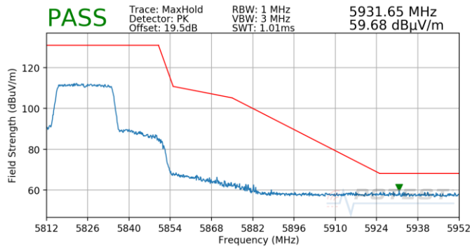
Plot 7-827. Antenna 4b (Pk, Ch.165, 802.11ax(SU), MCS3)
