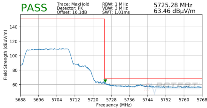
Plot 7-821. Antenna 4b (Pk, Ch.140, 802.11ax(SU), MCS3)
