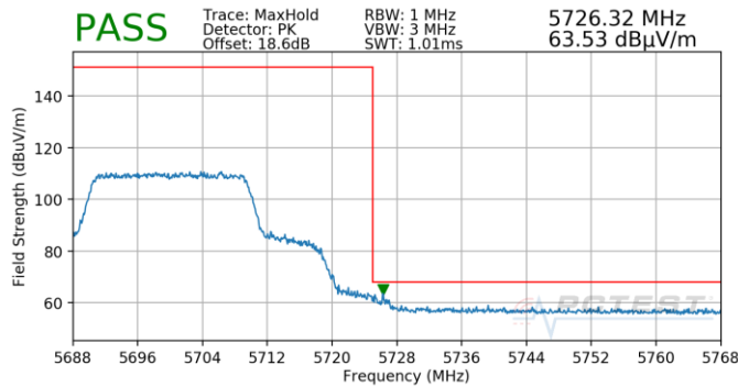
Plot 7-820. Antenna 4b (Pk, Ch.140, 802.11ax(SU), MCS0)
