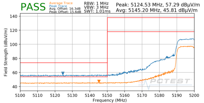
Plot 7-800. Antenna 4b (Pk & Avg, Ch.40, 802.11ax(SU), MCS11)
