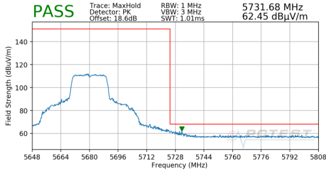
Plot 7-819. Antenna 4b (Pk, Ch.136, 802.11ax(SU), MCS11)
