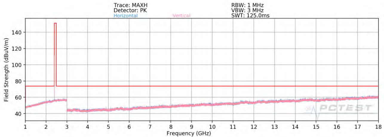
Plot 7-84. Radiated Spurious Emissions Above 1GHz Antenna 2a (1Mbps, ePA – Ch. 0)
