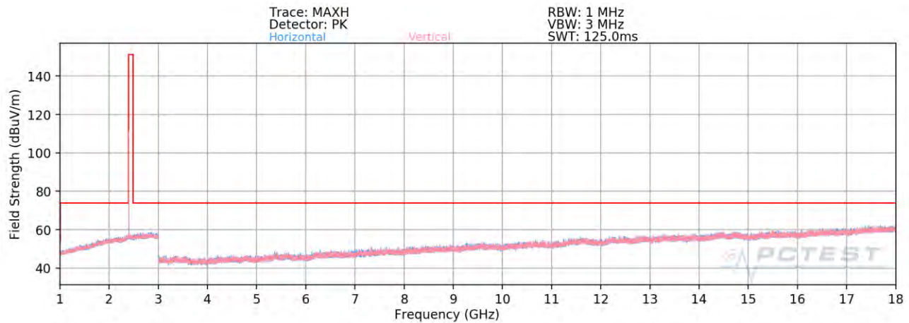
Plot 7-81. Radiated Spurious Emissions Above 1GHz Antenna 4a (1Mbps, ePA – Ch. 0)
