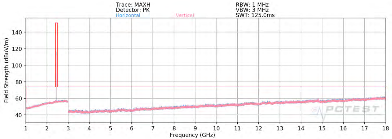
Plot 7-85. Radiated Spurious Emissions Above 1GHz Antenna 2a (1Mbps, ePA – Ch. 19)
