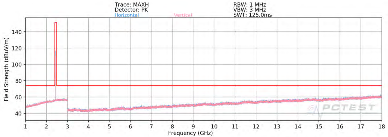
Plot 7-82. Radiated Spurious Emissions Above 1GHz Antenna 4a (1Mbps, ePA – Ch. 19)
