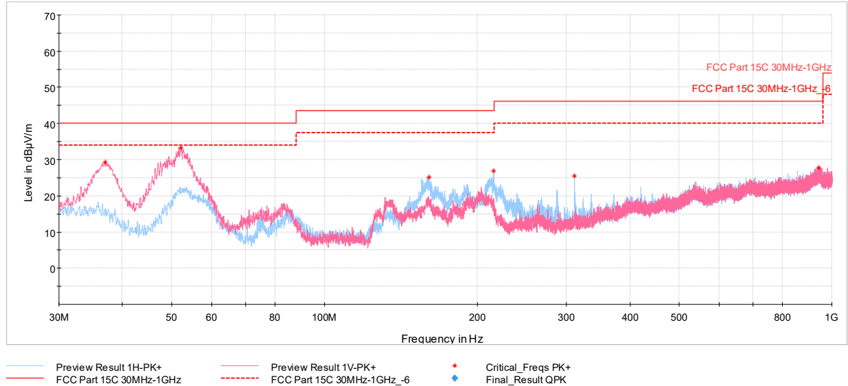
Plot 7-104. Radiated Spurious Emissions Below 1GHz TxBF (1Mbps, ePA – Ch.19, Pol. H & V, with AC/DC Adapter)
