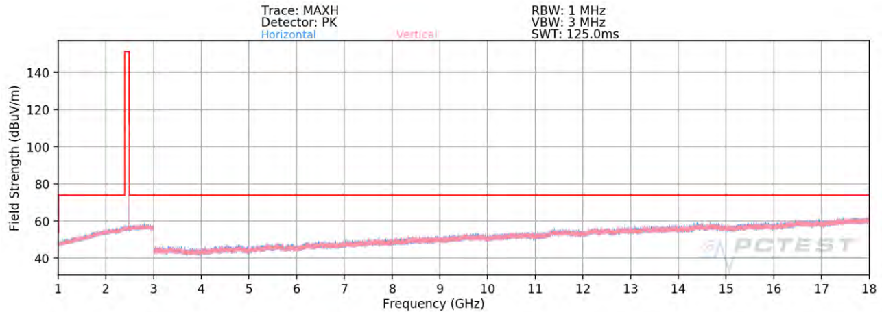
Plot 7-86. Radiated Spurious Emissions Above 1GHz Antenna 2a (1Mbps, ePA – Ch. 39)
