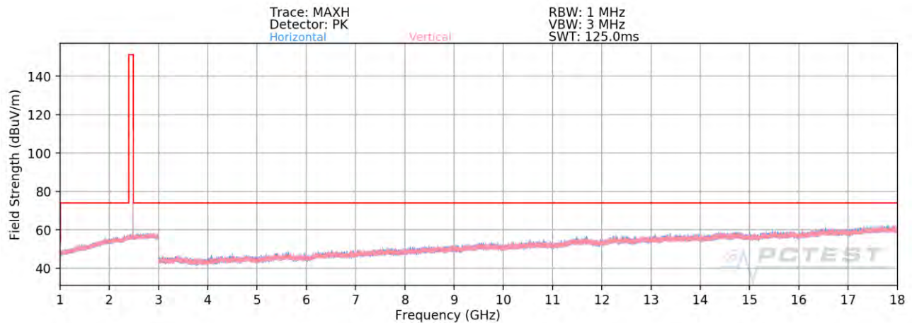
Plot 7-83. Radiated Spurious Emissions Above 1GHz Antenna 4a (1Mbps ePA – Ch. 39)
