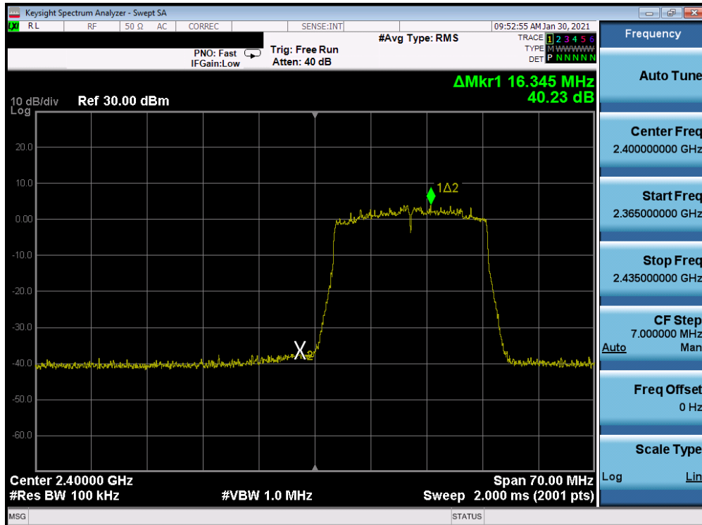
Plot 7-80. Band Edge Antenna 4a (802.11ax OFDMA – RU242 – Ch. 1)
