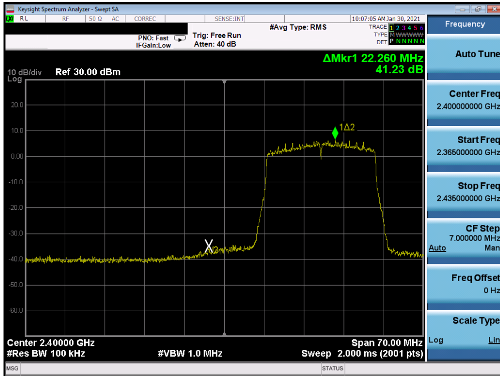
Plot 7-81. Band Edge Antenna 4a (802.11ax OFDMA – RU242 – Ch. 2)
