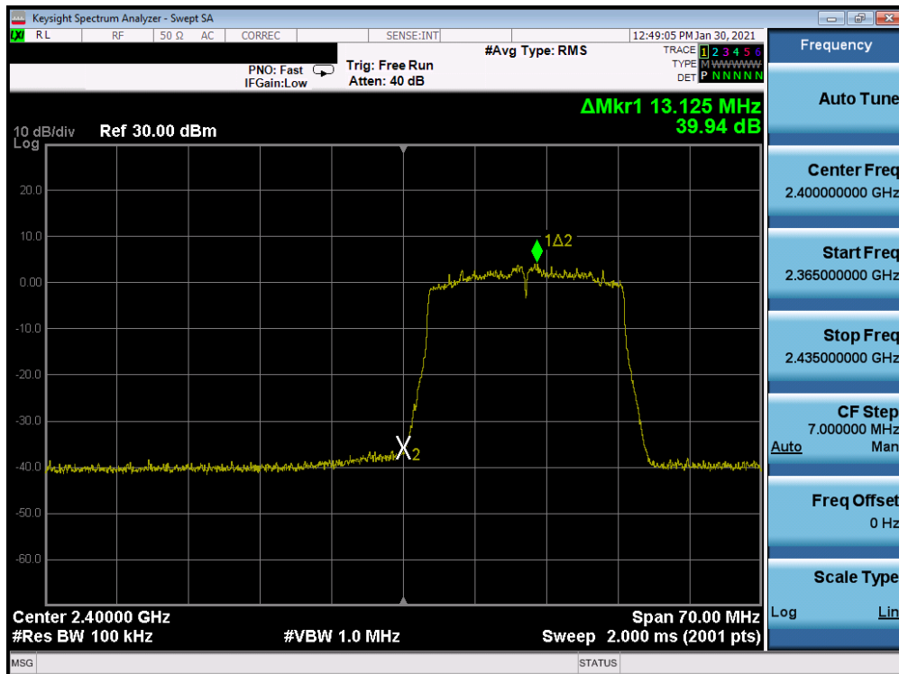
Plot 7-94. Band Edge Antenna 2a (802.11ax OFDMA – RU242 – Ch. 1)
