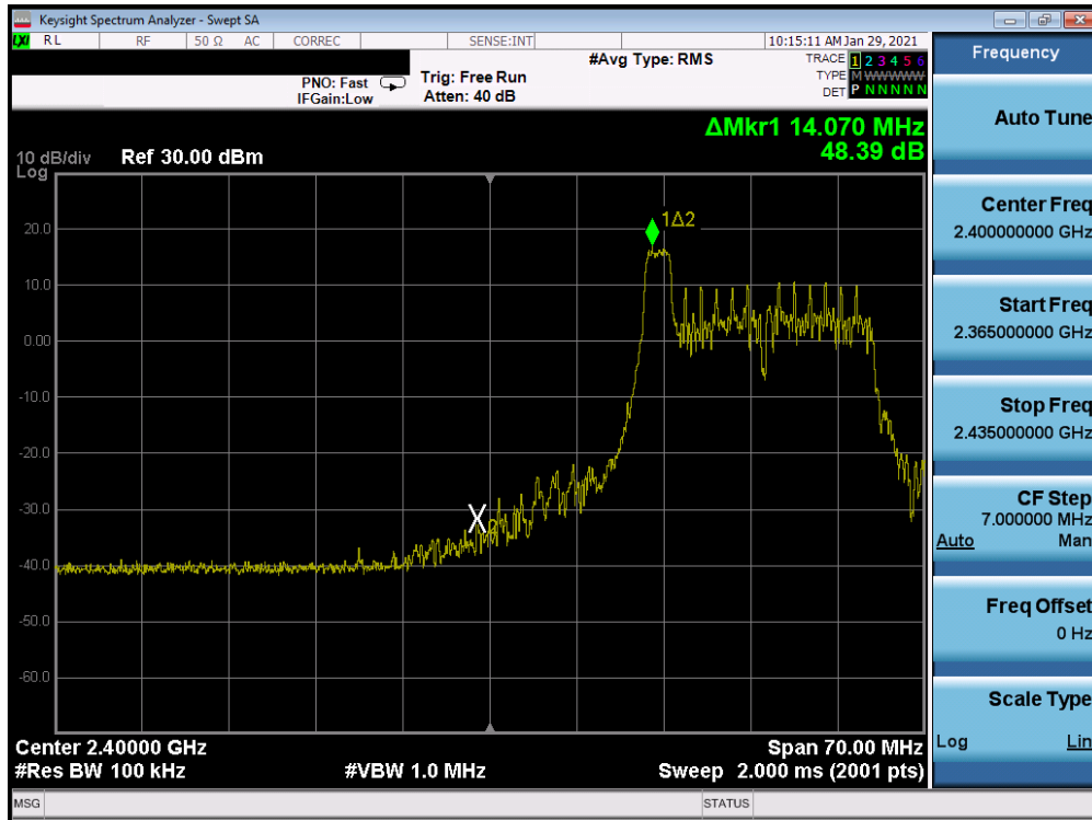
Plot 7-89. Band Edge Antenna 2a (802.11ax OFDMA – RU26 Index 0 – Ch. 3)
