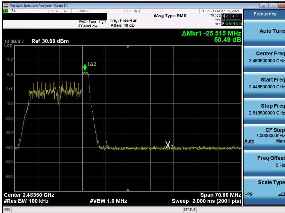
Plot 7-78. Band Edge Antenna 4a (802.11ax OFDMA – RU26 Index 8 – Ch. 11)
