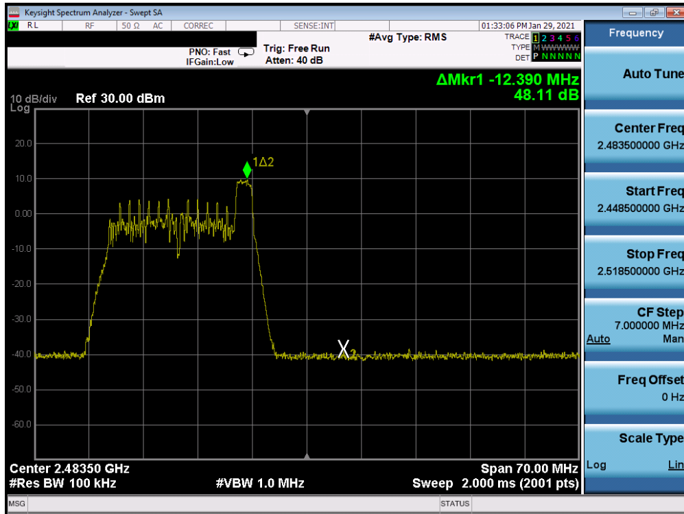
Plot 7-79. Band Edge Antenna 4a (802.11ax OFDMA – RU26 Index 8 – Ch. 12)
