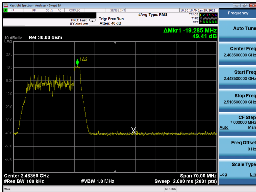
Plot 7-92. Band Edge Antenna 2a (802.11ax OFDMA – RU26 Index 8 – Ch. 11)
