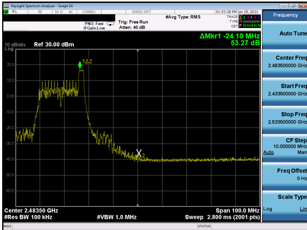
Plot 7-76. Band Edge Antenna 4a (802.11ax OFDMA – RU26 Index 8 – Ch. 9)
