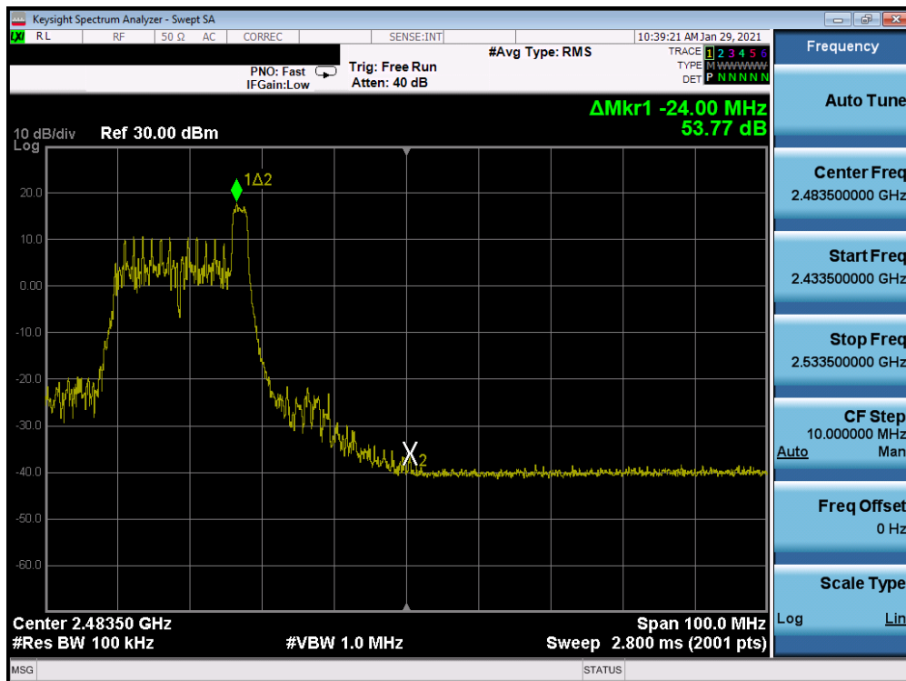
Plot 7-90. Band Edge Antenna 2a (802.11ax OFDMA – RU26 Index 8 – Ch. 9)
