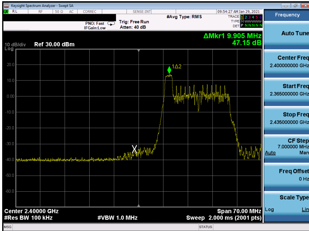
Plot 7-88. Band Edge Antenna 2a (802.11ax OFDMA – RU26 Index 0 – Ch. 2)
