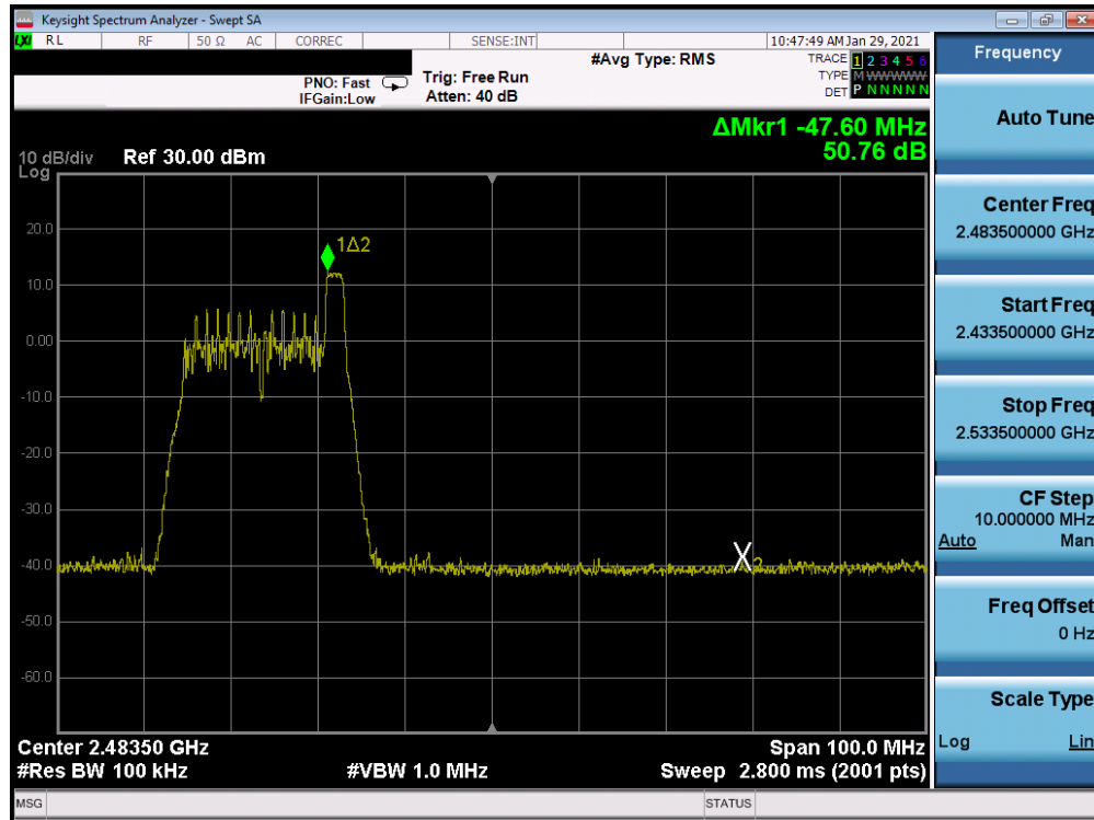
Plot 7-91. Band Edge Antenna 2a (802.11ax OFDMA – RU26 Index 8 – Ch. 10)
