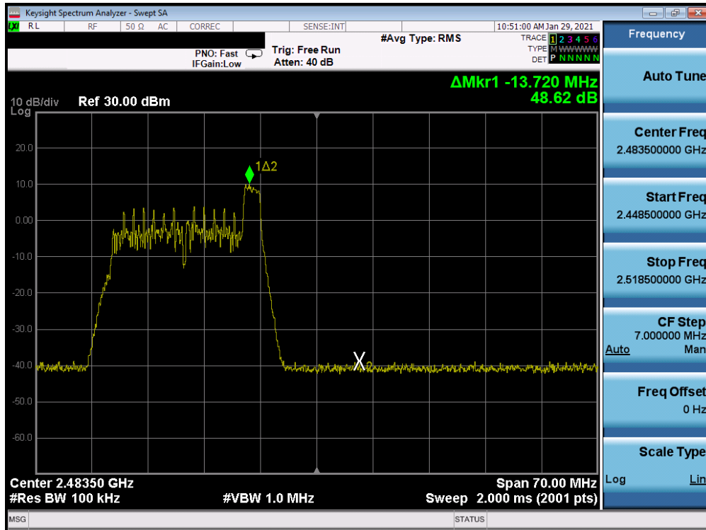
Plot 7-93. Band Edge Antenna 2a (802.11ax OFDMA – RU26 Index 8 – Ch. 12)
