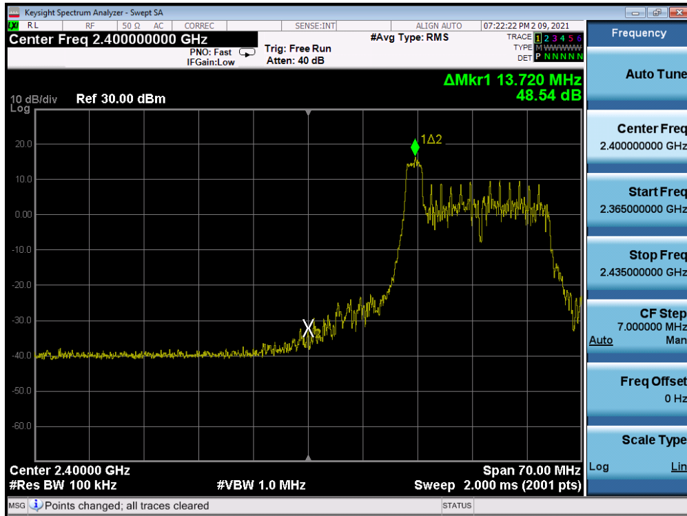
Plot 7-75. Band Edge Antenna 4a (802.11ax OFDMA – RU26 Index 0 – Ch. 3)
