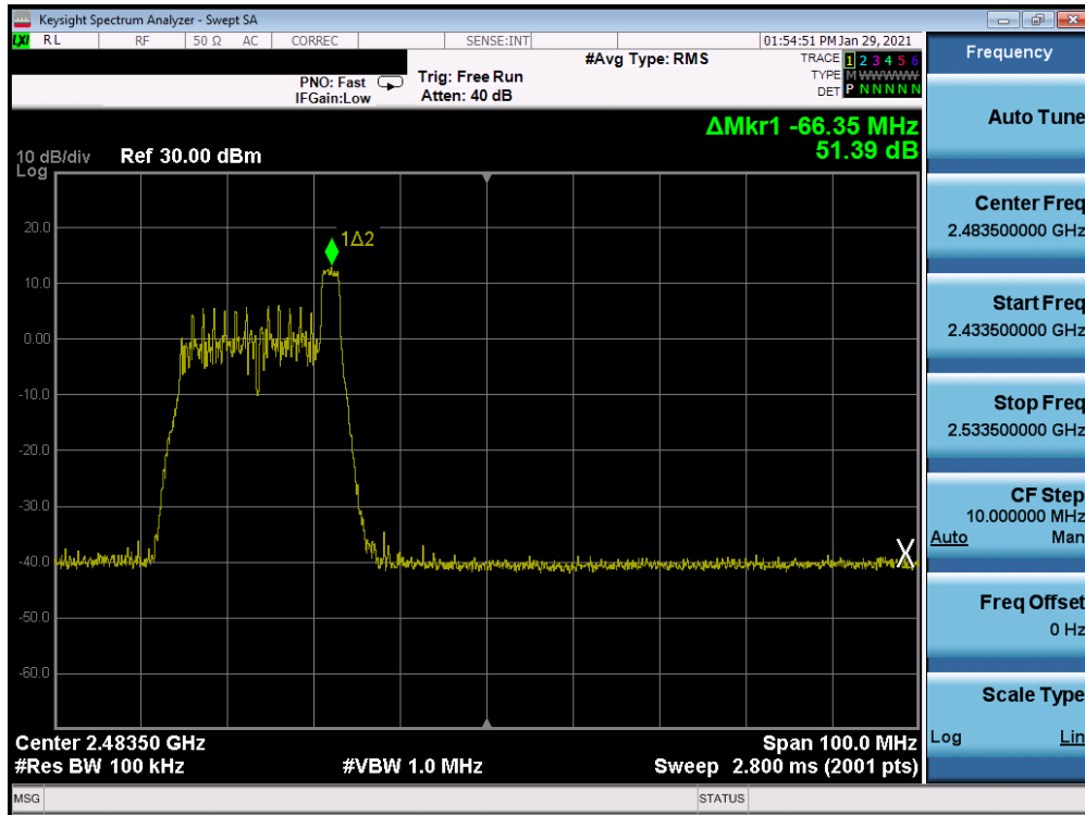
Plot 7-77. Band Edge Antenna 4a (802.11ax OFDMA – RU26 Index 8 – Ch. 10)
