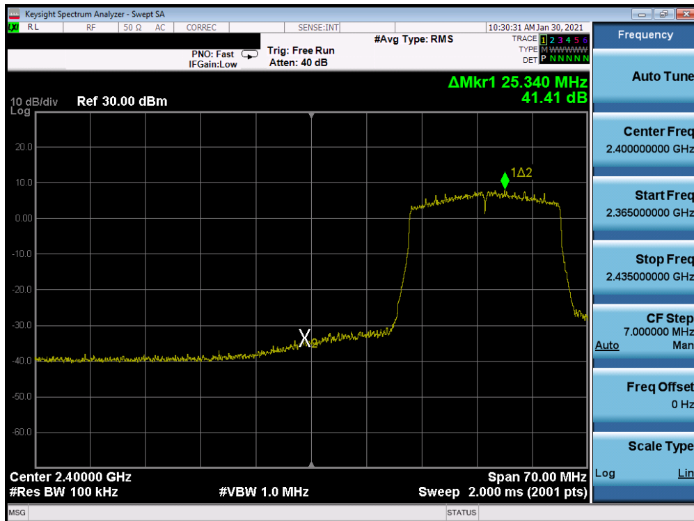
Plot 7-82. Band Edge Antenna 4a (802.11ax OFDMA – RU242 – Ch. 3)
