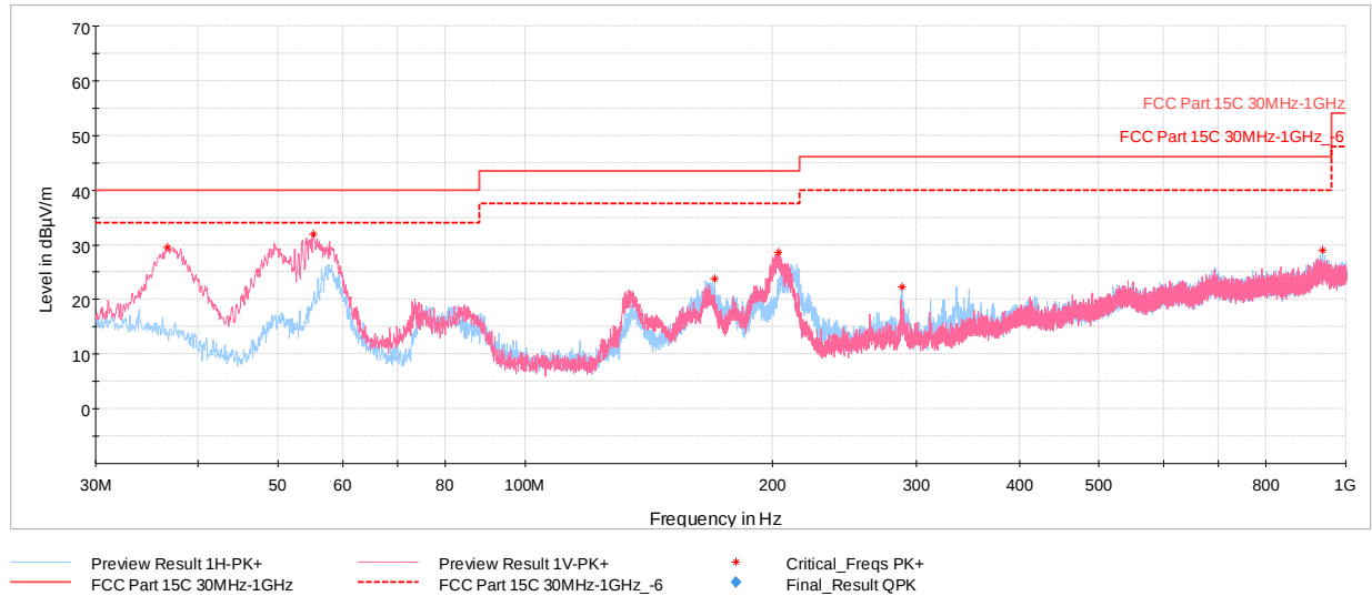
Plot 7-499. Radiated Spurious Emissions below 1GHz CDD 11ax - SU Ch.6, with AC/DC Adapter
