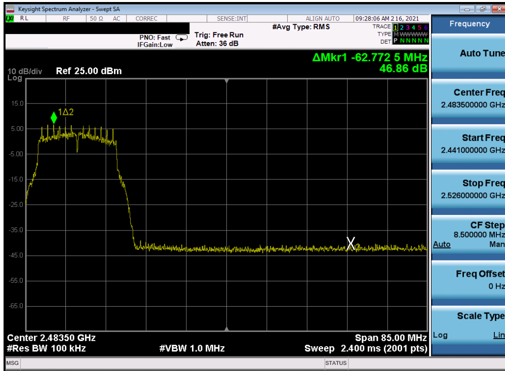
Plot 7-274. Band Edge Plot Antenna 2a (802.11g – Ch. 9) – 18Mbps
