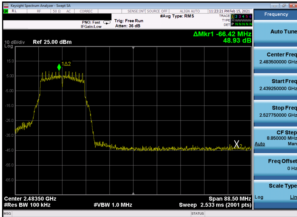
Plot 7-275. Band Edge Plot Antenna 2a (802.11g – Ch. 10) – 18Mbps
