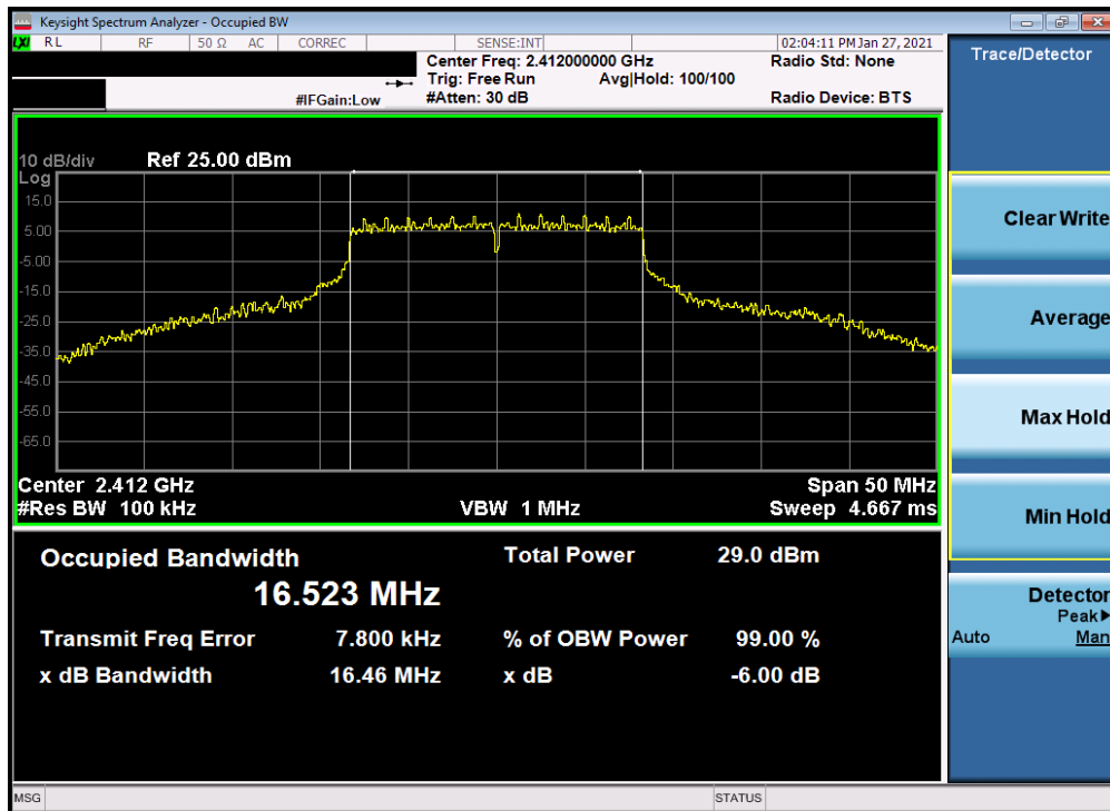
Plot 7-52. 6dB Bandwidth Plot Antenna 2a (802.11g – Ch. 1) – 54Mbps
