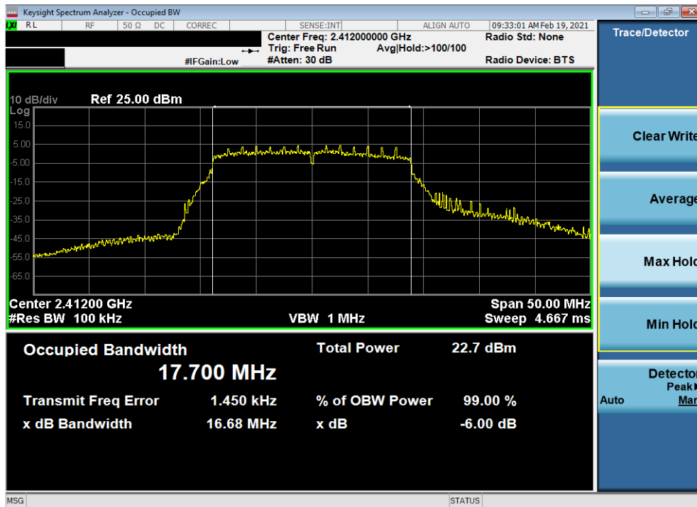
Plot 7-34. 6dB Bandwidth Plot Antenna 2a (802.11n (2.4GHz) – Ch. 1) – MCS0
