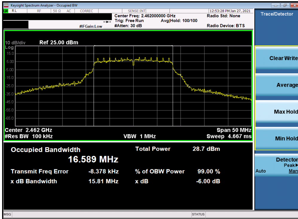
Plot 7-33. 6dB Bandwidth Plot Antenna 2a (802.11g – Ch. 11) – 6Mbps
