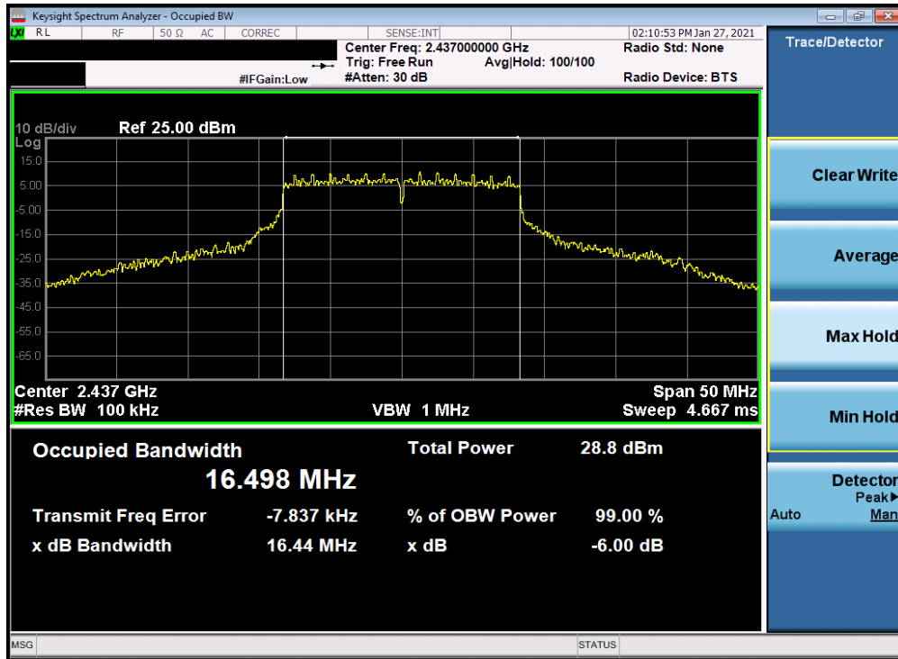
Plot 7-53. 6dB Bandwidth Plot Antenna 2a (802.11g – Ch. 6) – 54Mbps
