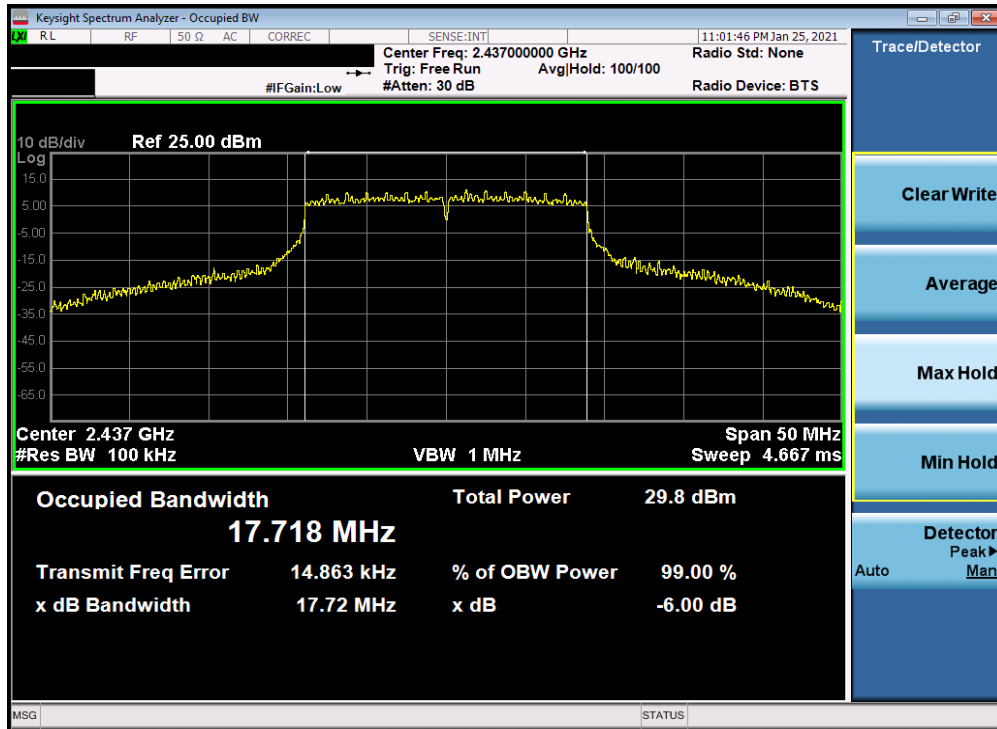
Plot 7-56. 6dB Bandwidth Plot Antenna 2a (802.11n (2.4GHz) – Ch. 6) – MCS7
