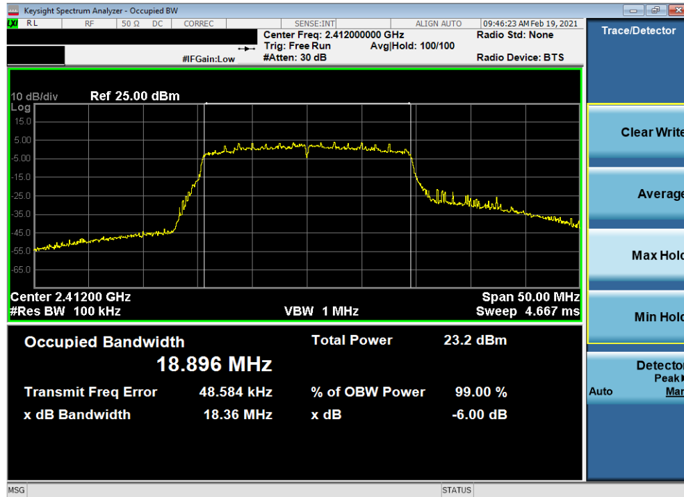
Plot 7-37. 6dB Bandwidth Plot Antenna 2a (802.11ax (SU - 2.4GHz) – Ch. 1) – MCS0
