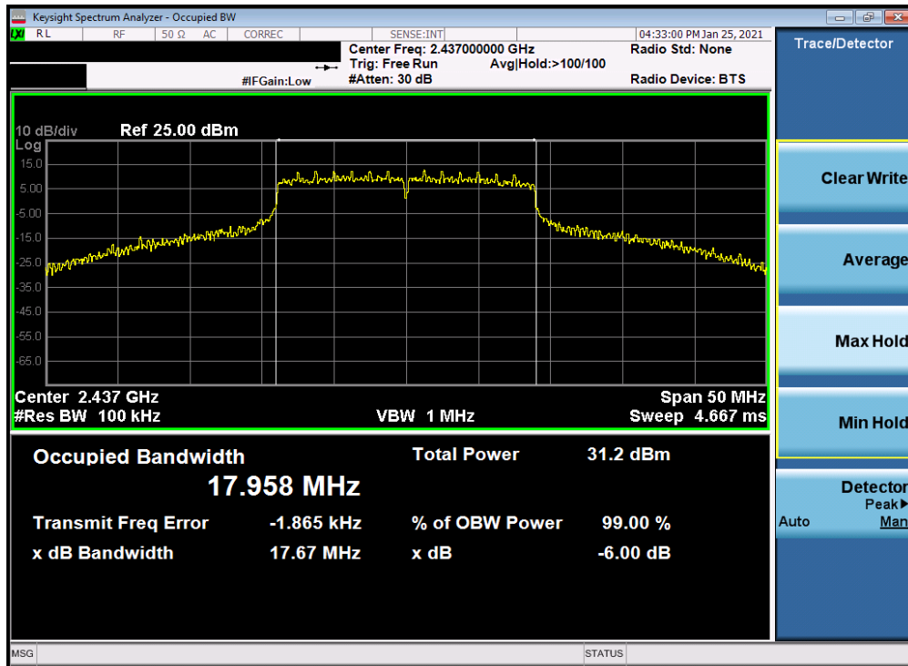
Plot 7-26. 6dB Bandwidth Plot Antenna 4a (802.11n (2.4GHz) – Ch. 6) – MCS7
