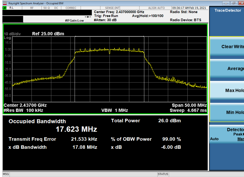
Plot 7-35. 6dB Bandwidth Plot Antenna 2a (802.11n (2.4GHz) – Ch. 6) – MCS0
