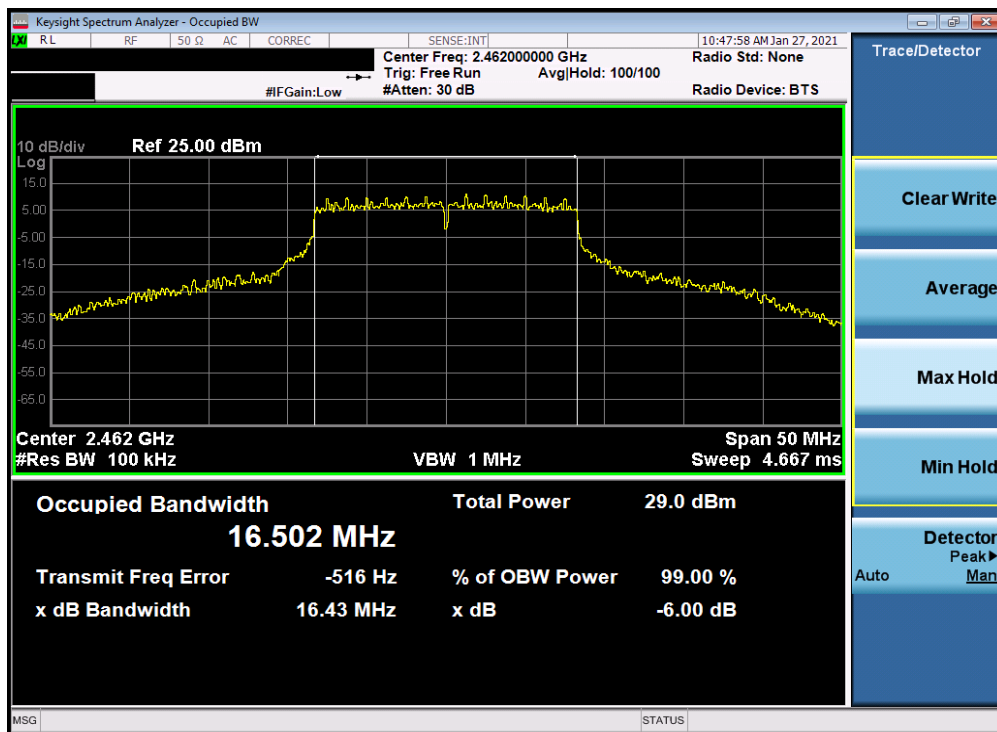
Plot 7-24. 6dB Bandwidth Plot Antenna 4a (802.11g – Ch. 11) – 54Mbps
