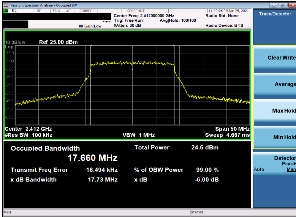
Plot 7-55. 6dB Bandwidth Plot Antenna 2a (802.11n (2.4GHz) – Ch. 1) – MCS7
