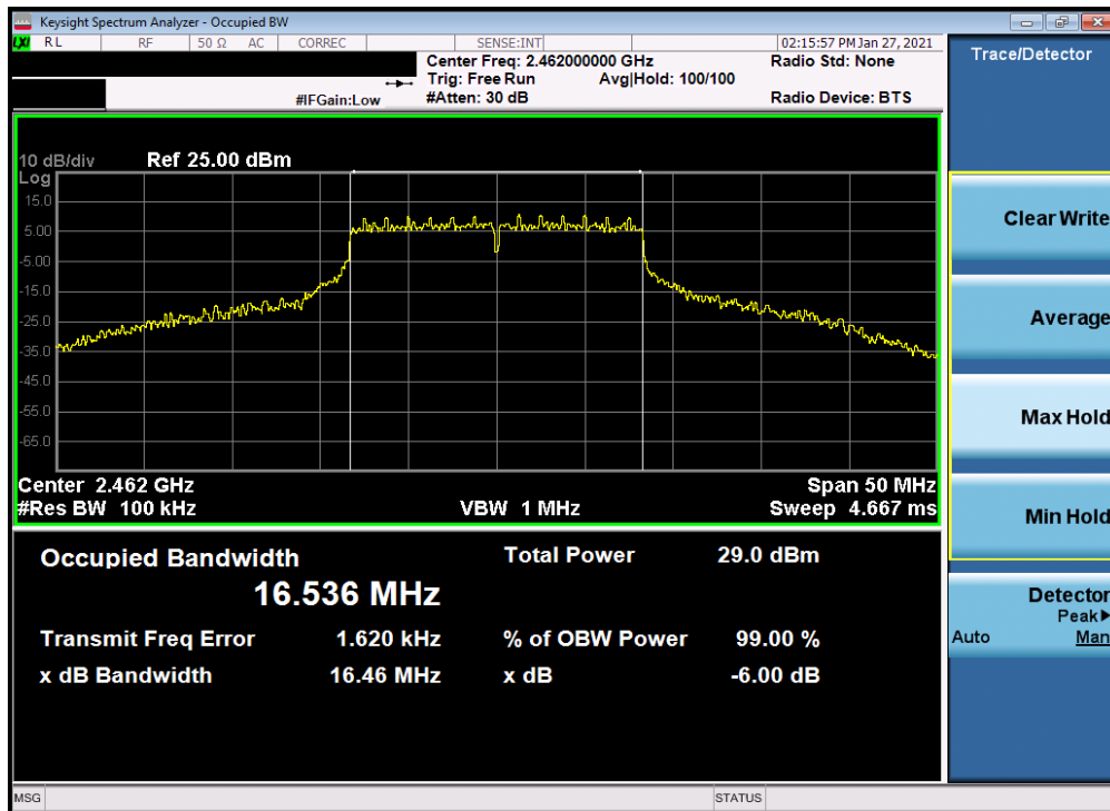
Plot 7-54. 6dB Bandwidth Plot Antenna 2a (802.11g – Ch. 11) – 54Mbps
