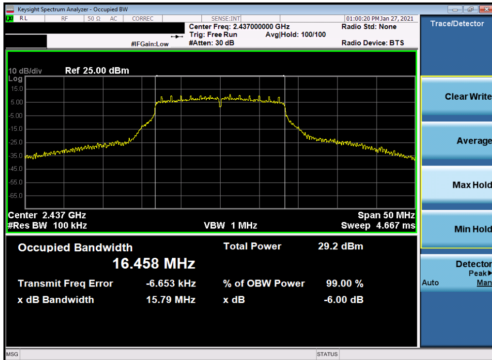
Plot 7-32. 6dB Bandwidth Plot Antenna 2a (802.11g – Ch. 6) – 6Mbps
