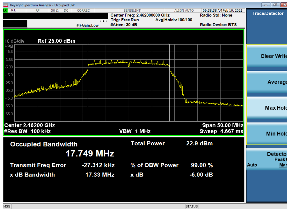
Plot 7-36. 6dB Bandwidth Plot Antenna 2a (802.11n (2.4GHz) – Ch. 11) – MCS0
