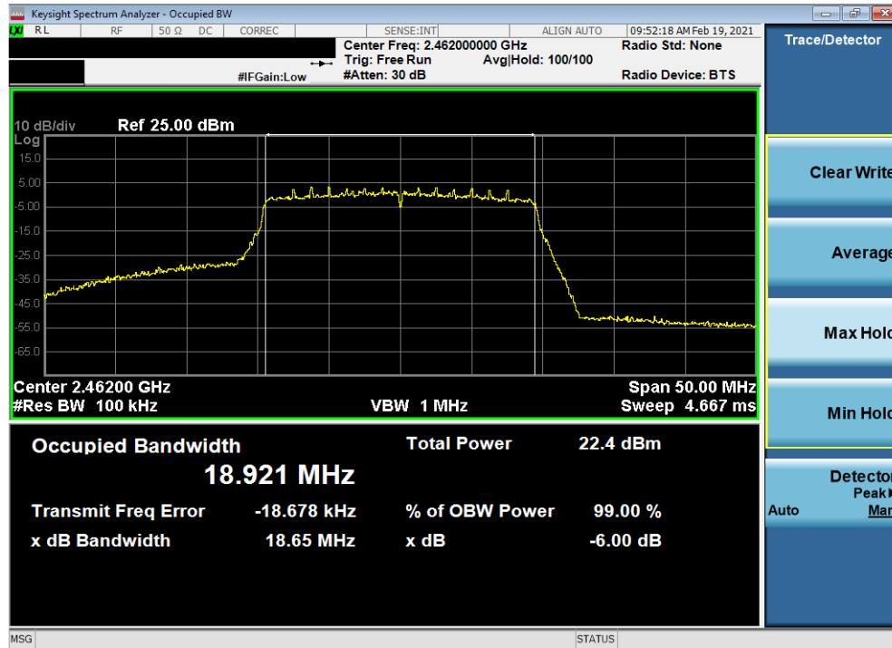
Plot 7-39. 6dB Bandwidth Plot Antenna 2a (802.11ax (SU - 2.4GHz) – Ch. 11) – MCS0
