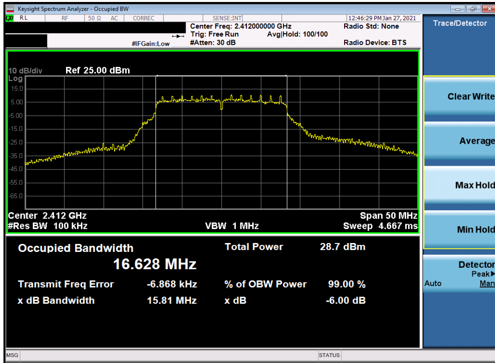
Plot 7-31. 6dB Bandwidth Plot Antenna 2a (802.11g – Ch. 1) – 6Mbps
