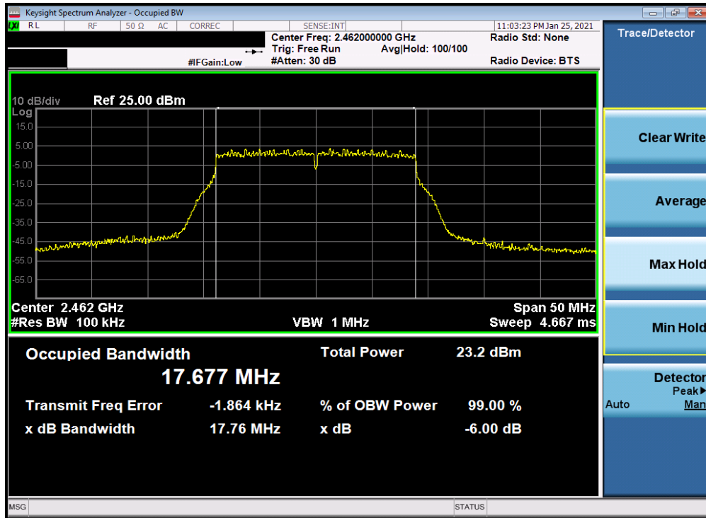
Plot 7-57. 6dB Bandwidth Plot Antenna 2a (802.11n (2.4GHz) – Ch. 11) – MCS7
