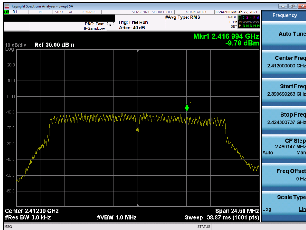
Plot 7-94. Power Spectral Density Plot Antenna 2a (802.11n (2.4GHz) – Ch. 1) – MCS0
