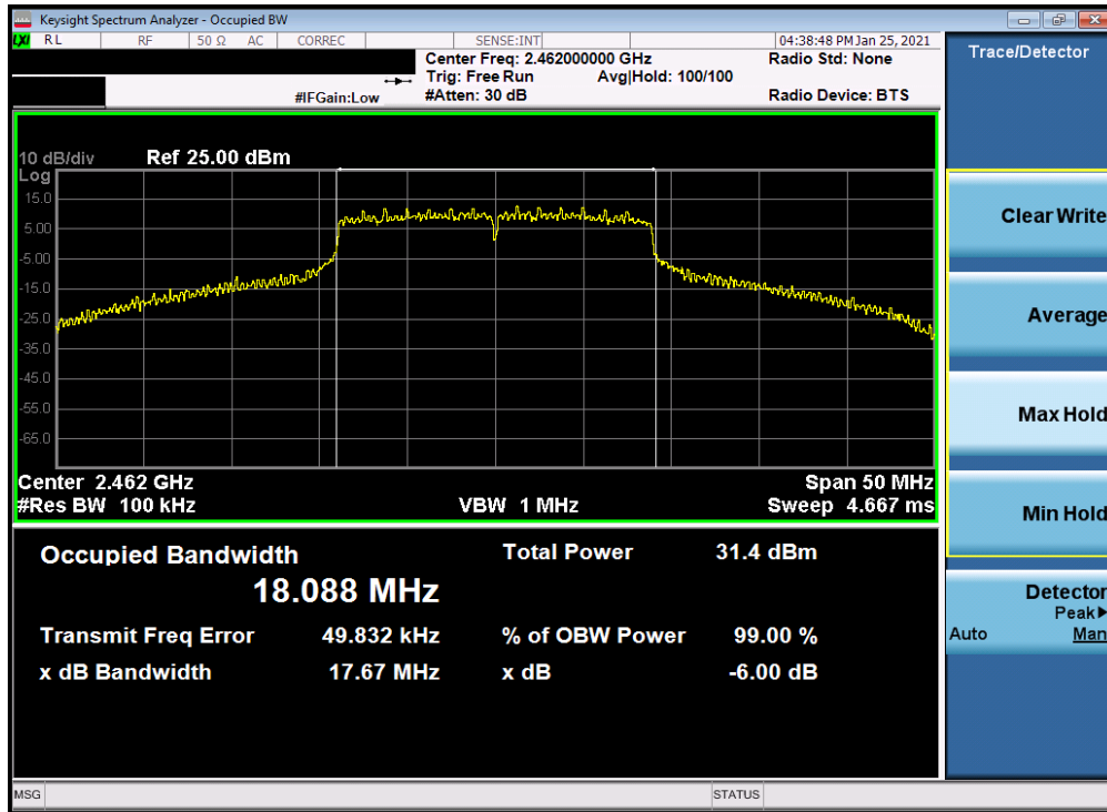
Plot 7-27. 6dB Bandwidth Plot Antenna 4a (802.11n (2.4GHz) – Ch. 11) – MCS7
