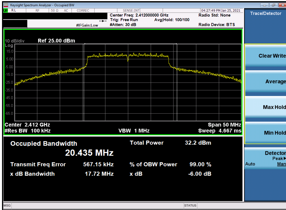
Plot 7-25. 6dB Bandwidth Plot Antenna 4a (802.11n (2.4GHz) – Ch. 1) – MCS7
