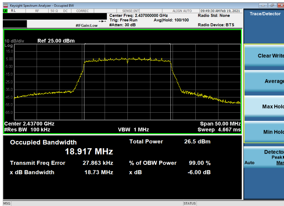
Plot 7-38. 6dB Bandwidth Plot Antenna 2a (802.11ax (SU - 2.4GHz) – Ch. 6) – MCS0
