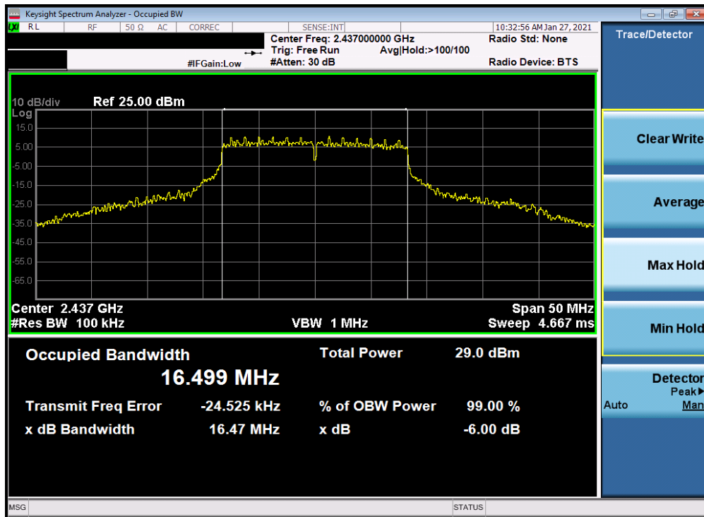
Plot 7-23. 6dB Bandwidth Plot Antenna 4a (802.11g – Ch. 6) – 54Mbps
