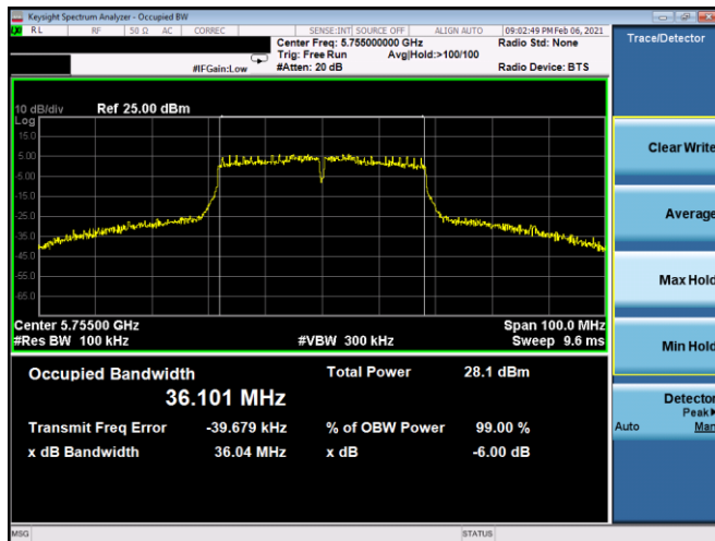
Plot 7-135. 6dB BW & 99% OBW Antenna 4b (40MHz BW 802.11n – Ch. 151, MCS3)
