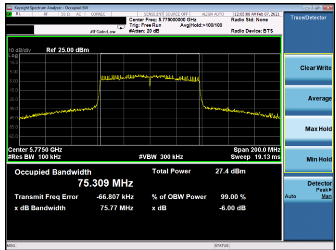
Plot 7-137. 6dB BW & 99% OBW Antenna 4b (80MHz BW 802.11ac – Ch. 155, MCS3)
