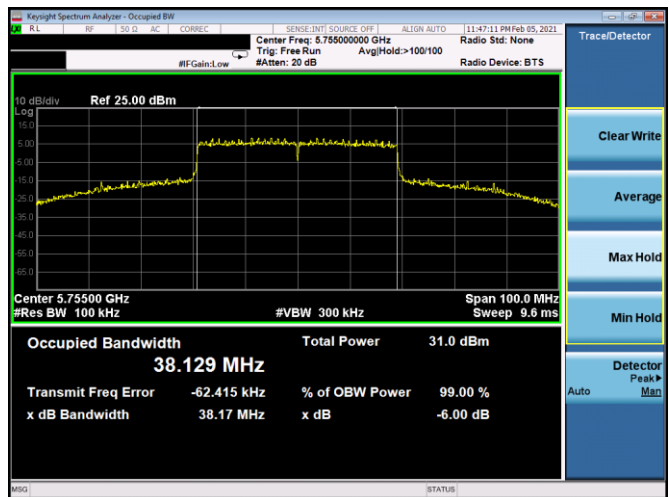
Plot 7-136. 6dB BW & 99% OBW Antenna 4b (40MHz BW 802.11ax (SU) – Ch. 151, MCS3)
