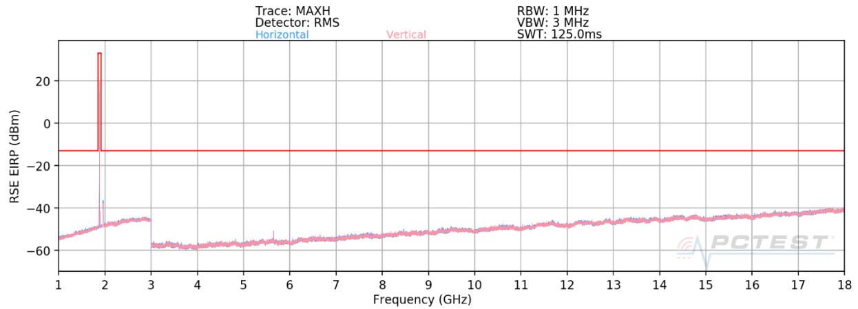
Plot 7-263. Radiated Spurious Plot (LTE Band 25/2)
