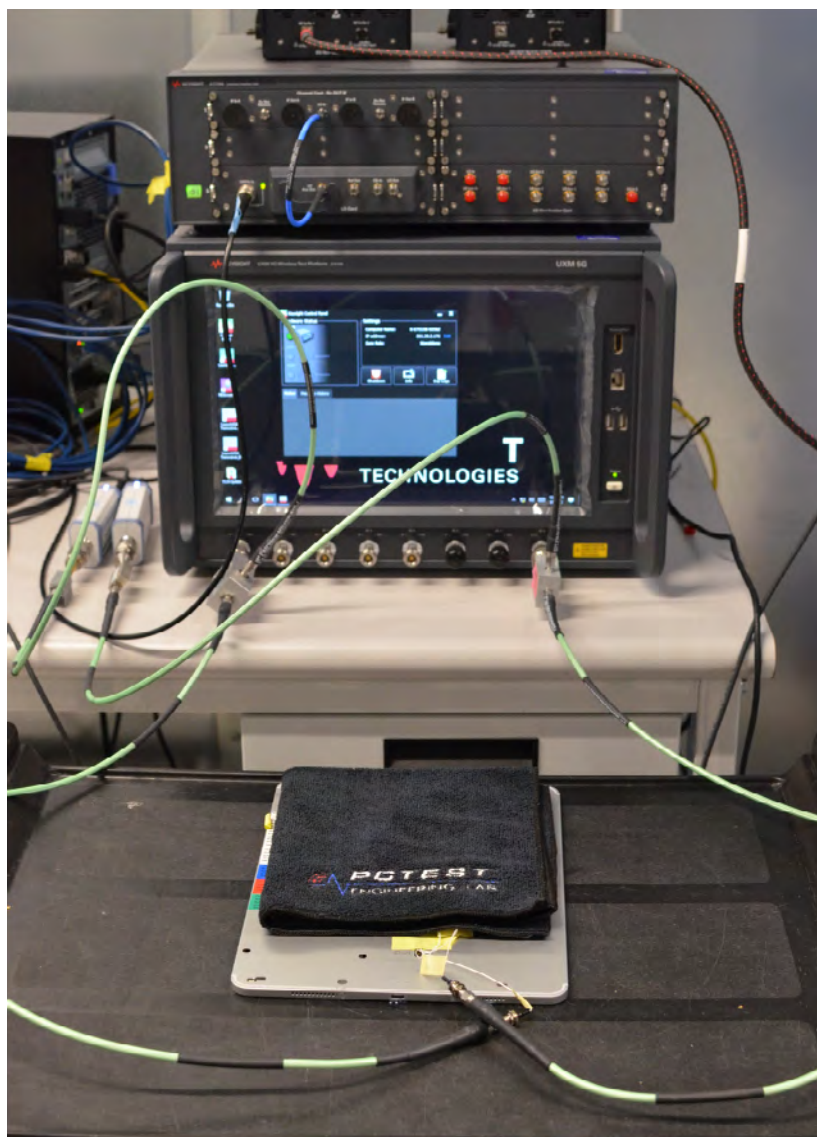
Test Setup Photo 5 – Conducted Test Setup (Figure 6-1e)
