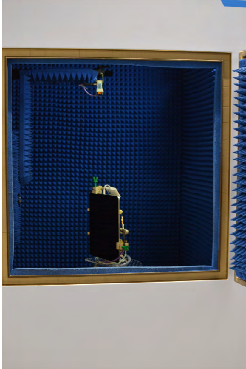
Test Setup Photo 12 – Radiated Power Measurement Setup (Figure 7-1)
