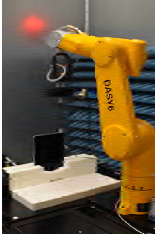
Test Setup Photo 11 – Power Density Setup (Figure 7-2)
