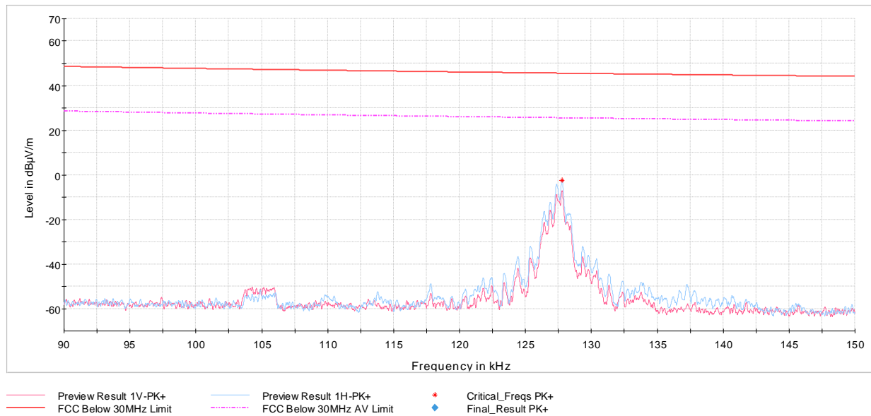
Plot 6-2. Radiated Restricted Lower Band Edge Peak Measurement (Charging Rate 10C)
