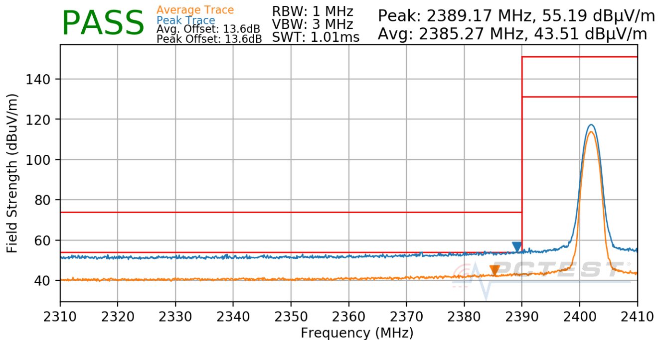
Plot 7-73. Radiated Restricted Lower Band Edge Measurement Antenna 7 (Average & Peak)
