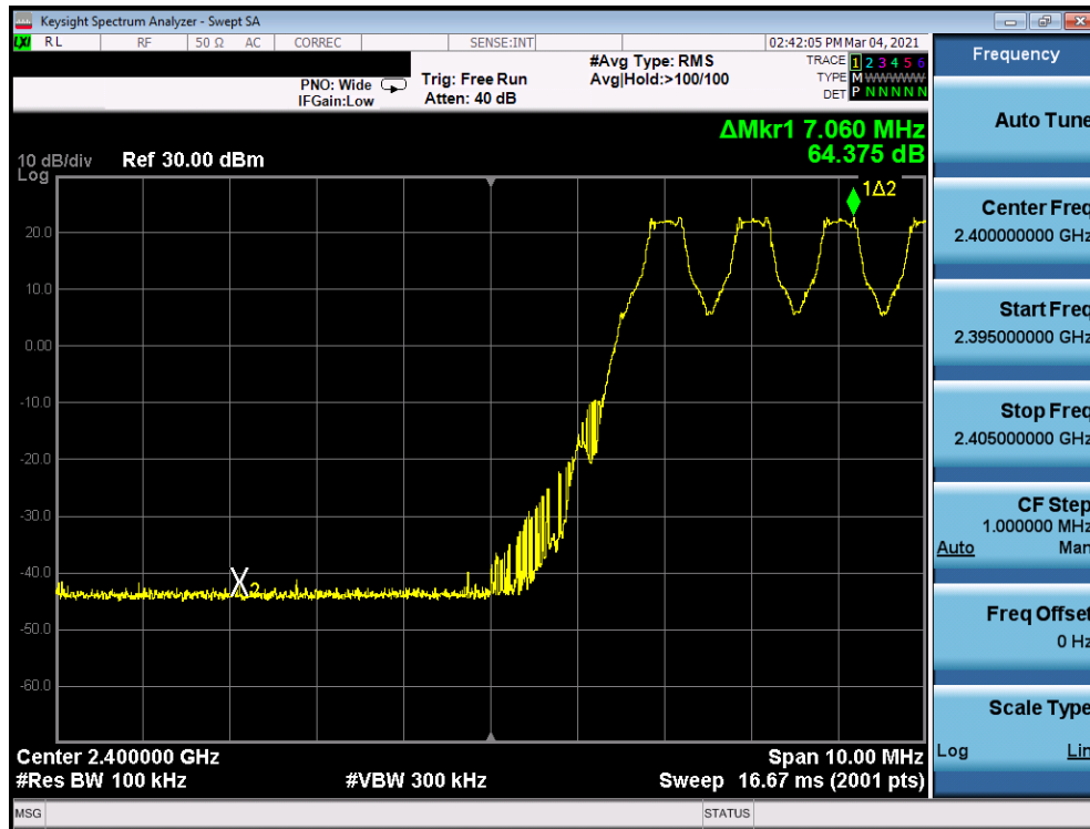
Plot 7-23. Band Edge Plot Antenna 7 (Bluetooth with Hopping Enabled, GFSK, ePA)
