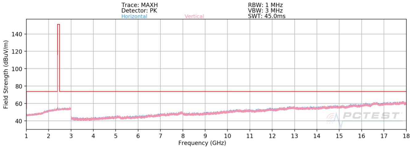
Plot 7-60. Radiated Spurious Emissions above 1GHz Antenna 7 (BT GFSK ePA – Ch. 0)
