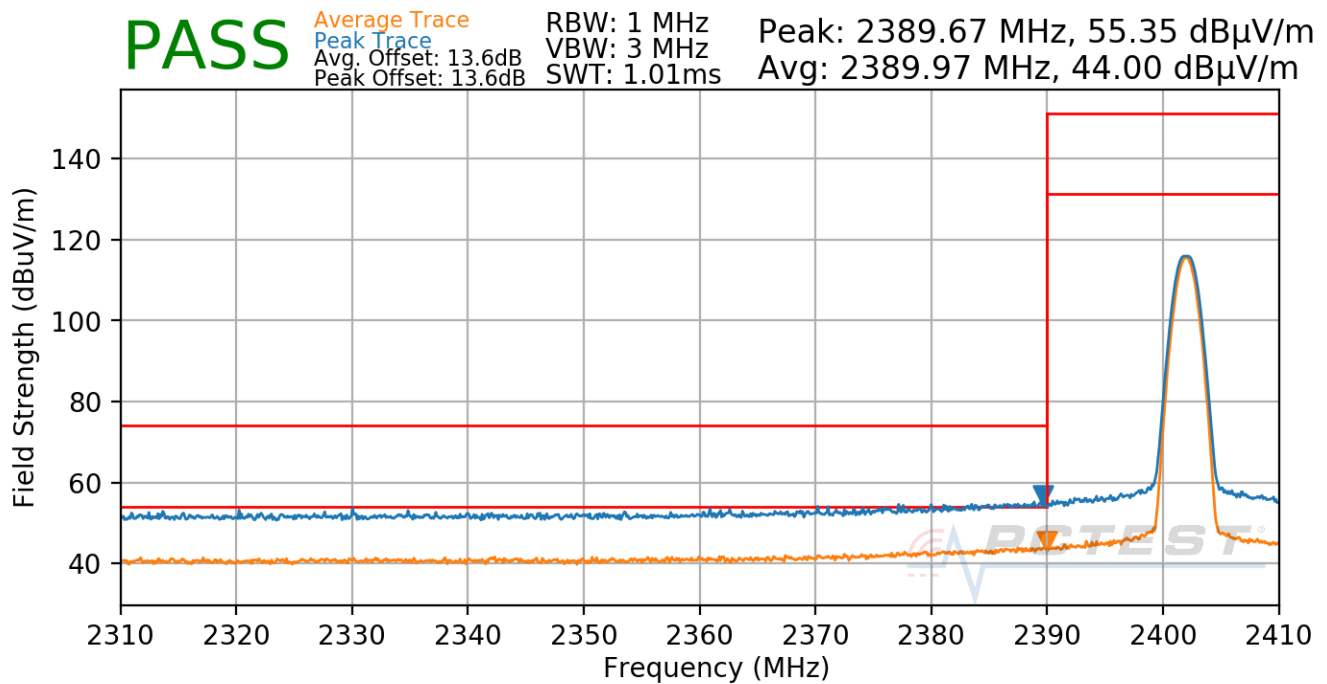
Plot 7-68. Radiated Restricted Lower Band Edge Measurement Antenna 8 (Average & Peak)
