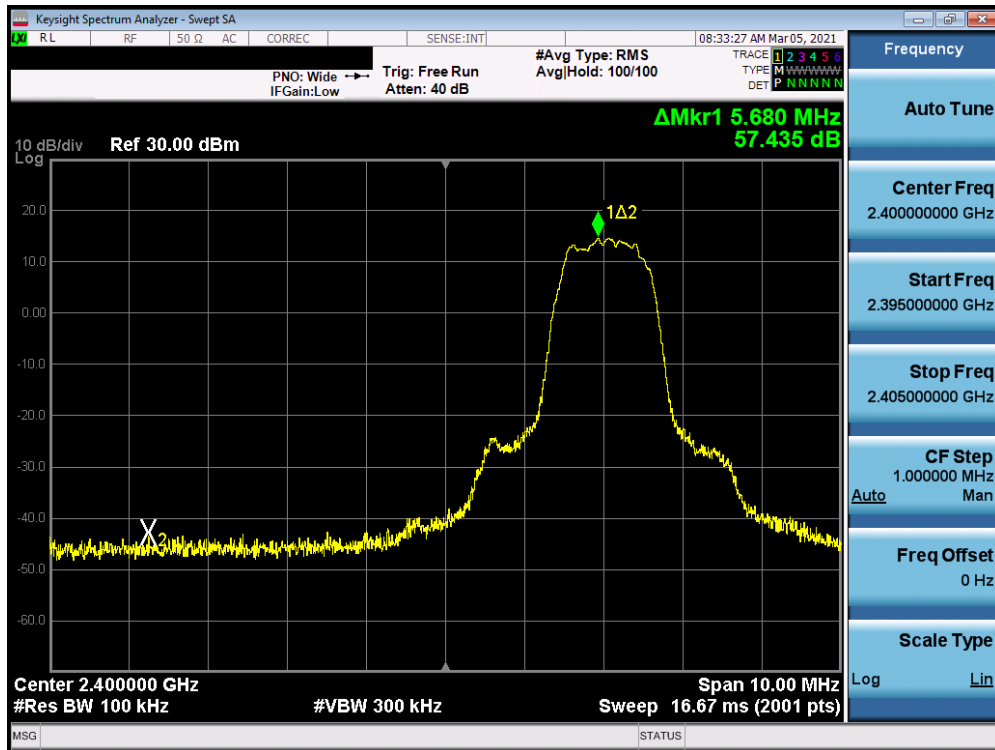
Plot 7-17. Band Edge Plot Antenna 8 (Bluetooth with Hopping Disabled, 8DPSK, ePA – Ch. 0)
