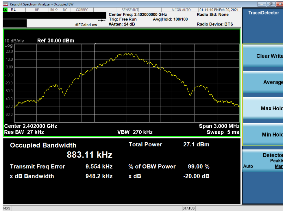
Plot 7-7. 20dB BW and 99% OBW Plot Antenna 7 (Bluetooth, GFSK, ePA – Ch. 0)
