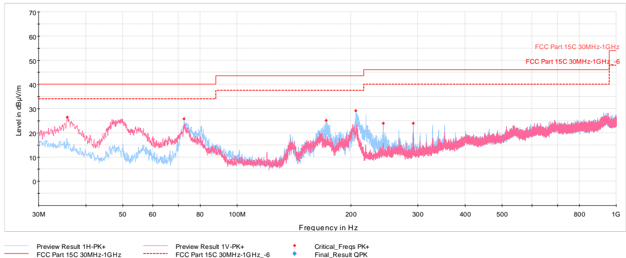
Plot 7-80. Radiated Spurious Emissions below 1GHz TxBF (GFSK ePA – Ch.0, with AC/DC Adapter)
