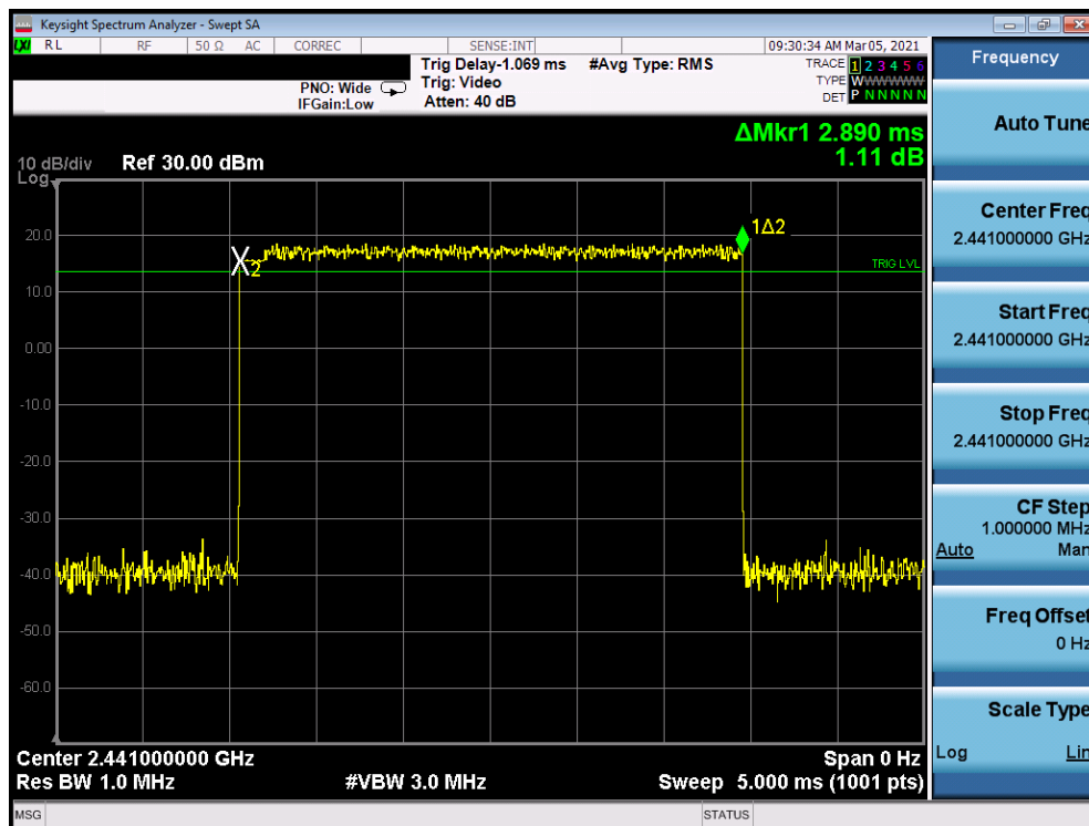
Plot 7-34. Time of Occupancy Plot Antenna 8 (Bluetooth, 8DPSK, ePA)
