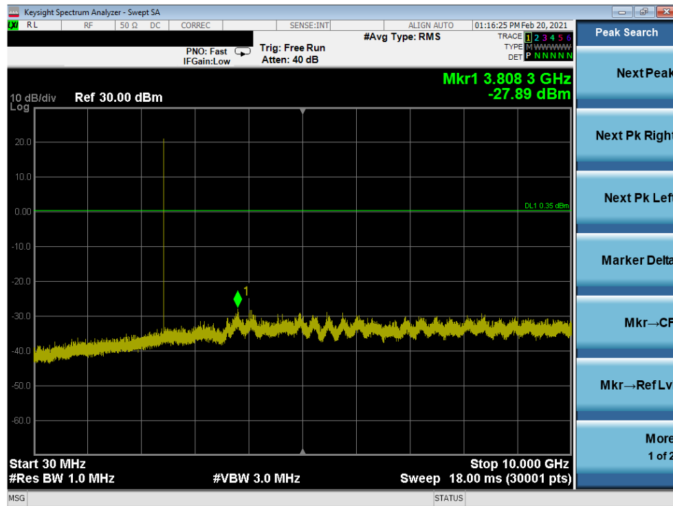
Plot 7-53. Conducted Spurious Plot Antenna 7 (Bluetooth, GFSK, ePA – Ch. 39)
