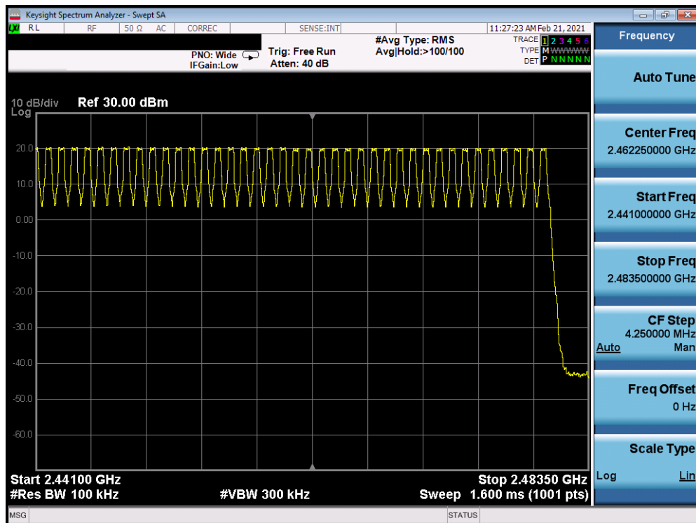
Plot 7-42. High End Spectrum Channel Hopping Plot Antenna 7 (Bluetooth, GFSK, ePA)
