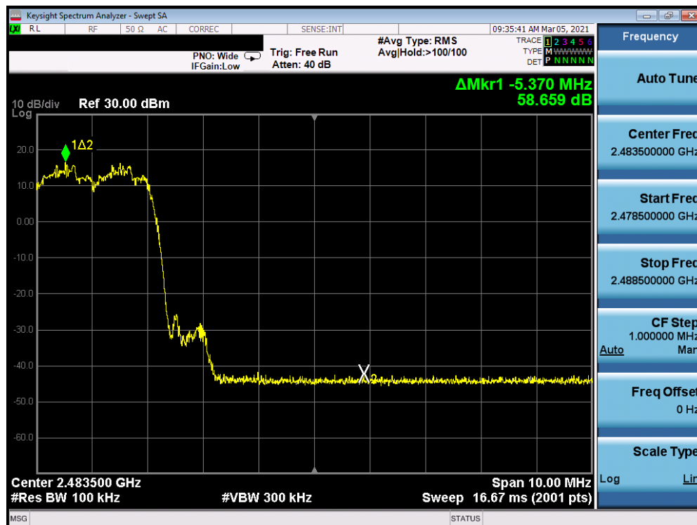
Plot 7-20. Band Edge Plot Antenna 8 (Bluetooth with Hopping Enabled, 8DPSK, ePA)
