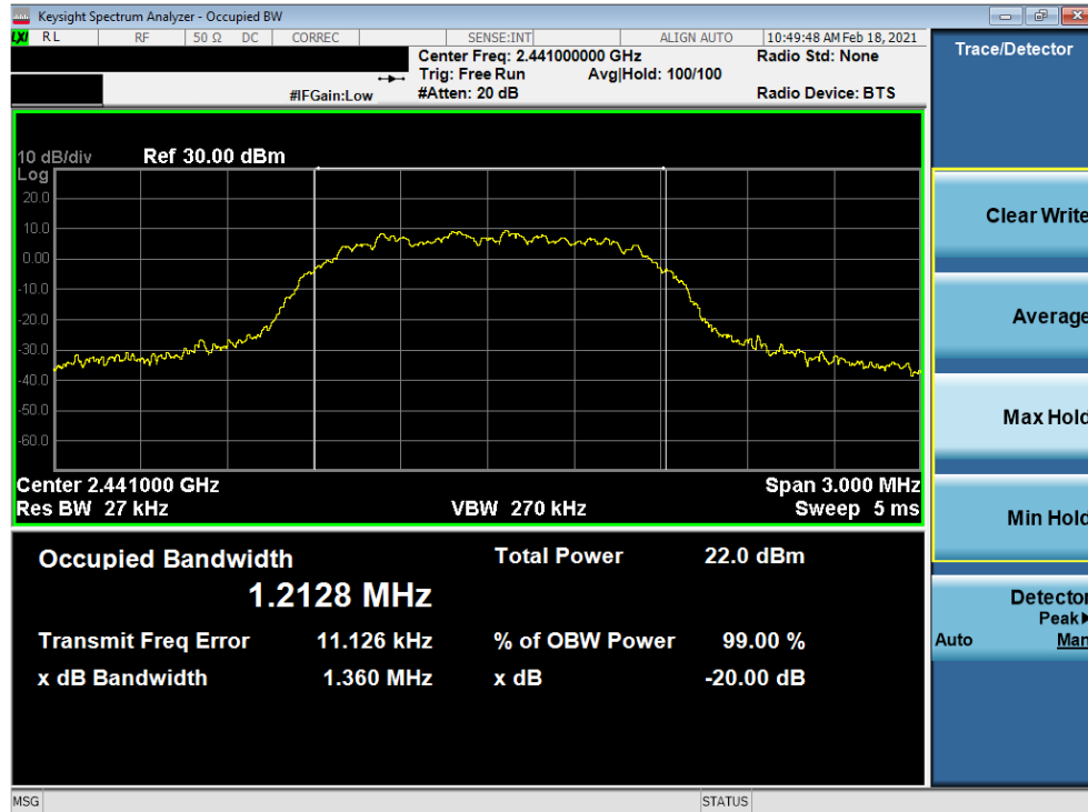
Plot 7-5. 20dB BW and 99% OBW Plot Antenna 8 (Bluetooth, 8DPSK, ePA – Ch. 39)
