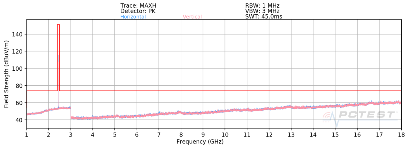
Plot 7-58. Radiated Spurious Emissions above 1GHz Antenna 8 (BT GFSK ePA – Ch. 39)
