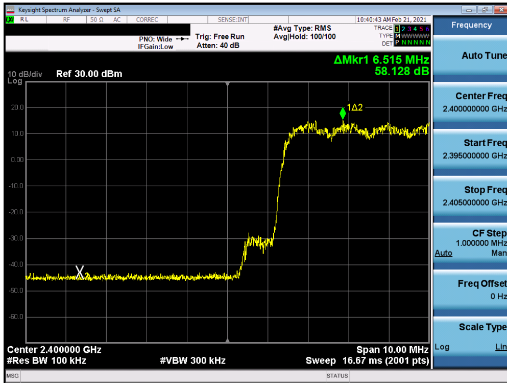
Plot 7-27. Band Edge Plot Antenna 7 (Bluetooth with Hopping Enabled, 8DPSK, ePA)
