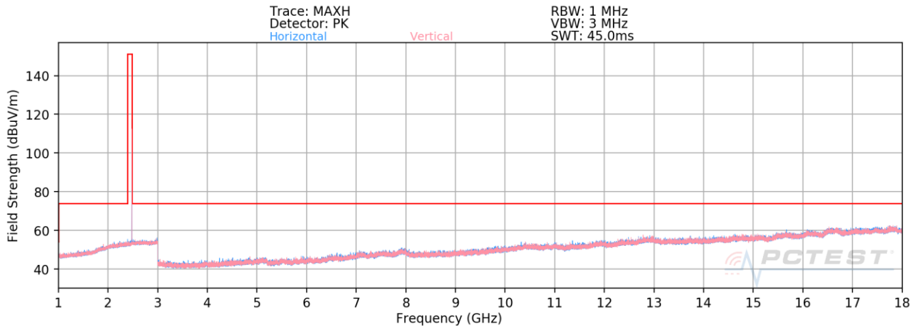
Plot 7-62. Radiated Spurious Emissions above 1GHz Antenna 7 (BT GFSK ePA – Ch. 78)
