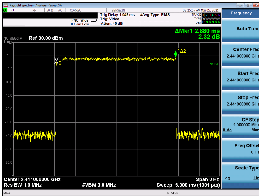
Plot 7-36. Time of Occupancy Plot Antenna 7 (Bluetooth, 8DPSK, ePA)
