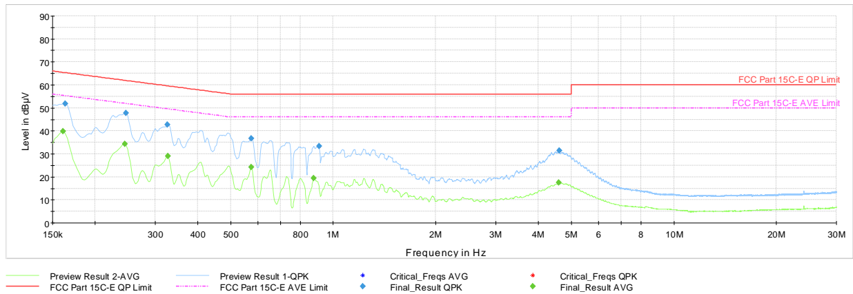
Plot 7-82. AC Line-Conducted Test Plot TxBF (N, GFSK ePA – Ch.0, with AC/DC Adapter)
