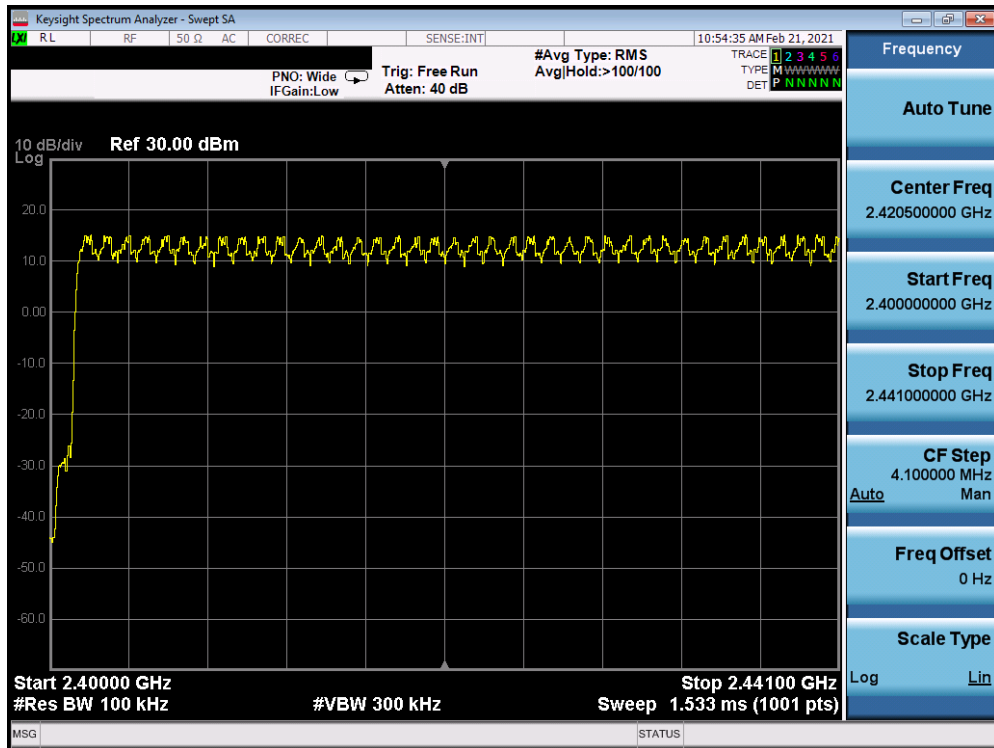
Plot 7-43. Low End Spectrum Channel Hopping Plot Antenna 7 (Bluetooth, 8DPSK, ePA)
