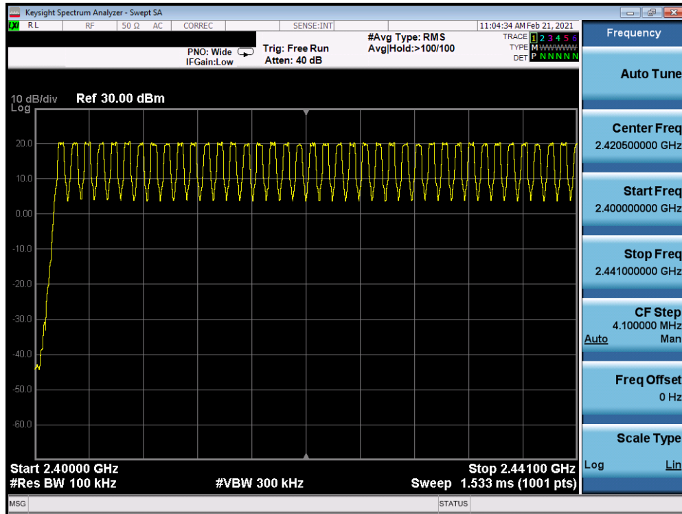
Plot 7-41. Low End Spectrum Channel Hopping Plot Antenna 7 (Bluetooth, GFSK, ePA)
