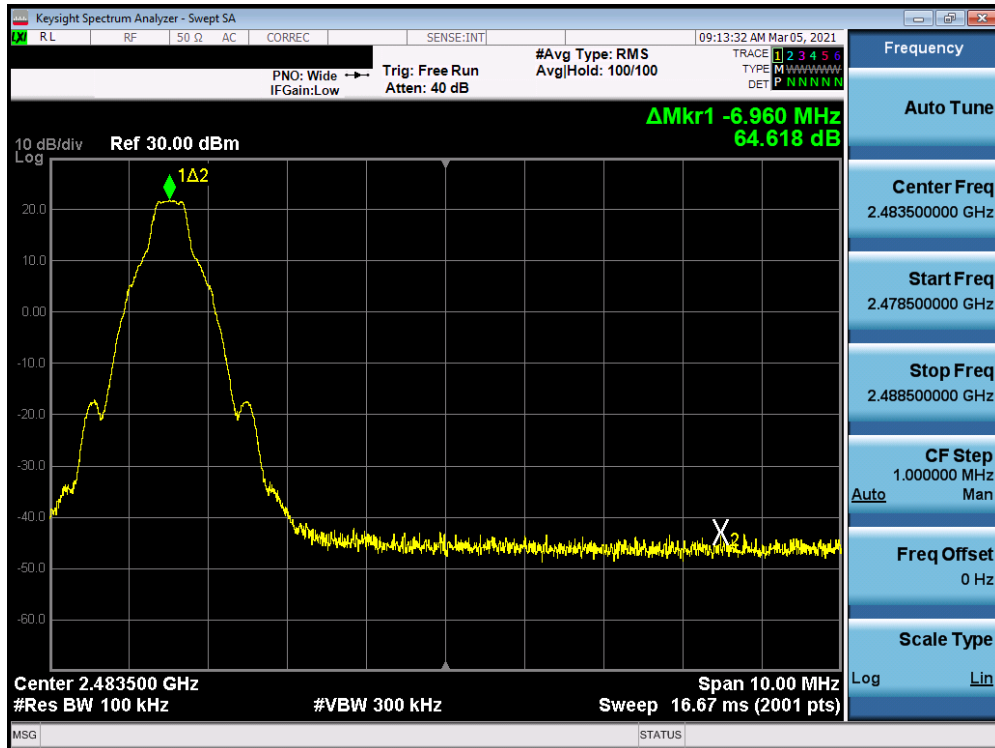
Plot 7-22. Band Edge Plot Antenna 7 (Bluetooth with Hopping Disabled, GFSK, ePA – Ch. 78)
