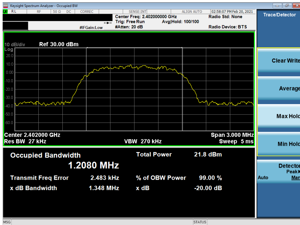
Plot 7-10. 20dB BW and 99% OBW Plot Antenna 7 (Bluetooth, 8DPSK, ePA – Ch. 0)
