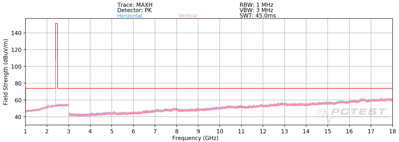
Plot 7-57. Radiated Spurious Emissions above 1GHz Antenna 8 (BT GFSK ePA – Ch. 0)
