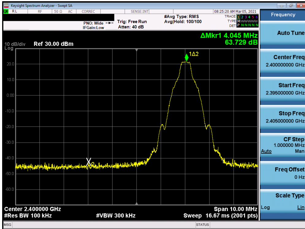
Plot 7-13. Band Edge Plot Antenna 8 (Bluetooth with Hopping Disabled, GFSK, ePA – Ch. 0)
