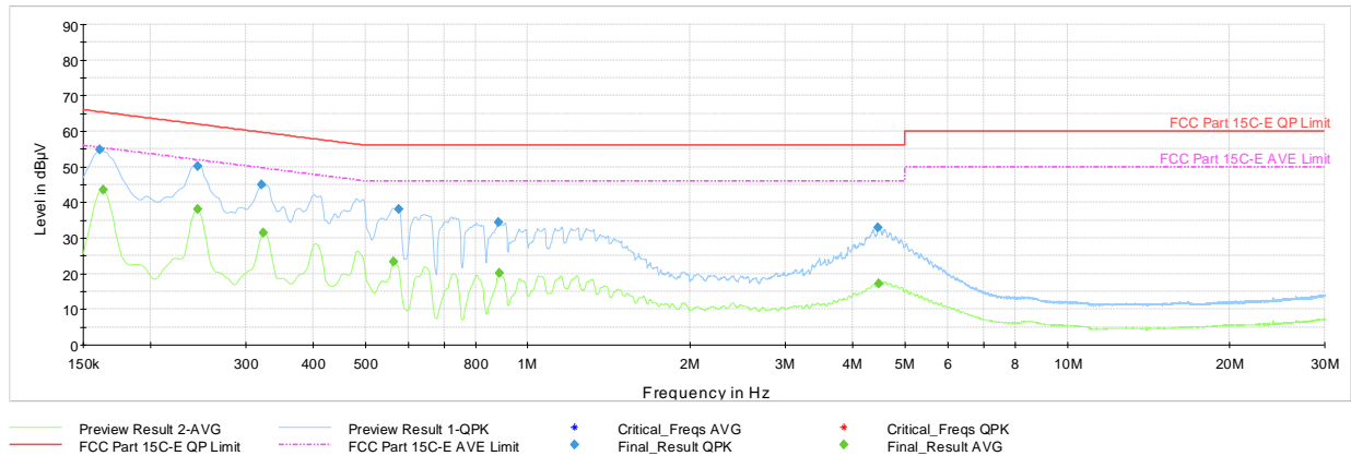
Plot 7-81. AC Line-Conducted Test Plot TxBF (L1, GFSK ePA – Ch.0, with AC/DC Adapter)
