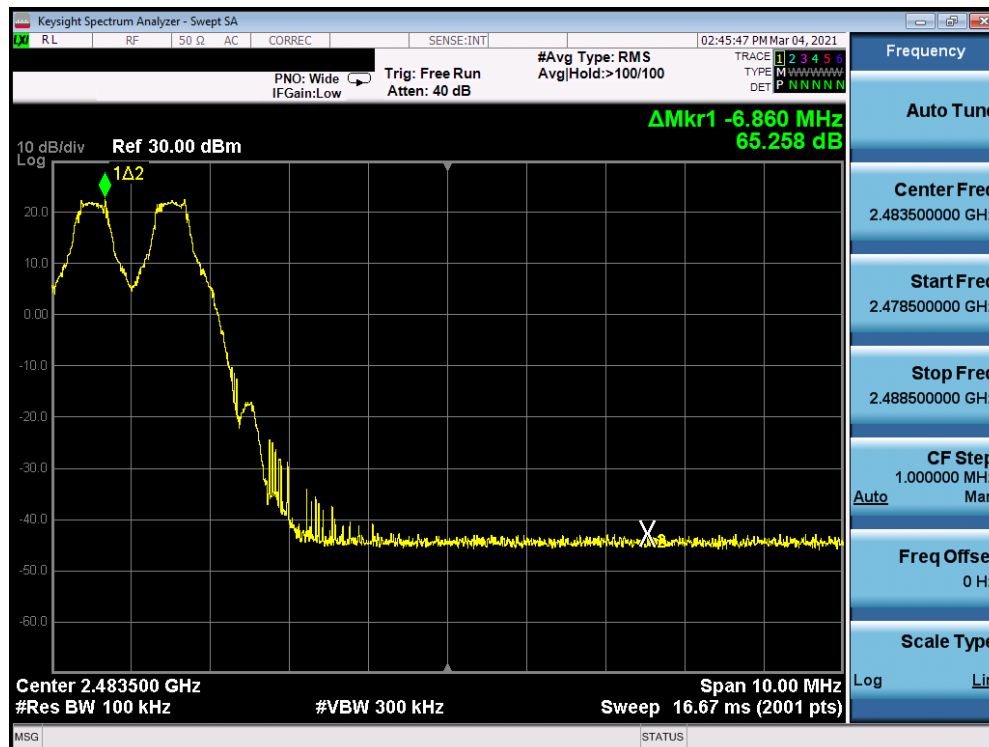
Plot 7-24. Band Edge Plot Antenna 7 (Bluetooth with Hopping Enabled, GFSK, ePA)
