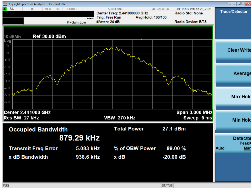
Plot 7-8. 20dB BW and 99% OBW Plot Antenna 7 (Bluetooth, GFSK, ePA – Ch. 39)
