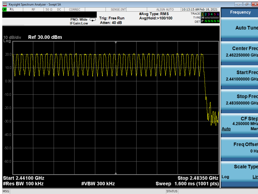
Plot 7-38. High End Spectrum Channel Hopping Plot Antenna 8 (Bluetooth, GFSK, ePA)
