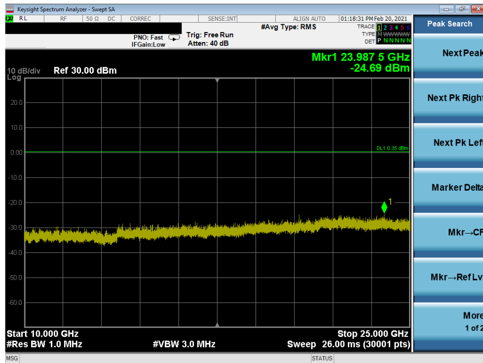
Plot 7-54. Conducted Spurious Plot Antenna 7 (Bluetooth, GFSK, ePA Ch. 39)
