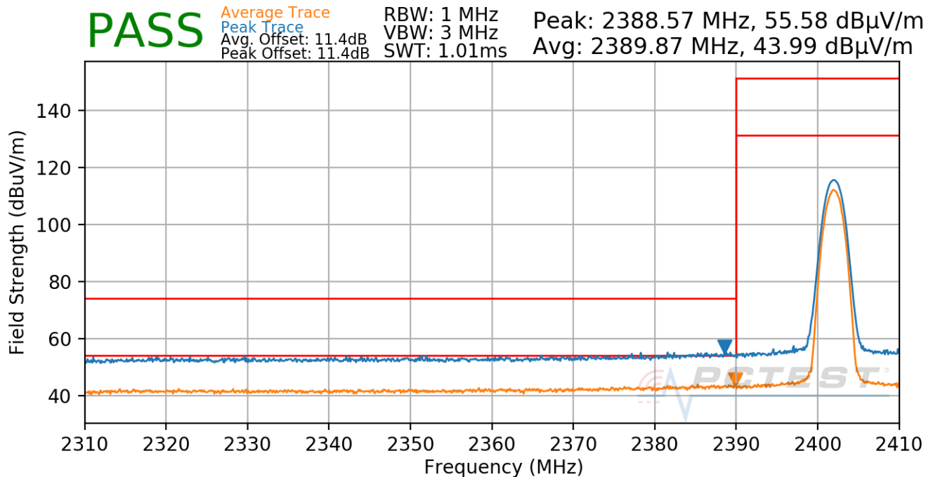
Plot 7-69. Radiated Restricted Lower Band Edge Measurement Antenna 8 (Average & Peak)
