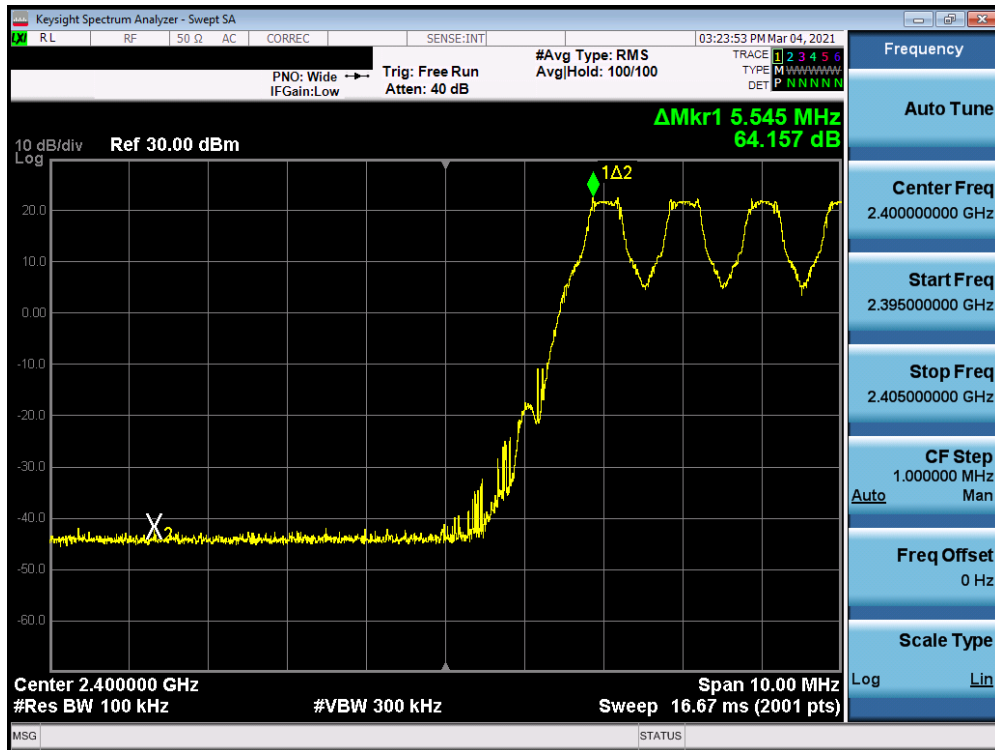
Plot 7-15. Band Edge Plot Antenna 8 (Bluetooth with Hopping Enabled, GFSK, ePA)
