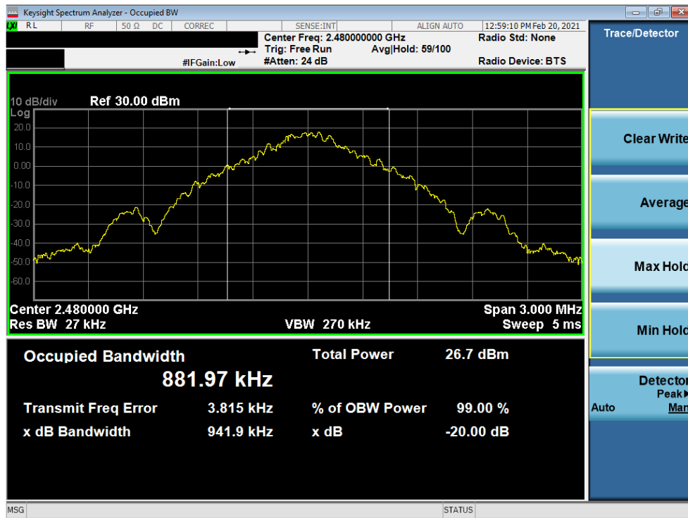
Plot 7-9. 20dB BW and 99% OBW Plot Antenna 7 (Bluetooth, GFSK, ePA – Ch. 78)
