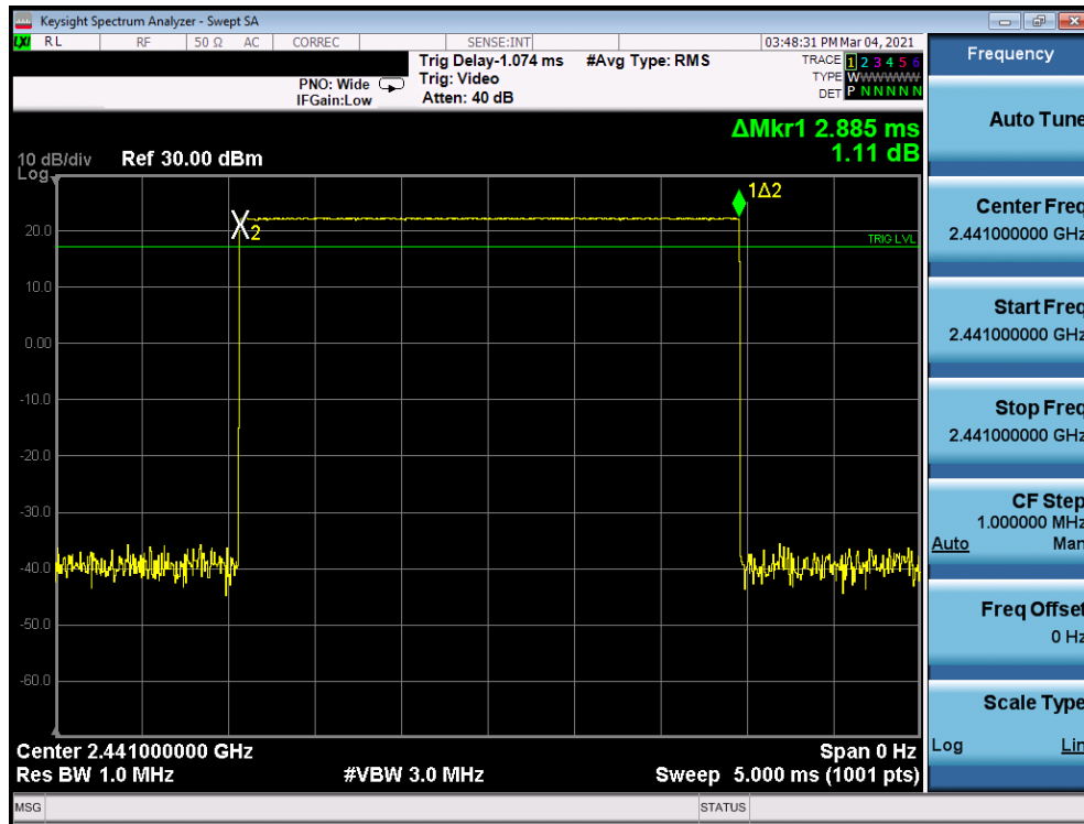
Plot 7-33. Time of Occupancy Plot Antenna 8 (Bluetooth, GFSK, ePA)
