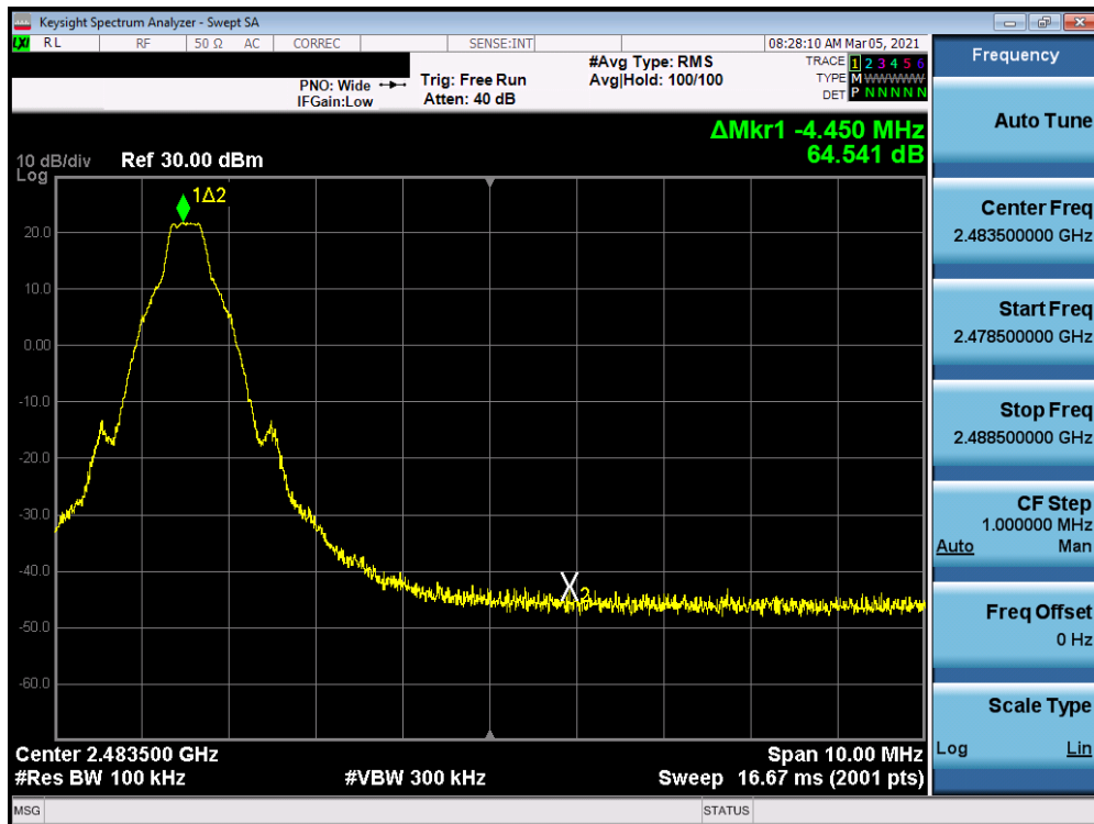
Plot 7-14. Band Edge Plot Antenna 8 (Bluetooth with Hopping Disabled, GFSK, ePA – Ch. 78)
