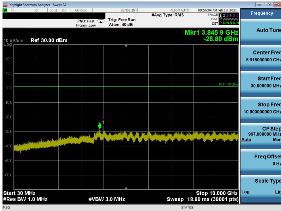
Plot 7-45. Conducted Spurious Plot Antenna 8 (Bluetooth, GFSK, ePA – Ch. 0)
