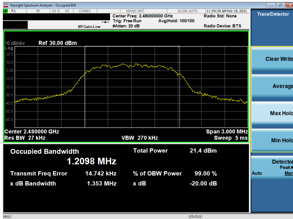
Plot 7-6. 20dB BW and 99% OBW Plot Antenna 8 (Bluetooth, 8DPSK, ePA – Ch. 78)
