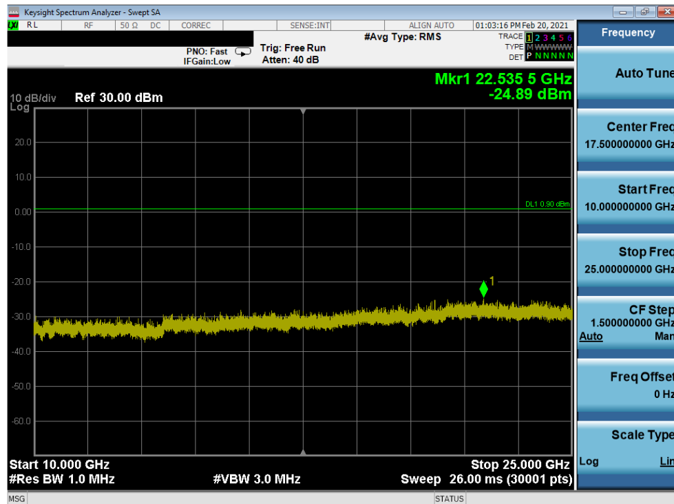
Plot 7-56. Conducted Spurious Plot Antenna 7 (Bluetooth, GFSK, ePA – Ch. 78)
