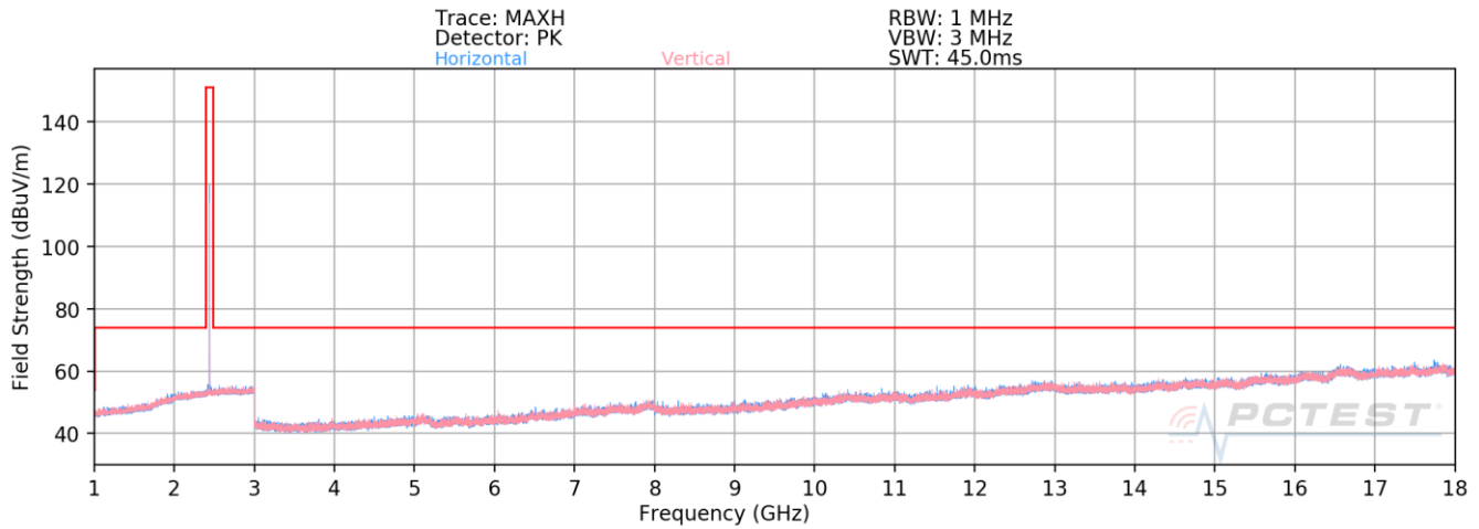
Plot 7-61. Radiated Spurious Emissions above 1GHz Antenna 7 (BT GFSK ePA – Ch. 39)
