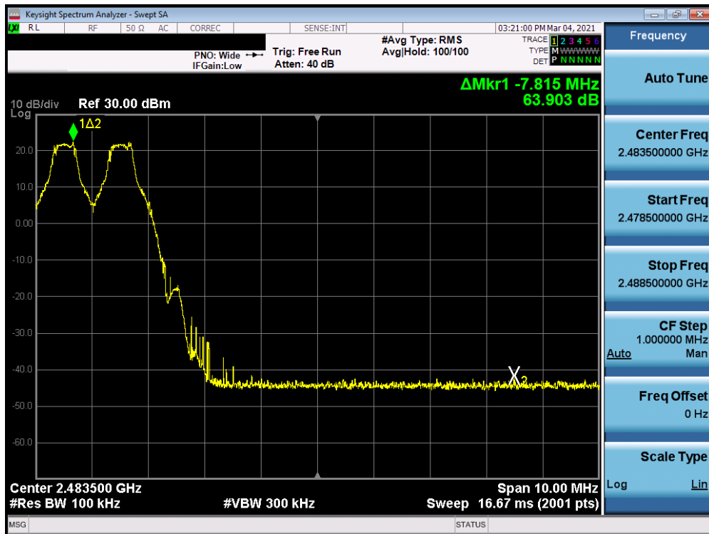
Plot 7-16. Band Edge Plot Antenna 8 (Bluetooth with Hopping Enabled, GFSK, ePA)
