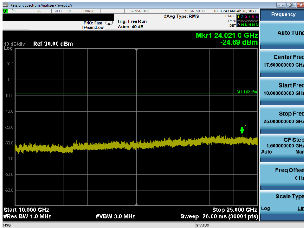
Plot 7-52. Conducted Spurious Plot Antenna 7 (Bluetooth, GFSK, ePA – Ch. 0)
