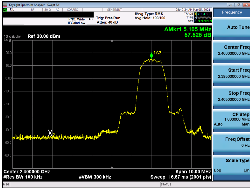
Plot 7-25. Band Edge Plot Antenna 7 (Bluetooth with Hopping Disabled, 8DPSK, ePA – Ch. 0)
