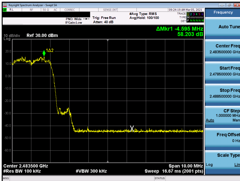
Plot 7-28. Band Edge Plot Antenna 7 (Bluetooth with Hopping Enabled, 8DPSK, ePA)
