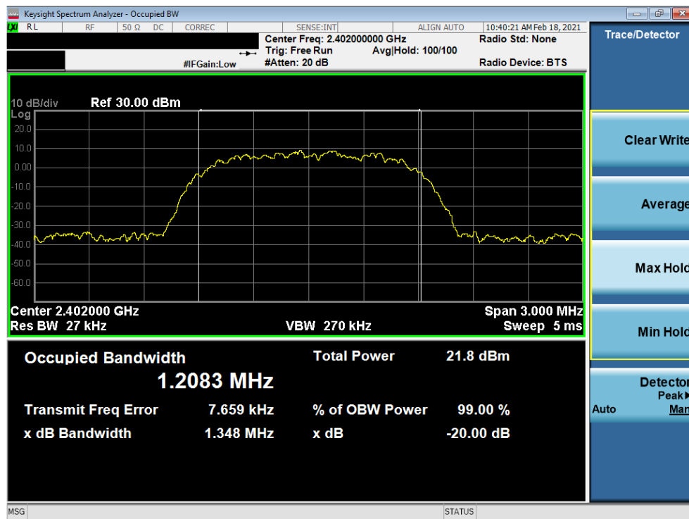
Plot 7-4. 20dB BW and 99% OBW Plot Antenna 8 (Bluetooth, 8DPSK, ePA – Ch. 0)
