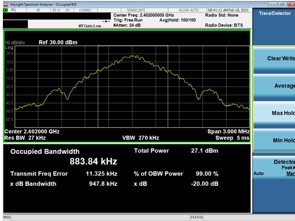
Plot 7-1. 20dB BW and 99% OBW Plot Antenna 8 (Bluetooth, GFSK, ePA – Ch. 0)
