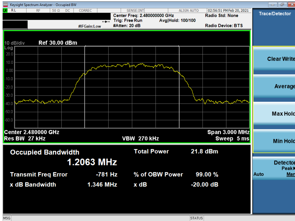
Plot 7-12. 20dB BW and 99% OBW Plot Antenna 7 (Bluetooth, 8DPSK, ePA – Ch. 78)
