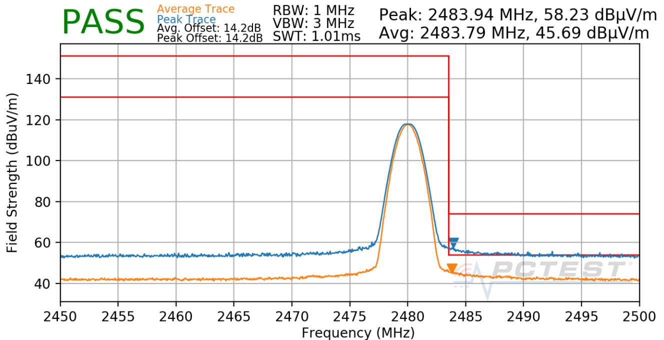
Plot 7-74. Radiated Restricted Upper Band Edge Measurement Antenna 7 (Average & Peak)
