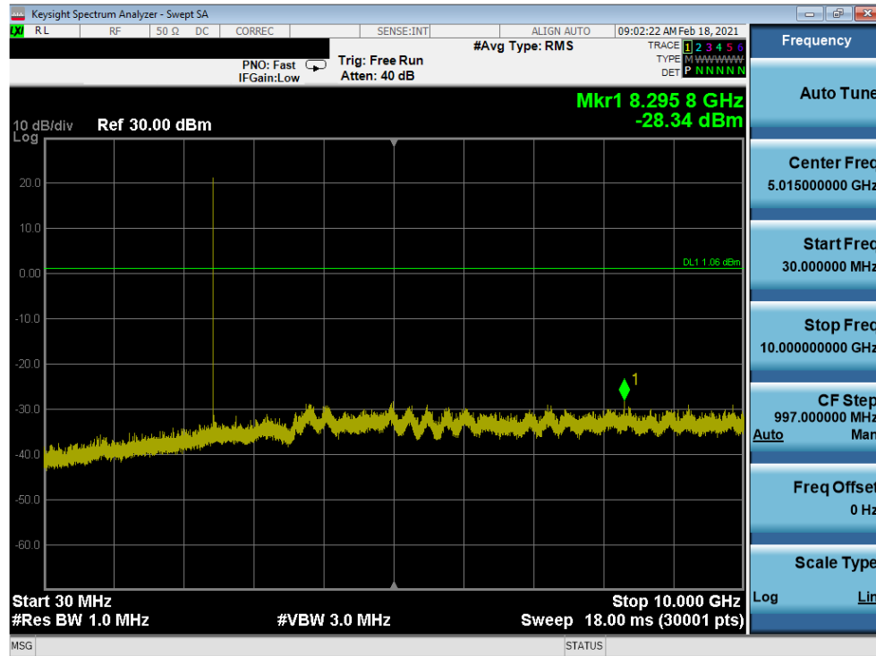
Plot 7-47. Conducted Spurious Plot Antenna 8 (Bluetooth, GFSK, ePA – Ch. 39)
