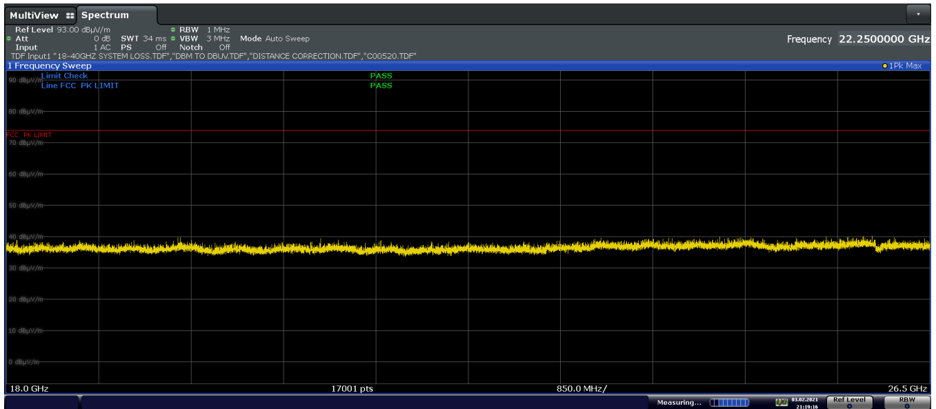
Plot 7-67. Radiated Spurious Emissions above 18GHz TxBF (GFSK ePA – Ch.0, Pol. V)
