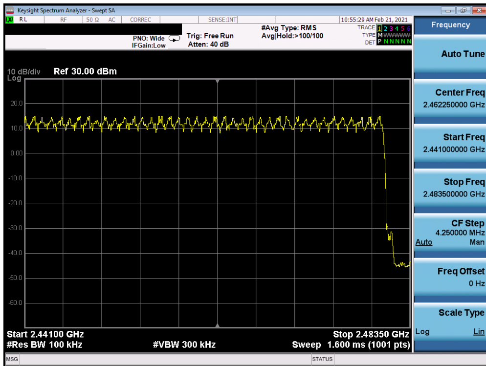
Plot 7-44. High End Spectrum Channel Hopping Plot Antenna 7 (Bluetooth, 8DPSK, ePA)
