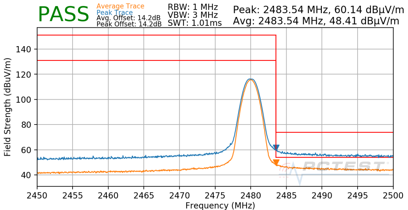
Plot 7-71. Radiated Restricted Upper Band Edge Measurement Antenna 8 (Average & Peak)
