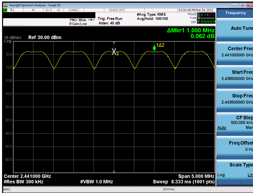
Plot 7-29. Channel Spacing Plot Antenna 8 (Bluetooth, GFSK, ePA)
