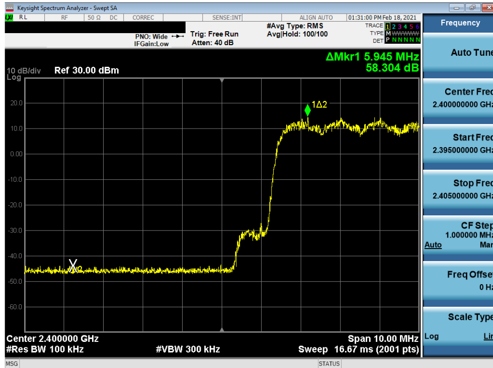
Plot 7-19. Band Edge Plot Antenna 8 (Bluetooth with Hopping Enabled, 8DPSK, ePA)
