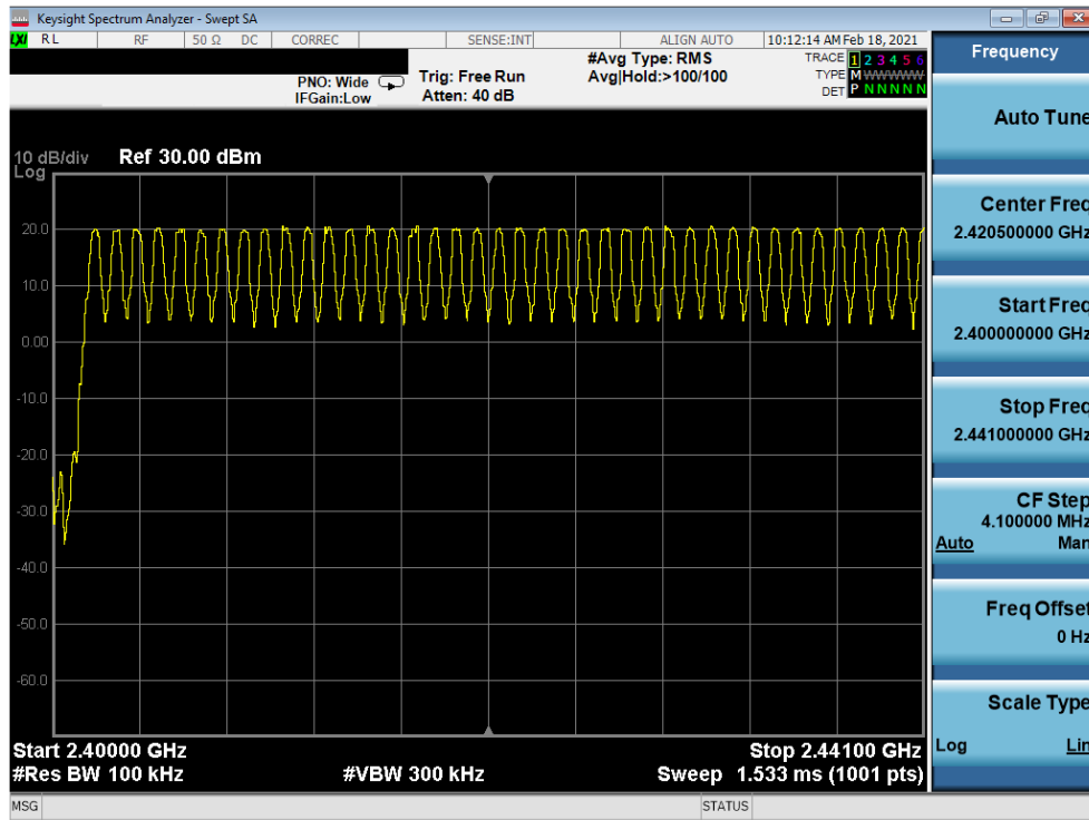
Plot 7-37. Low End Spectrum Channel Hopping Plot Antenna 8 (Bluetooth, GFSK, ePA)
