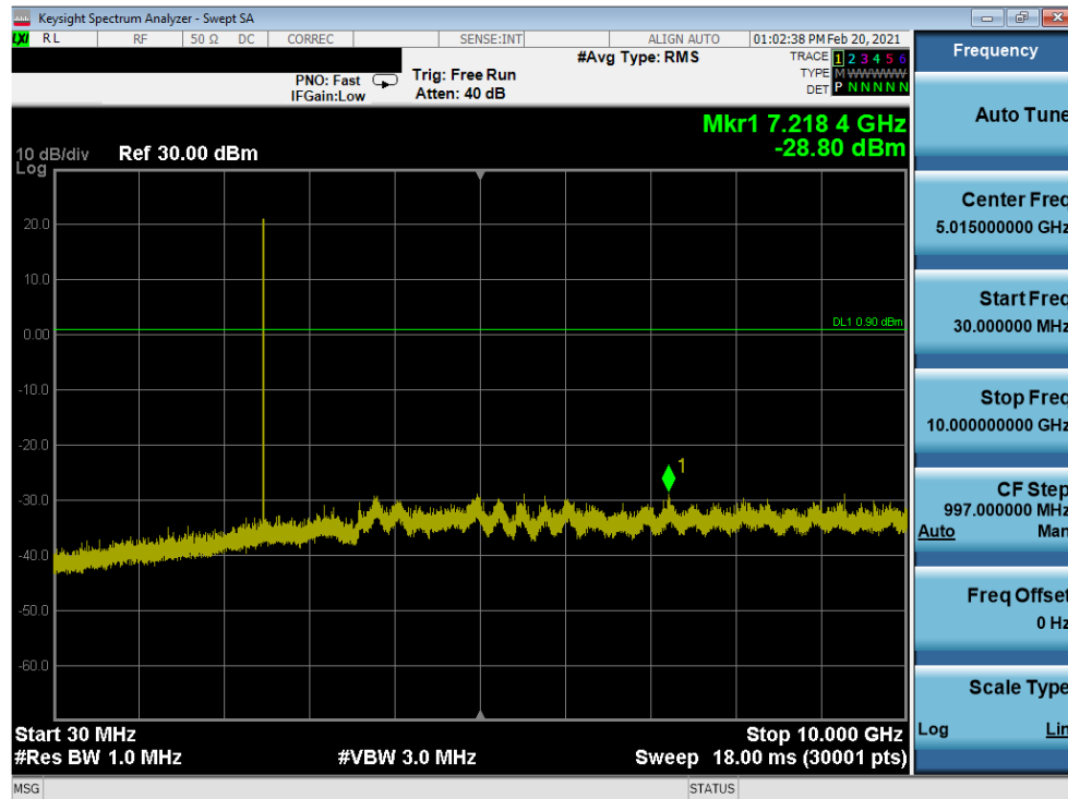
Plot 7-55. Conducted Spurious Plot Antenna 7 (Bluetooth, GFSK, ePA – Ch. 78)
