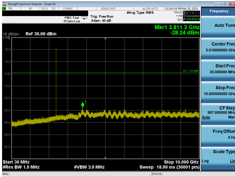
Plot 7-51. Conducted Spurious Plot Antenna 7 (Bluetooth, GFSK, ePA – Ch. 0)
