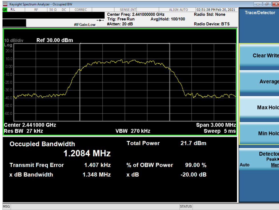
Plot 7-11. 20dB BW and 99% OBW Plot Antenna 7 (Bluetooth, 8DPSK, ePA – Ch. 39)
