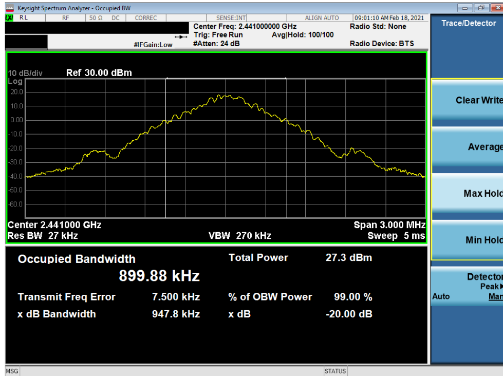
Plot 7-2. 20dB BW and 99% OBW Plot Antenna 8 (Bluetooth, GFSK, ePA – Ch. 39)
