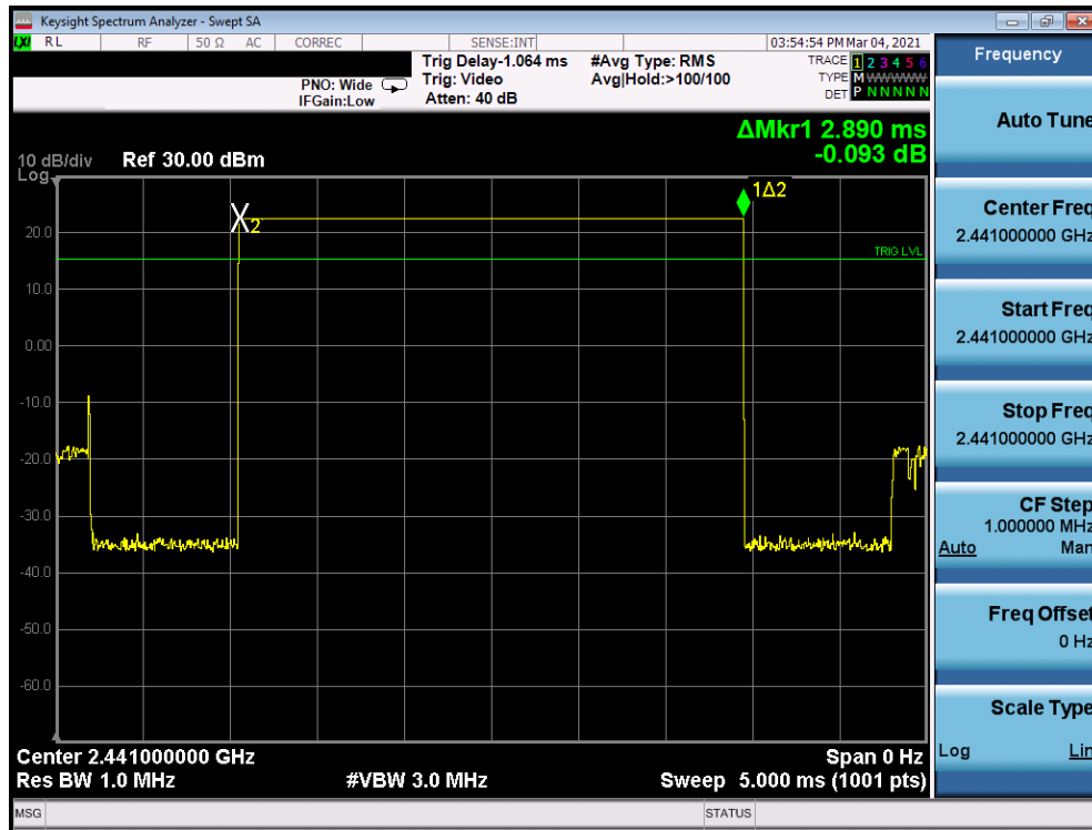
Plot 7-35. Time of Occupancy Plot Antenna 7 (Bluetooth, GFSK, ePA)
