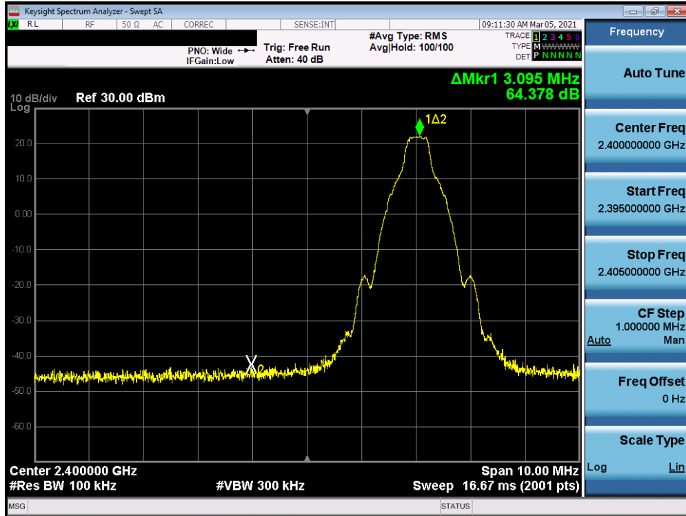
Plot 7-21. Band Edge Plot Antenna 7 (Bluetooth with Hopping Disabled, GFSK, ePA – Ch. 0)
