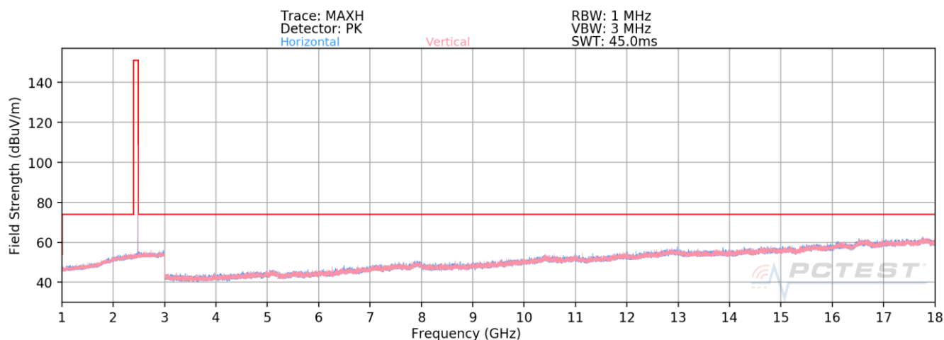
Plot 7-59. Radiated Spurious Emissions above 1GHz Antenna 8 (BT GFSK ePA – Ch. 78)
