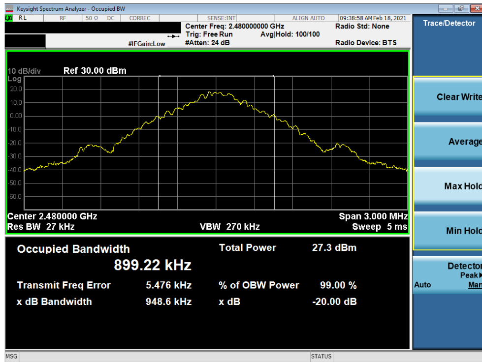
Plot 7-3. 20dB BW and 99% OBW Plot Antenna 8 (Bluetooth, GFSK, ePA – Ch. 78)
