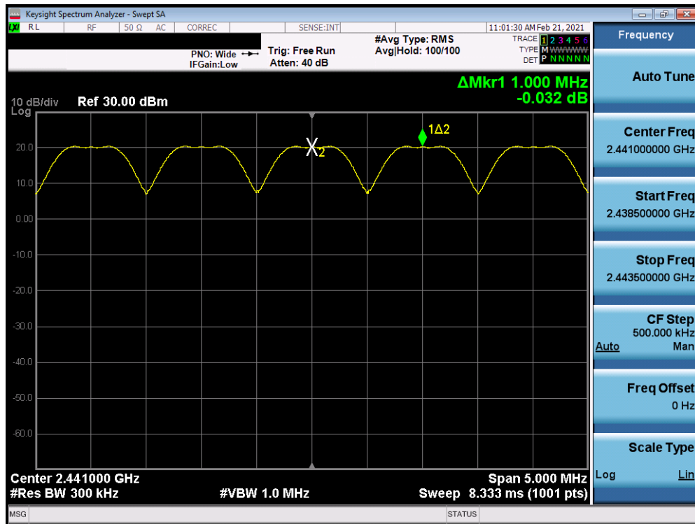
Plot 7-31. Channel Spacing Plot Antenna 7 (Bluetooth, GFSK, ePA)
