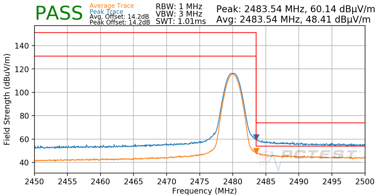
Plot 7-70. Radiated Restricted Upper Band Edge Measurement Antenna 8 (Average & Peak)
