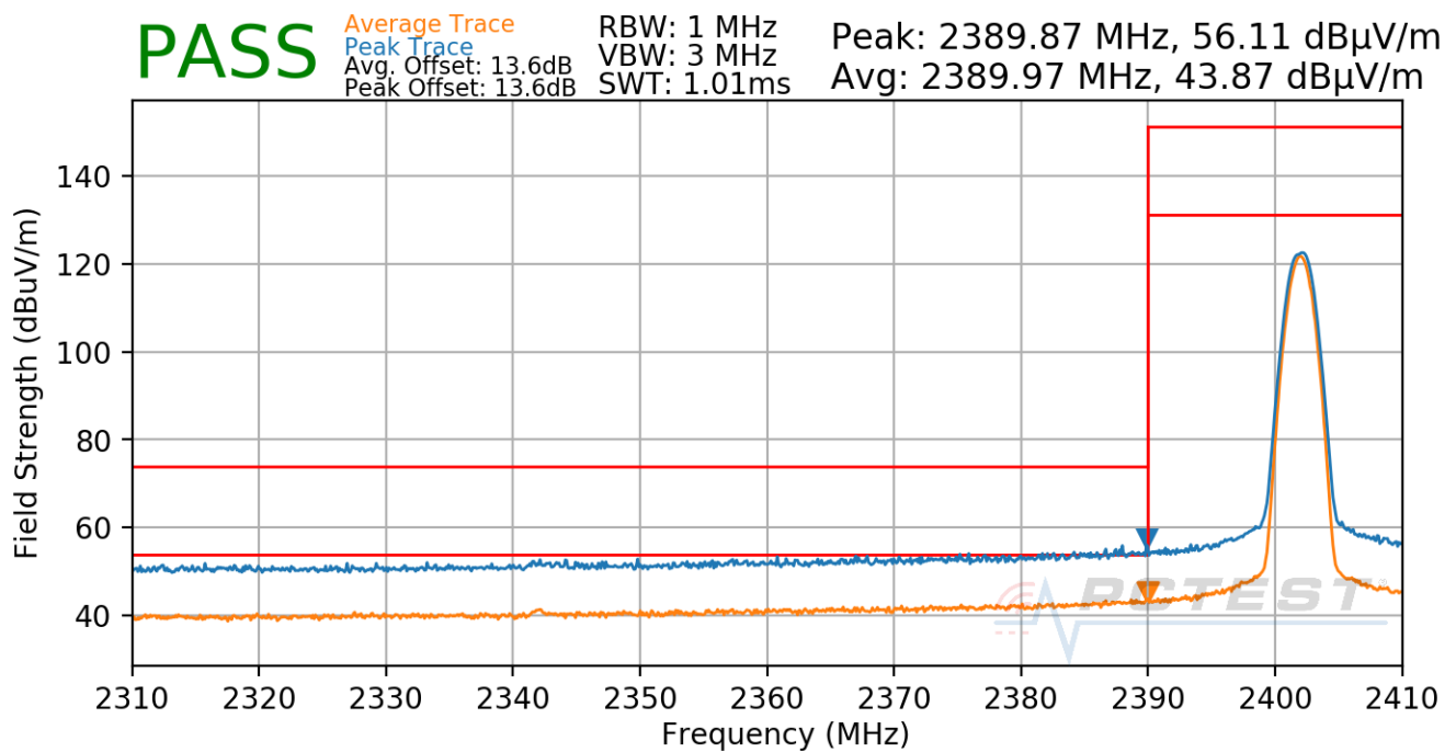
Plot 7-72. Radiated Restricted Lower Band Edge Measurement Antenna 7 (Average & Peak)
