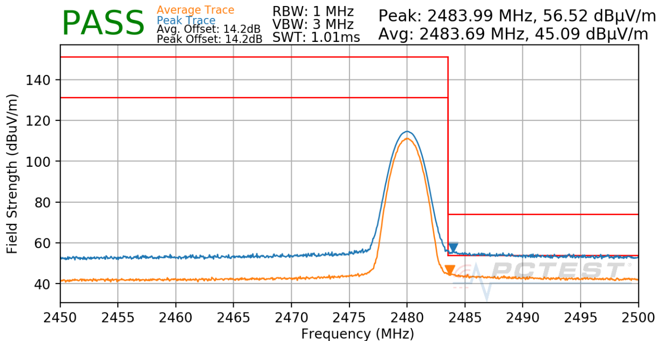
Plot 7-75. Radiated Restricted Upper Band Edge Measurement Antenna 7 (Average & Peak)
