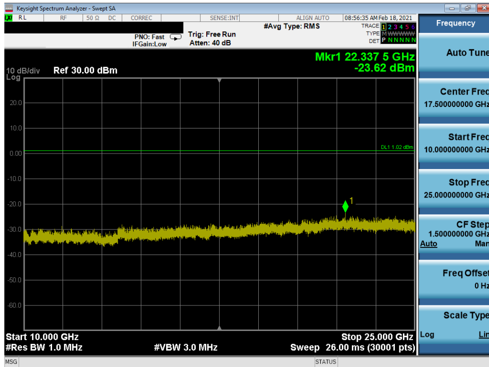
Plot 7-46. Conducted Spurious Plot Antenna 8 (Bluetooth, GFSK, ePA – Ch. 0)
