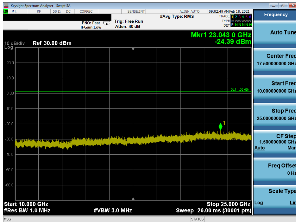
Plot 7-48. Conducted Spurious Plot Antenna 8 (Bluetooth, GFSK, ePA Ch. 39)
