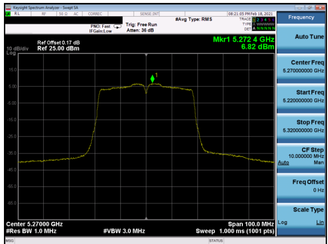
Plot 7-342. PSD SDM Antenna 5B (40MHz BW 802.11n – Ch. 54, MCS8)
