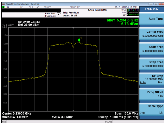
Plot 7-365. PSD SDM Antenna 5T (40MHz BW 802.11n – Ch. 46, MCS11)
