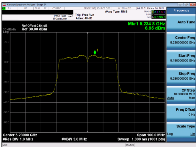
Plot 7-366. PSD SDM Antenna 5B (40MHz BW 802.11n – Ch. 46, MCS11)
