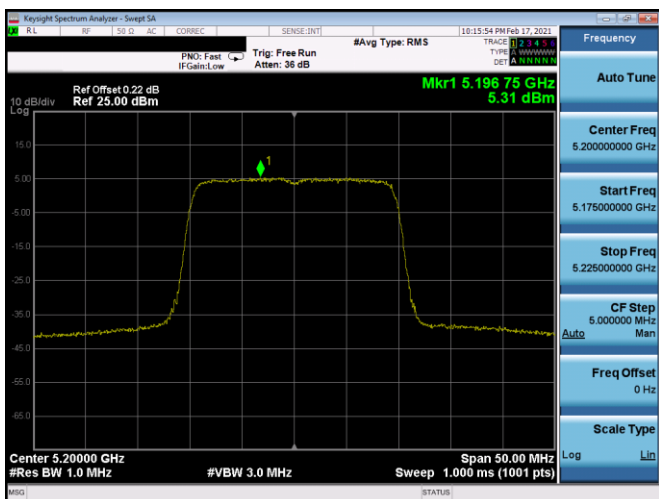
Plot 7-364. PSD SDM Antenna 5B (20MHz BW 802.11ax(SU) – Ch. 40, MCS3)
