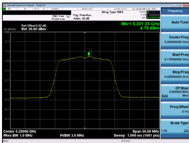
Plot 7-361. PSD SDM Antenna 5T (20MHz BW 802.11n – Ch. 40, MCS11)
