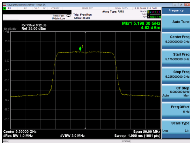
Plot 7-363. PSD SDM Antenna 5T (20MHz BW 802.11ax(SU) – Ch. 40, MCS3)
