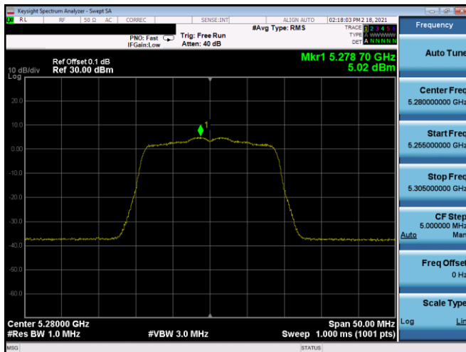
Plot 7-338. PSD SDM Antenna 5B (20MHz BW 802.11n – Ch. 56, MCS8)
