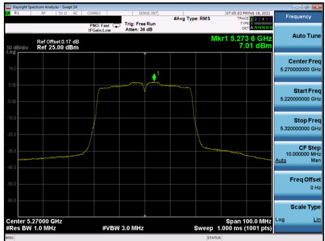
Plot 7-341. PSD SDM Antenna 5T (40MHz BW 802.11n – Ch. 54, MCS8)
