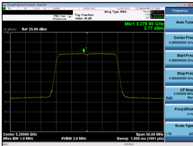
Plot 7-339. PSD SDM Antenna 5T (20MHz BW 802.11ax(SU) – Ch. 56, MCS0)
