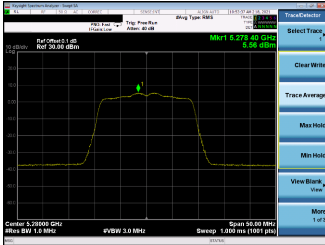
Plot 7-337. PSD SDM Antenna 5T (20MHz BW 802.11n – Ch. 56, MCS8)
