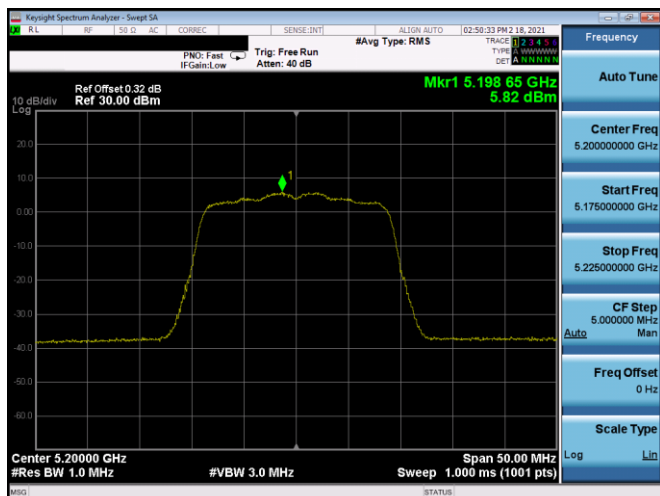
Plot 7-362. PSD SDM Antenna 5B (20MHz BW 802.11n – Ch. 40, MCS11)
