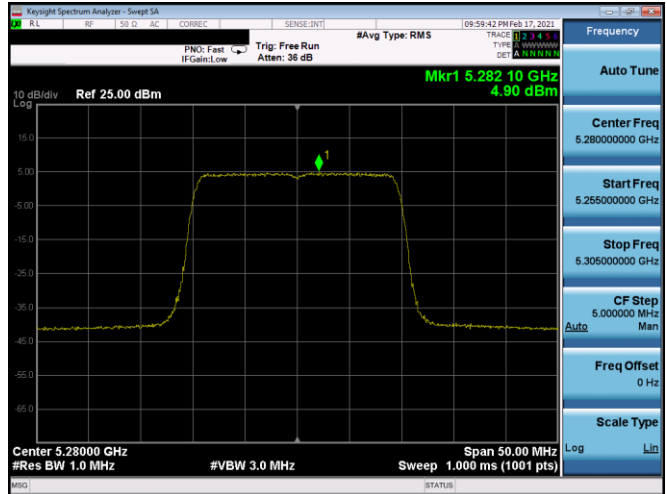
Plot 7-340. PSD SDM Antenna 5B (20MHz BW 802.11ax(SU) – Ch. 56, MCS0)
