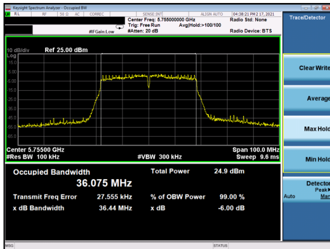
Plot 7-135. 6dB BW & 99% OBW Antenna 5B (40MHz BW 802.11n – Ch. 151, MCS3)
