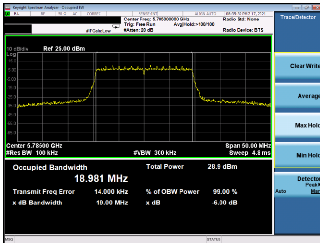
Plot 7-110. 6dB BW & 99% OBW Antenna 5T (20MHz BW 802.11ax(SU) - Ch. 157, MCS0)
