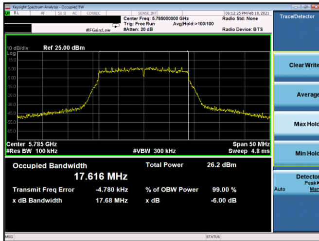
Plot 7-133. 6dB BW & 99% OBW Antenna 5B (20MHz BW 802.11n – Ch. 157, MCS3)
