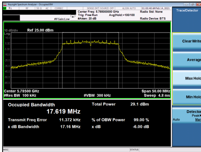
Plot 7-109. 6dB BW & 99% OBW Antenna 5T (20MHz BW 802.11n - Ch. 157, MCS0)
