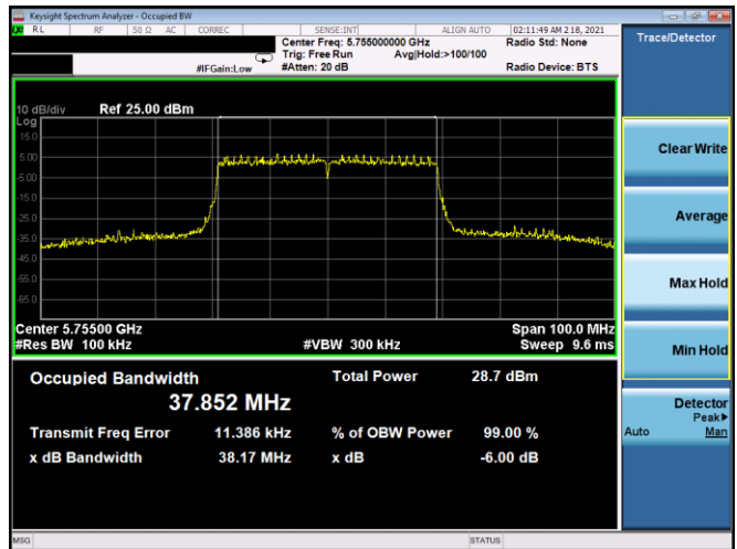
Plot 7-112. 6dB BW & 99% OBW Antenna 5T (40MHz BW 802.11ax(SU) - Ch. 151, MCS0)
