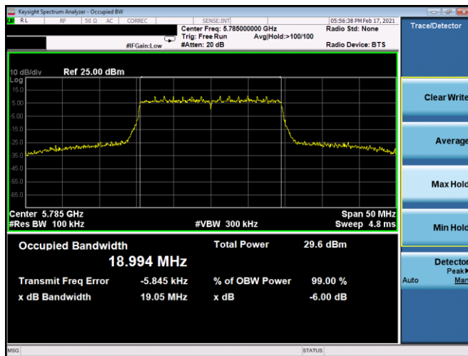
Plot 7-128. 6dB BW & 99% OBW Antenna 5B (20MHz BW 802.11ax(SU) – Ch. 157, MCS0)
