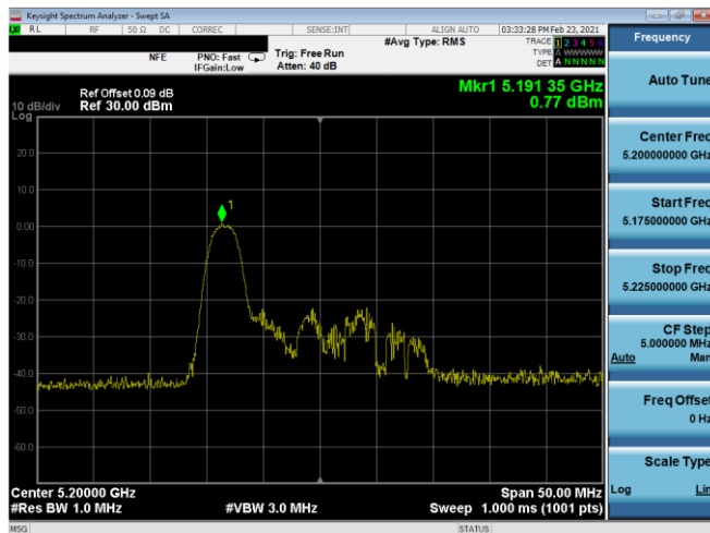
Plot 7-314. ISD PSD SDM Antenna 5B (20MHz BW 11ax Index 0 – RU26 – Ch.40)
