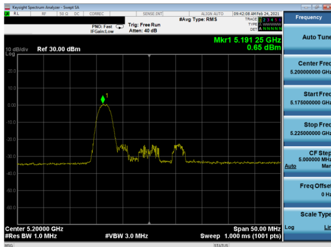
Plot 7-313. ISD PSD SDM Antenna 5T (20MHz BW 11ax Index 0 – RU26 – Ch.40)
