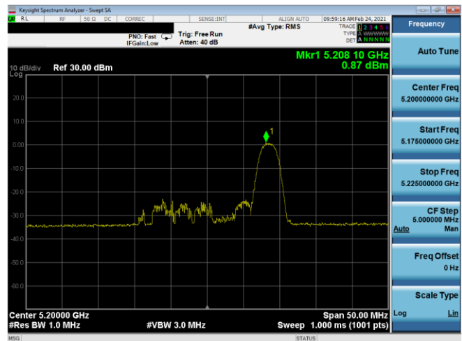
Plot 7-317. ISD PSD SDM Antenna 5T (20MHz BW 11ax Index 8 – RU26 – Ch.40)
