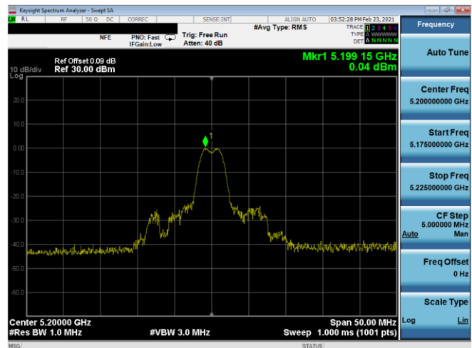
Plot 7-316. ISD PSD SDM Antenna 5B (20MHz BW 11ax Index 4 – RU26 – Ch.40)
