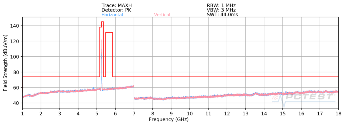
Plot 7-340. RSE above 1GHz Antenna 5T (11ax – Ch.52 – RU26)
