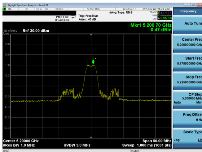
Plot 7-315. ISD PSD SDM Antenna 5T (20MHz BW 11ax Index 4 – RU26 – Ch.40)
