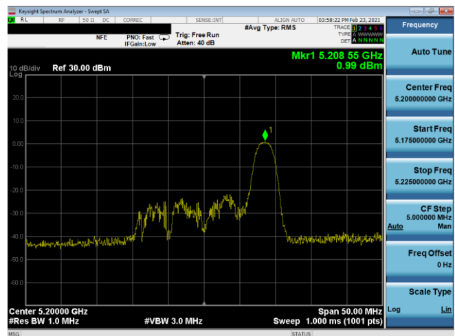
Plot 7-318. ISD PSD SDM Antenna 5B (20MHz BW 11ax Index 8 – RU26 – Ch.40)
