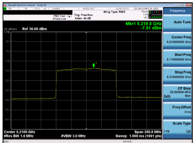
Plot 7-240. PSD CDD Antenna 5B (80MHz BW 11ax - RU996 - Ch.42)
