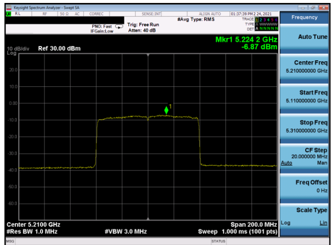
Plot 7-239. PSD CDD Antenna 5T (80MHz BW 11ax - RU996 - Ch.42)
