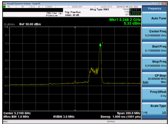
Plot 7-238. PSD SDM Antenna 5B (80MHz BW 11ax Index 36 - RU26 - Ch.42)
