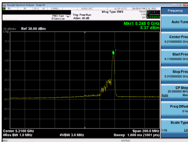
Plot 7-237. PSD SDM Antenna 5T (80MHz BW 11ax Index 36 - RU26 - Ch.42)
