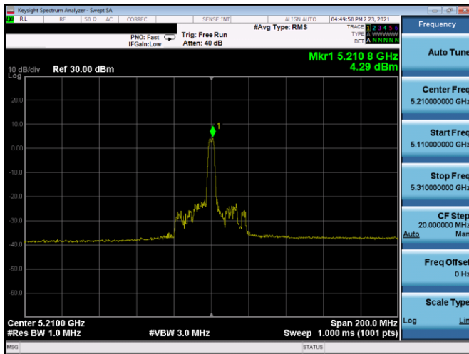
Plot 7-235. PSD SDM Antenna 5T (80MHz BW 11ax Index 18 - RU26 - Ch.42)
