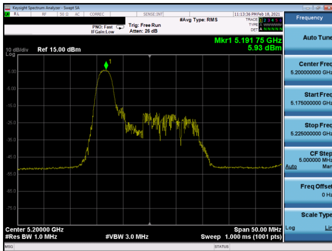
Plot 7-218. SDM CDD Antenna 5B (20MHz BW 11ax Index 0 – RU26 – Ch.40)
