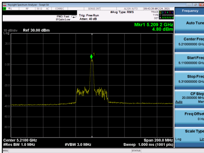
Plot 7-236. PSD SDM Antenna 5B (80MHz BW 11ax Index 18 - RU26 - Ch.42)
