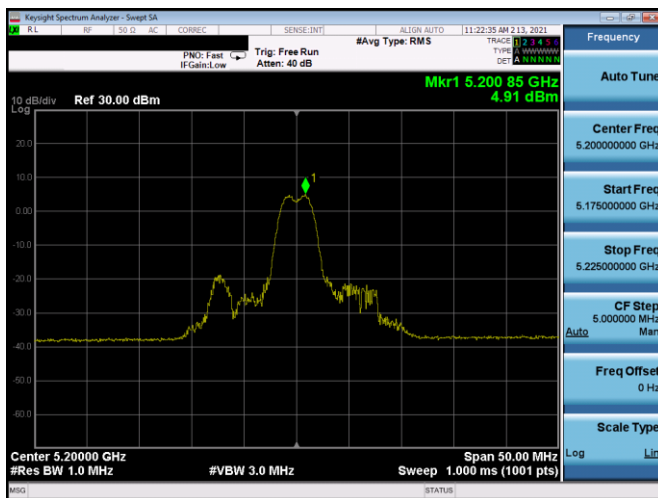
Plot 7-219. PSD SDM Antenna 5T (20MHz BW 11ax Index 4 – RU26 – Ch.40)
