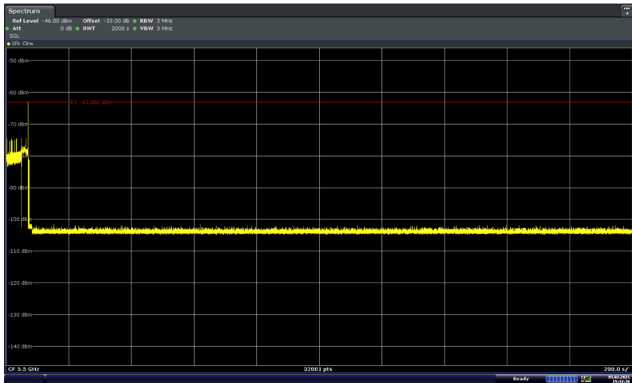
Figure 9-37. 5500MHz - Non-Occupancy Period (30 Minutes) - Mode 1 (20MHz)
