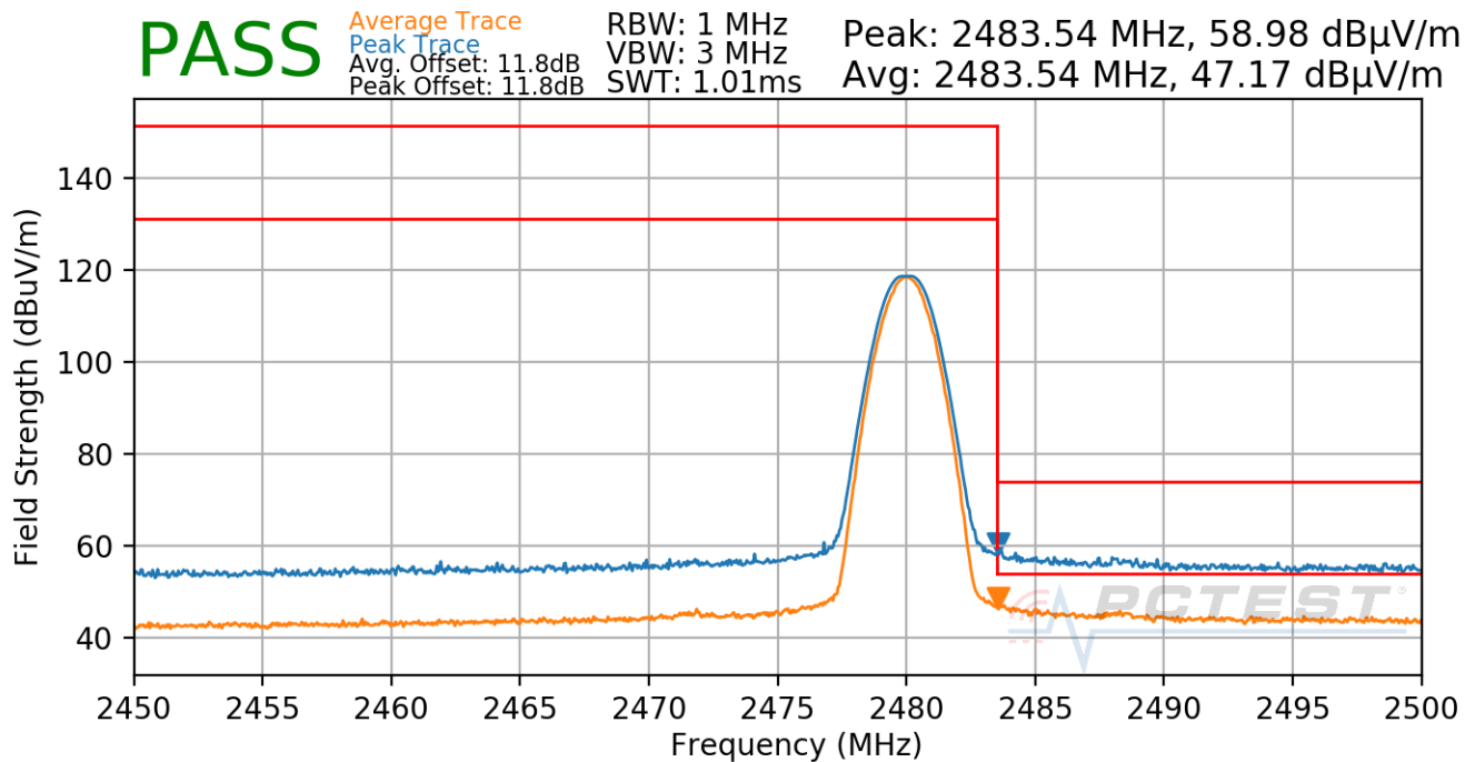
Plot 7-74. Radiated Restricted Upper Band Edge Measurement Antenna WF7 (Average & Peak)
