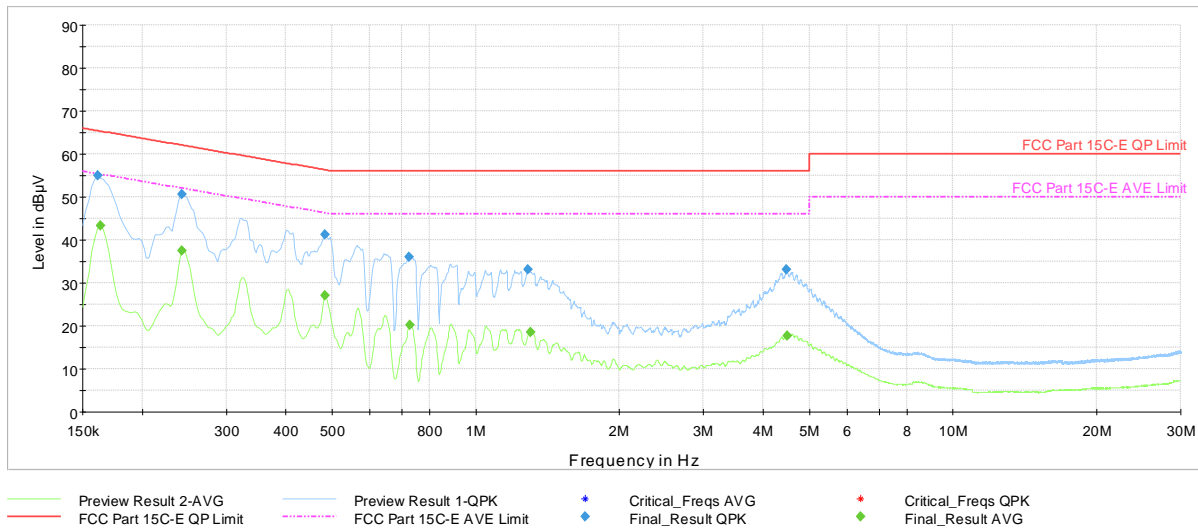
Plot 7-81. AC Line-Conducted Test Plot TxBF (L1, GFSK ePA – Ch.39, with AC/DC Adapter)
