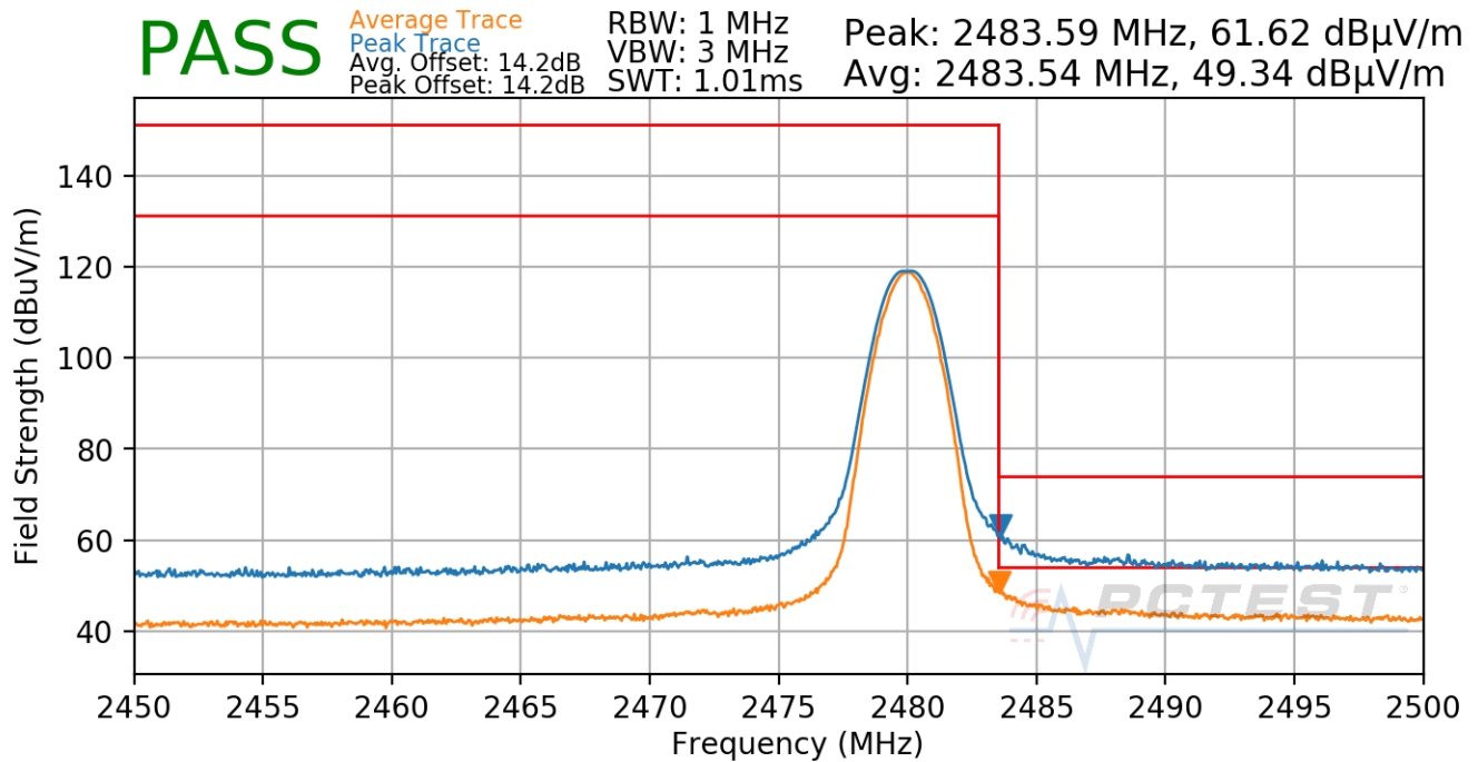
Plot 7-70. Radiated Restricted Upper Band Edge Measurement Antenna WF8 (Average & Peak)
