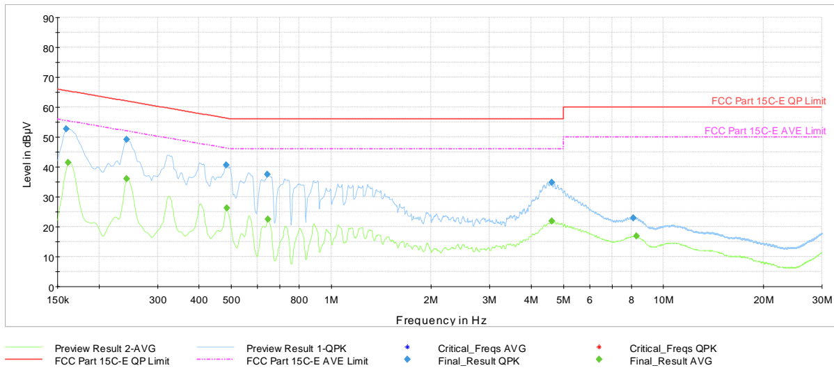
Plot 7-82. AC Line-Conducted Test Plot TxBF (N, GFSK ePA – Ch.39, with AC/DC Adapter)
