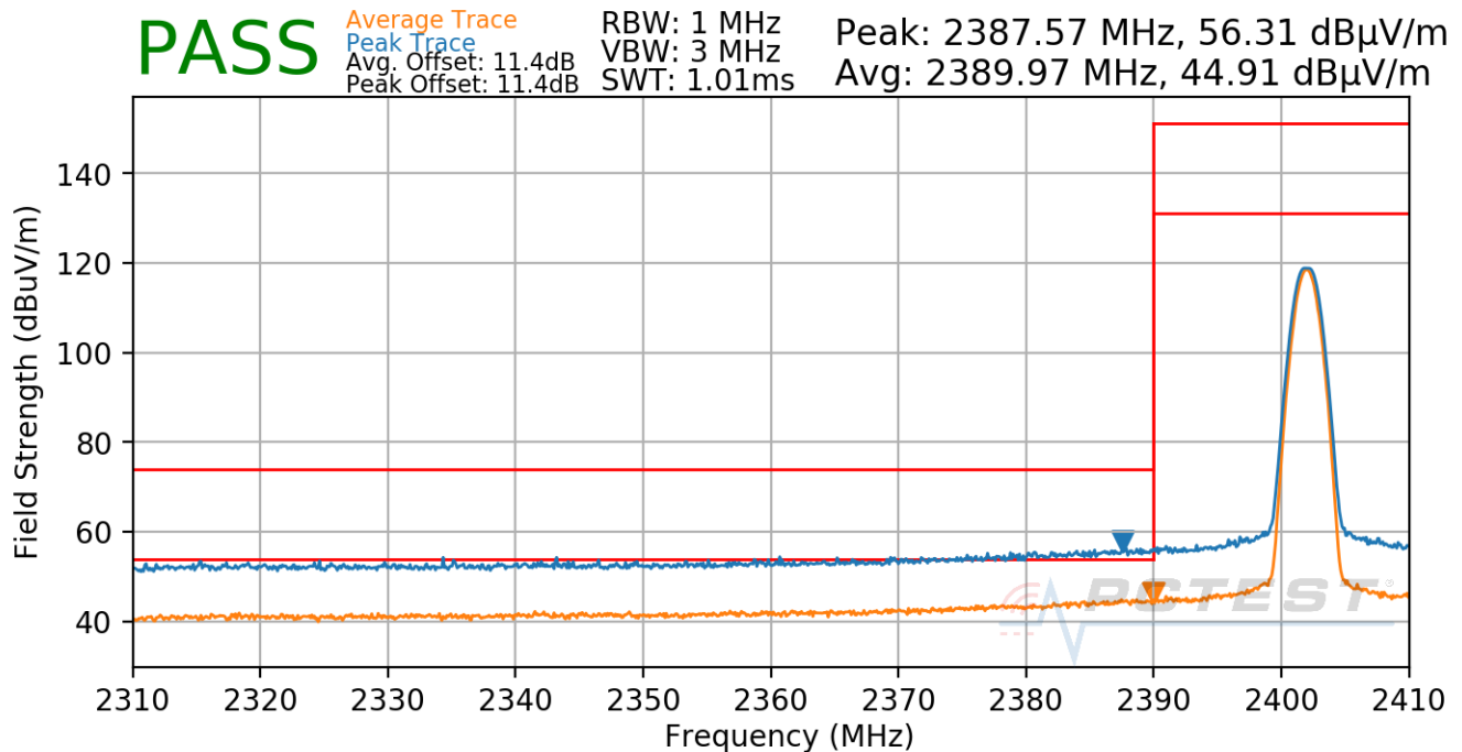
Plot 7-72. Radiated Restricted Lower Band Edge Measurement Antenna WF7 (Average & Peak)
