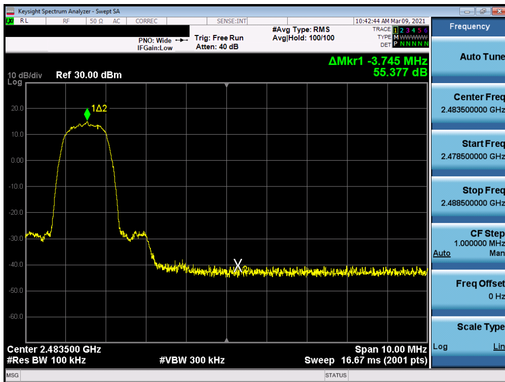
Plot 7-26. Band Edge Plot Antenna WF7 (Bluetooth with Hopping Disabled, 8DPSK, ePA – Ch. 78)
