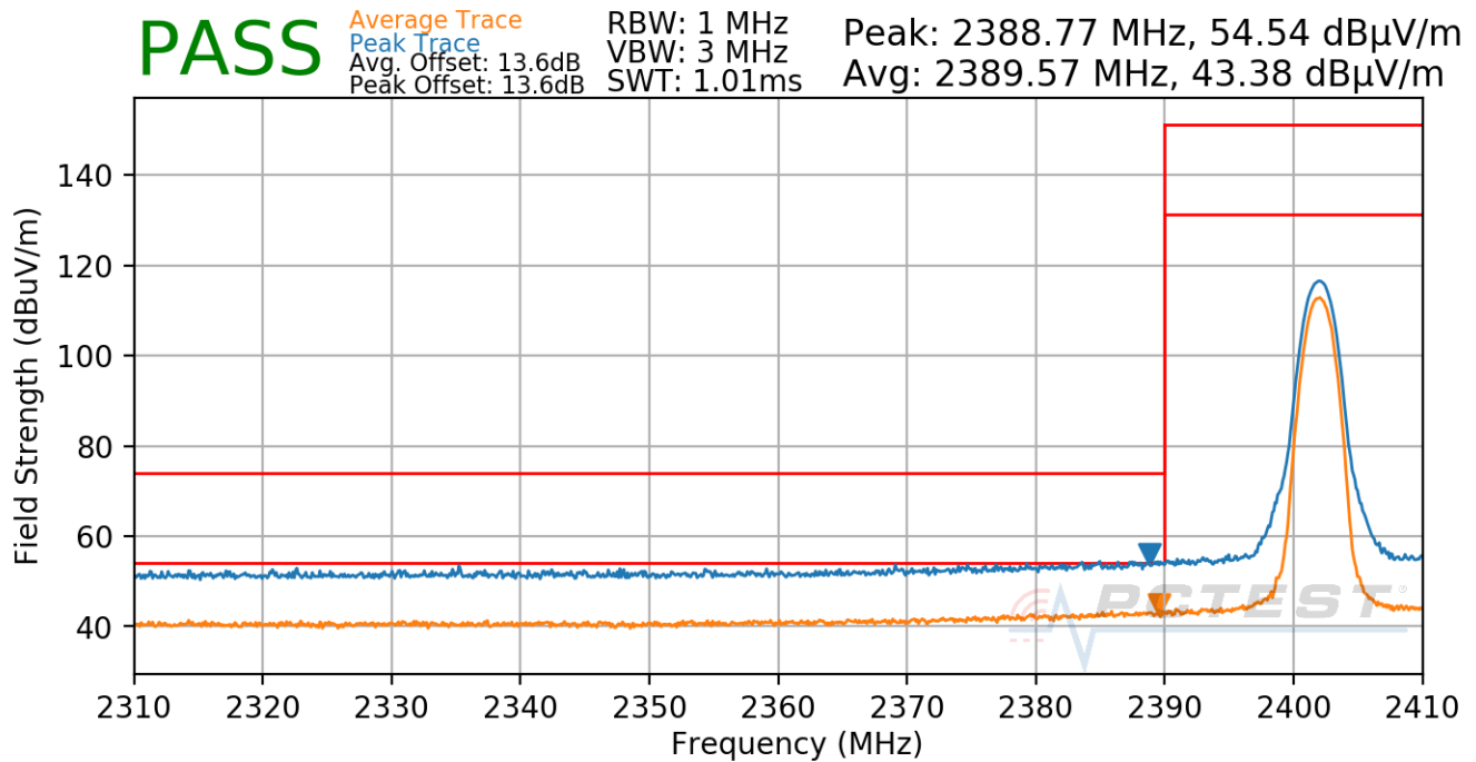
Plot 7-69. Radiated Restricted Lower Band Edge Measurement Antenna WF8 (Average & Peak)
