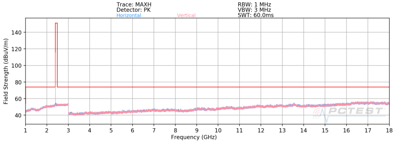
Plot 7-60. Radiated Spurious Emissions Above 1GHz Antenna WF7 (BT GFSK ePA – Ch. 0)
