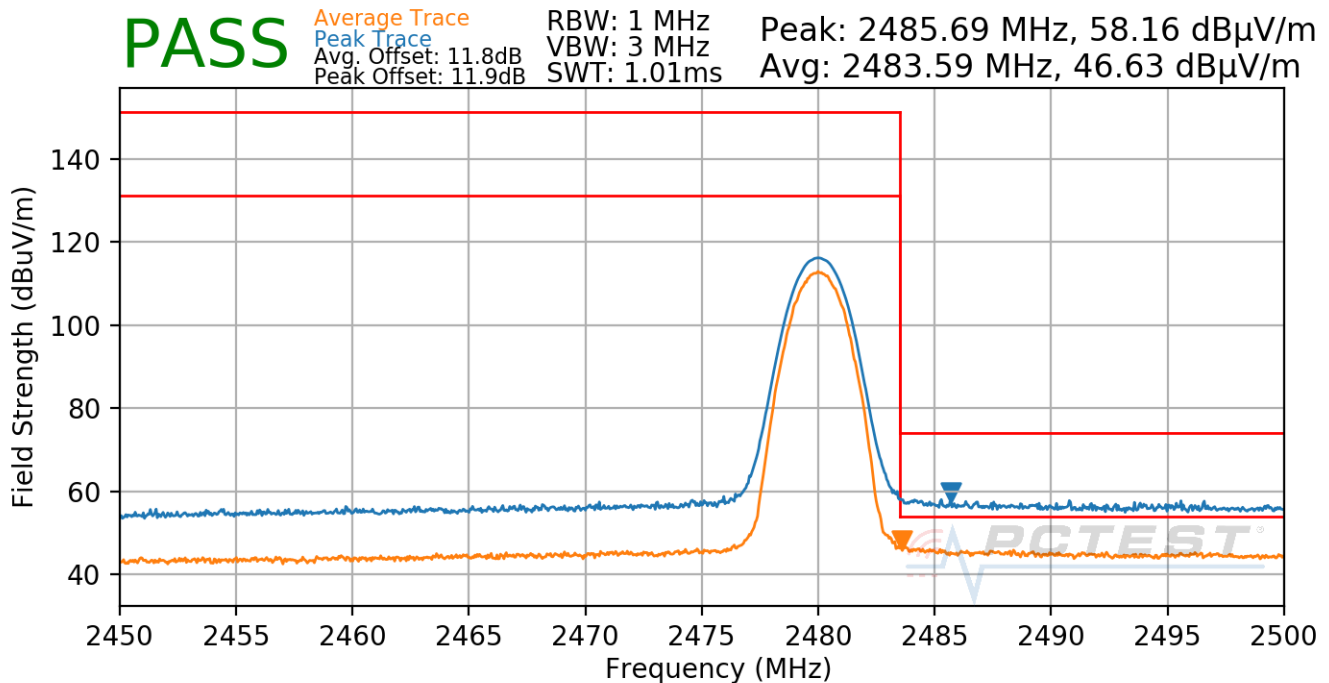
Plot 7-75. Radiated Restricted Upper Band Edge Measurement Antenna WF7 (Average & Peak)
