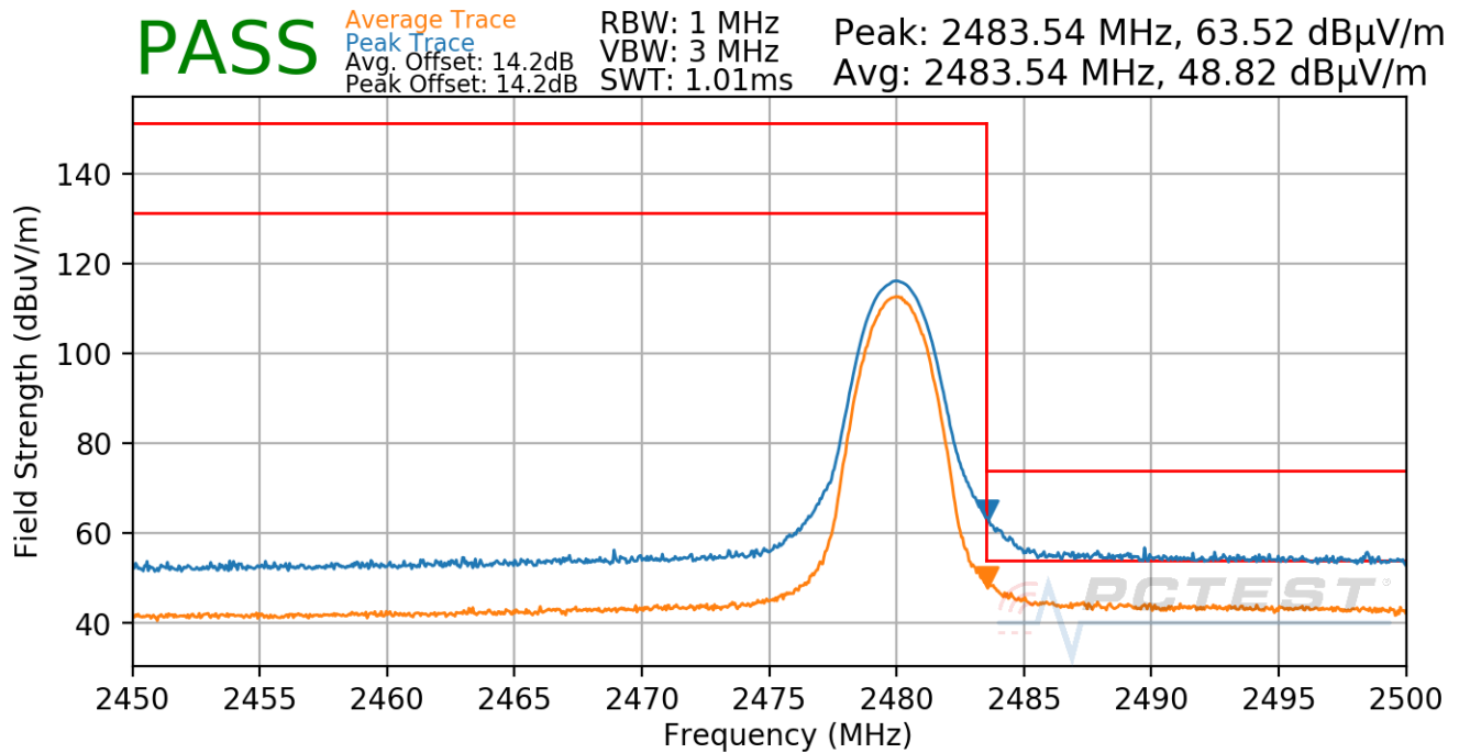
Plot 7-71. Radiated Restricted Upper Band Edge Measurement Antenna WF8 (Average & Peak)
