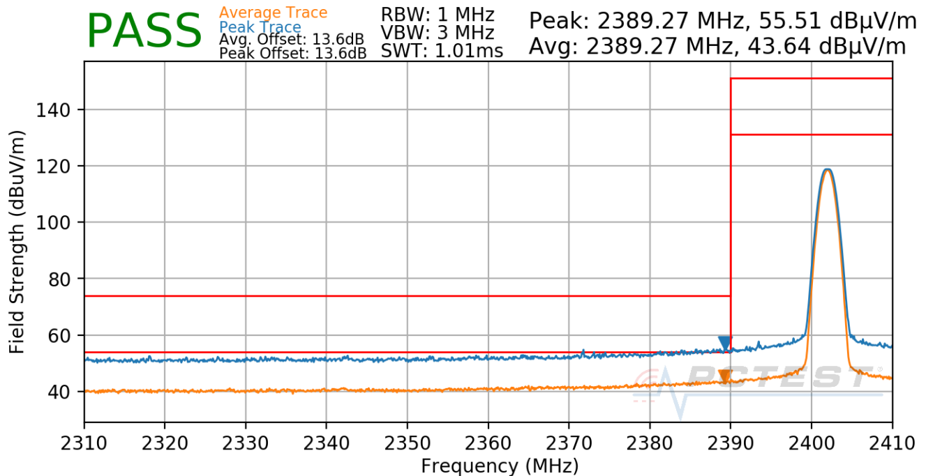
Plot 7-68. Radiated Restricted Lower Band Edge Measurement Antenna WF8 (Average & Peak)
