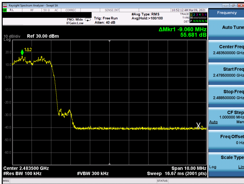
Plot 7-28. Band Edge Plot Antenna WF7 (Bluetooth with Hopping Enabled, 8DPSK, ePA)
