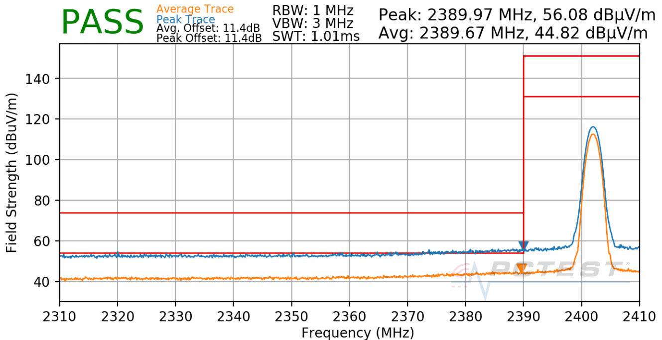
Plot 7-73. Radiated Restricted Lower Band Edge Measurement Antenna WF7 (Average & Peak)
