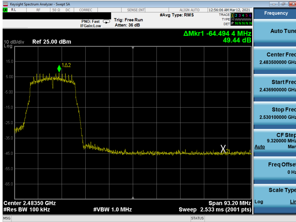
Plot 7-231. Band Edge Plot Antenna WF8 (802.11n (2.4GHz) - Ch. 9) - MCS0
