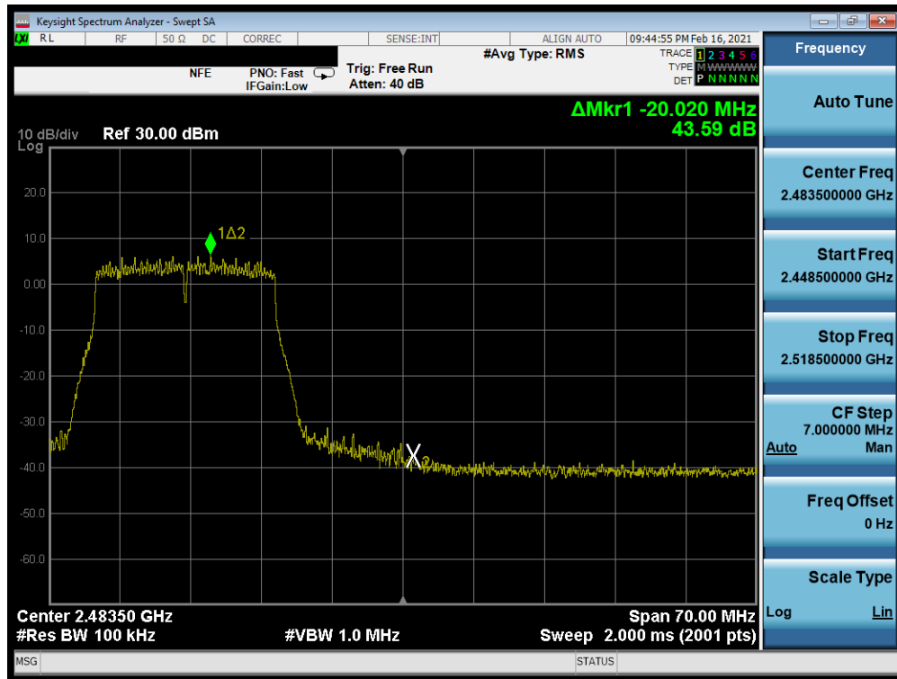
Plot 7-239. Band Edge Plot Antenna WF8 (802.11n (2.4GHz) - Ch. 11) - MCS7
