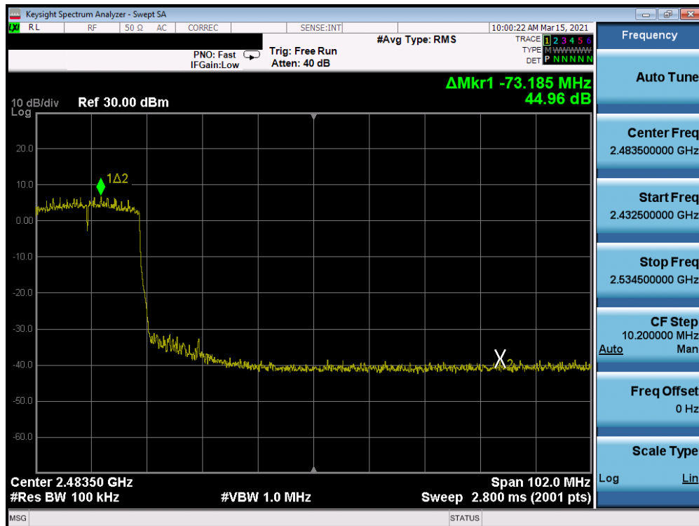
Plot 7-266: Band Edge Plot Antenna WF8 (802.11ax (SU – 2.4GHz) – Ch. 7) – MCS5
