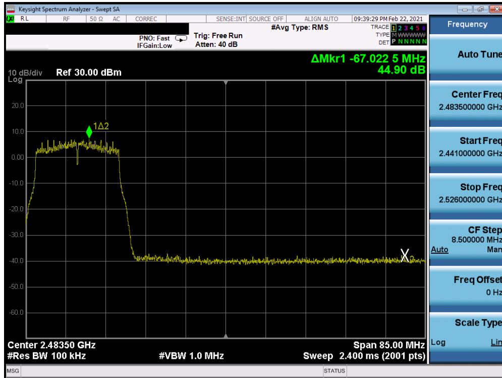
Plot 7-232. Band Edge Plot Antenna WF8 (802.11n (2.4GHz) - Ch. 9) - MCS3
