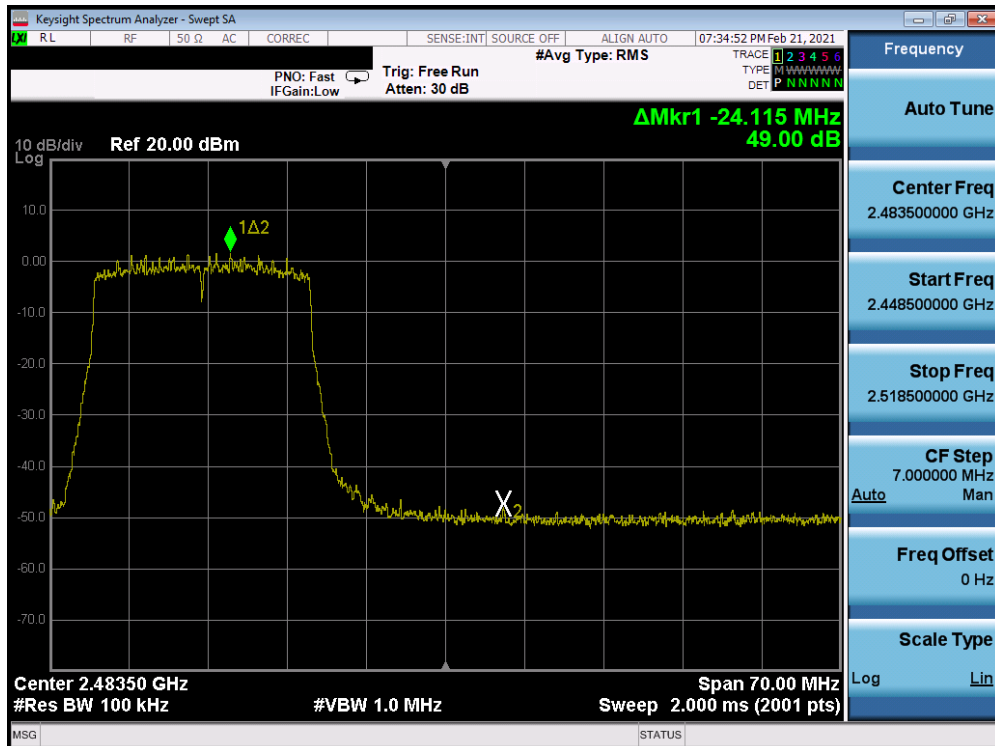
Plot 7-278. Band Edge Plot Antenna WF8 (802.11ax (SU - 2.4GHz) - Ch. 11) - MCS5
