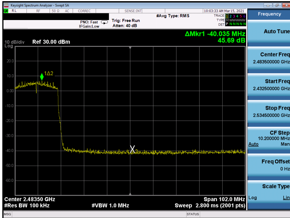
Plot 7-265: Band Edge Plot Antenna WF8 (802.11ax (SU – 2.4GHz) – Ch. 7) – MCS3
