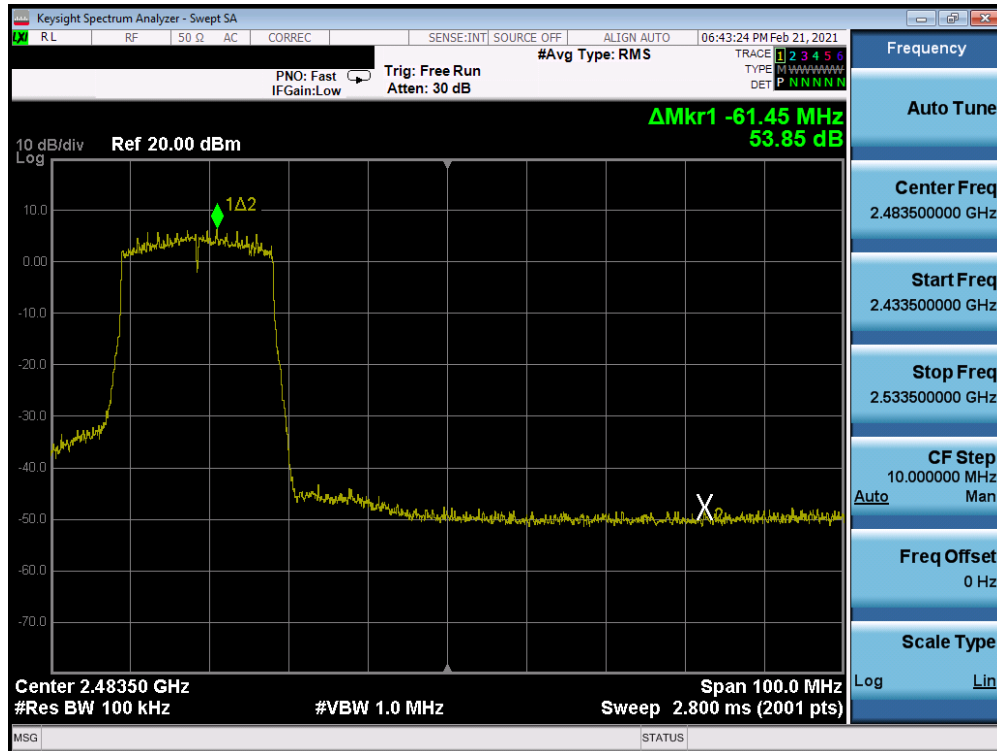
Plot 7-271. Band Edge Plot Antenna WF8 (802.11ax (SU – 2.4GHz) – Ch. 9) – MCS3
