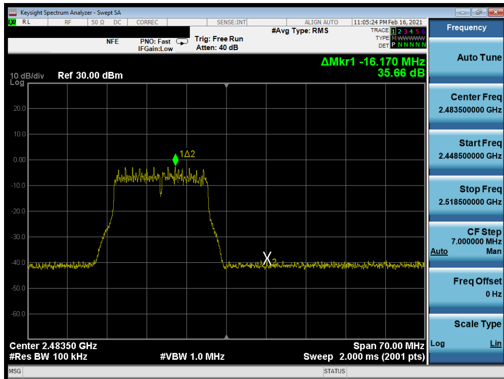
Plot 7-321. Band Edge Plot Antenna WF7 (802.11g - Ch. 13) – 54Mbps
