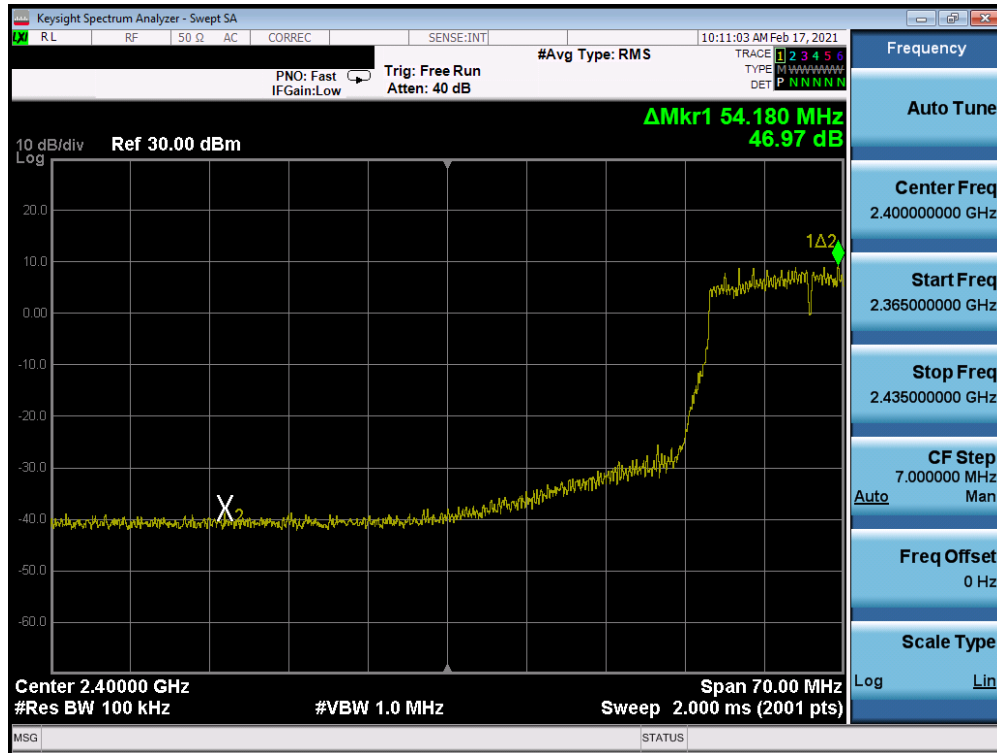
Plot 7-223. Band Edge Plot Antenna WF8 (802.11n (2.4GHz) - Ch. 5) - MCS3
