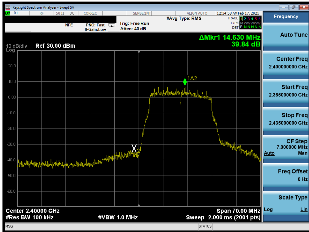
Plot 7-322. Band Edge Plot Antenna WF7 (802.11n (2.4GHz) – Ch. 1) – MCS0
