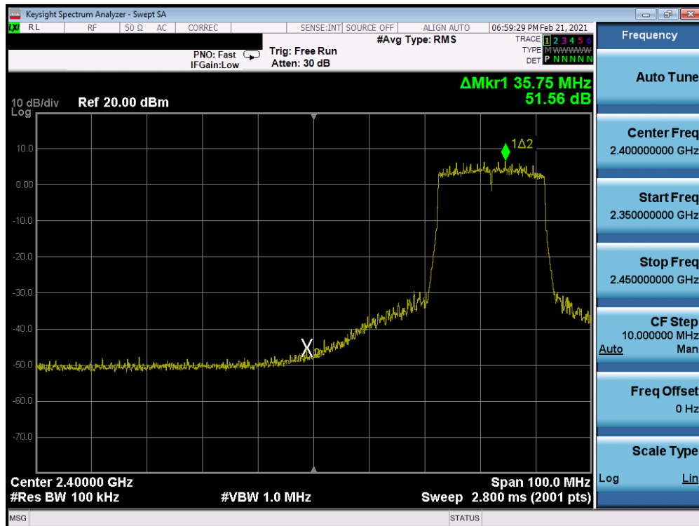
Plot 7-260. Band Edge Plot Antenna WF8 (802.11ax (SU – 2.4GHz) – Ch. 5) – MCS5
