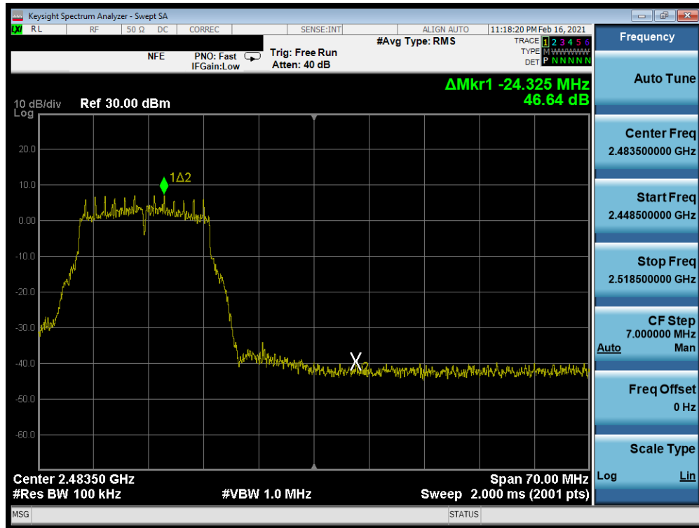
Plot 7-314. Band Edge Plot Antenna WF7 (802.11g - Ch. 11) – 18Mbps
