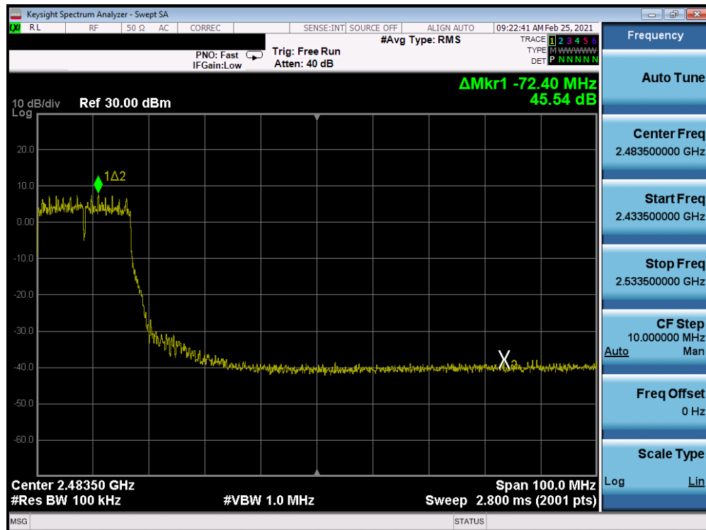
Plot 7-303: Band Edge Plot Antenna WF7 (802.11g - Ch. 7) - 54Mbps
