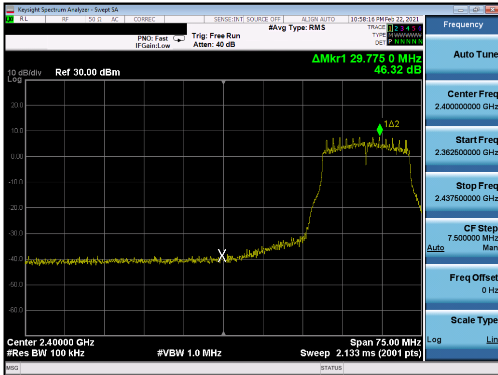
Plot 7-296. Band Edge Plot Antenna WF7 (802.11g- Ch. 4) – 18Mbps
