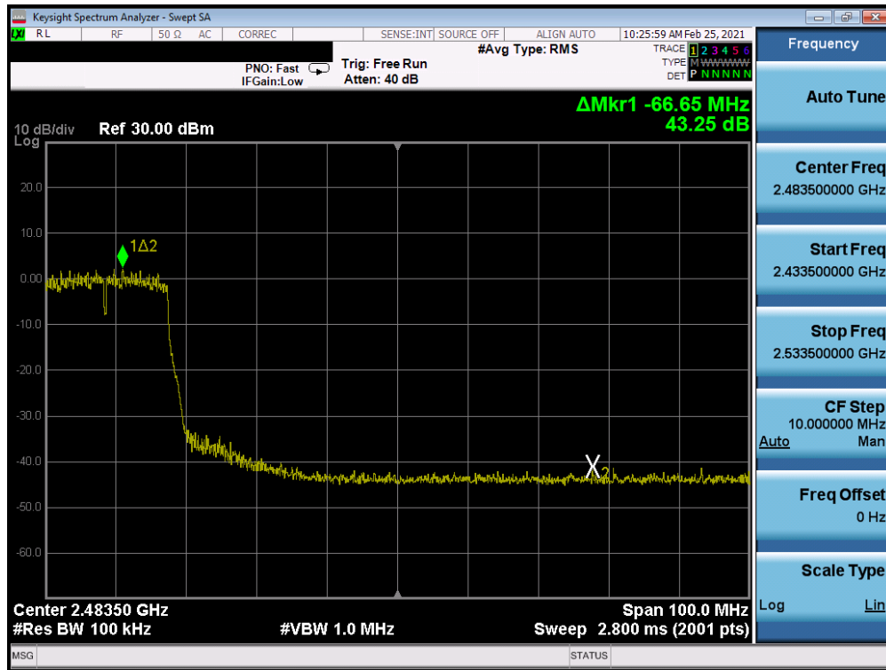
Plot 7-227. Band Edge Plot Antenna WF8 (802.11n (2.4GHz) – Ch. 7) – MCS7
