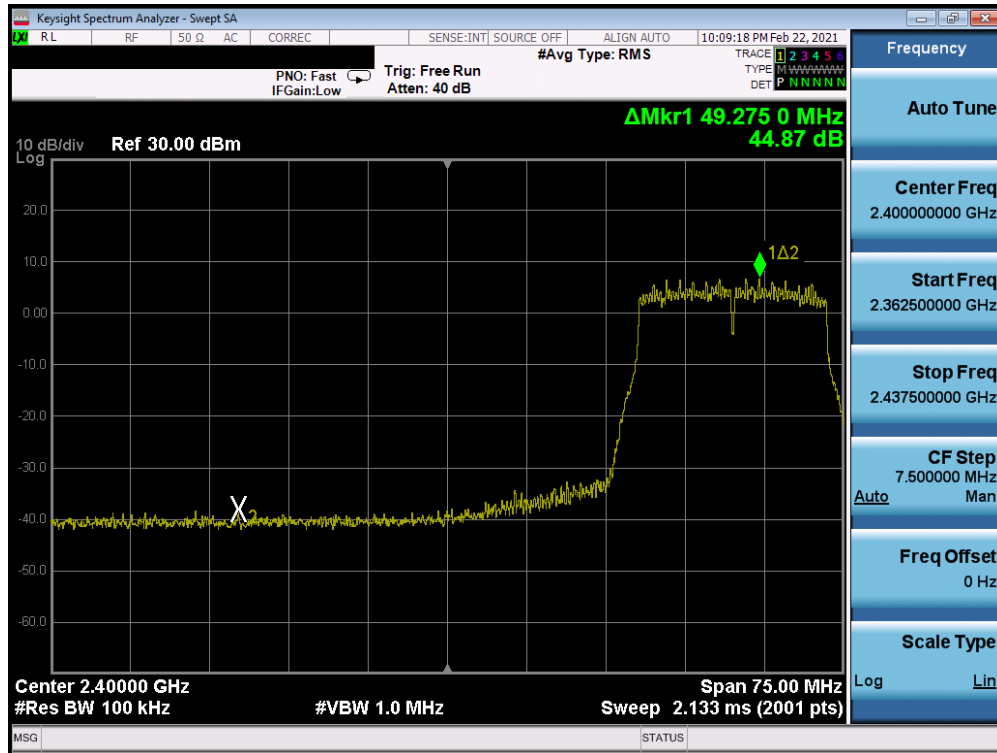
Plot 7-221. Band Edge Plot Antenna WF8 (802.11n (2.4GHz) – Ch. 4) – MCS7
