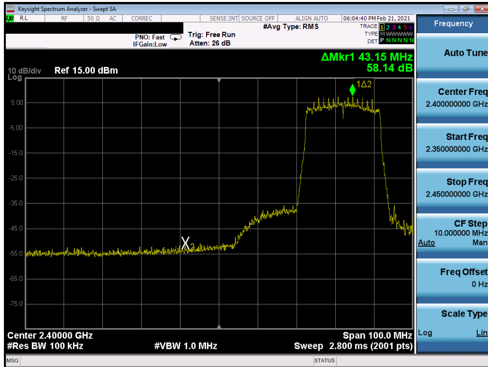
Plot 7-258. Band Edge Plot Antenna WF8 (802.11ax (SU – 2.4GHz) – Ch. 5) – MCS0
