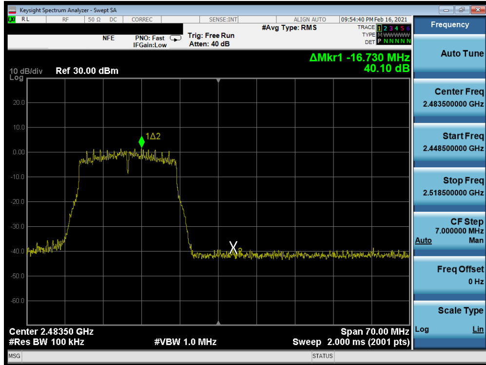
Plot 7-241. Band Edge Plot Antenna WF8 (802.11n (2.4GHz) – Ch. 12) – MCS3
