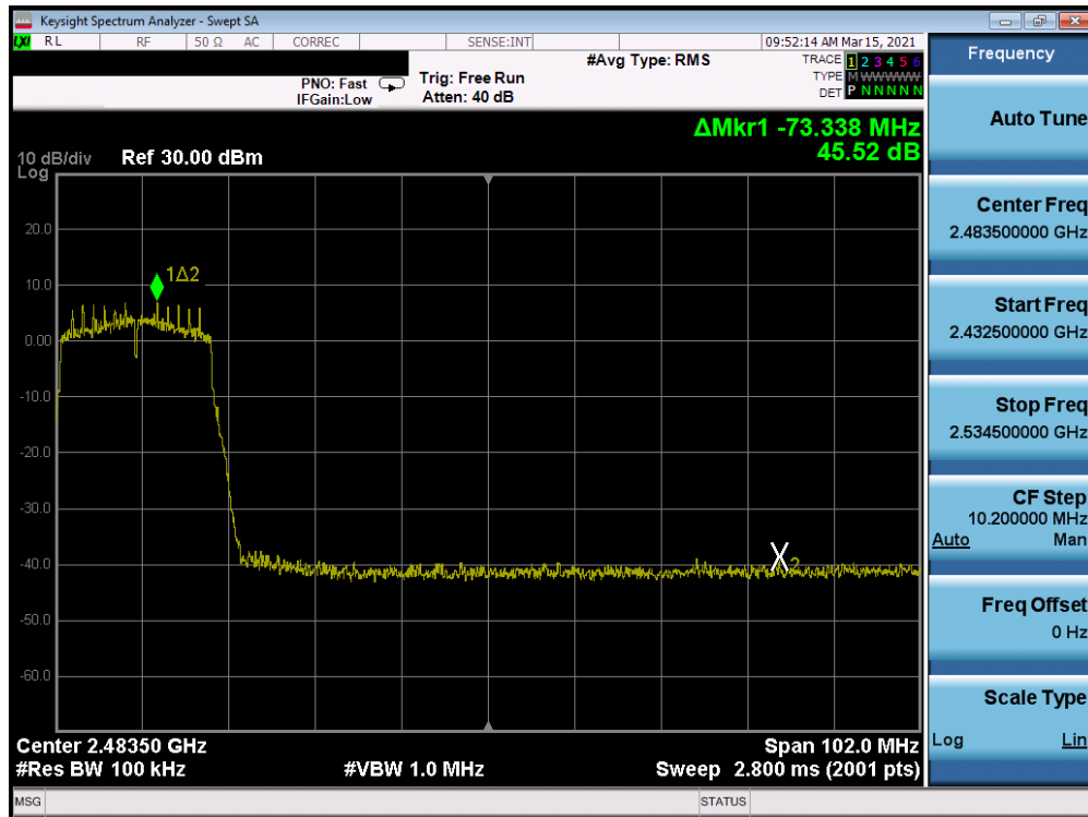
Plot 7-225. Band Edge Plot Antenna WF8 (802.11n (2.4GHz) – Ch. 7) – MCS0
