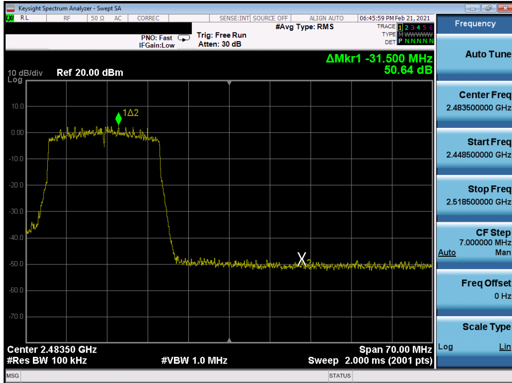
Plot 7-277. Band Edge Plot Antenna WF8 (802.11ax (SU - 2.4GHz) - Ch. 11) - MCS3
