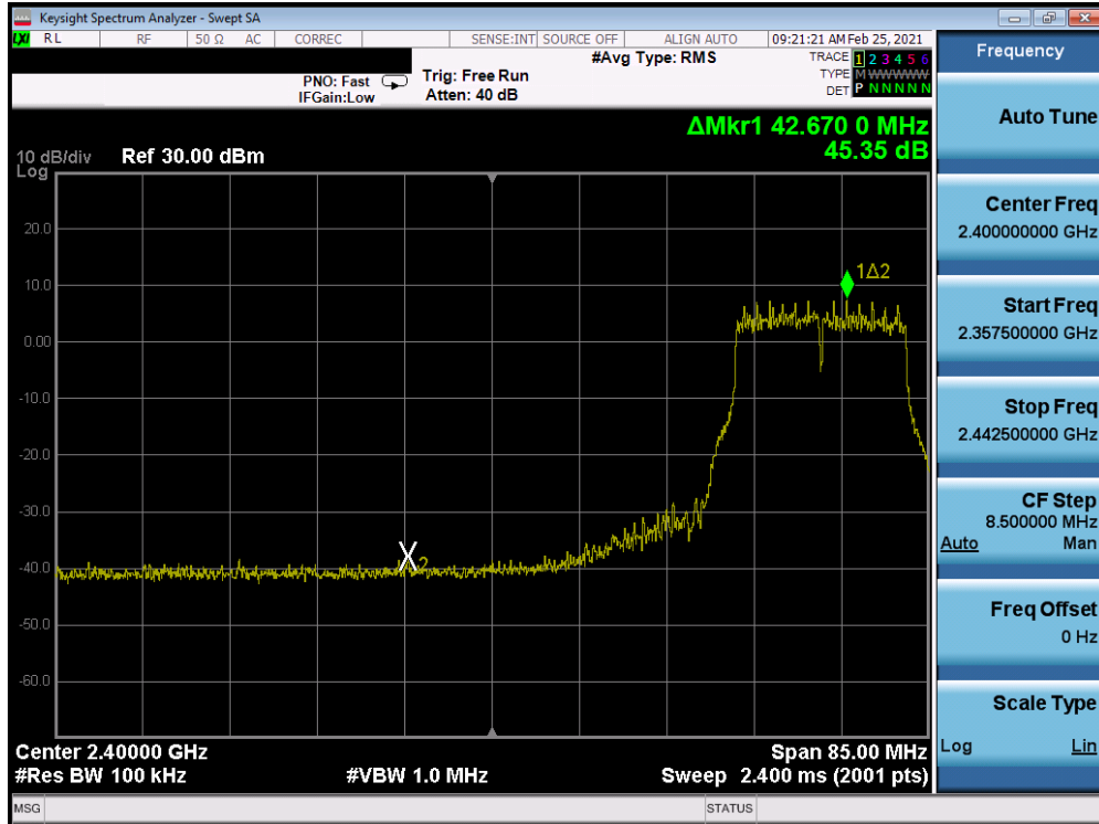
Plot 7-300. Band Edge Plot Antenna WF7 (802.11g- Ch. 5) – 54Mbps
