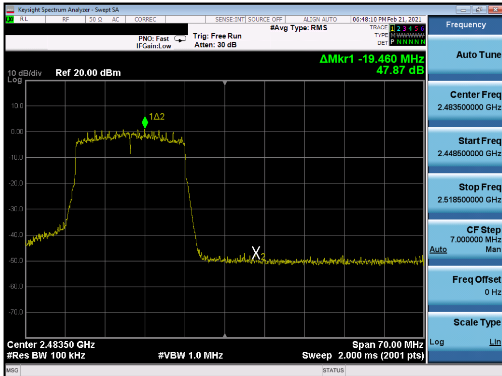
Plot 7-280. Band Edge Plot Antenna WF8 (802.11ax (SU - 2.4GHz) - Ch. 12) - MCS3
