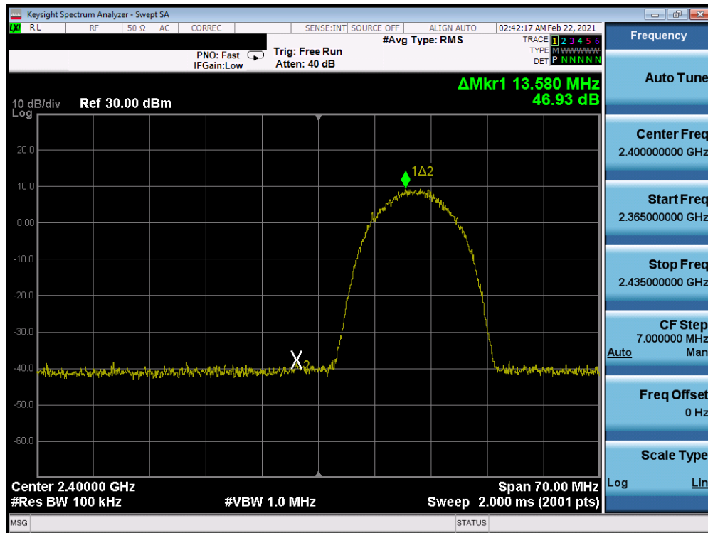
Plot 7-282. Band Edge Plot Antenna WF7 (802.11b – Ch. 1) – 11Mbps
