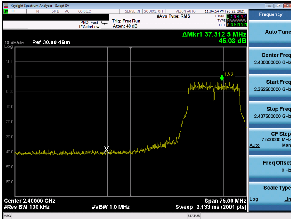
Plot 7-297. Band Edge Plot Antenna WF7 (802.11g- Ch. 4) – 54Mbps
