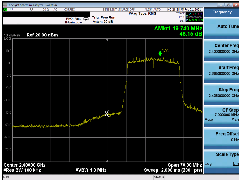
Plot 7-250. Band Edge Plot Antenna WF8 (802.11ax (SU – 2.4GHz) – Ch. 2) – MCS3
