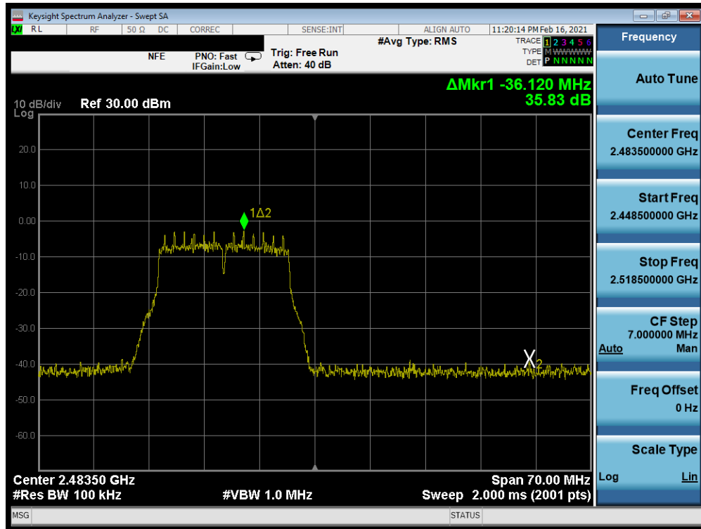
Plot 7-320. Band Edge Plot Antenna WF7 (802.11g - Ch. 13) – 18Mbps
