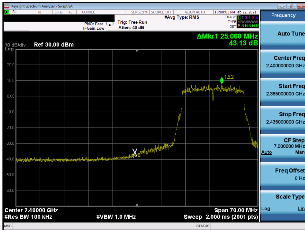
Plot 7-218. Band Edge Plot Antenna WF8 (802.11n (2.4GHz) – Ch. 3) – MCS7
