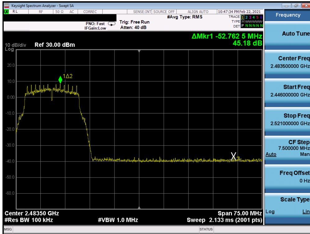
Plot 7-310. Band Edge Plot Antenna WF7 (802.11g - Ch. 10) - 6Mbps
