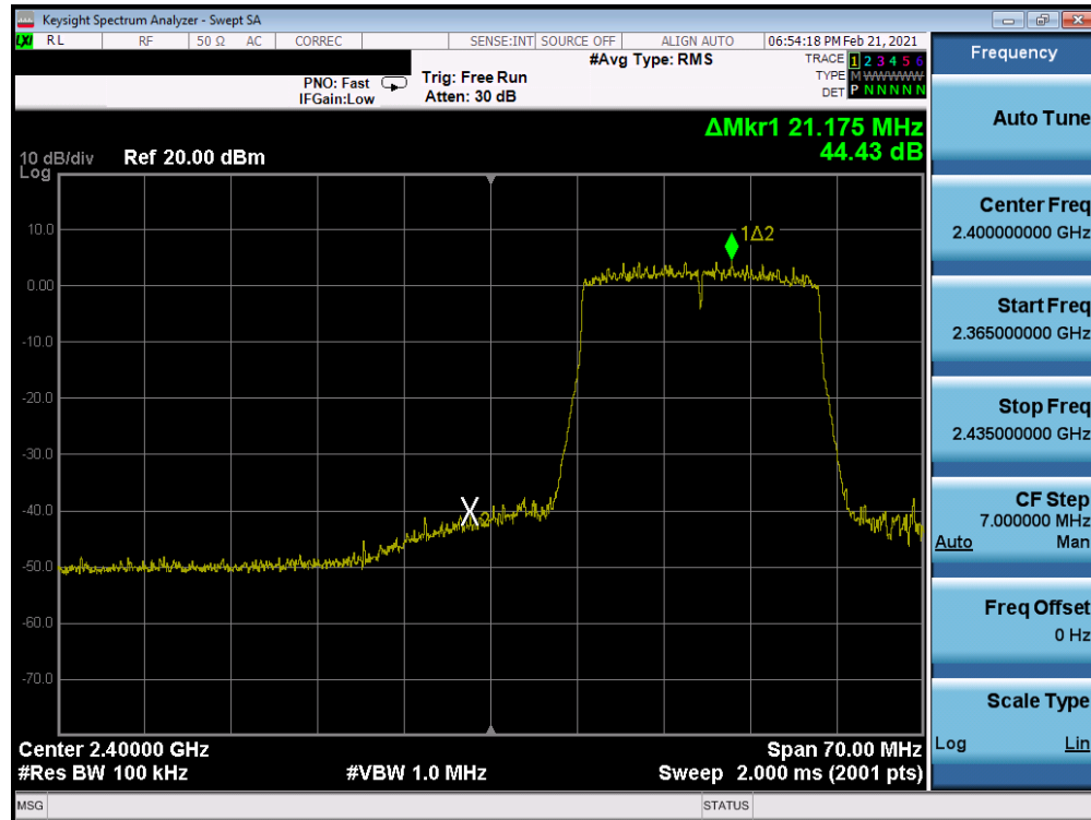
Plot 7-251. Band Edge Plot Antenna WF8 (802.11ax (SU – 2.4GHz) – Ch. 2) – MCS5
