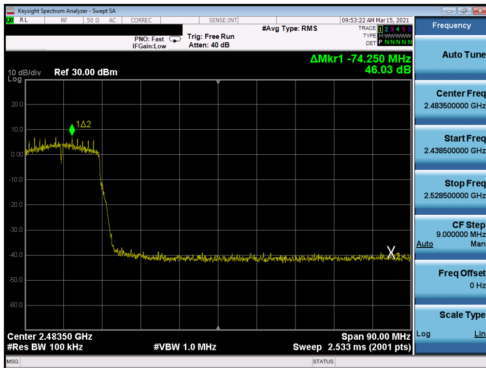
Plot 7-228: Band Edge Plot Antenna WF8 (802.11n (2.4GHz) – Ch. 8) – MCS0
