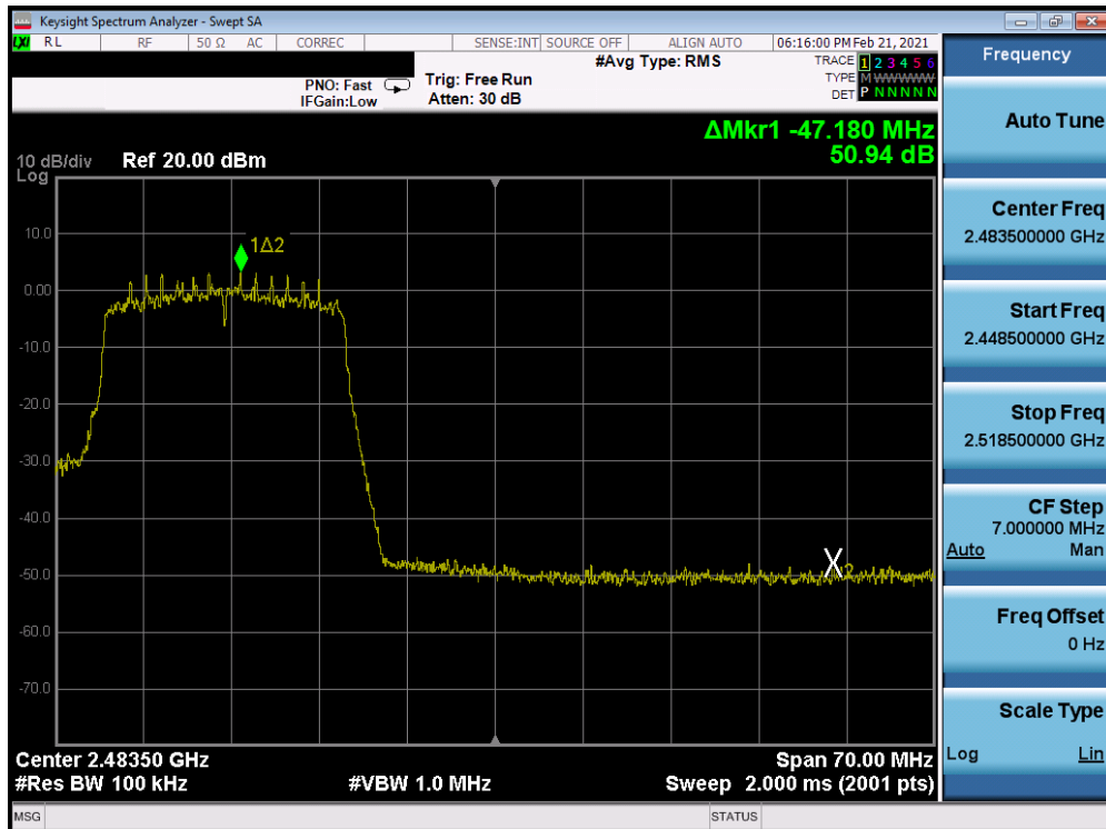
Plot 7-276. Band Edge Plot Antenna WF8 (802.11ax (SU – 2.4GHz) – Ch. 11) – MCS5
