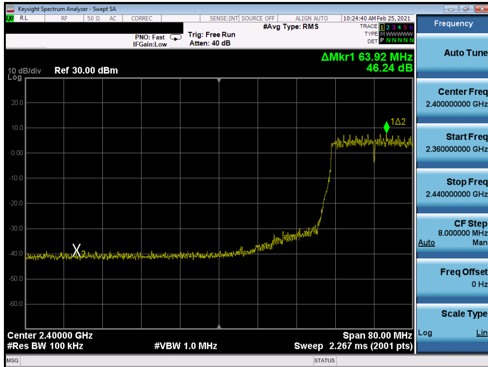
Plot 7-224. Band Edge Plot Antenna WF8 (802.11n (2.4GHz) - Ch. 5) - MCS7
