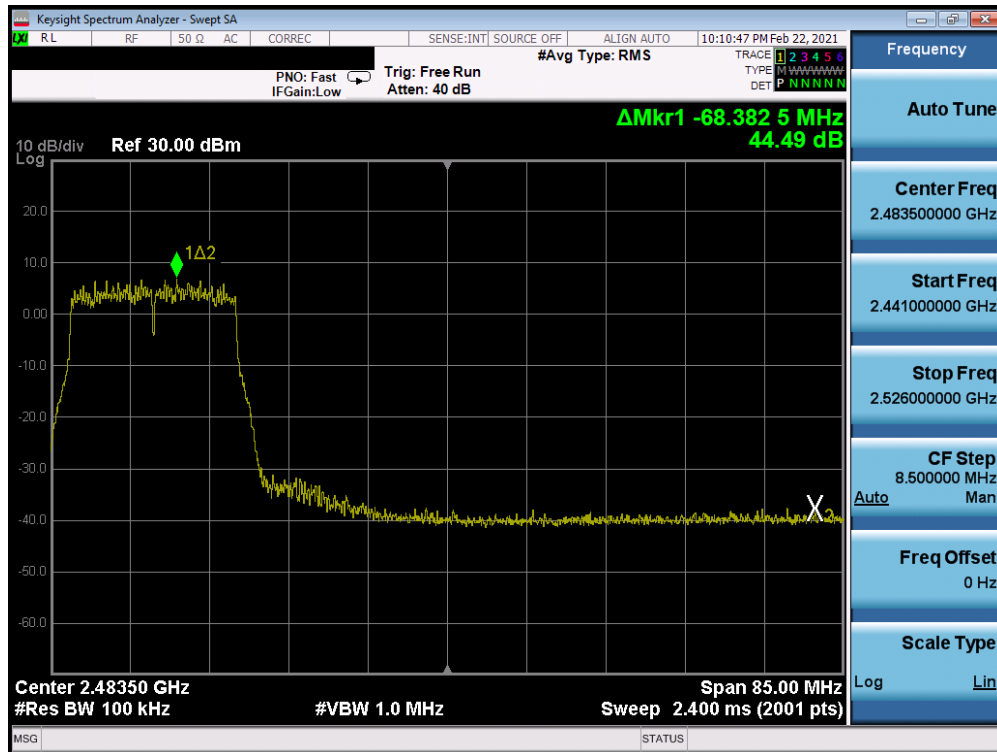
Plot 7-233. Band Edge Plot Antenna WF8 (802.11n (2.4GHz) - Ch. 9) - MCS7
