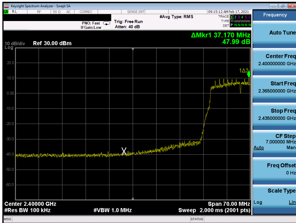
Plot 7-222. Band Edge Plot Antenna WF8 (802.11n (2.4GHz) – Ch. 5) – MCS0
