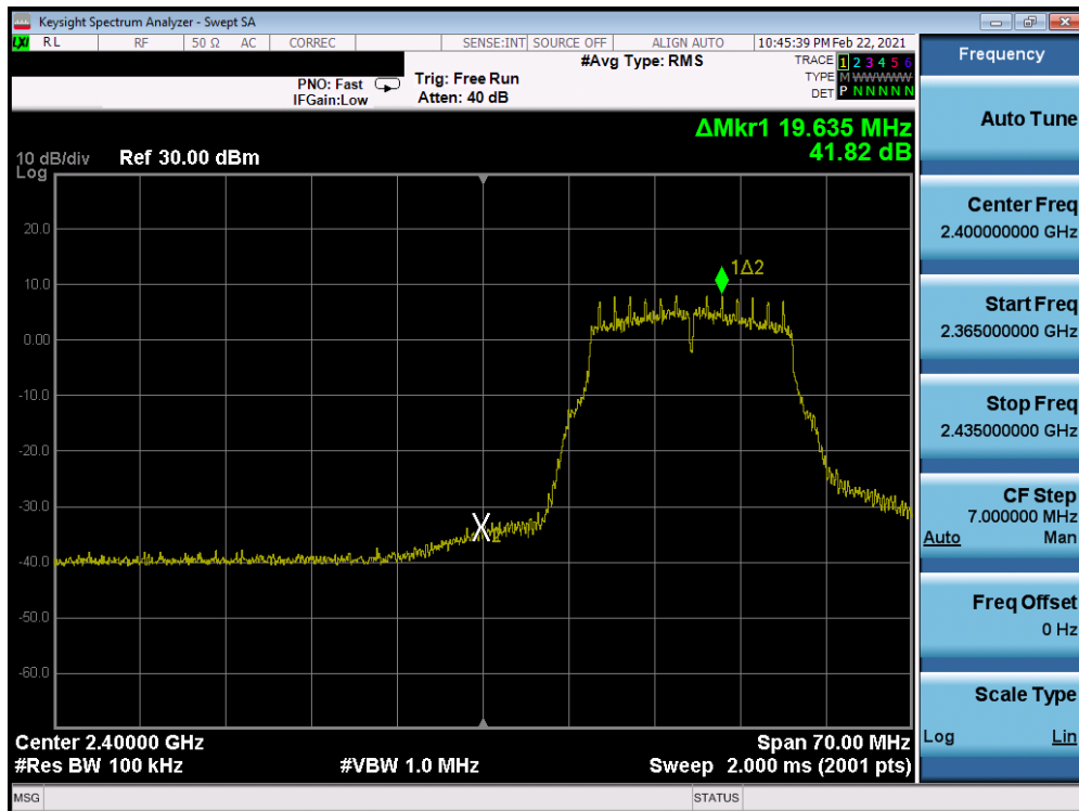
Plot 7-289. Band Edge Plot Antenna WF7 (802.11g- Ch. 2) – 6Mbps
