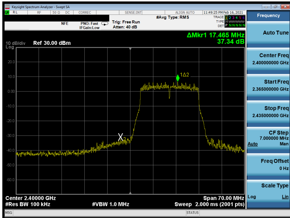
Plot 7-324. Band Edge Plot Antenna WF7 (802.11n (2.4GHz) – Ch. 1) – MCS7
