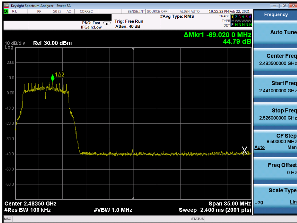
Plot 7-308. Band Edge Plot Antenna WF7 (802.11g - Ch. 9) - 18Mbps
