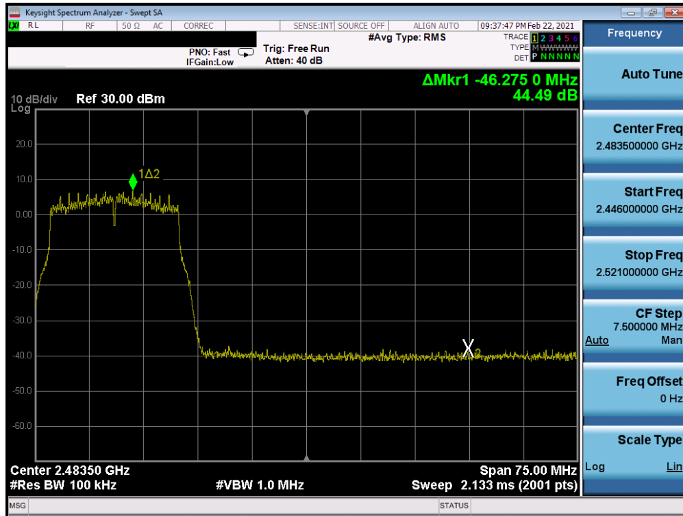
Plot 7-235. Band Edge Plot Antenna WF8 (802.11n (2.4GHz) – Ch. 10) – MCS3
