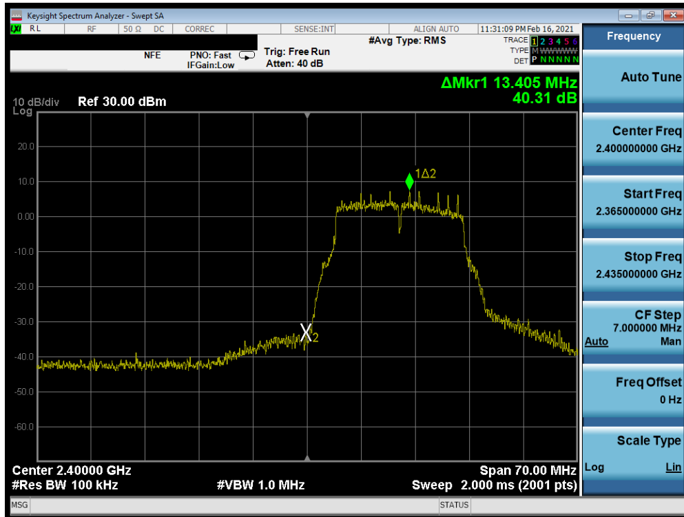
Plot 7-286. Band Edge Plot Antenna WF7 (802.11g- Ch. 1) – 6Mbps
