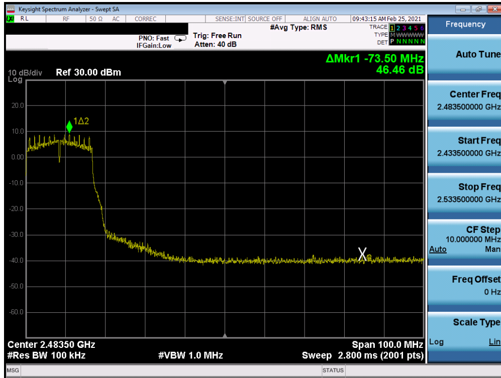
Plot 7-302: Band Edge Plot Antenna WF7 (802.11g - Ch. 7) - 18Mbps
