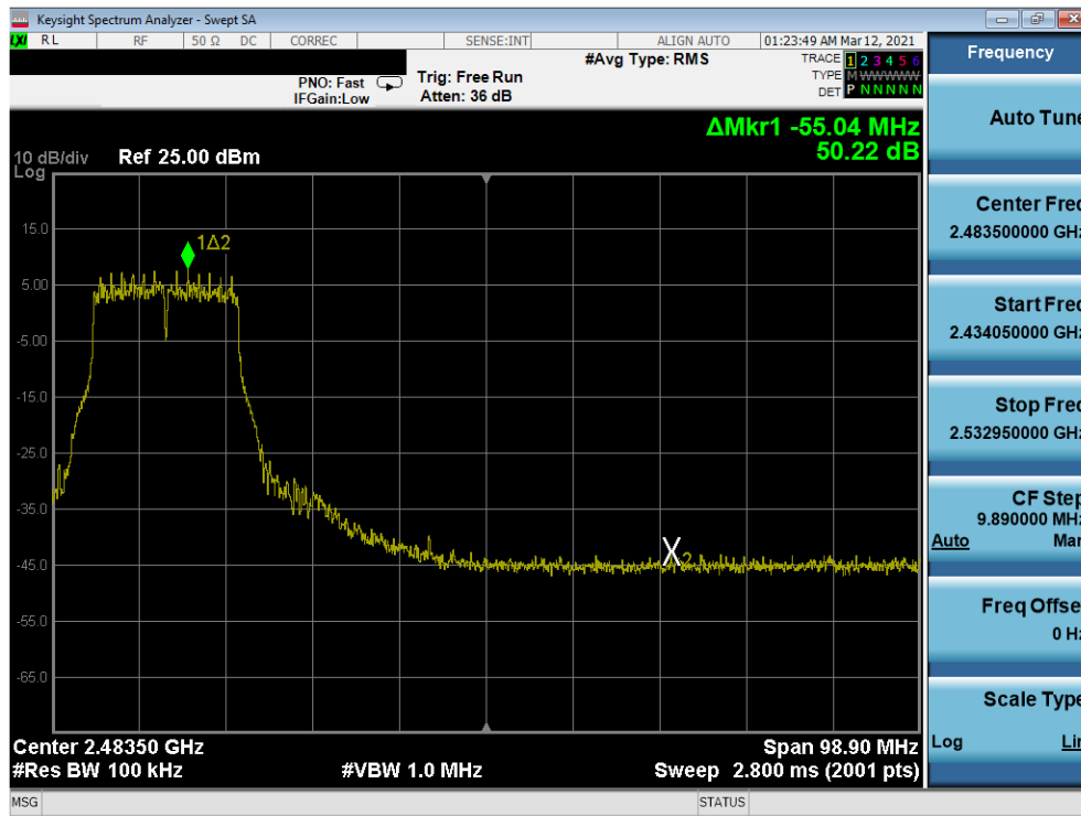
Plot 7-306. Band Edge Plot Antenna WF7 (802.11g - Ch. 8) - 54Mbps
