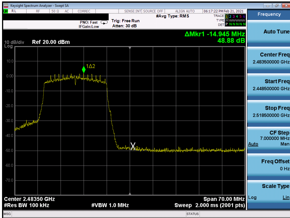
Plot 7-279. Band Edge Plot Antenna WF8 (802.11ax (SU - 2.4GHz) - Ch. 12) - MCS0
