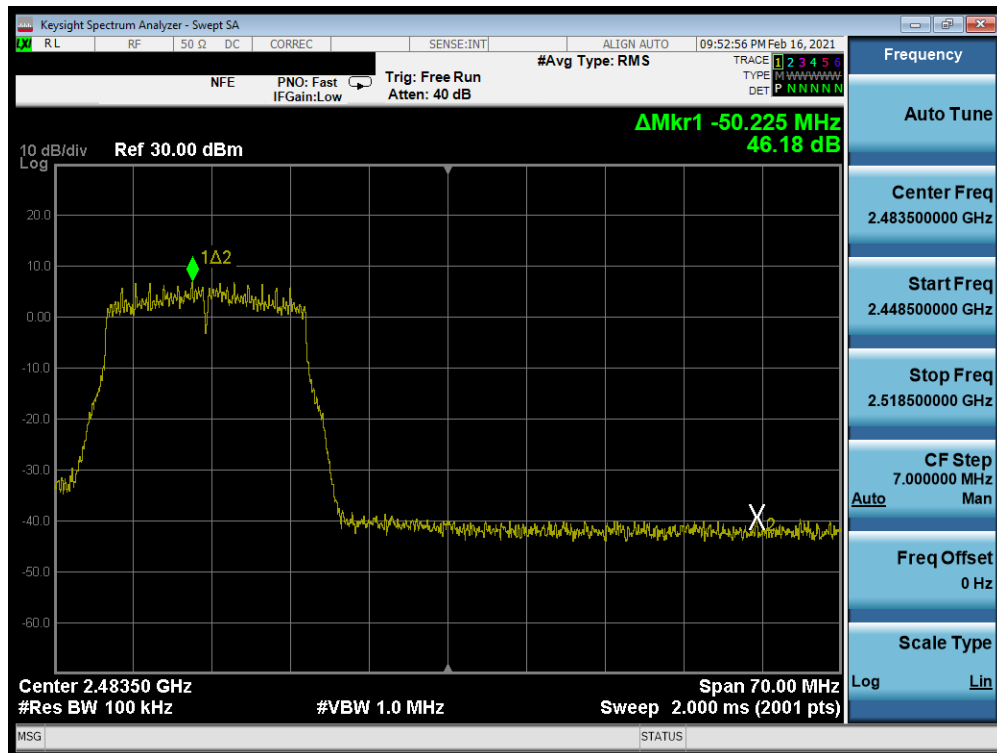
Plot 7-238. Band Edge Plot Antenna WF8 (802.11n (2.4GHz) - Ch. 11) - MCS3
