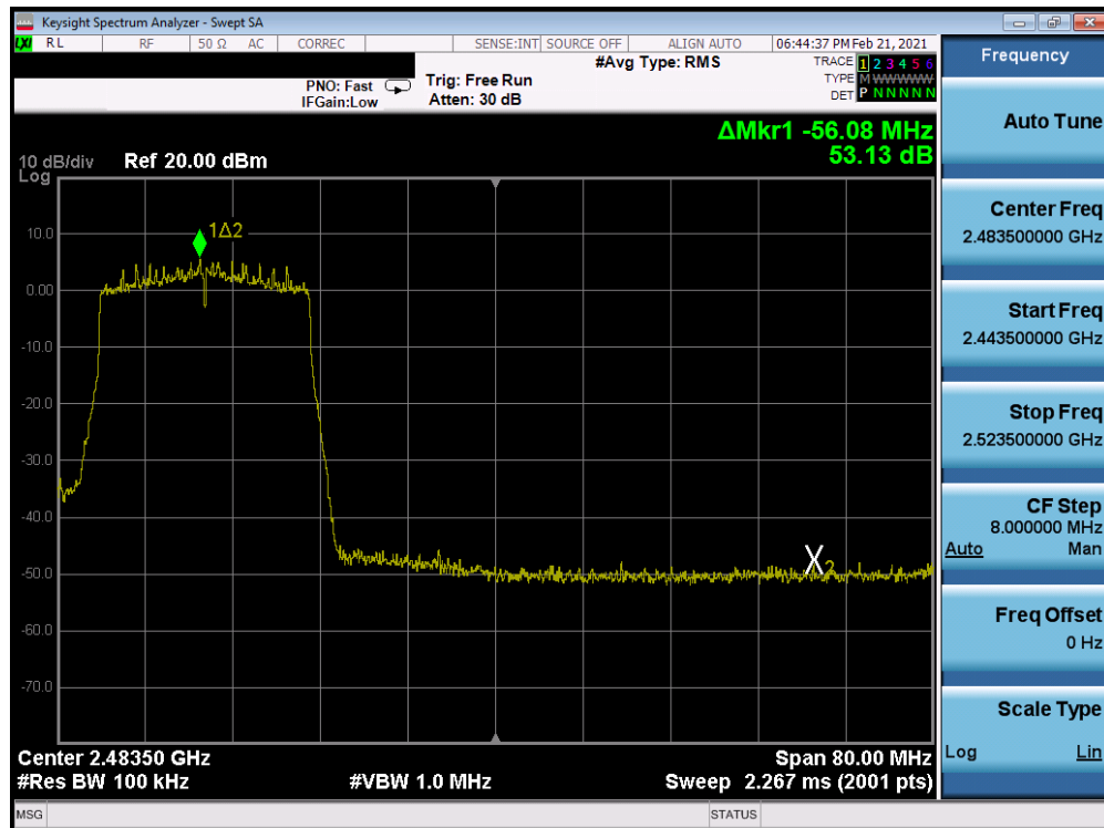
Plot 7-274. Band Edge Plot Antenna WF8 (802.11ax (SU – 2.4GHz) – Ch. 10) – MCS3
