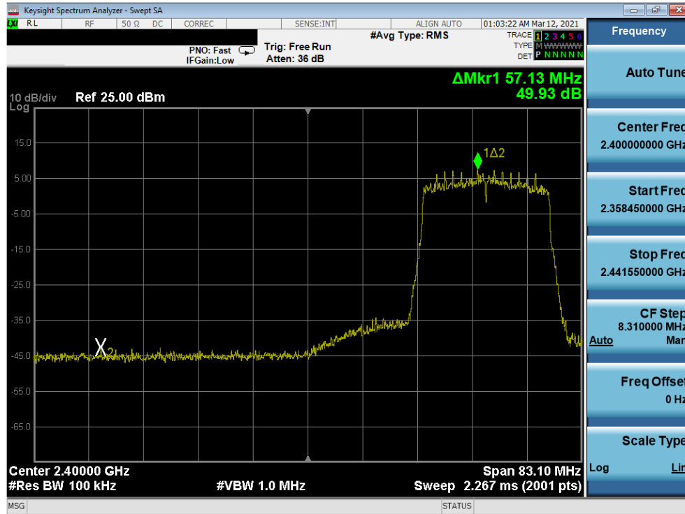
Plot 7-255: Band Edge Plot Antenna WF8 (802.11ax (SU – 2.4GHz) – Ch. 4) – MCS0
