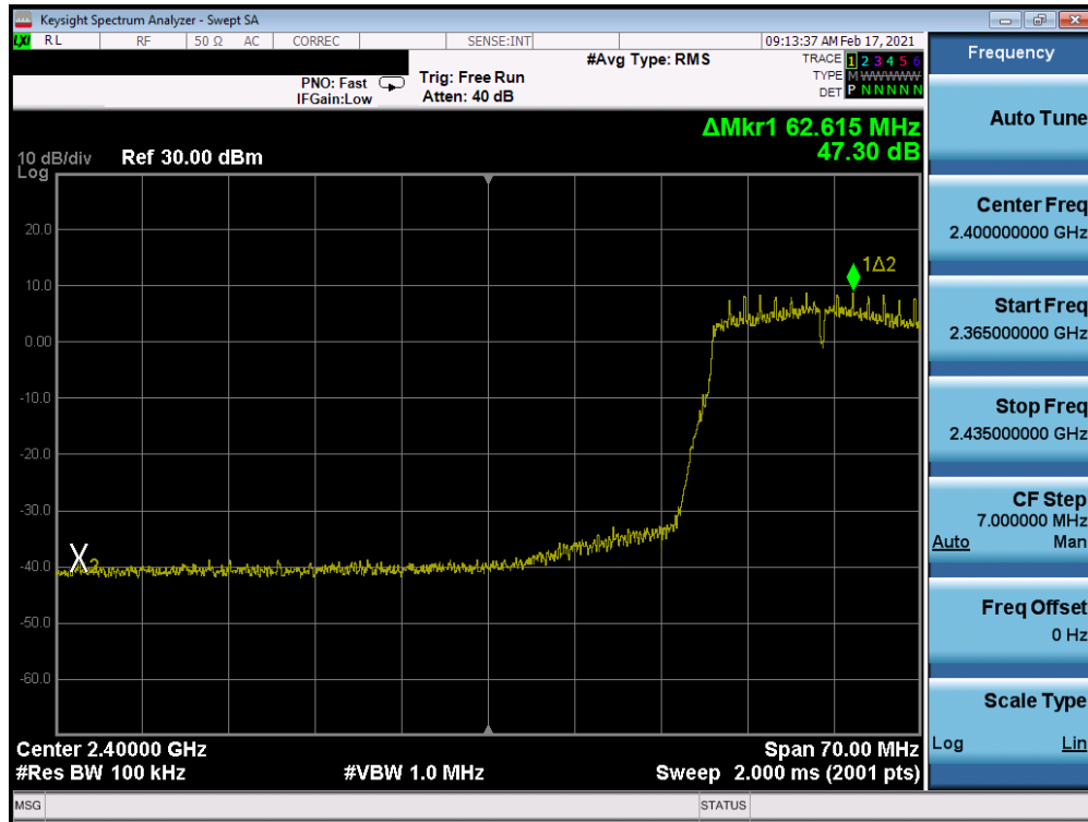
Plot 7-219: Band Edge Plot Antenna WF8 (802.11n (2.4GHz) – Ch. 4) – MCS0
