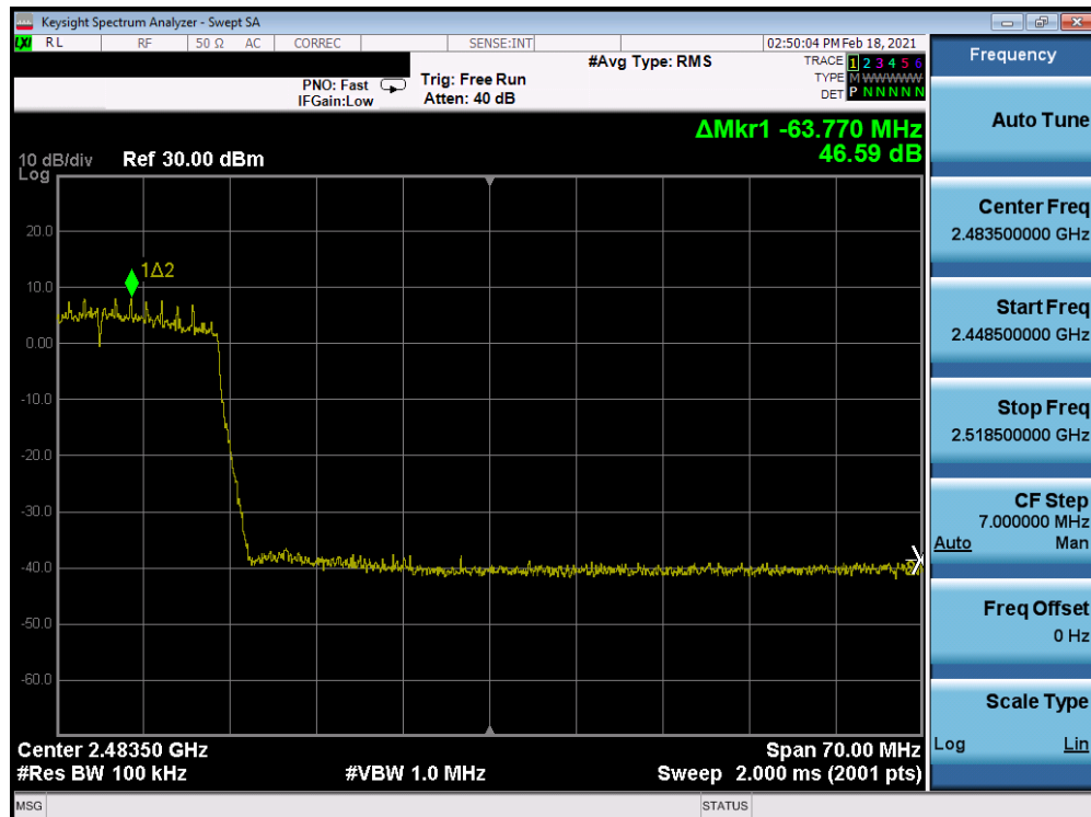
Plot 7-270: Band Edge Plot Antenna WF8 (802.11ax (SU – 2.4GHz) – Ch. 9) – MCS0
