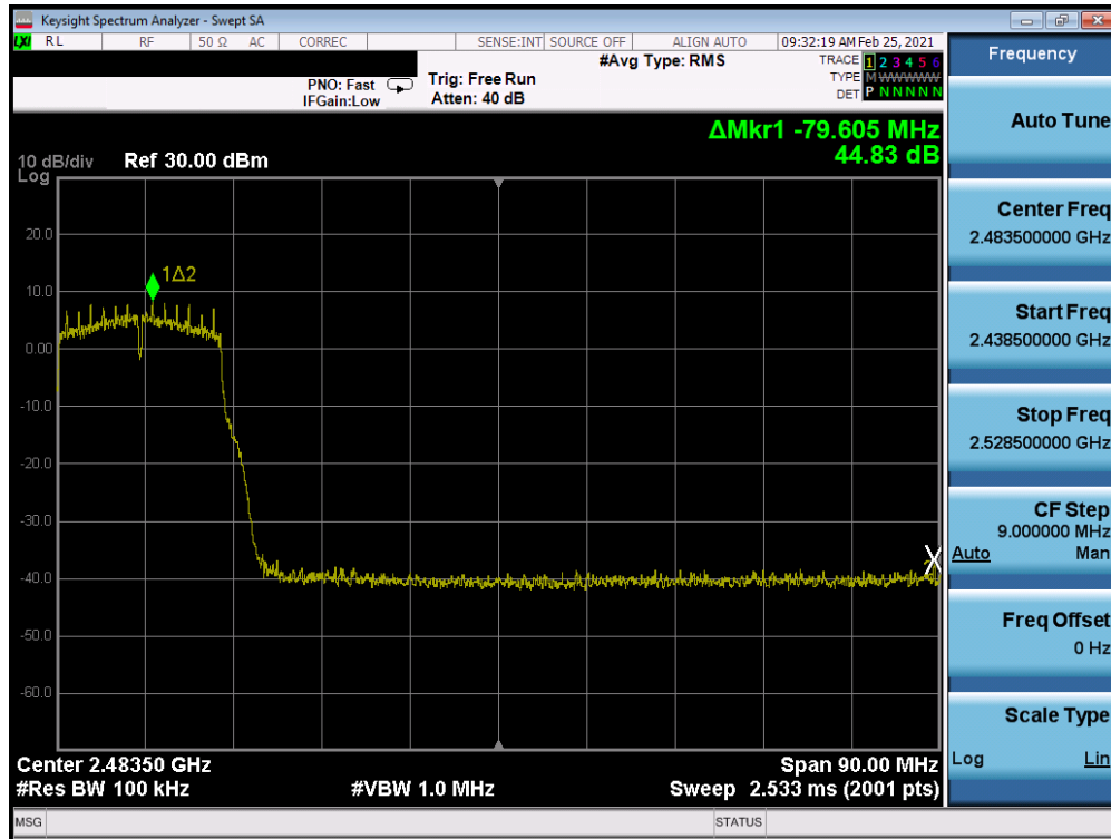
Plot 7-304: Band Edge Plot Antenna WF7 (802.11g - Ch. 8) - 6Mbps
