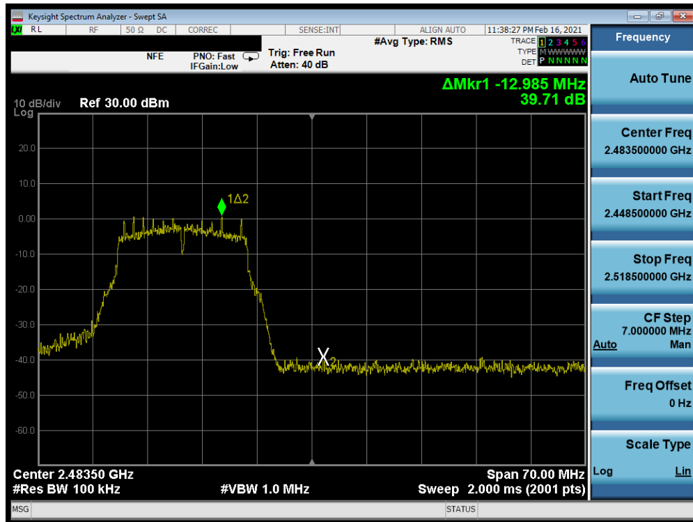
Plot 7-316. Band Edge Plot Antenna WF7 (802.11g – Ch. 12) – 6Mbps
