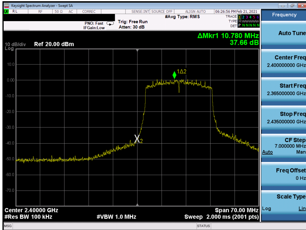
Plot 7-247. Band Edge Plot Antenna WF8 (802.11ax (SU – 2.4GHz) – Ch. 1) – MCS3
