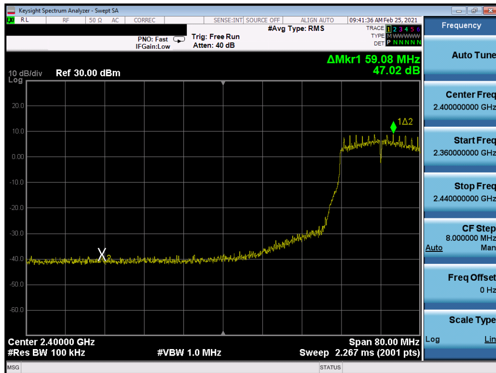
Plot 7-299. Band Edge Plot Antenna WF7 (802.11g- Ch. 5) – 18Mbps
