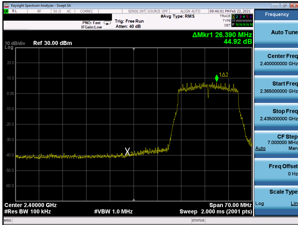
Plot 7-217. Band Edge Plot Antenna WF8 (802.11n (2.4GHz) – Ch. 3) – MCS3
