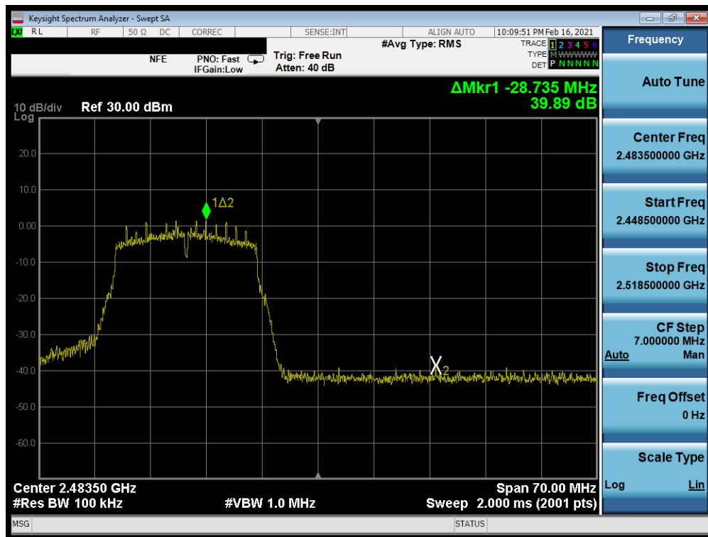
Plot 7-240. Band Edge Plot Antenna WF8 (802.11n (2.4GHz) - Ch. 12) - MCS0
