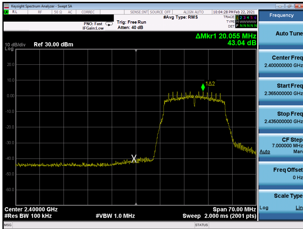
Plot 7-213. Band Edge Plot Antenna WF8 (802.11n (2.4GHz) – Ch. 2) – MCS0
