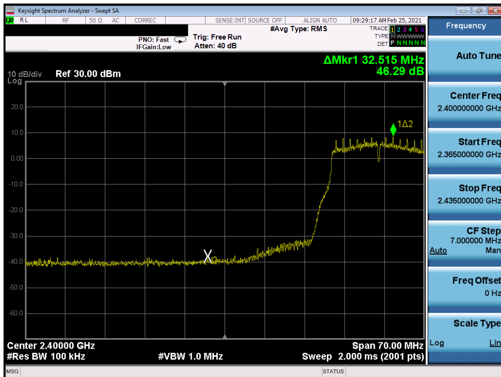
Plot 7-295: Band Edge Plot Antenna WF7 (802.11g- Ch. 4) – 6Mbps
