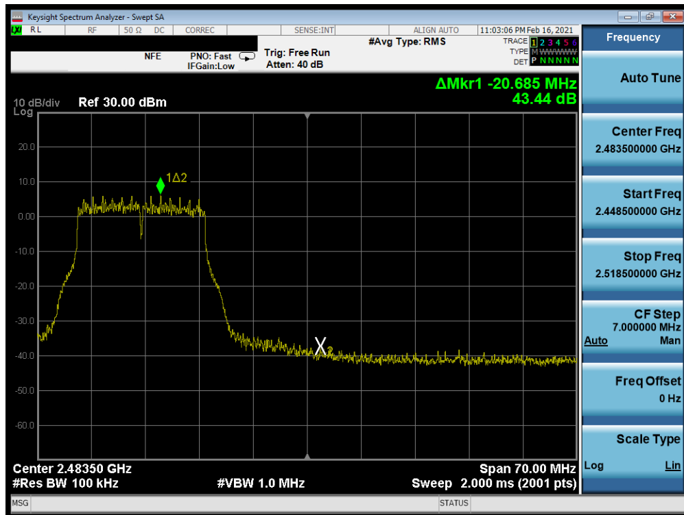
Plot 7-315. Band Edge Plot Antenna WF7 (802.11g - Ch. 11) – 54Mbps
