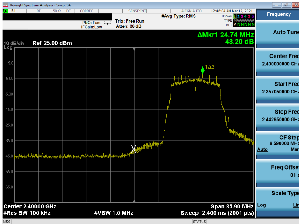
Plot 7-216. Band Edge Plot Antenna WF8 (802.11n (2.4GHz) – Ch. 3) – MCS0
