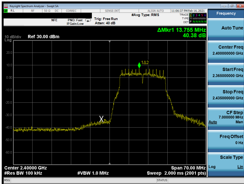
Plot 7-287. Band Edge Plot Antenna WF7 (802.11g- Ch. 1) – 18Mbps
