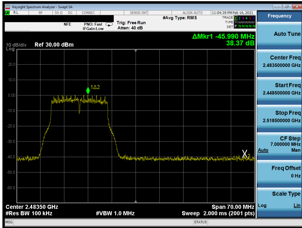
Plot 7-318. Band Edge Plot Antenna WF7 (802.11g – Ch. 12) – 54Mbps
