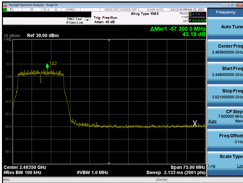
Plot 7-236. Band Edge Plot Antenna WF8 (802.11n (2.4GHz) – Ch. 10) – MCS7
