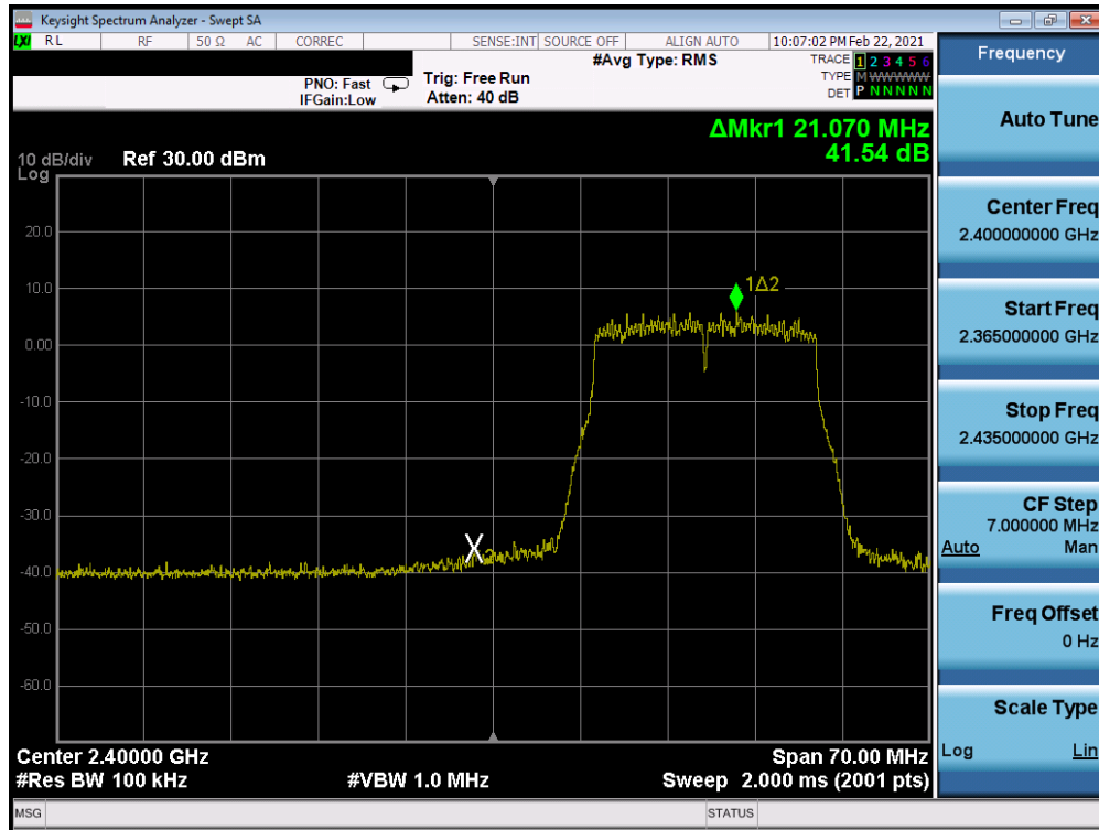
Plot 7-215. Band Edge Plot Antenna WF8 (802.11n (2.4GHz) – Ch. 2) – MCS7
