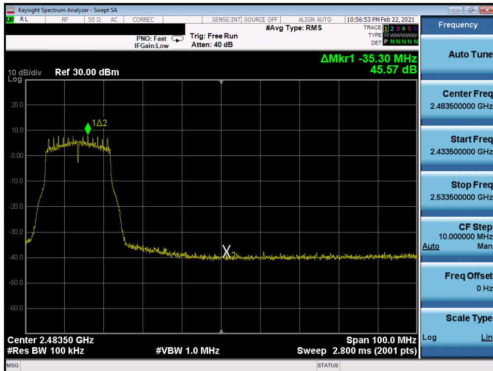
Plot 7-305. Band Edge Plot Antenna WF7 (802.11g - Ch. 8) - 18Mbps
