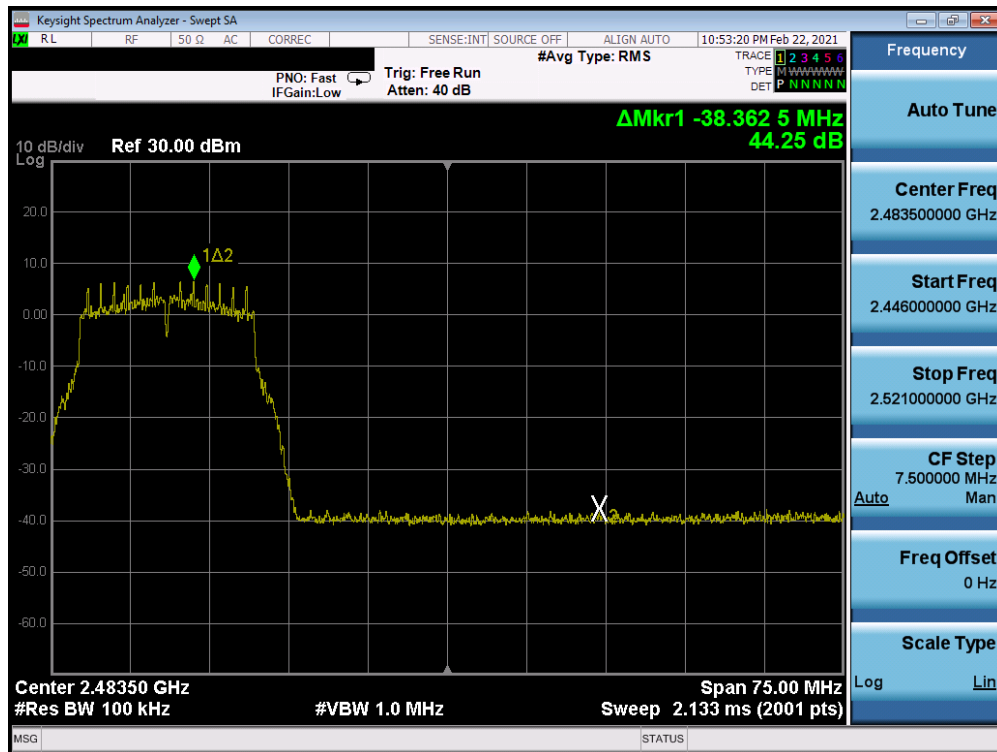
Plot 7-311. Band Edge Plot Antenna WF7 (802.11g - Ch. 10) - 18Mbps
