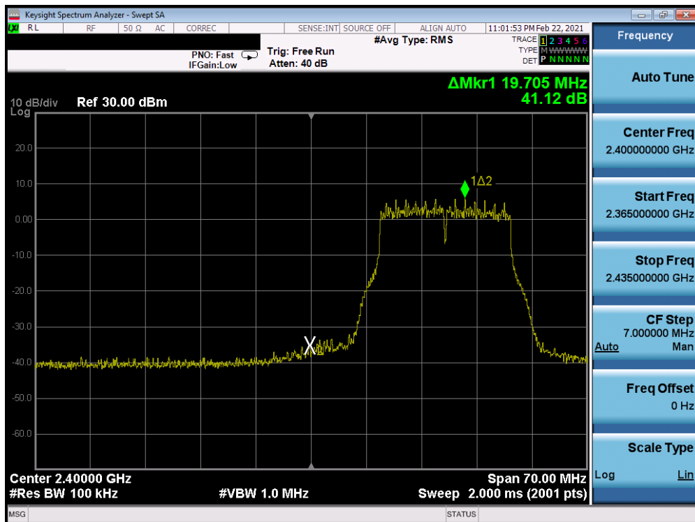
Plot 7-291. Band Edge Plot Antenna WF7 (802.11g- Ch. 2) – 54Mbps
