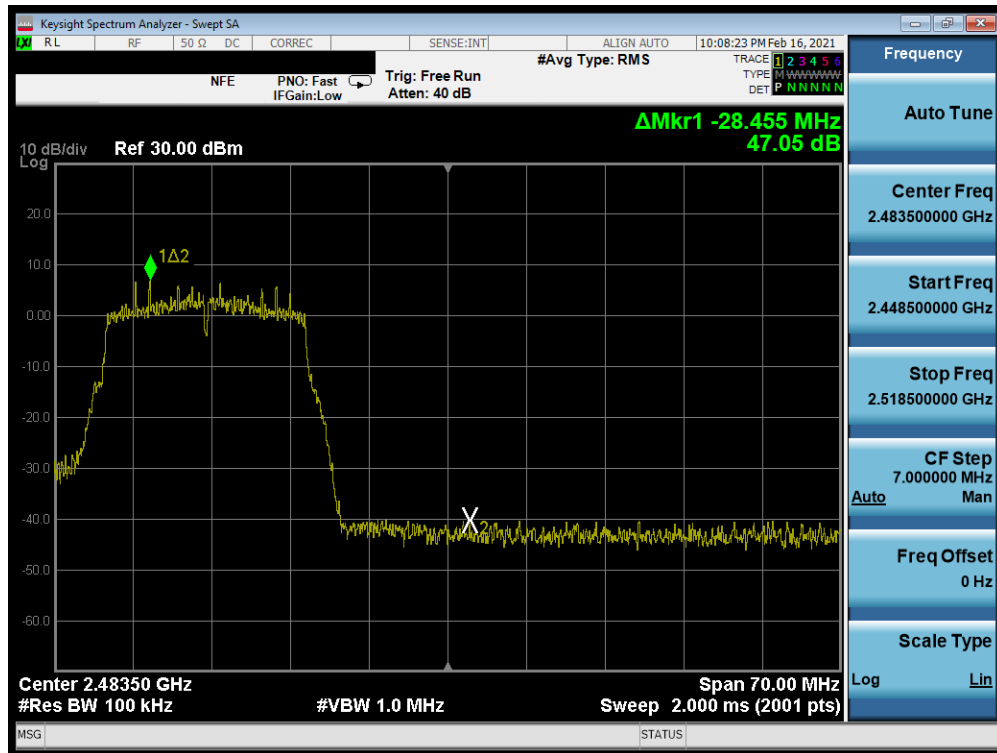
Plot 7-237. Band Edge Plot Antenna WF8 (802.11n (2.4GHz) - Ch. 11) - MCS0
