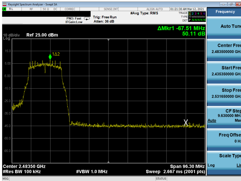
Plot 7-307. Band Edge Plot Antenna WF7 (802.11g - Ch. 9) - 6Mbps
