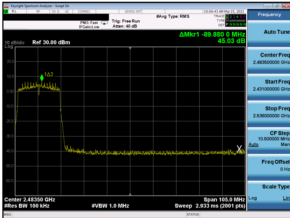
Plot 7-264: Band Edge Plot Antenna WF8 (802.11ax (SU – 2.4GHz) – Ch. 7) – MCS0
