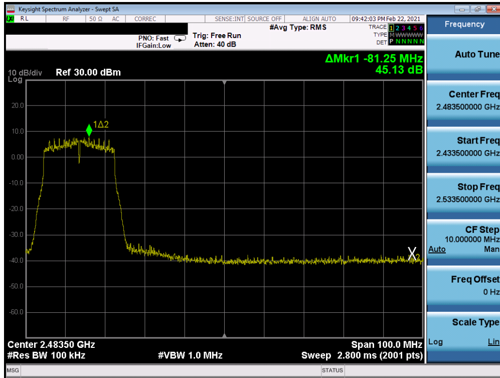
Plot 7-229. Band Edge Plot Antenna WF8 (802.11n (2.4GHz) - Ch. 8) - MCS3
