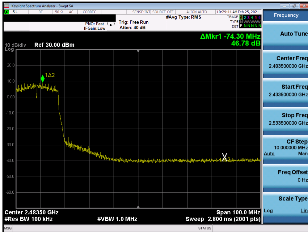
Plot 7-226. Band Edge Plot Antenna WF8 (802.11n (2.4GHz) – Ch. 7) – MCS3
