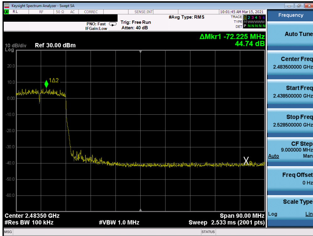
Plot 7-269: Band Edge Plot Antenna WF8 (802.11ax (SU – 2.4GHz) – Ch. 8) – MCS5
