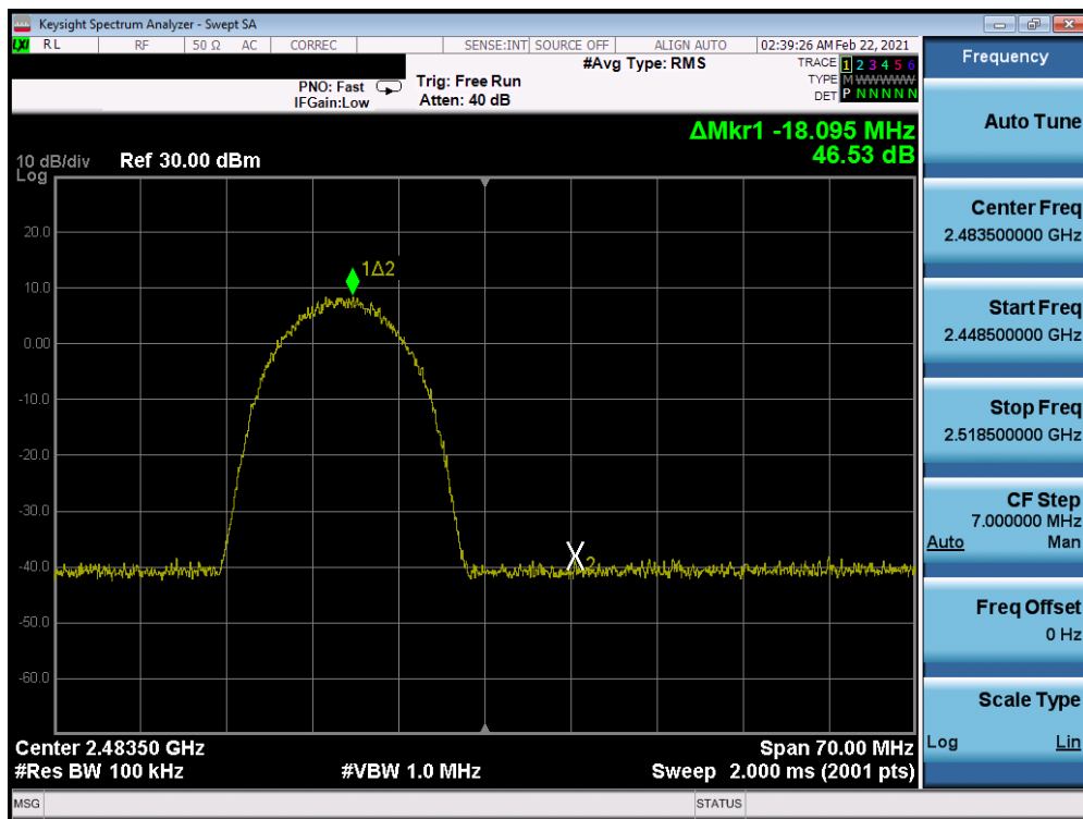
Plot 7-285. Band Edge Plot Antenna WF7 (802.11b - Ch. 13) - 11Mbps
