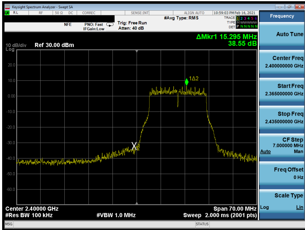
Plot 7-288. Band Edge Plot Antenna WF7 (802.11g- Ch. 1) – 54Mbps
