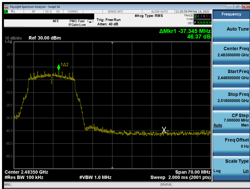
Plot 7-313. Band Edge Plot Antenna WF7 (802.11g – Ch. 11) – 6Mbps
