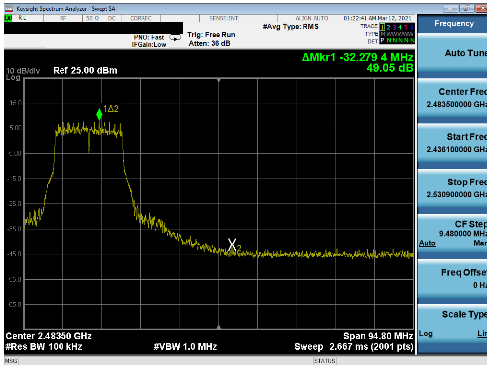
Plot 7-309. Band Edge Plot Antenna WF7 (802.11g - Ch. 9) - 54Mbps
