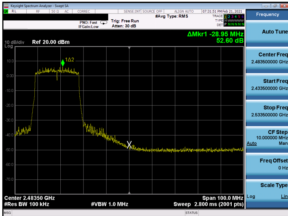
Plot 7-272. Band Edge Plot Antenna WF8 (802.11ax (SU – 2.4GHz) – Ch. 9) – MCS5
