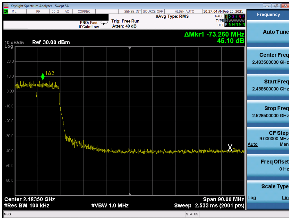
Plot 7-230. Band Edge Plot Antenna WF8 (802.11n (2.4GHz) - Ch. 8) - MCS7
