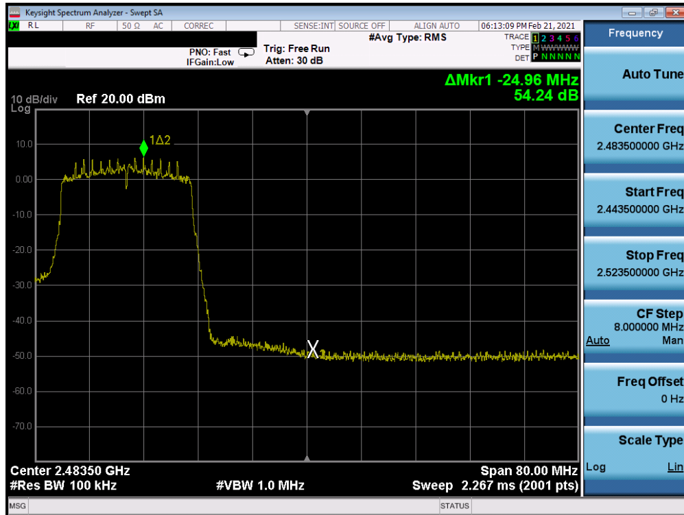
Plot 7-273. Band Edge Plot Antenna WF8 (802.11ax (SU – 2.4GHz) – Ch. 10) – MCS0
