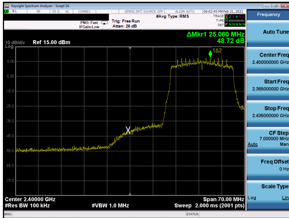
Plot 7-252. Band Edge Plot Antenna WF8 (802.11ax (SU – 2.4GHz) – Ch. 3) – MCS0
