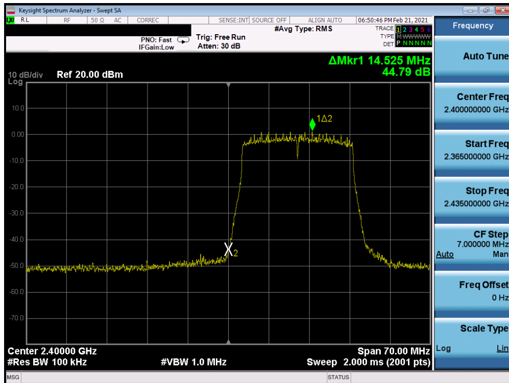
Plot 7-248. Band Edge Plot Antenna WF8 (802.11ax (SU – 2.4GHz) – Ch. 1) – MCS5
