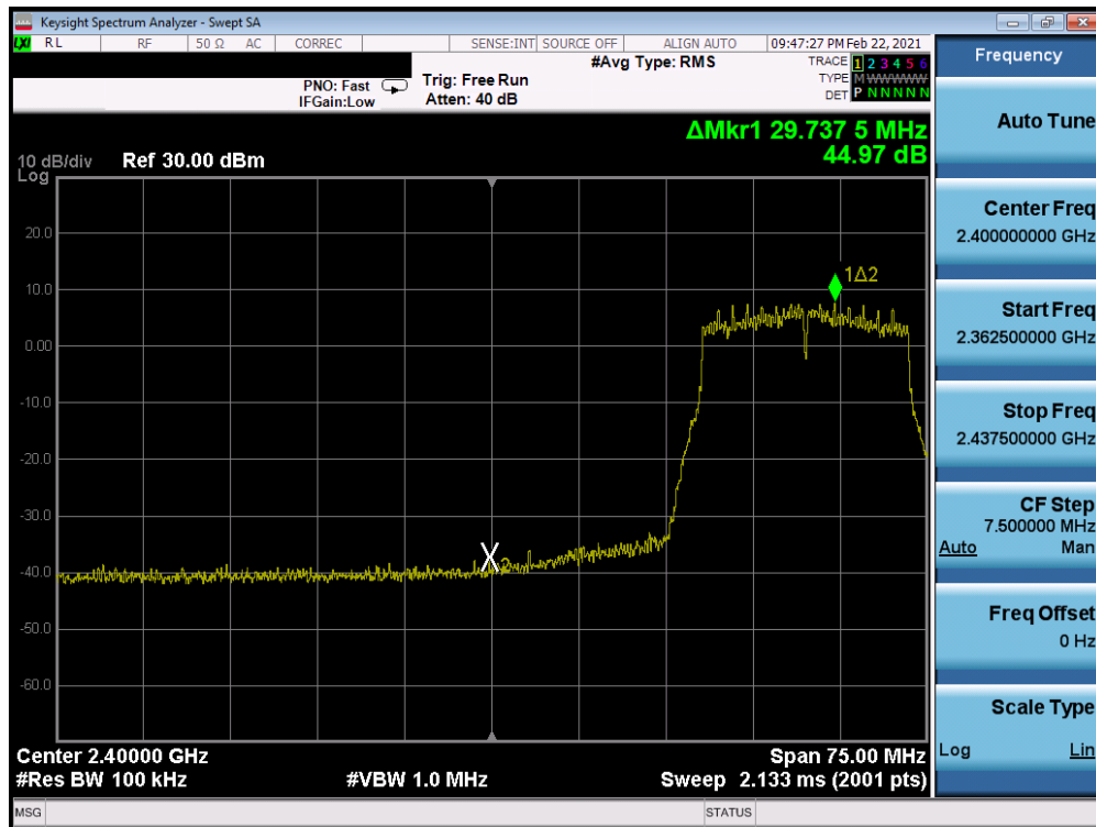
Plot 7-220: Band Edge Plot Antenna WF8 (802.11n (2.4GHz) – Ch. 4) – MCS3
