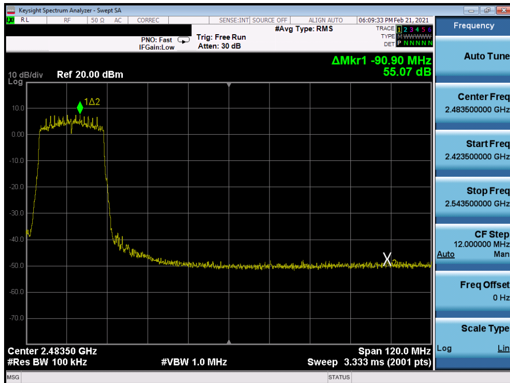
Plot 7-262: Band Edge Plot Antenna WF8 (802.11ax (SU – 2.4GHz) – Ch. 6) – MCS0
