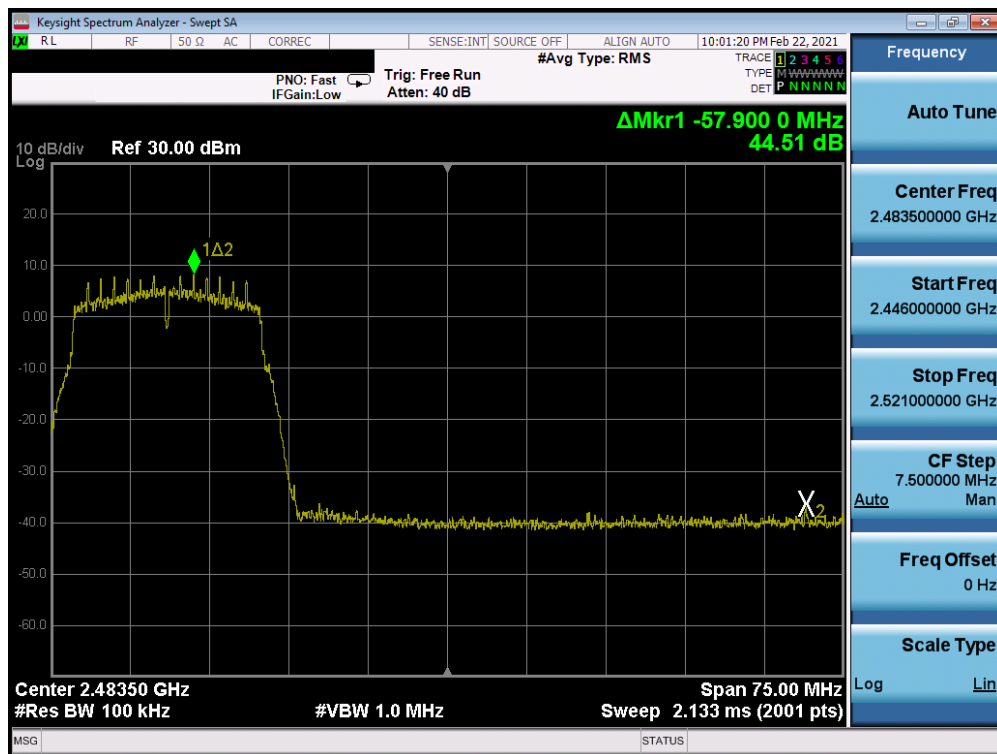
Plot 7-234. Band Edge Plot Antenna WF8 (802.11n (2.4GHz) - Ch. 10) - MCS0
