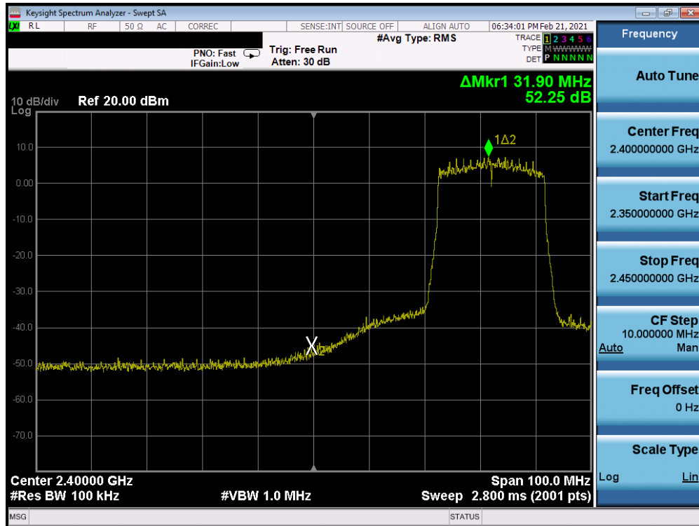
Plot 7-259. Band Edge Plot Antenna WF8 (802.11ax (SU – 2.4GHz) – Ch. 5) – MCS3
