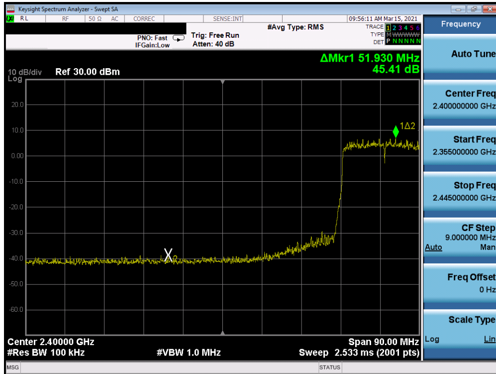
Plot 7-261: Band Edge Plot Antenna WF8 (802.11ax (SU – 2.4GHz) – Ch. 6) – MCS5
