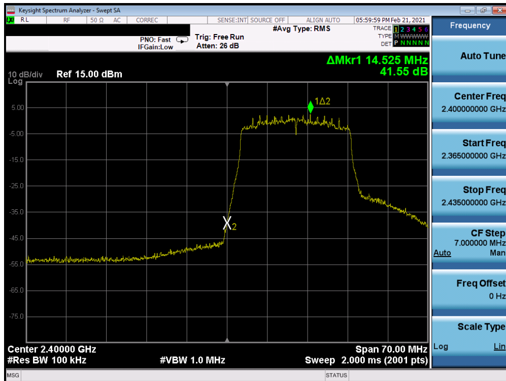
Plot 7-246. Band Edge Plot Antenna WF8 (802.11ax (SU – 2.4GHz) – Ch. 1) – MCS0
