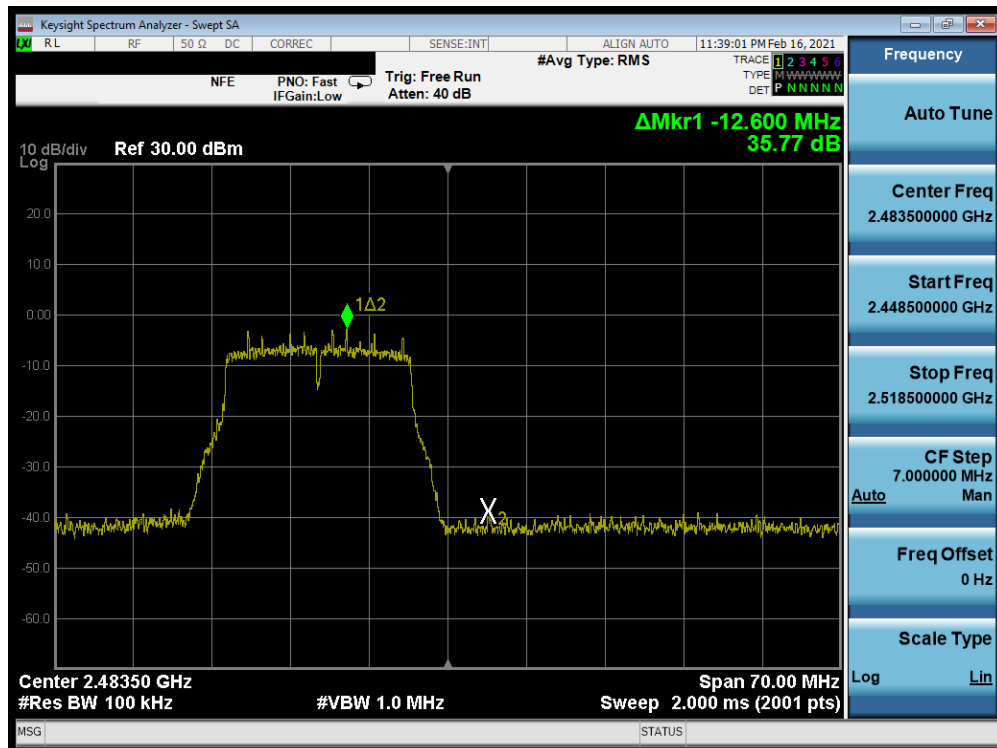
Plot 7-319. Band Edge Plot Antenna WF7 (802.11g – Ch. 13) – 6Mbps
