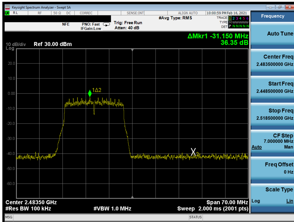
Plot 7-244. Band Edge Plot Antenna WF8 (802.11n (2.4GHz) – Ch. 13) – MCS3
