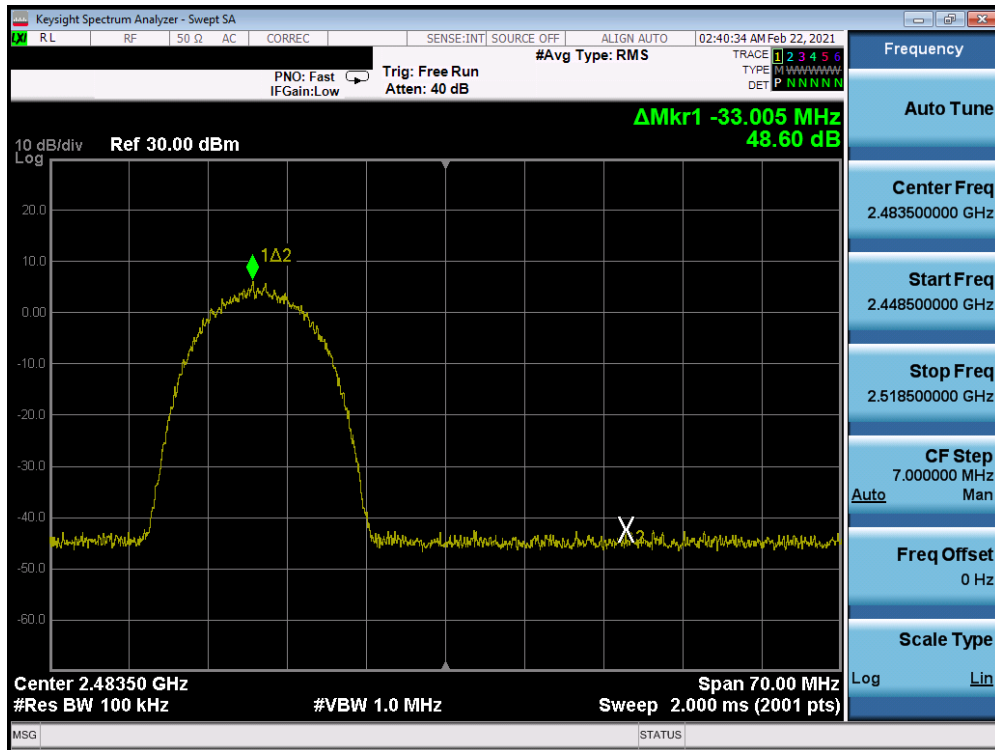
Plot 7-284. Band Edge Plot Antenna WF7 (802.11b - Ch. 12) - 11Mbps
