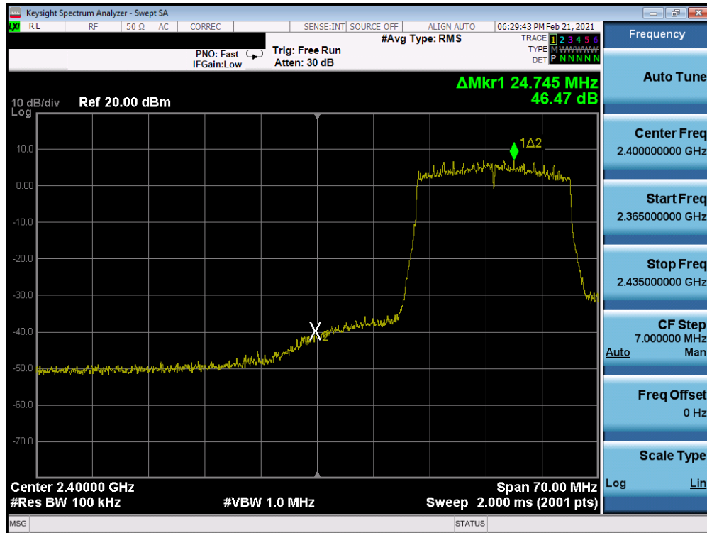
Plot 7-253. Band Edge Plot Antenna WF8 (802.11ax (SU – 2.4GHz) – Ch. 3) – MCS3
