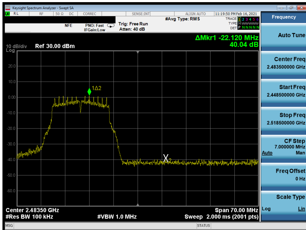
Plot 7-317. Band Edge Plot Antenna WF7 (802.11g – Ch. 12) – 18Mbps
