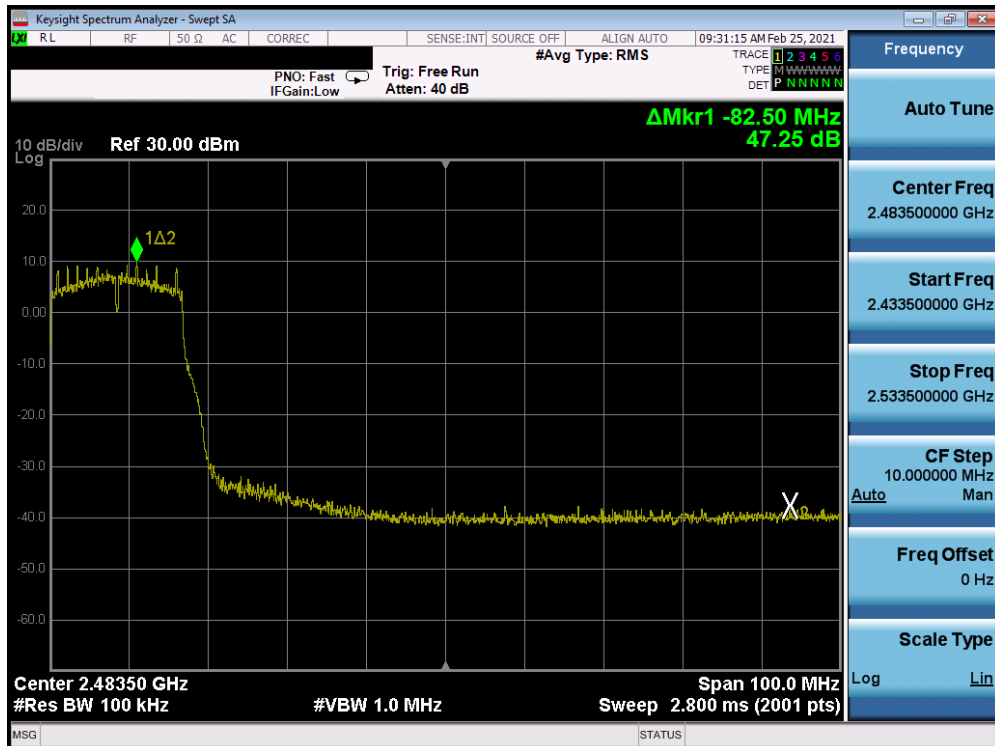
Plot 7-301:Band Edge Plot Antenna WF7 (802.11g - Ch. 7) – 6Mbps
