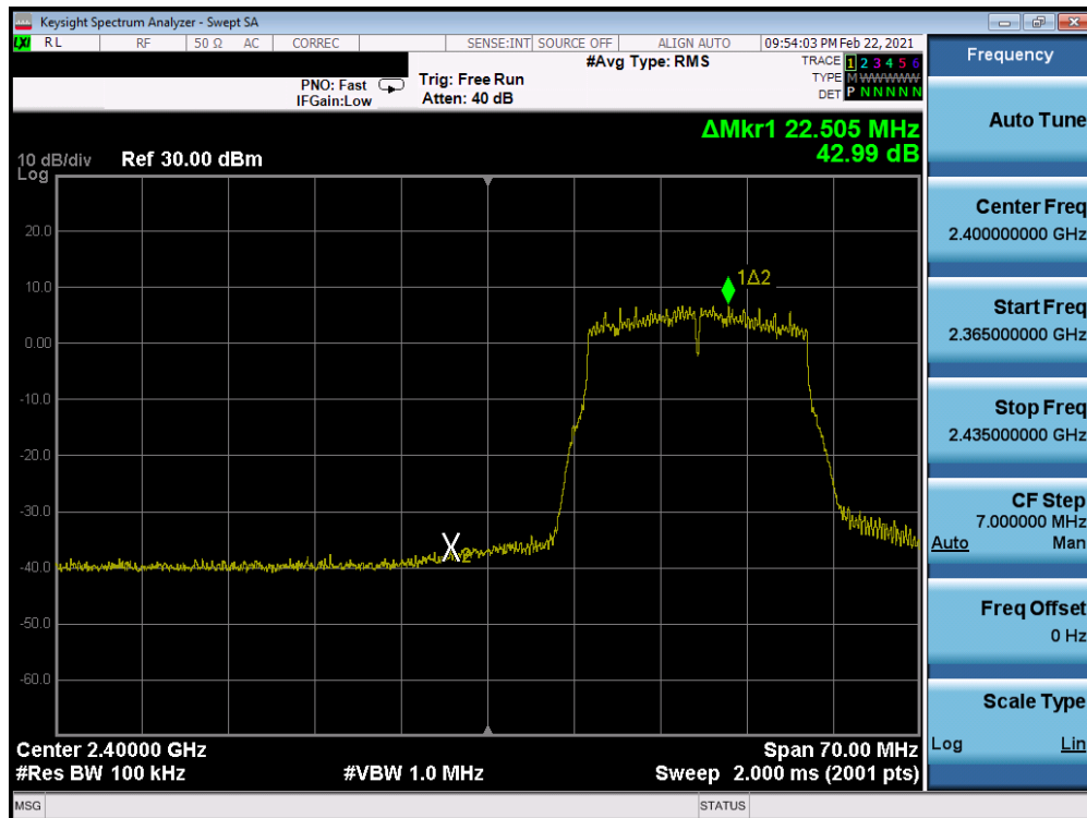
Plot 7-214. Band Edge Plot Antenna WF8 (802.11n (2.4GHz) – Ch. 2) – MCS3
