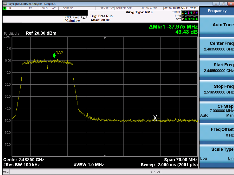
Plot 7-281. Band Edge Plot Antenna WF8 (802.11ax (SU – 2.4GHz) – Ch. 12) – MCS5
