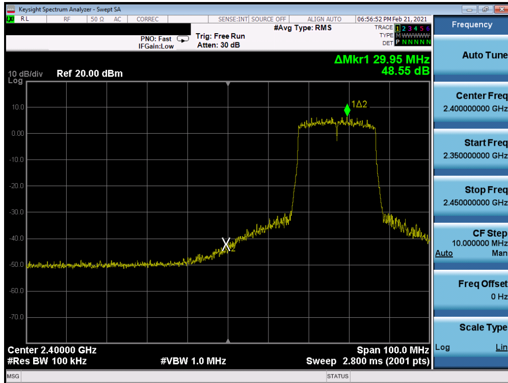
Plot 7-257. Band Edge Plot Antenna WF8 (802.11ax (SU – 2.4GHz) – Ch. 4) – MCS5
