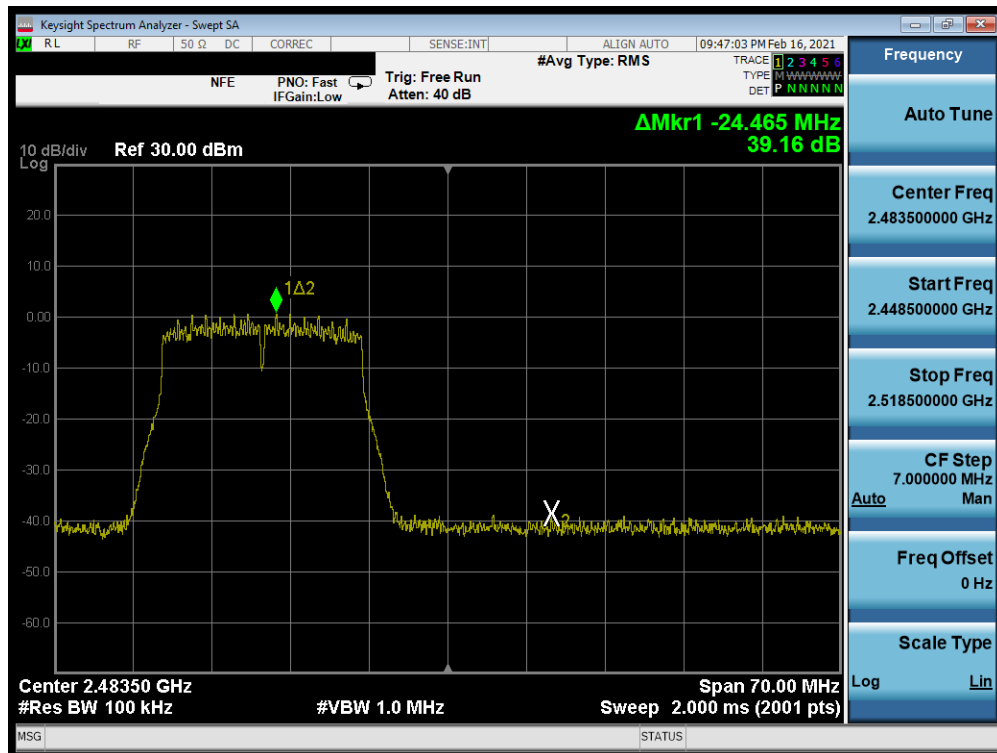
Plot 7-242. Band Edge Plot Antenna WF8 (802.11n (2.4GHz) – Ch. 12) – MCS7
