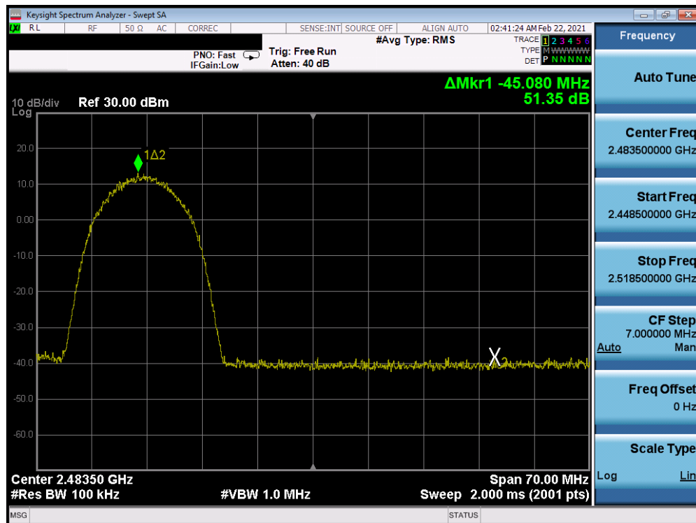
Plot 7-283. Band Edge Plot Antenna WF7 (802.11b – Ch. 11) – 11Mbps
