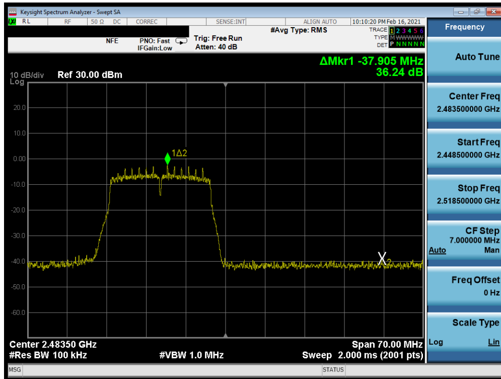
Plot 7-243. Band Edge Plot Antenna WF8 (802.11n (2.4GHz) – Ch. 13) – MCS0
