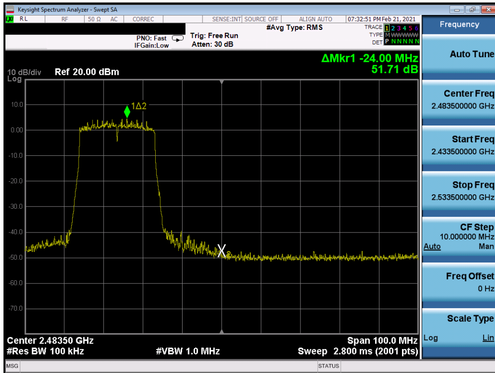
Plot 7-275. Band Edge Plot Antenna WF8 (802.11ax (SU – 2.4GHz) – Ch. 10) – MCS5
