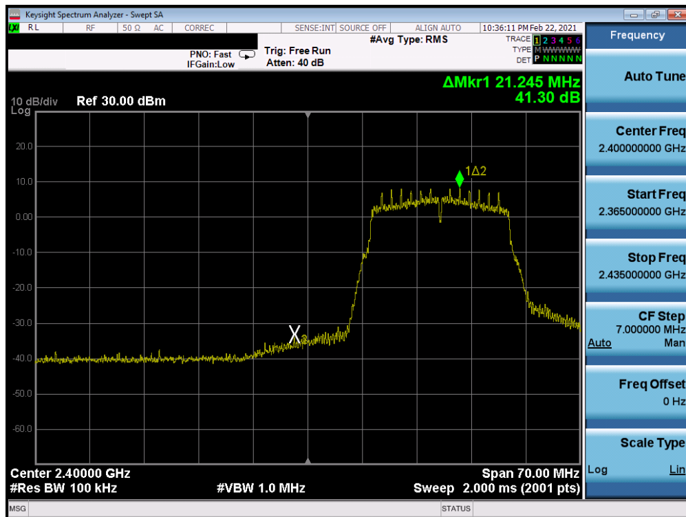
Plot 7-325. Band Edge Plot Antenna WF7 (802.11n (2.4GHz) – Ch. 2) – MCS0
