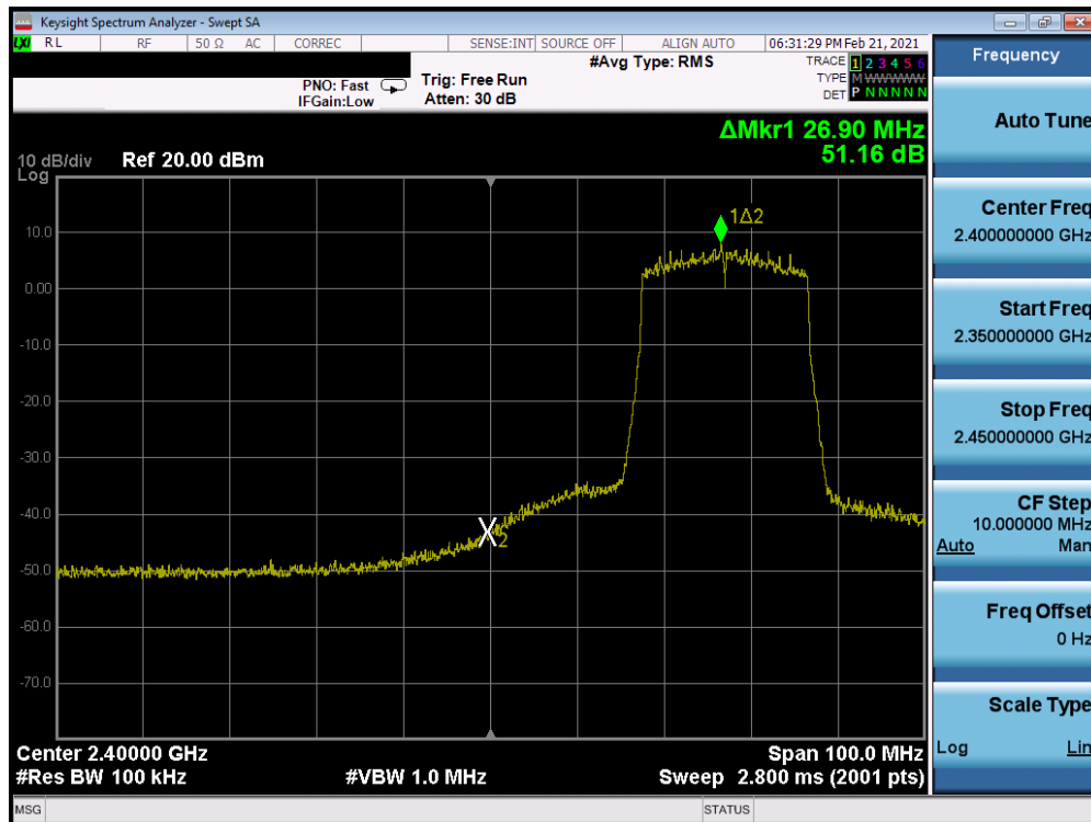
Plot 7-256. Band Edge Plot Antenna WF8 (802.11ax (SU – 2.4GHz) – Ch. 4) – MCS3
