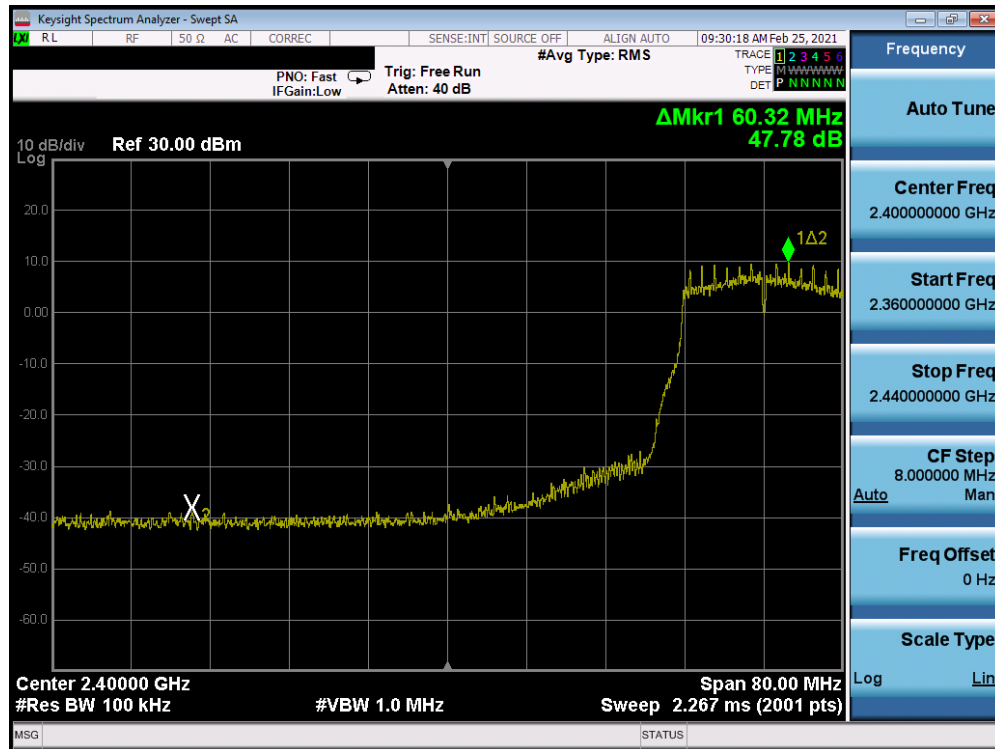
Plot 7-298. Band Edge Plot Antenna WF7 (802.11g- Ch. 5) – 6Mbps
