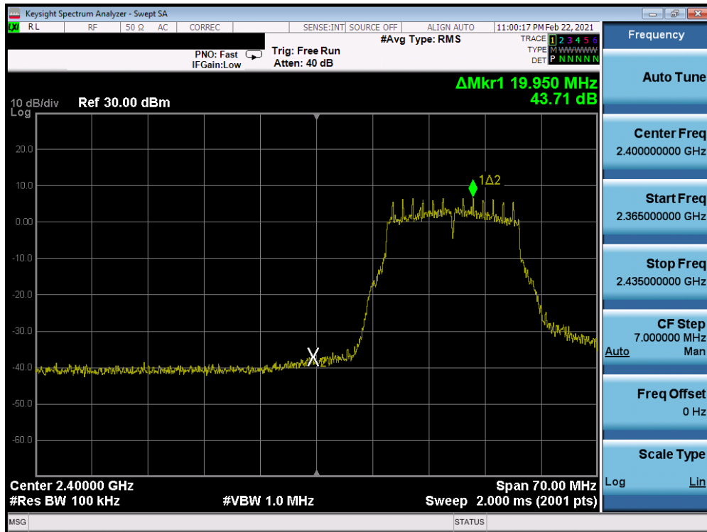
Plot 7-290. Band Edge Plot Antenna WF7 (802.11g- Ch. 2) – 18Mbps
