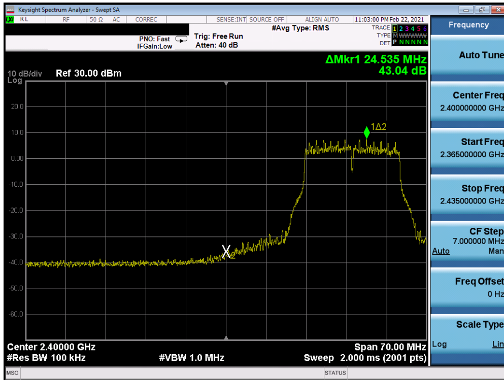
Plot 7-294. Band Edge Plot Antenna WF7 (802.11g- Ch. 3) – 54Mbps
