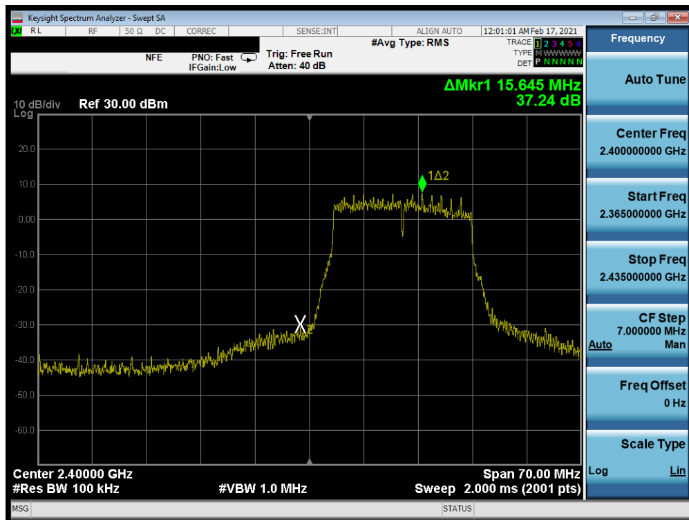
Plot 7-323. Band Edge Plot Antenna WF7 (802.11n (2.4GHz) – Ch. 1) – MCS3
