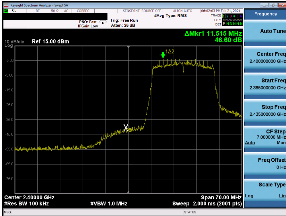
Plot 7-249. Band Edge Plot Antenna WF8 (802.11ax (SU – 2.4GHz) – Ch. 2) – MCS0
