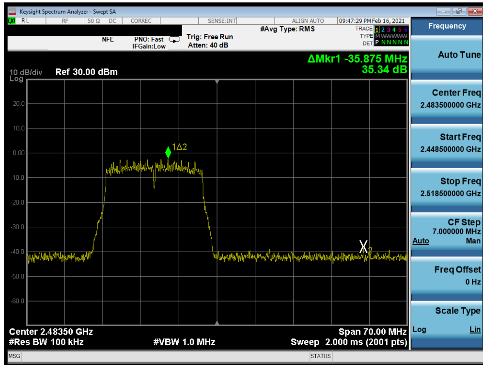
Plot 7-245. Band Edge Plot Antenna WF8 (802.11n (2.4GHz) – Ch. 13) – MCS7
