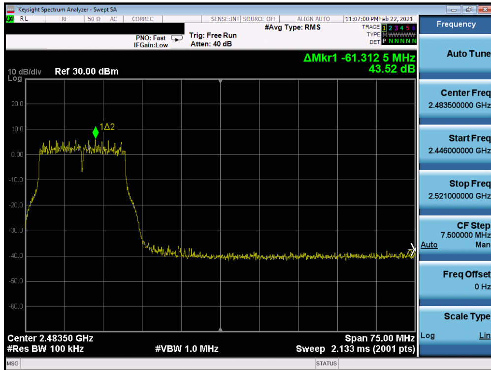
Plot 7-312. Band Edge Plot Antenna WF7 (802.11g – Ch. 10) – 54Mbps
