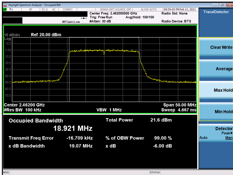
Plot 7-60. 6dB BW and 99% OBW Plot Antenna WF7 (802. 11ax (SU - 2.4GHz) – Ch. 11) – MCS5
