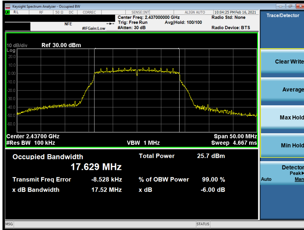
Plot 7-5. 6dB BW and 99% OBW Plot Antenna WF8 (802.11n (2.4GHz) – Ch. 6) – MCS0
