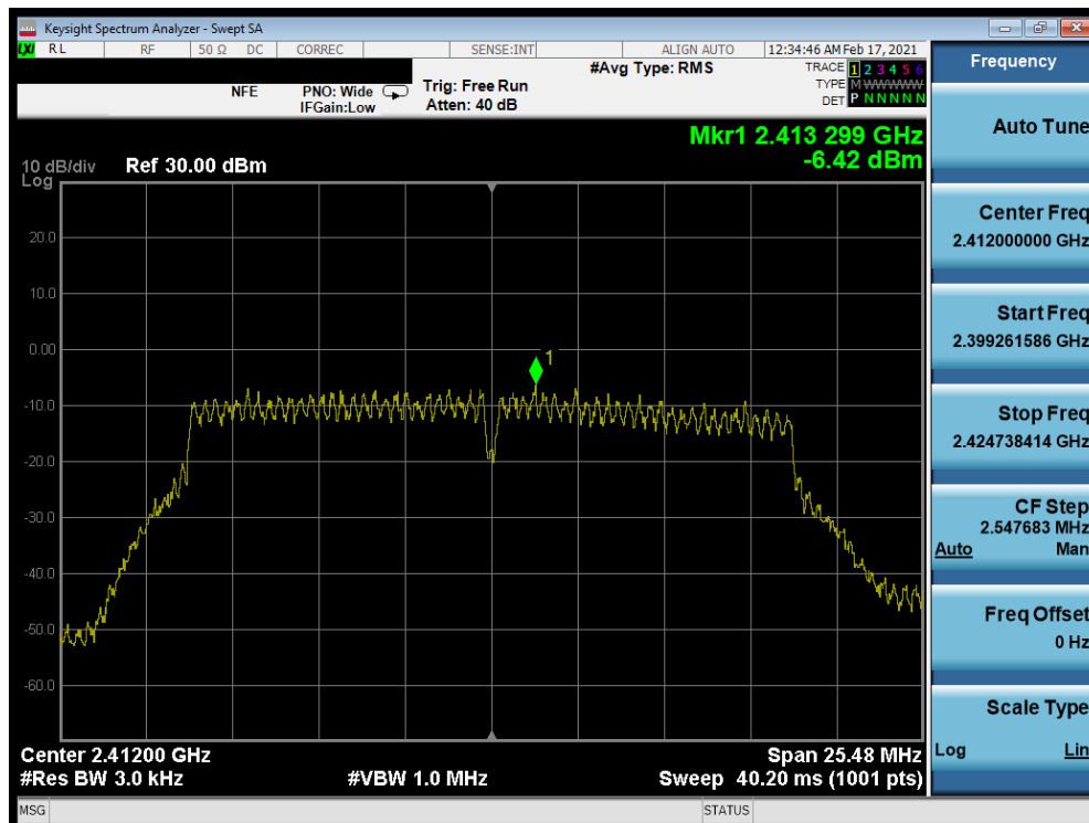
Plot 7-94. Power Spectral Density Plot Antenna WF7 (802.11n (2.4GHz) – Ch. 1) – MCS0
