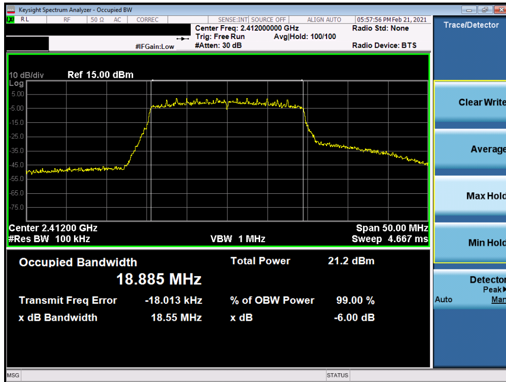
Plot 7-7. 6dB BW and 99% OBW Plot Antenna WF8 (802.11ax (SU - 2.4GHz) – Ch. 1) – MCS0
