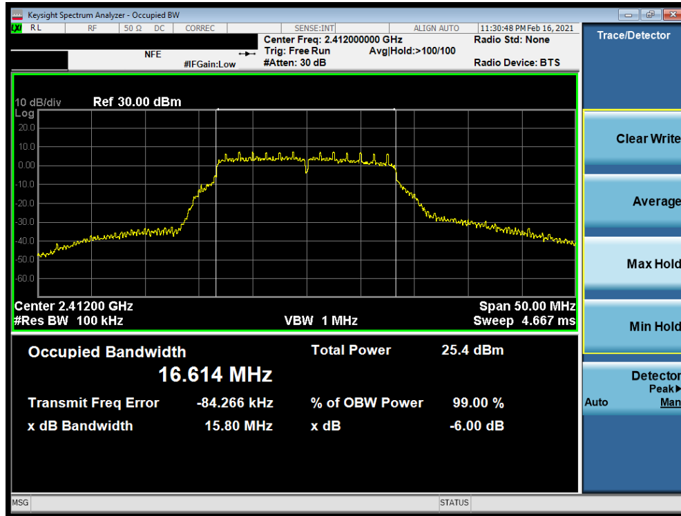
Plot 7-31. 6dB BW and 99% OBW Plot Antenna WF7 (802.11g – Ch. 1) – 6Mbps
