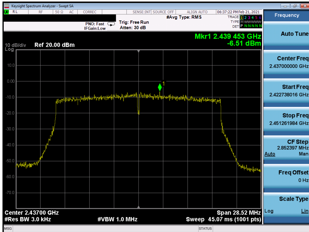
Plot 7-77. Power Spectral Density Plot Antenna WF8 (802.11ax (SU – 2.4GHz) – Ch. 6) – MCS3
