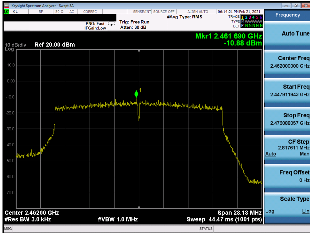
Plot 7-69. Power Spectral Density Plot Antenna WF8 (802.11ax (SU – 2.4GHz) – Ch. 11) – MCS0
