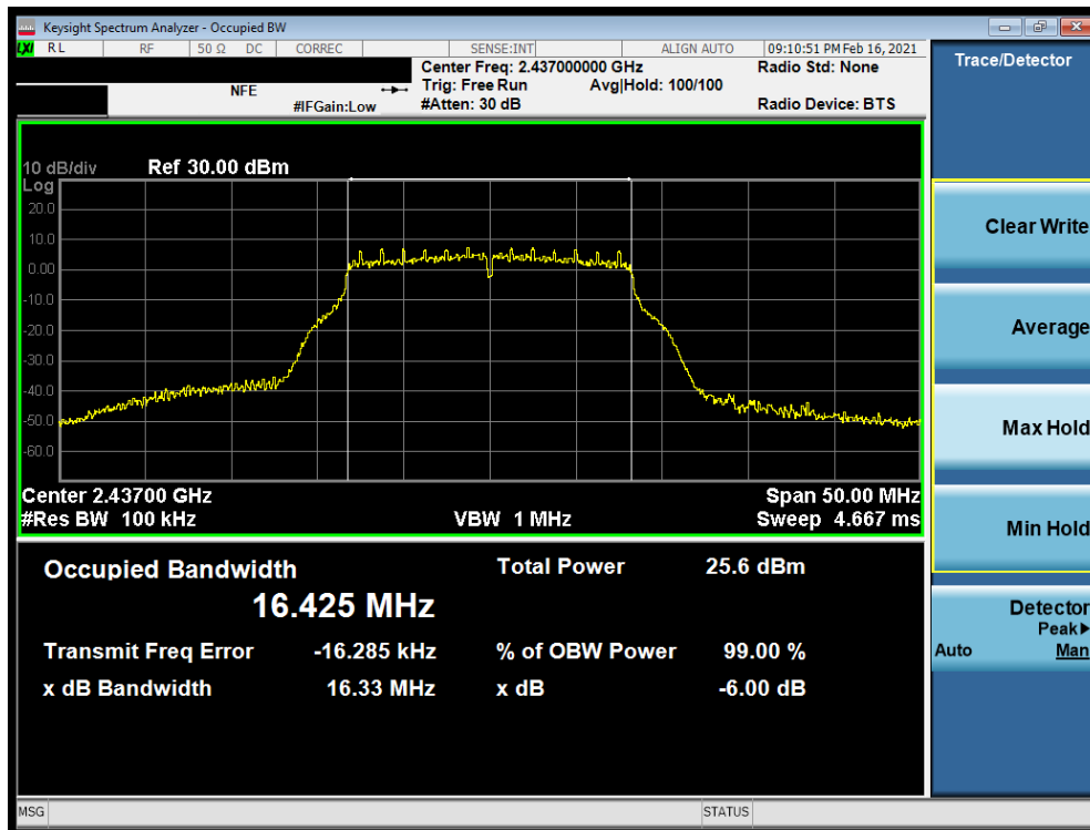
Plot 7-2: 6dB BW and 99% OBW Plot Antenna WF8 (802.11g – Ch. 6) – 6Mbps
