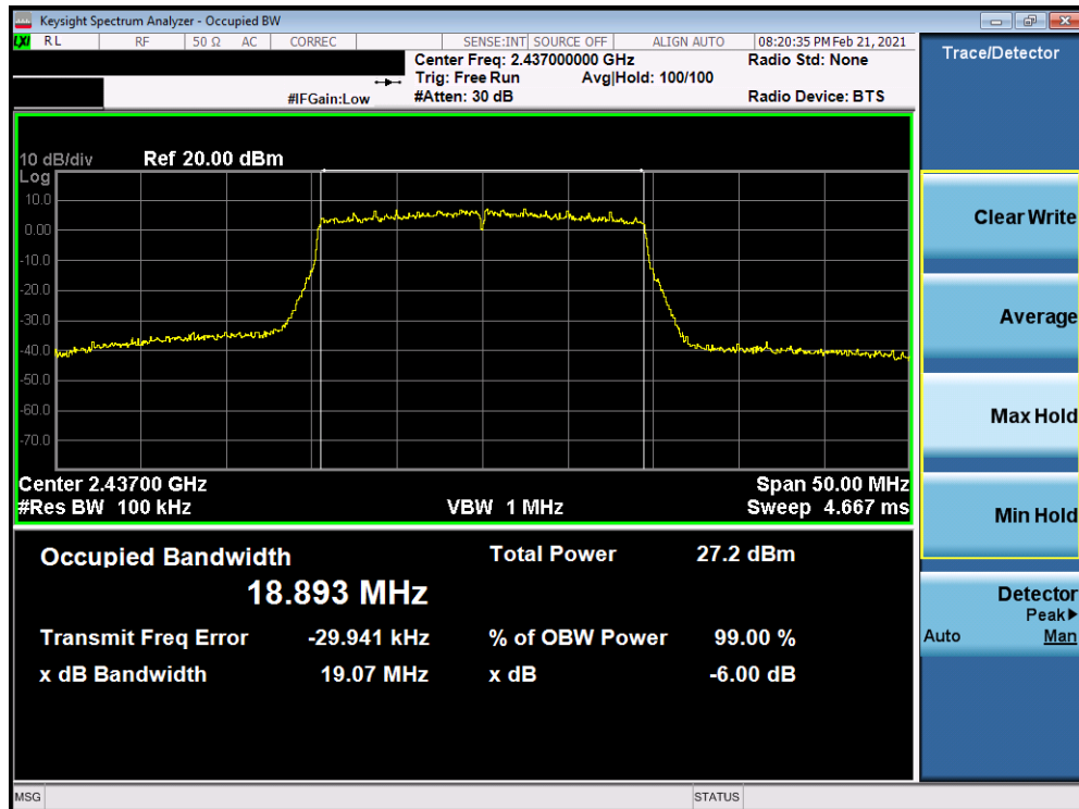
Plot 7-47. 6dB BW and 99% OBW Plot Antenna WF7 (802. 11ax (SU - 2.4GHz) – Ch. 6) – MCS3
