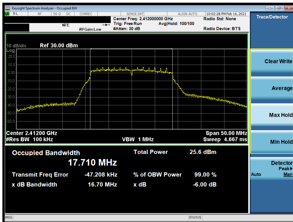
Plot 7-4. 6dB BW and 99% OBW Plot Antenna WF8 (802.11n (2.4GHz) – Ch. 1) – MCS0
