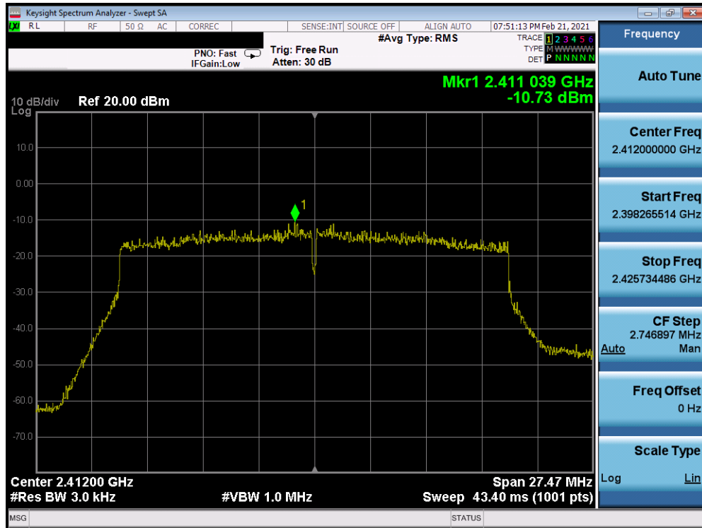
Plot 7-97. Power Spectral Density Plot Antenna WF7 (802.11ax (SU – 2.4GHz) – Ch. 1) – MCS0
