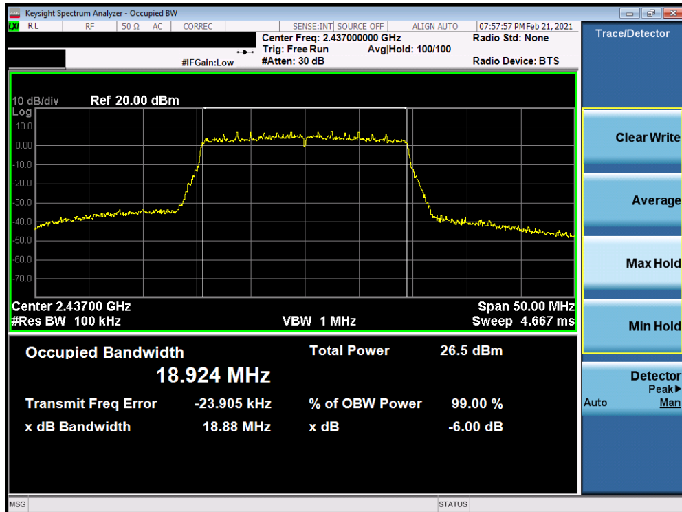
Plot 7-38. 6dB BW and 99% OBW Plot Antenna WF7 (802.11ax (SU - 2.4GHz) – Ch. 6) – MCS0
