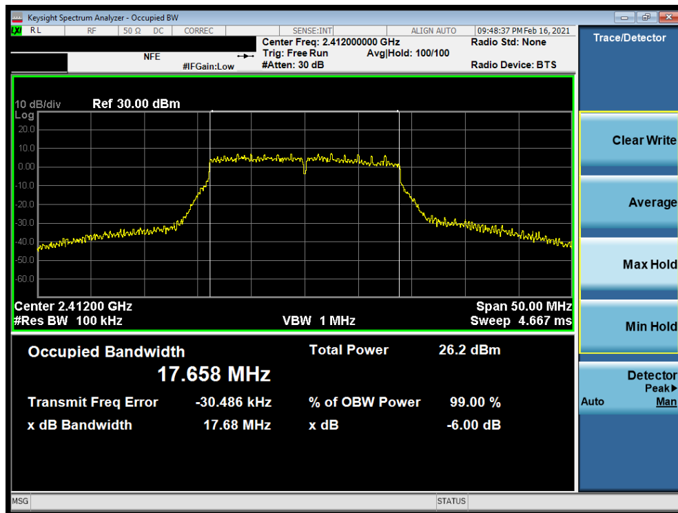
Plot 7-13. 6dB BW and 99% OBW Plot Antenna WF8 (802.11n (2.4GHz) – Ch. 1) – MCS3
