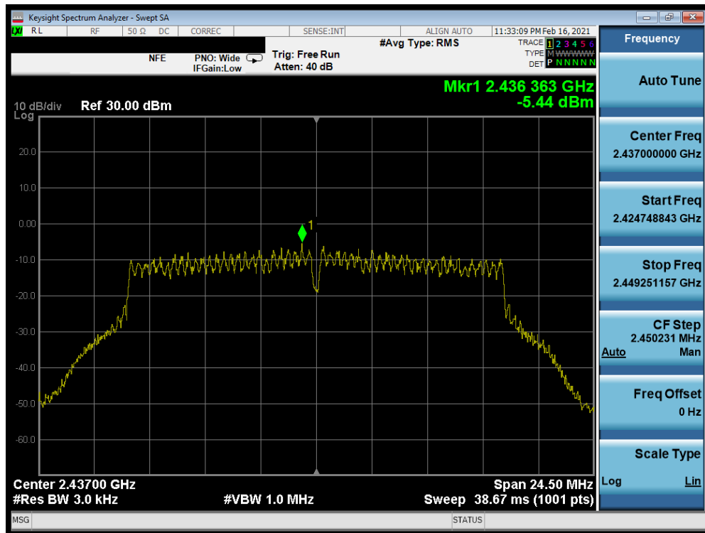
Plot 7-92. Power Spectral Density Plot Antenna WF7 (802.11g – Ch. 6) – 6Mbps
