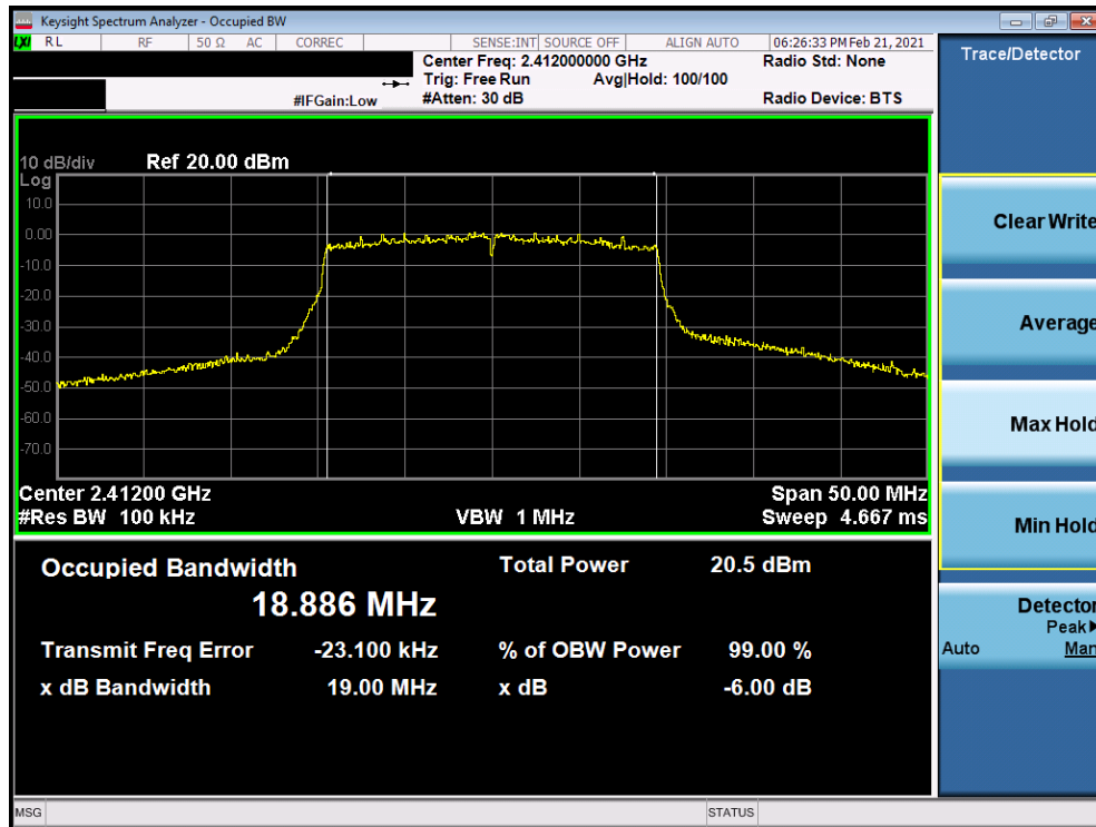
Plot 7-16. 6dB BW and 99% OBW Plot Antenna WF8 (802. 11ax (SU - 2.4GHz) – Ch. 1) – MCS3
