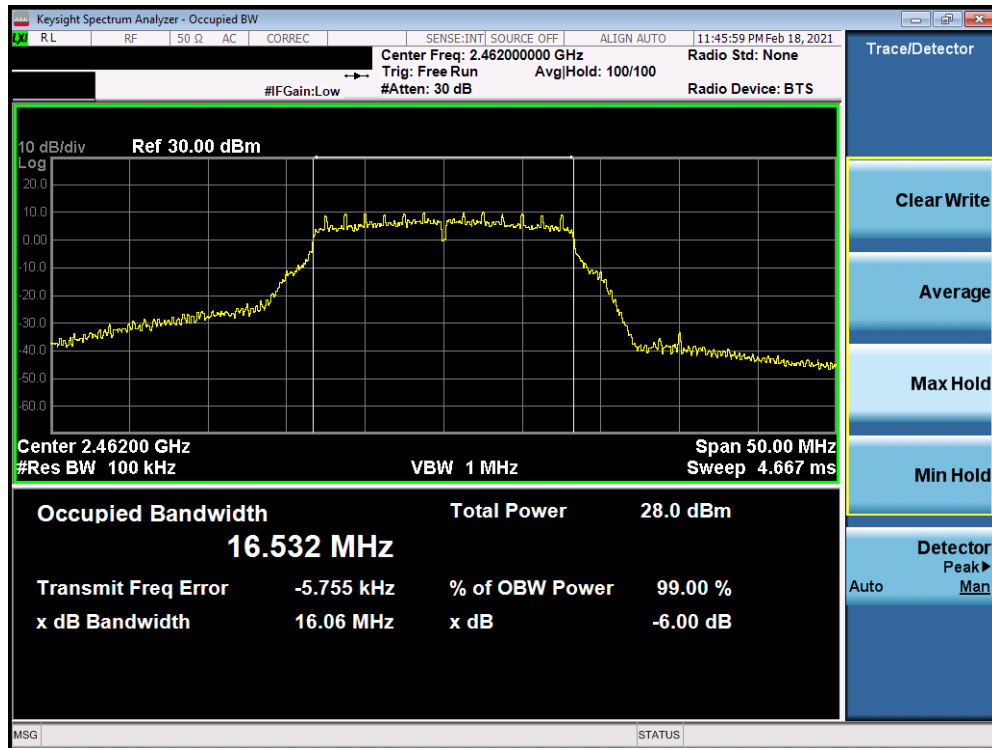
Plot 7-33. 6dB BW and 99% OBW Plot Antenna WF7 (802.11g – Ch. 11) – 6Mbps
