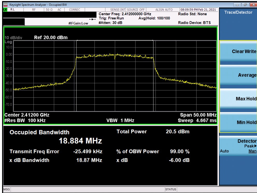
Plot 7-46. 6dB BW and 99% OBW Plot Antenna WF7 (802. 11ax (SU - 2.4GHz) – Ch. 1) – MCS3
