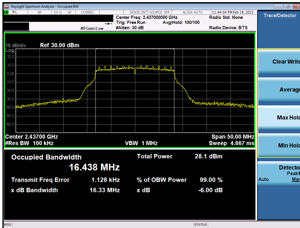
Plot 7-32. 6dB BW and 99% OBW Plot Antenna WF7 (802.11g – Ch. 6) – 6Mbps
