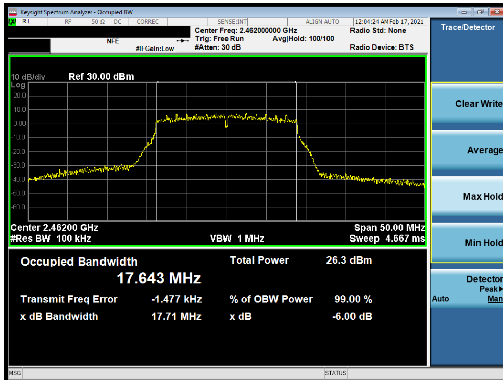
Plot 7-45. 6dB BW and 99% OBW Plot Antenna WF7 (802.11n (2.4GHz) – Ch. 11) – MCS3
