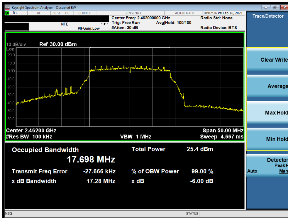
Plot 7-6. 6dB BW and 99% OBW Plot Antenna WF8 (802.11n (2.4GHz) – Ch. 11) – MCS0
