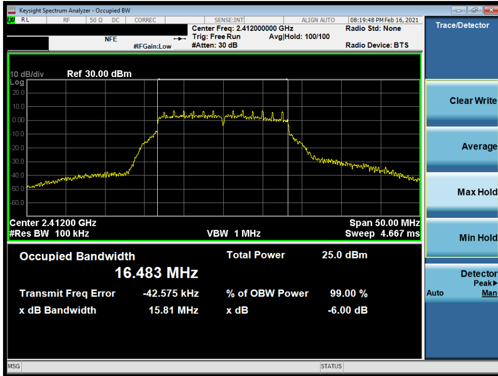
Plot 7-10. 6dB BW and 99% OBW Plot Antenna WF8 (802.11g – Ch. 1) – 18Mbps
