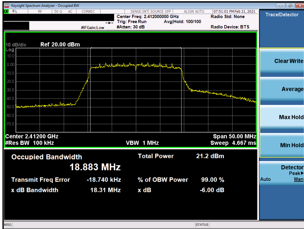
Plot 7-37. 6dB BW and 99% OBW Plot Antenna WF7 (802.11ax (SU - 2.4GHz) – Ch. 1) – MCS0
