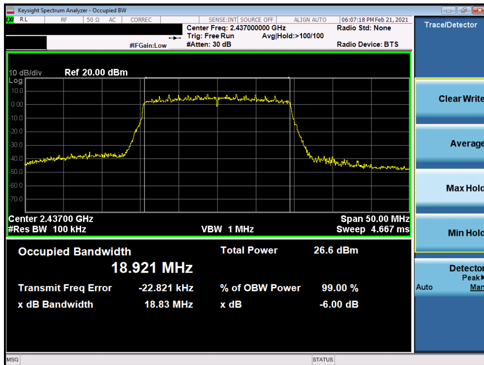
Plot 7-8. 6dB BW and 99% OBW Plot Antenna WF8 (802.11ax (SU - 2.4GHz) – Ch. 6) – MCS0
