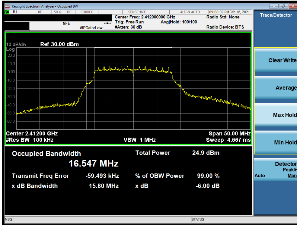
Plot 7-1: 6dB BW and 99% OBW Plot Antenna WF8 (802.11g – Ch. 1) – 6Mbps
