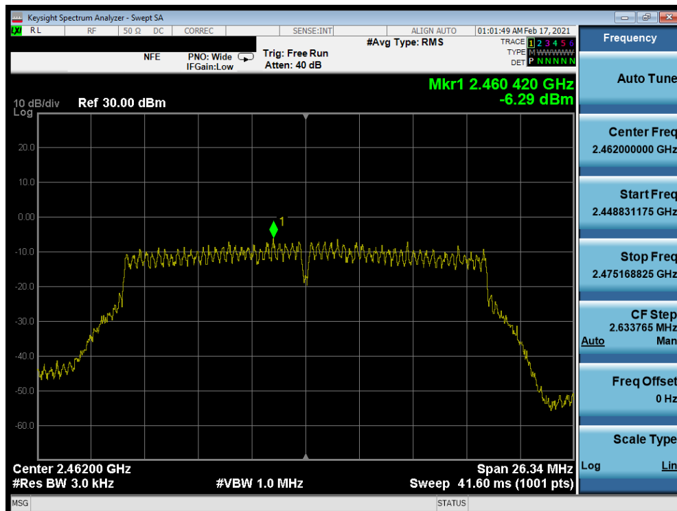
Plot 7-96. Power Spectral Density Plot Antenna WF7 (802.11n (2.4GHz) – Ch. 11) – MCS0
