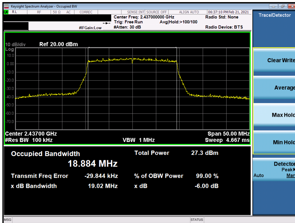
Plot 7-17. 6dB BW and 99% OBW Plot Antenna WF8 (802. 11ax (SU - 2.4GHz) – Ch. 6) – MCS3
