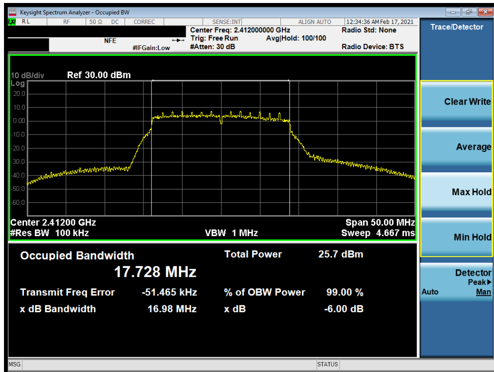
Plot 7-34. 6dB BW and 99% OBW Plot Antenna WF7 (802.11n (2.4GHz) – Ch. 1) – MCS0
