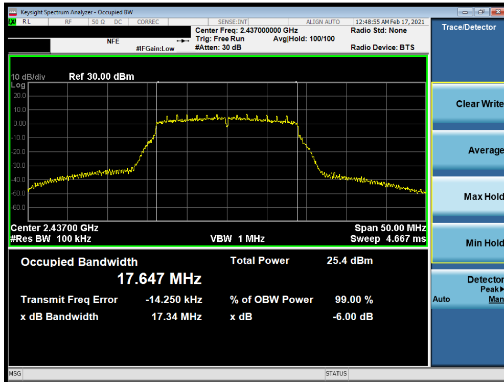
Plot 7-35. 6dB BW and 99% OBW Plot Antenna WF7 (802.11n (2.4GHz) – Ch. 6) – MCS0
