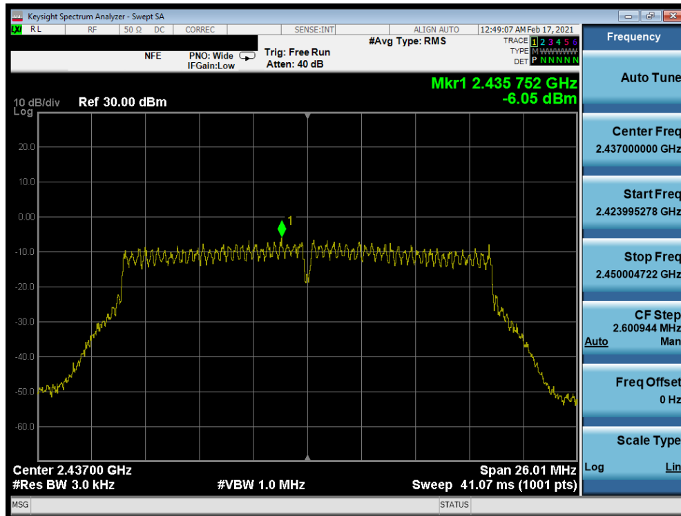
Plot 7-95. Power Spectral Density Plot Antenna WF7 (802.11n (2.4GHz) – Ch. 6) – MCS0
