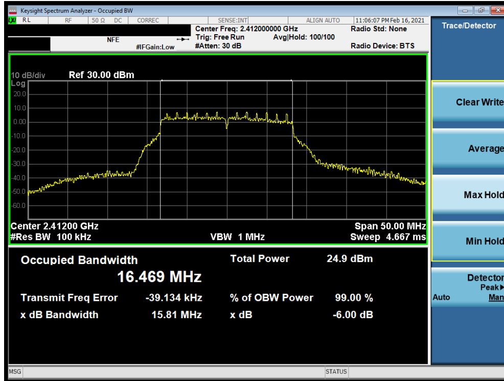
Plot 7-40. 6dB BW and 99% OBW Plot Antenna WF7 (802.11g – Ch. 1) – 18Mbps
