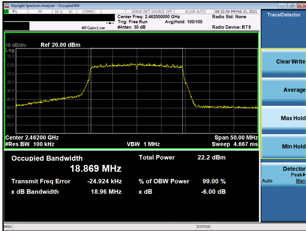
Plot 7-48. 6dB BW and 99% OBW Plot Antenna WF7 (802. 11ax (SU - 2.4GHz) – Ch. 11) – MCS3
