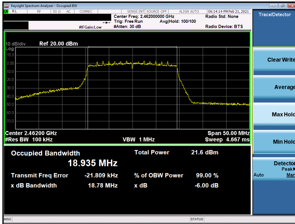
Plot 7-9. 6dB BW and 99% OBW Plot Antenna WF8 (802. 11ax (SU - 2.4GHz) – Ch. 11) – MCS0
