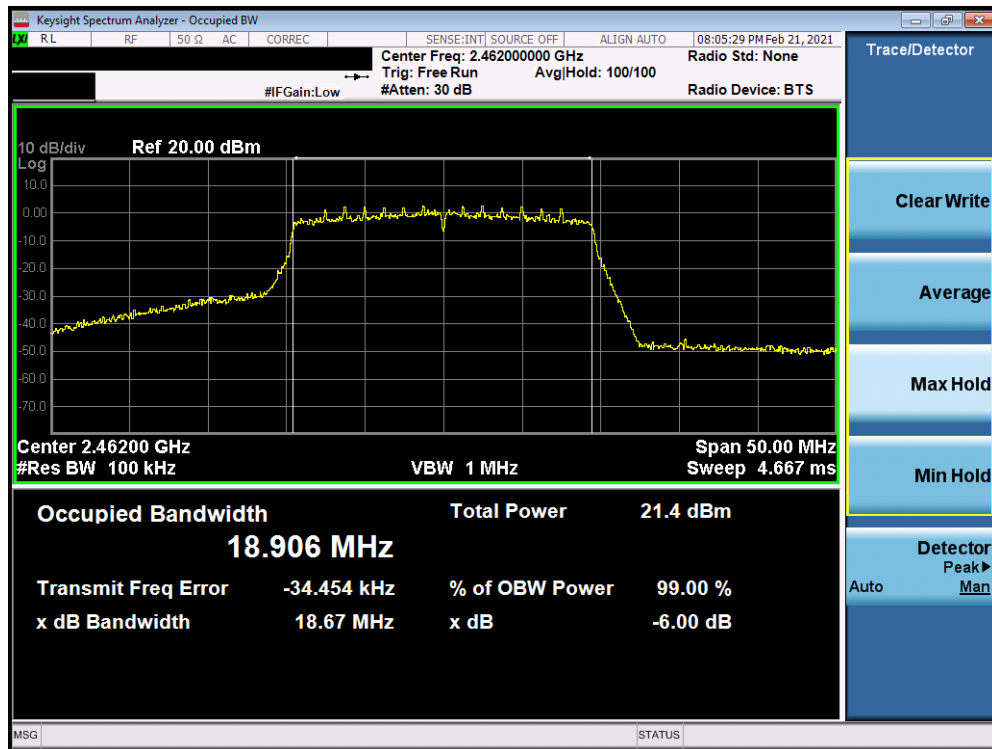
Plot 7-39. 6dB BW and 99% OBW Plot Antenna WF7 (802. 11ax (SU - 2.4GHz) – Ch. 11) – MCS0
