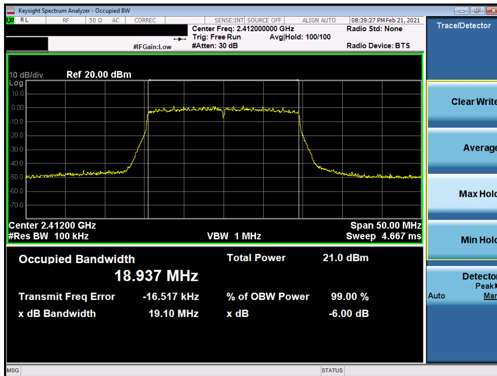
Plot 7-58. 6dB BW and 99% OBW Plot Antenna WF7 (802.11ax (SU - 2.4GHz) – Ch. 1) – MCS5
