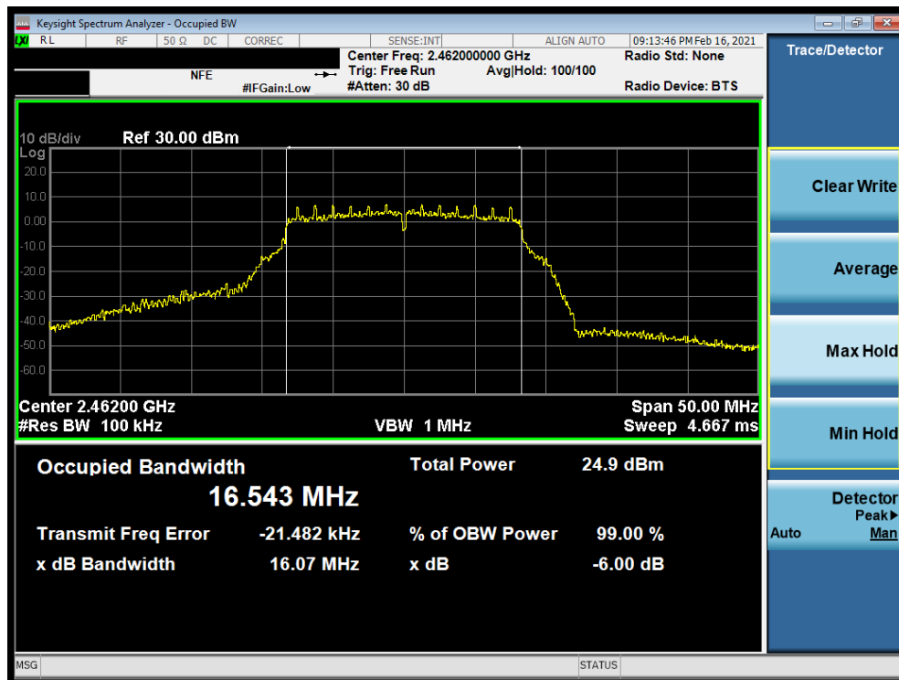
Plot 7-3. 6dB BW and 99% OBW Plot Antenna WF8 (802.11g – Ch. 11) – 6Mbps
