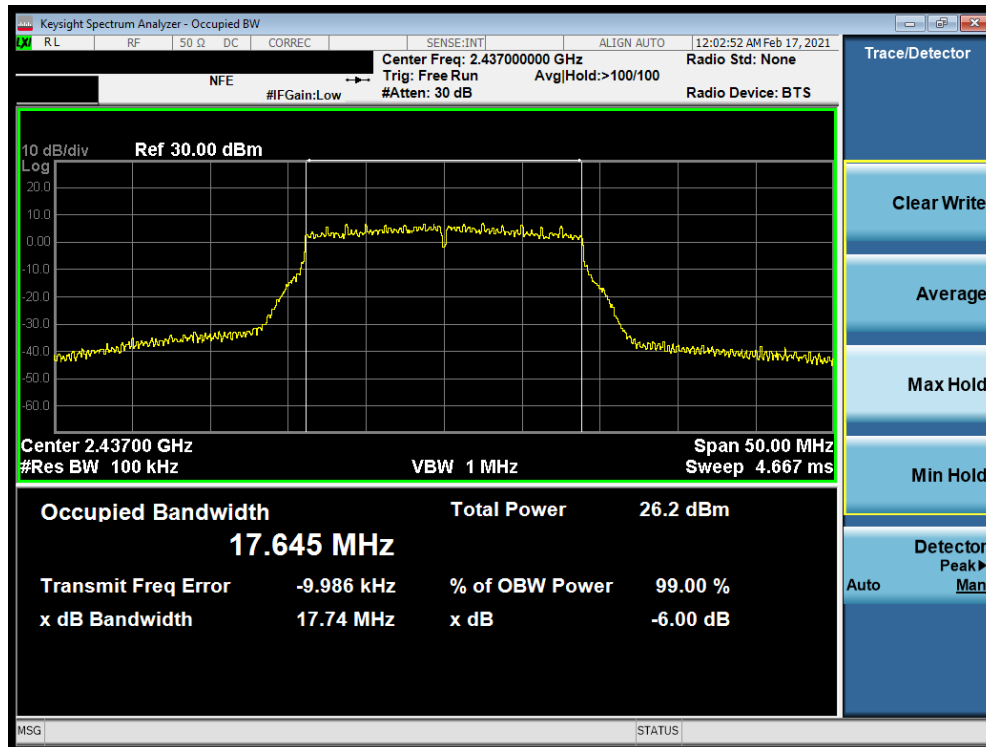
Plot 7-44. 6dB BW and 99% OBW Plot Antenna WF7 (802.11n (2.4GHz) – Ch. 6) – MCS3
