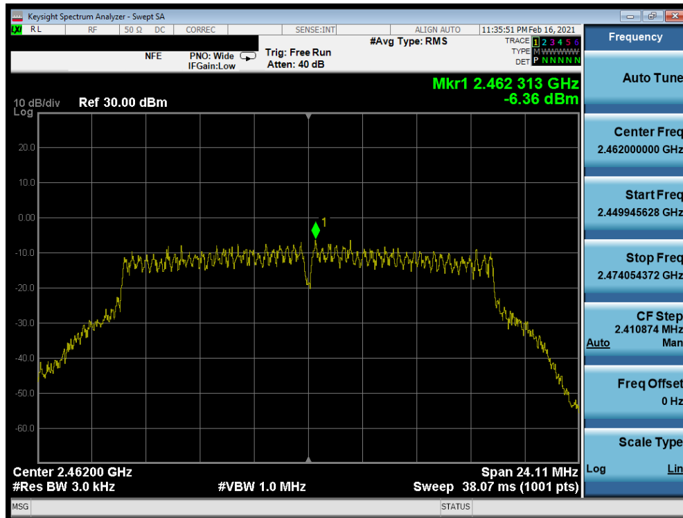
Plot 7-93. Power Spectral Density Plot Antenna WF7 (802.11g – Ch. 11) – 6Mbps
