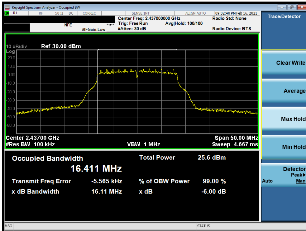
Plot 7-11. 6dB BW and 99% OBW Plot Antenna WF8 (802.11g – Ch. 6) – 18Mbps
