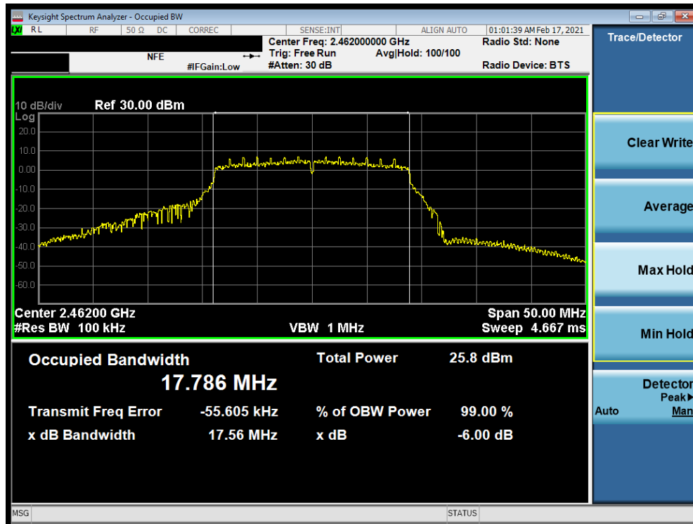
Plot 7-36. 6dB BW and 99% OBW Plot Antenna WF7 (802.11n (2.4GHz) – Ch. 11) – MCS0
