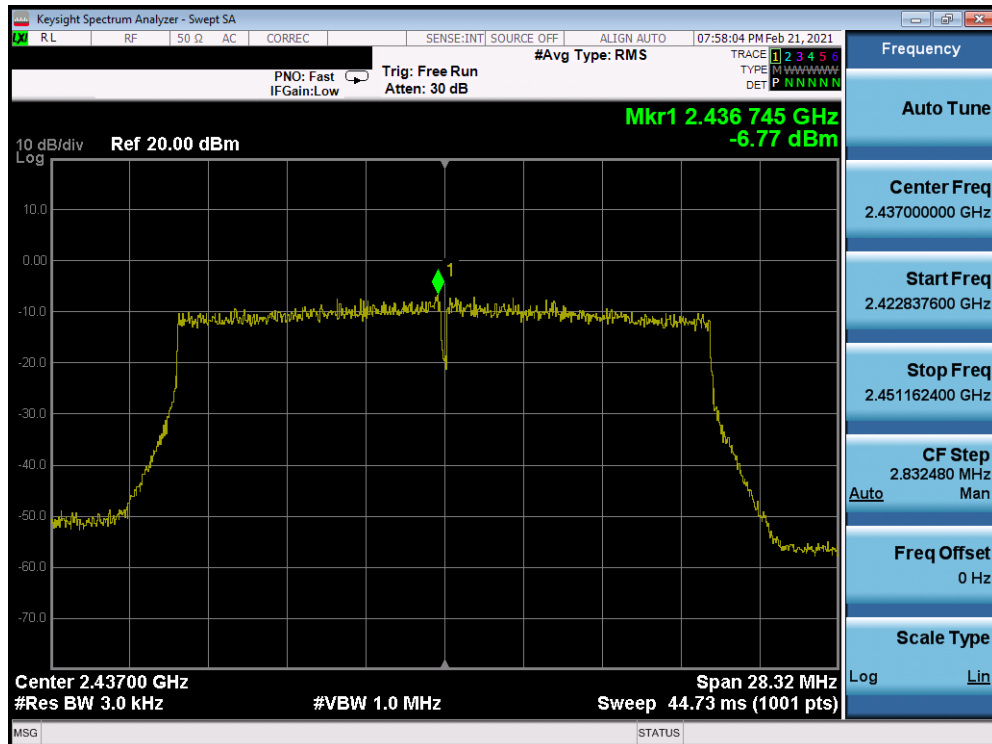
Plot 7-98. Power Spectral Density Plot Antenna WF7 (802.11ax (SU – 2.4GHz) – Ch. 6) – MCS0
