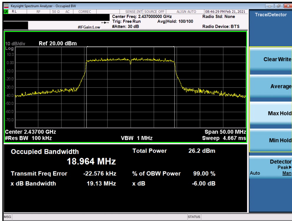
Plot 7-59. 6dB BW and 99% OBW Plot Antenna WF7 (802. 11ax (SU - 2.4GHz) – Ch. 6) – MCS5
