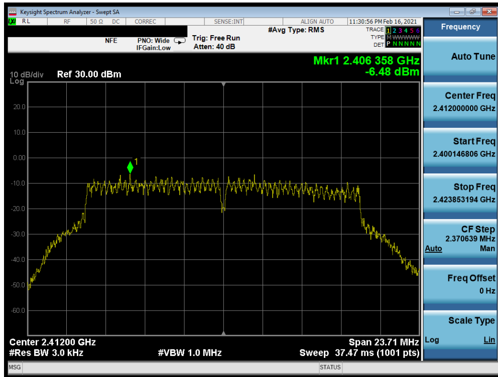
Plot 7-91. Power Spectral Density Plot Antenna WF7 (802.11g – Ch. 1) – 6Mbps
