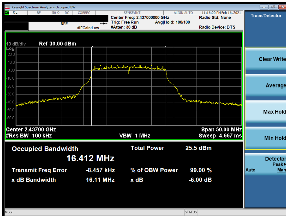
Plot 7-41. 6dB BW and 99% OBW Plot Antenna WF7 (802.11g – Ch. 6) – 18Mbps
