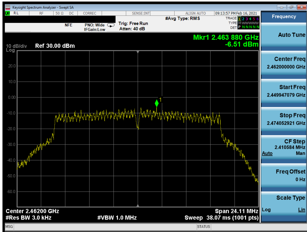
Plot 7-63. Power Spectral Density Plot Antenna WF8 (802.11g – Ch. 11) – 6Mbps
