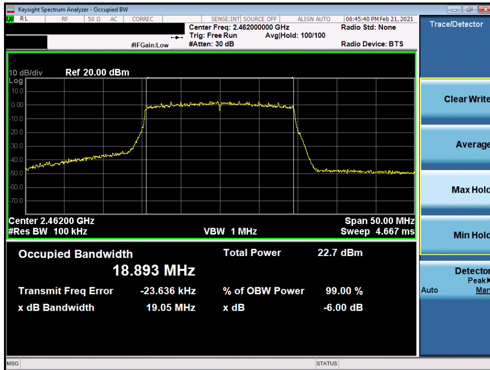
Plot 7-18. 6dB BW and 99% OBW Plot Antenna WF8 (802. 11ax (SU - 2.4GHz) – Ch. 11) – MCS3
