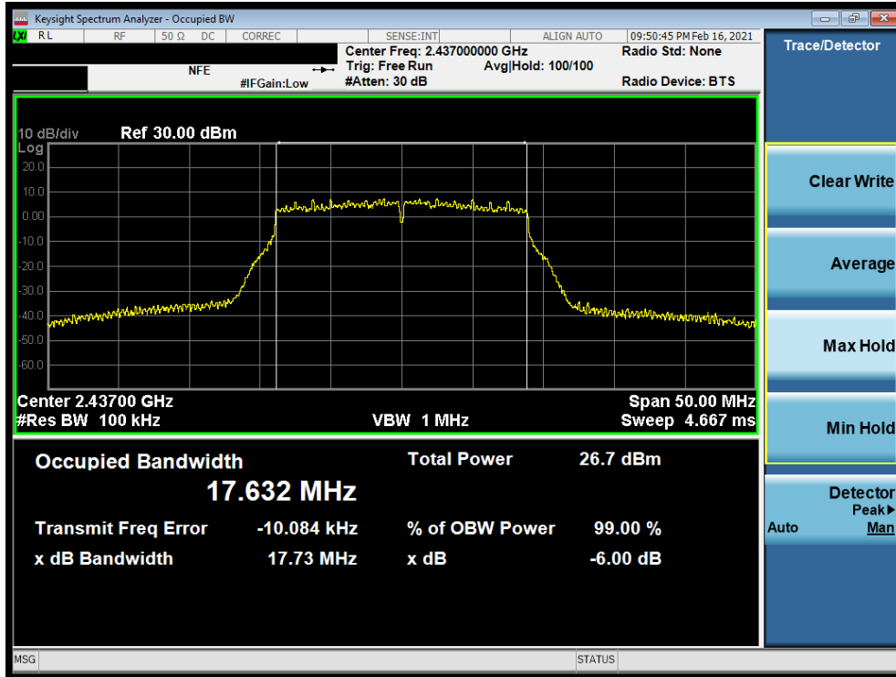
Plot 7-14. 6dB BW and 99% OBW Plot Antenna WF8 (802.11n (2.4GHz) – Ch. 6) – MCS3
