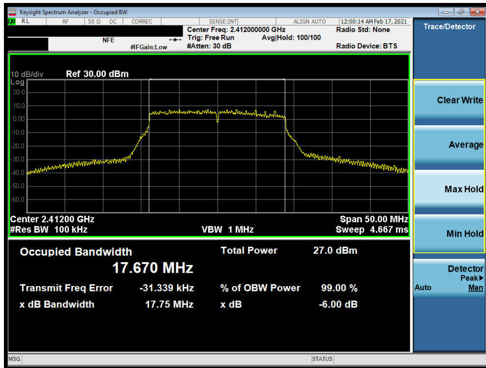
Plot 7-43. 6dB BW and 99% OBW Plot Antenna WF7 (802.11n (2.4GHz) – Ch. 1) – MCS3
