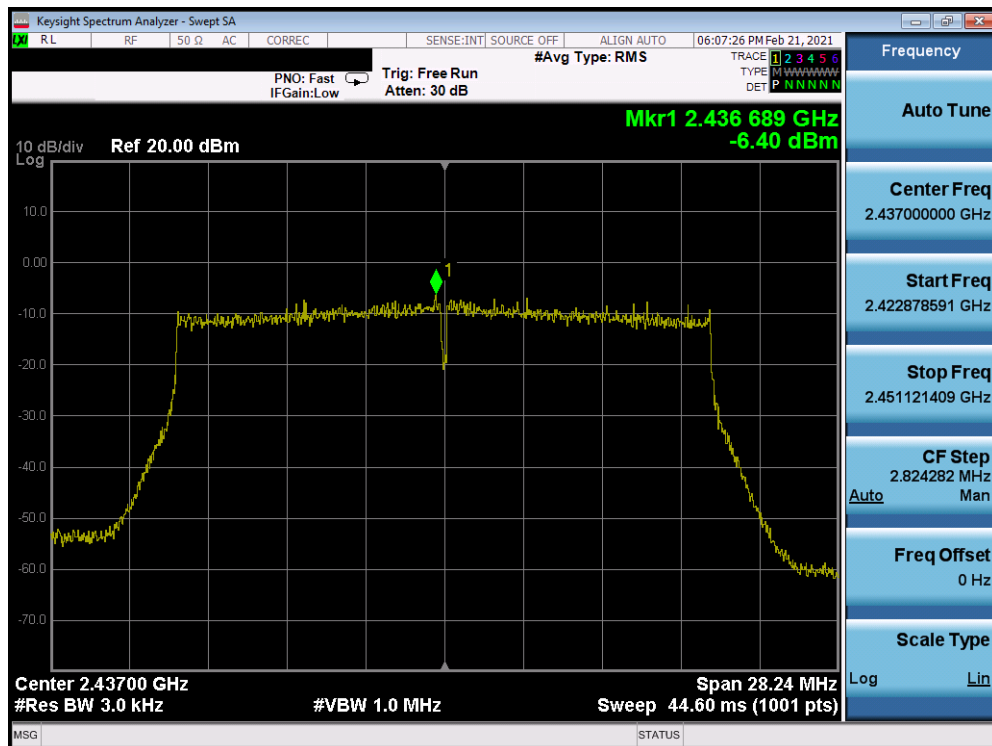
Plot 7-68. Power Spectral Density Plot Antenna WF8 (802.11ax (SU – 2.4GHz) – Ch. 6) – MCS0
