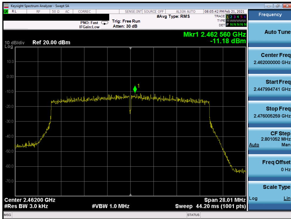
Plot 7-99. Power Spectral Density Plot Antenna WF7 (802.11ax (SU – 2.4GHz) – Ch. 11) – MCS0
