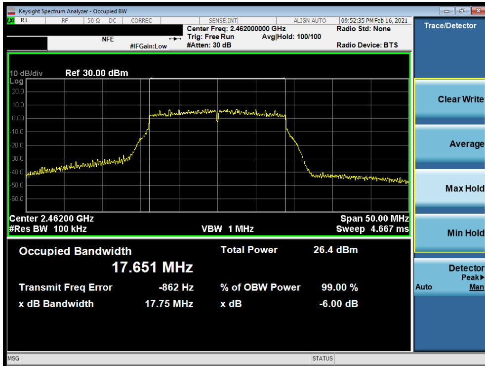
Plot 7-15. 6dB BW and 99% OBW Plot Antenna WF8 (802.11n (2.4GHz) – Ch. 11) – MCS3
