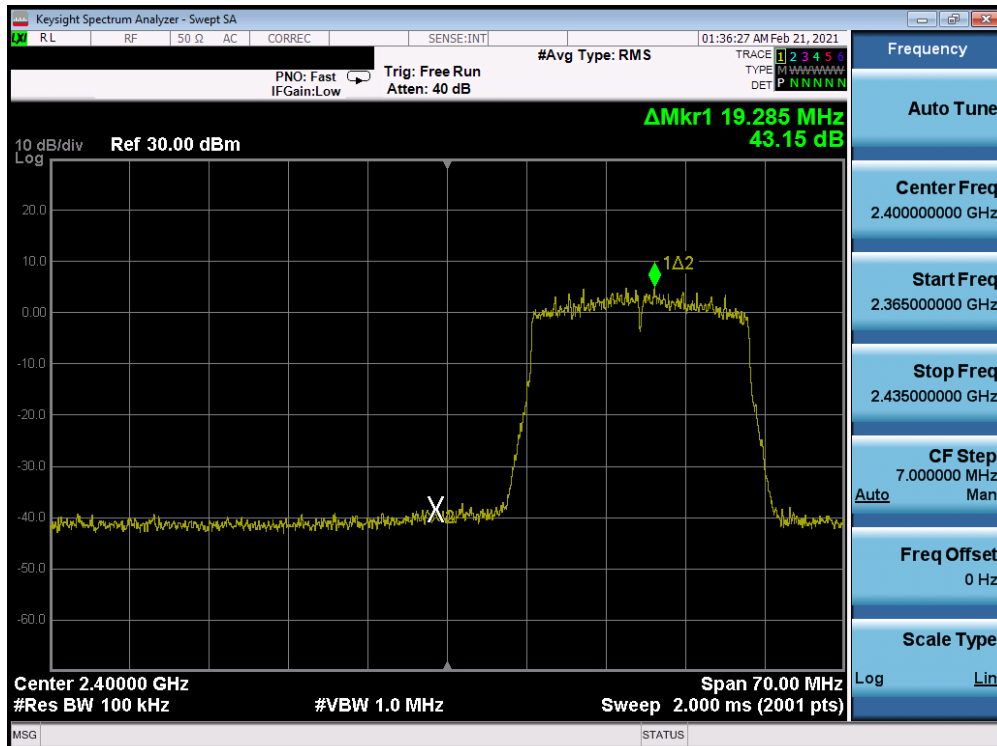
Plot 7-82. Band Edge Antenna WF8 (802.11ax OFDMA - RU242 - Ch. 2)
