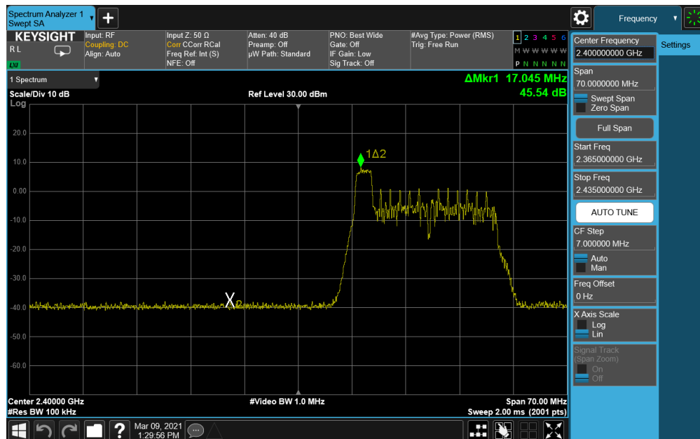
Plot 7-74. Band Edge Antenna WF8 (802.11ax OFDMA – RU26 Index 0 – Ch. 2)
