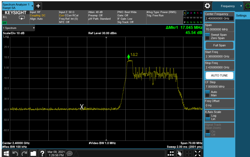
Plot 7-91. Band Edge Antenna WF7 (802.11ax OFDMA – RU26 Index 0 – Ch. 2)
