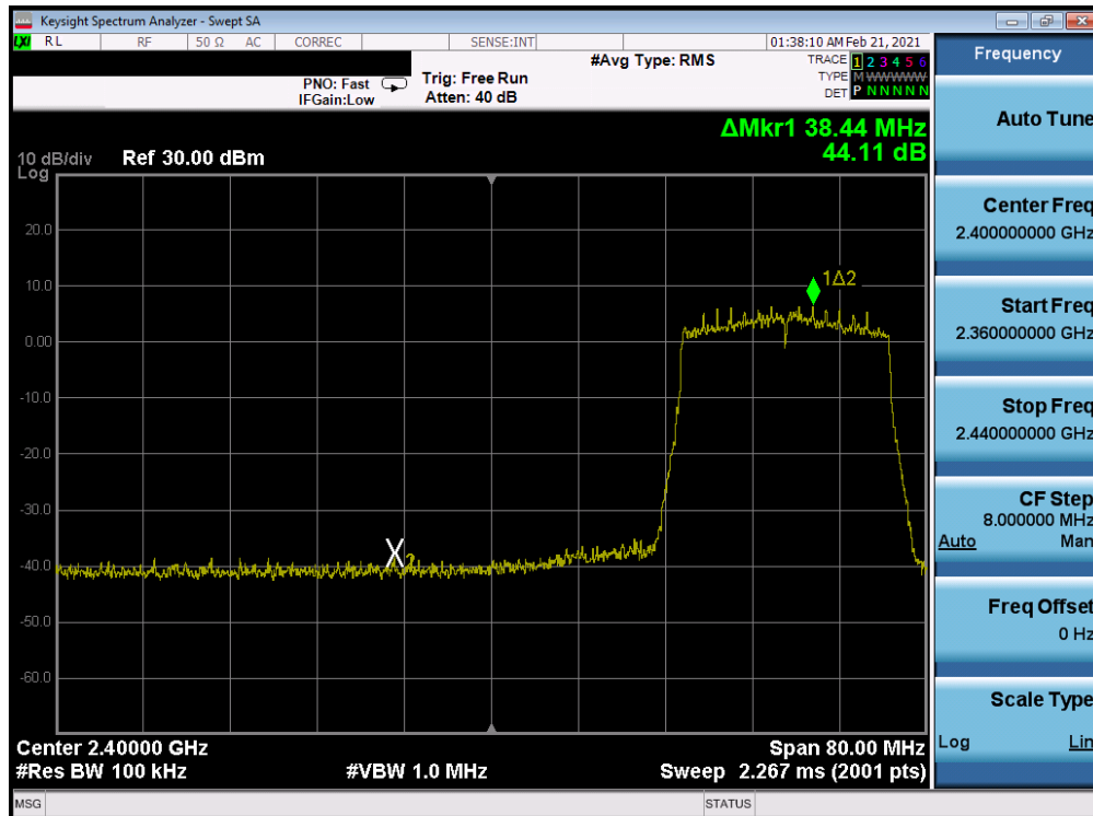
Plot 7-84. Band Edge Antenna WF8 (802.11ax OFDMA – RU242 – Ch. 4)
