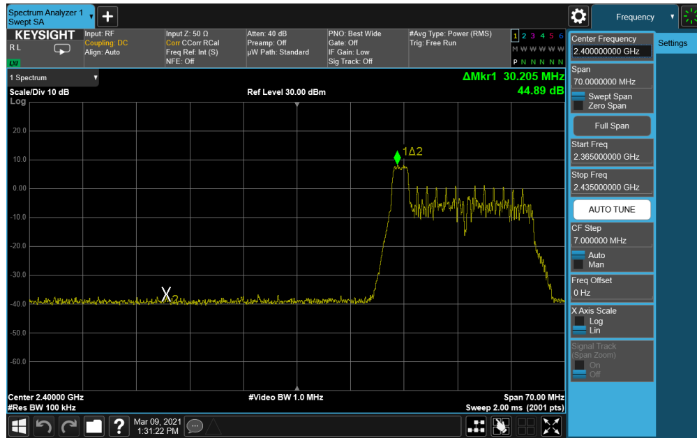
Plot 7-75. Band Edge Antenna WF8 (802.11ax OFDMA – RU26 Index 0 – Ch. 3)
