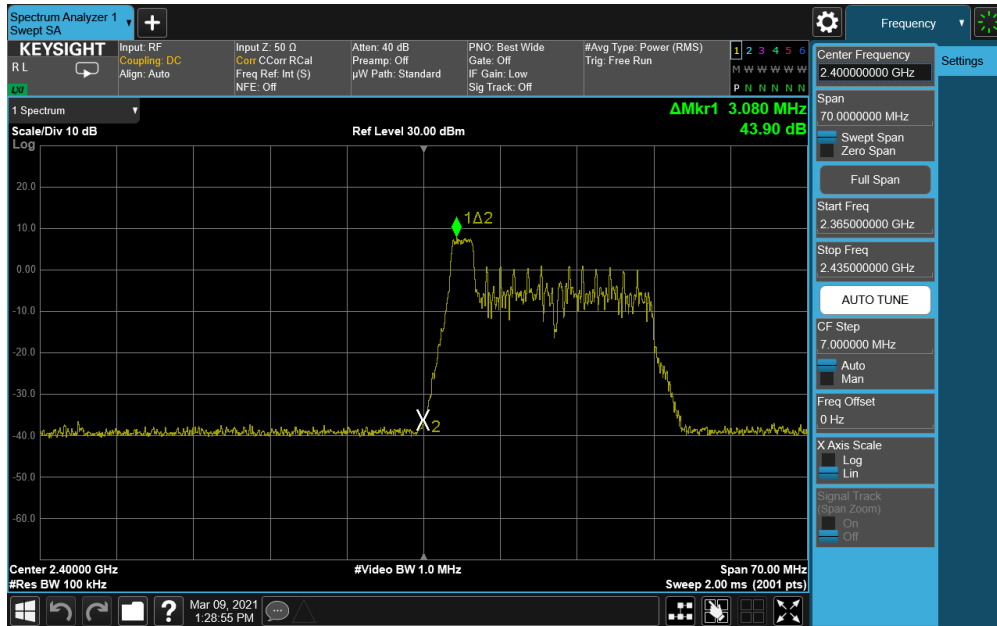
Plot 7-90. Band Edge Antenna WF7 (802.11ax OFDMA – RU26 Index 0 – Ch. 1)
