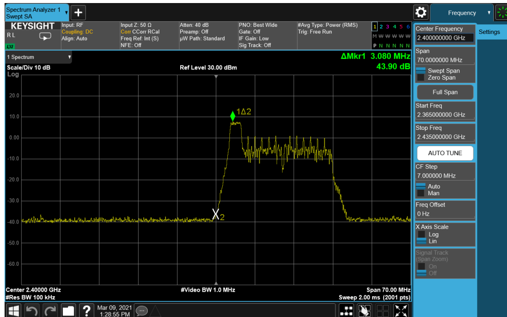
Plot 7-73. Band Edge Antenna WF8 (802.11ax OFDMA – RU26 Index 0 – Ch. 1)
