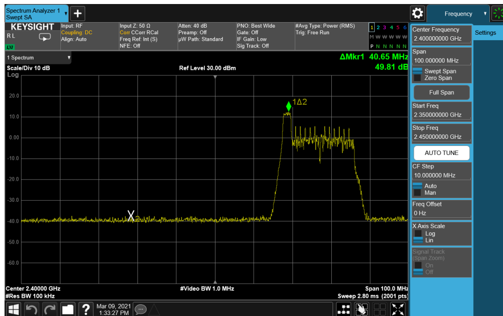
Plot 7-76. Band Edge Antenna WF8 (802.11ax OFDMA – RU26 Index 0 – Ch. 4)
