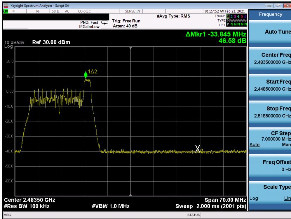
Plot 7-79. Band Edge Antenna WF8 (802.11ax OFDMA – RU26 Index 8 – Ch. 11)
