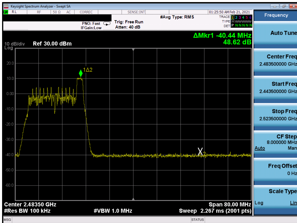
Plot 7-78. Band Edge Antenna WF8 (802.11ax OFDMA – RU26 Index 8 – Ch. 10)
