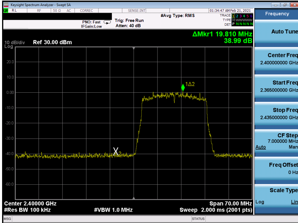
Plot 7-81. Band Edge Antenna WF8 (802.11ax OFDMA - RU242 - Ch. 1)
