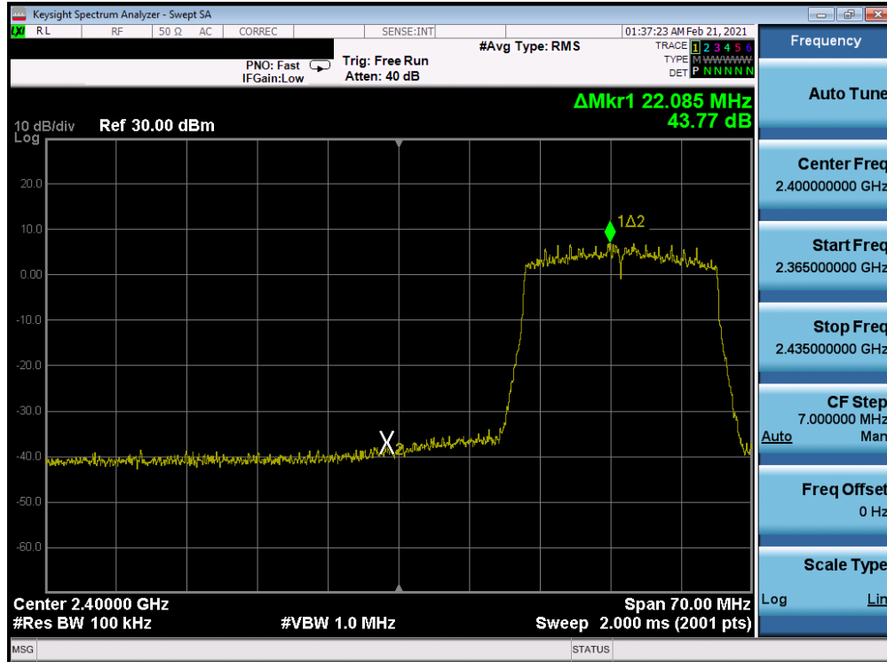
Plot 7-83. Band Edge Antenna WF8 (802.11ax OFDMA – RU242 – Ch. 3)
