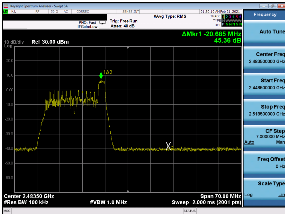
Plot 7-80. Band Edge Antenna WF8 (802.11ax OFDMA – RU26 Index 8 – Ch. 12)
