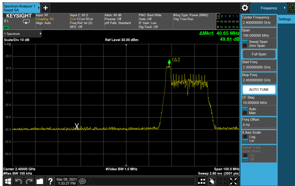
Plot 7-93. Band Edge Antenna WF7 (802.11ax OFDMA – RU26 Index 0 – Ch. 4)
