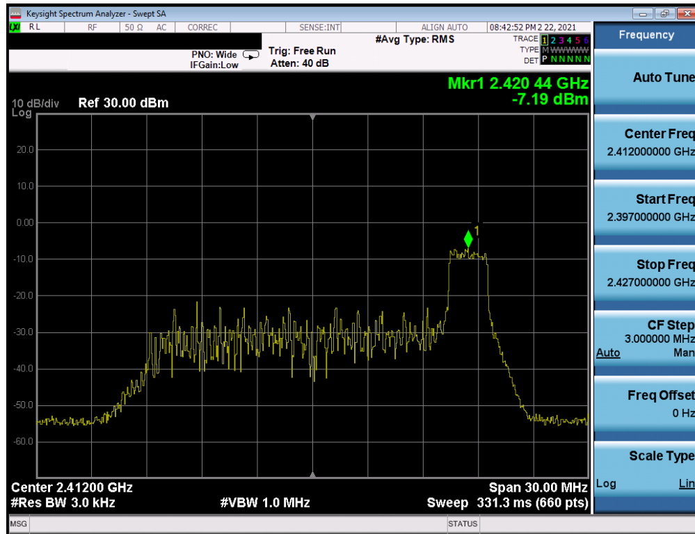
Plot 7-53. Power Spectral Density Plot CDD Antenna WF8 (802.11ax OFDMA – RU26 Index 8 – Ch. 1)
