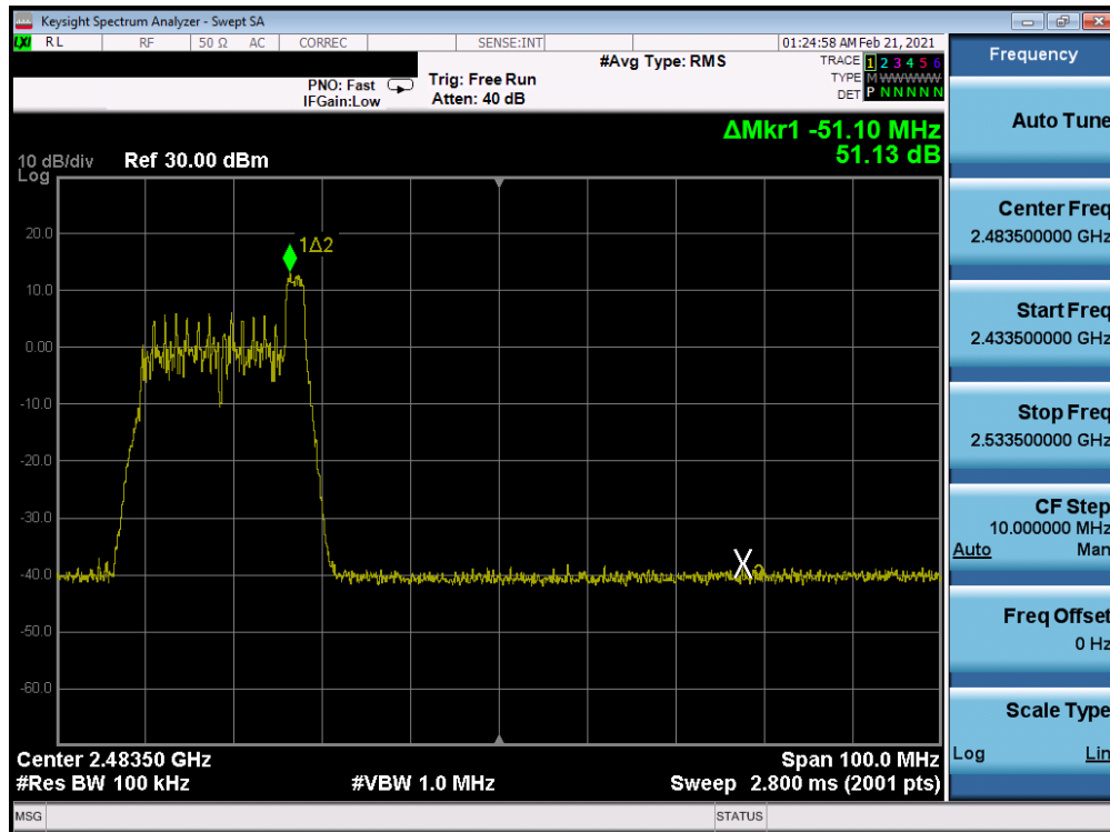
Plot 7-94. Band Edge Antenna WF7 (802.11ax OFDMA – RU26 Index 8 – Ch. 9)
