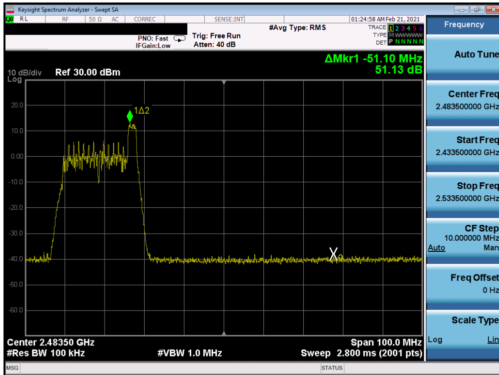
Plot 7-77. Band Edge Antenna WF8 (802.11ax OFDMA – RU26 Index 8 – Ch. 9)
