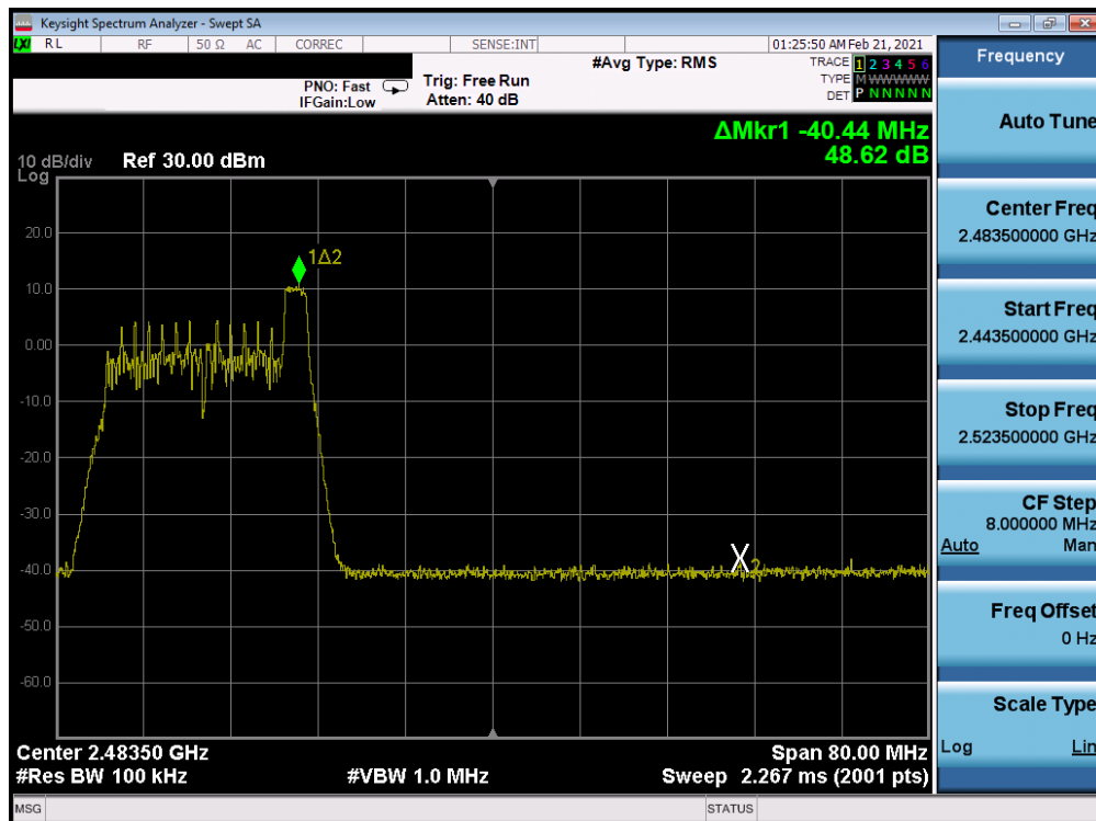
Plot 7-95. Band Edge Antenna WF7 (802.11ax OFDMA – RU26 Index 8 – Ch. 10)
