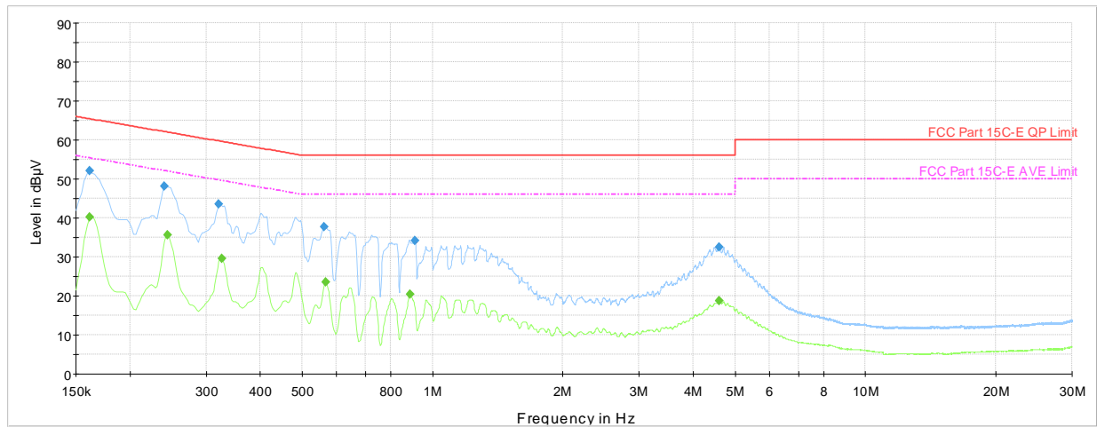
Plot 7-106. AC Line Conducted Plot with Bluetooth HDR Tx BF (N, 4Mbps ePA - Ch.38 with Laptop)
