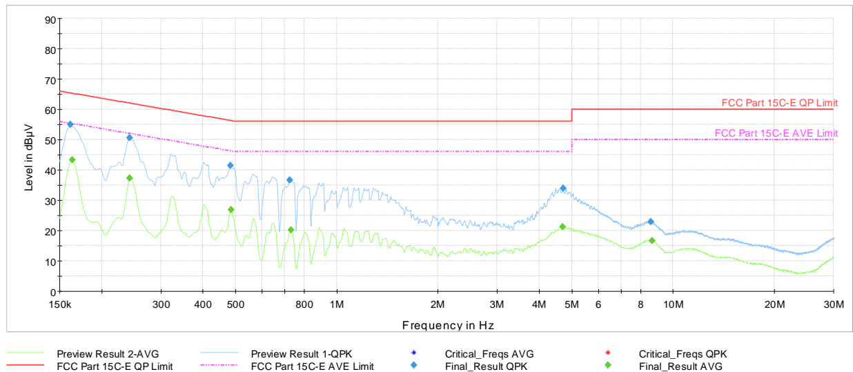
Plot 7-105. AC Line Conducted Plot with Bluetooth HDR TxBF (L1, 4Mbps ePA - Ch.38 with Laptop)
