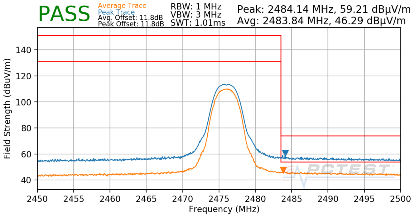
Plot 7-98. Radiated Restricted Upper Band Edge Measurement Antenna WF7 (Average & Peak)
