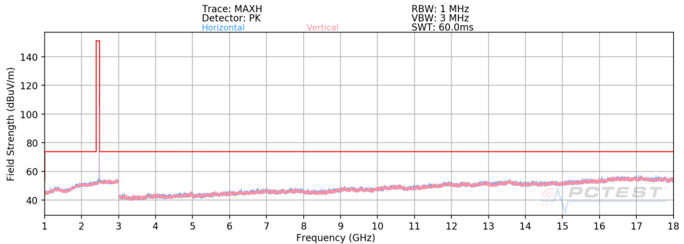
Plot 7-83. Radiated Spurious Emissions Above 1GHz Antenna WF8 (4Mbps, HDR4, ePA – Ch. 73)
