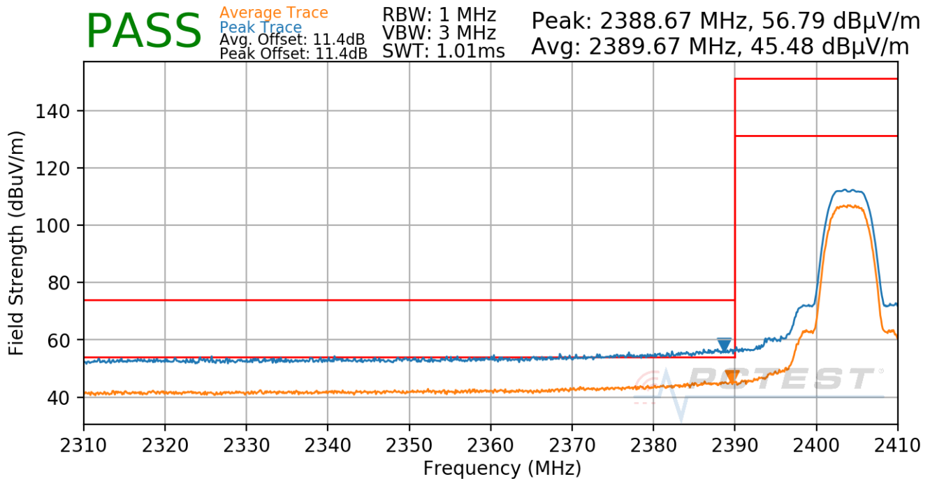
Plot 7-97. Radiated Restricted Lower Band Edge Measurement Antenna WF7 (Average & Peak)
