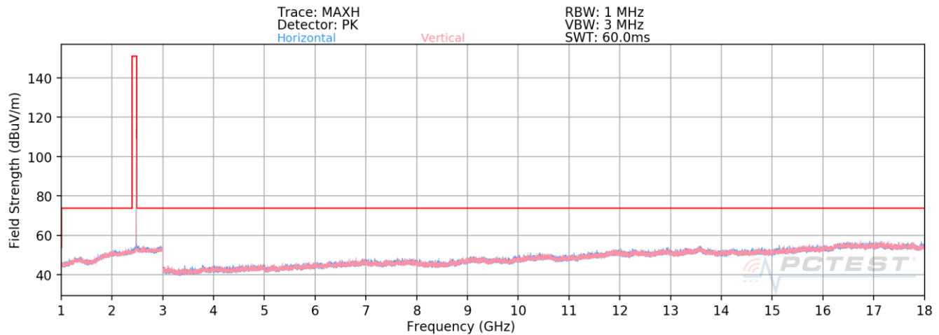
Plot 7-86. Radiated Spurious Emissions Above 1GHz Antenna WF7 (4Mbps, HDR4, ePA – Ch. 73)
