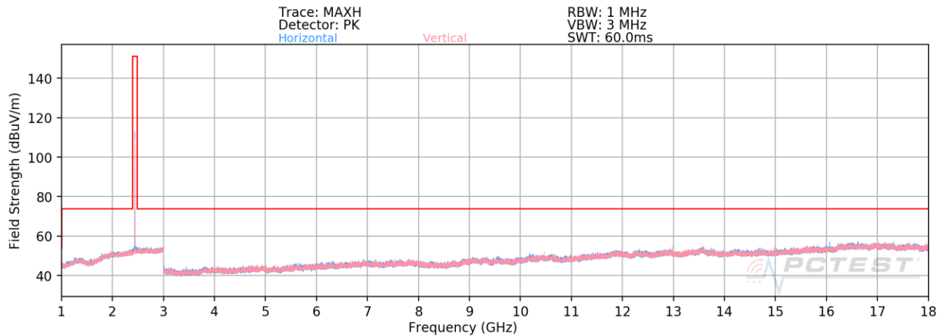
Plot 7-85. Radiated Spurious Emissions Above 1GHz Antenna WF7 (4Mbps, HDR4, ePA – Ch. 38)
