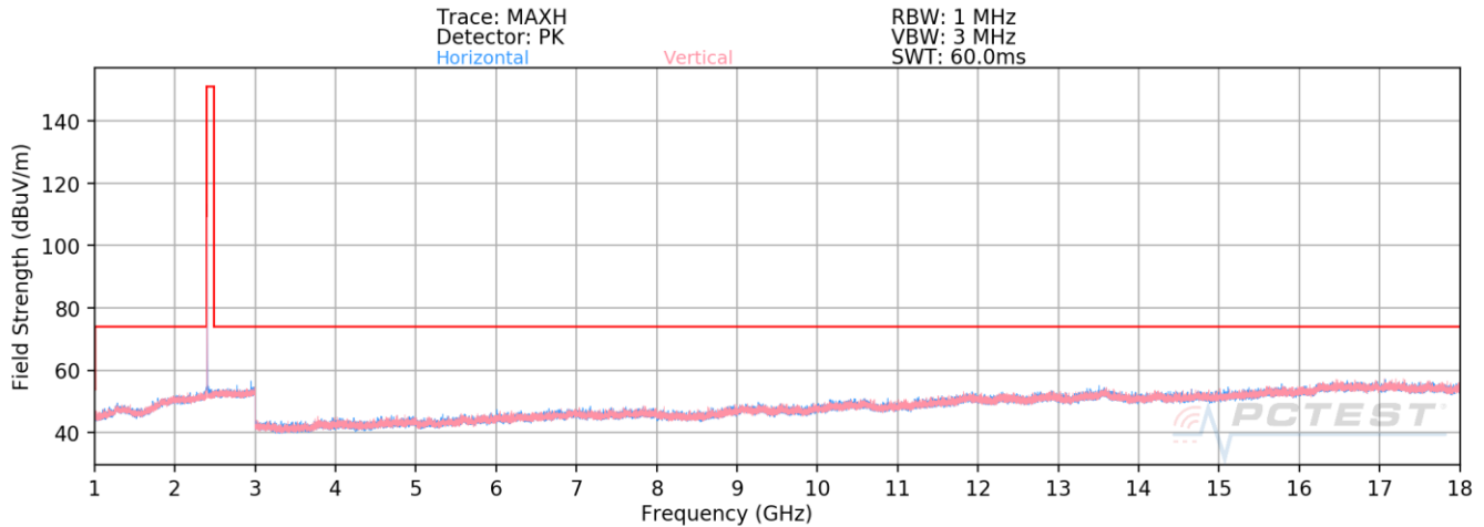
Plot 7-84. Radiated Spurious Emissions Above 1GHz Antenna WF7 (4Mbps, HDR4, ePA – Ch. 1)
