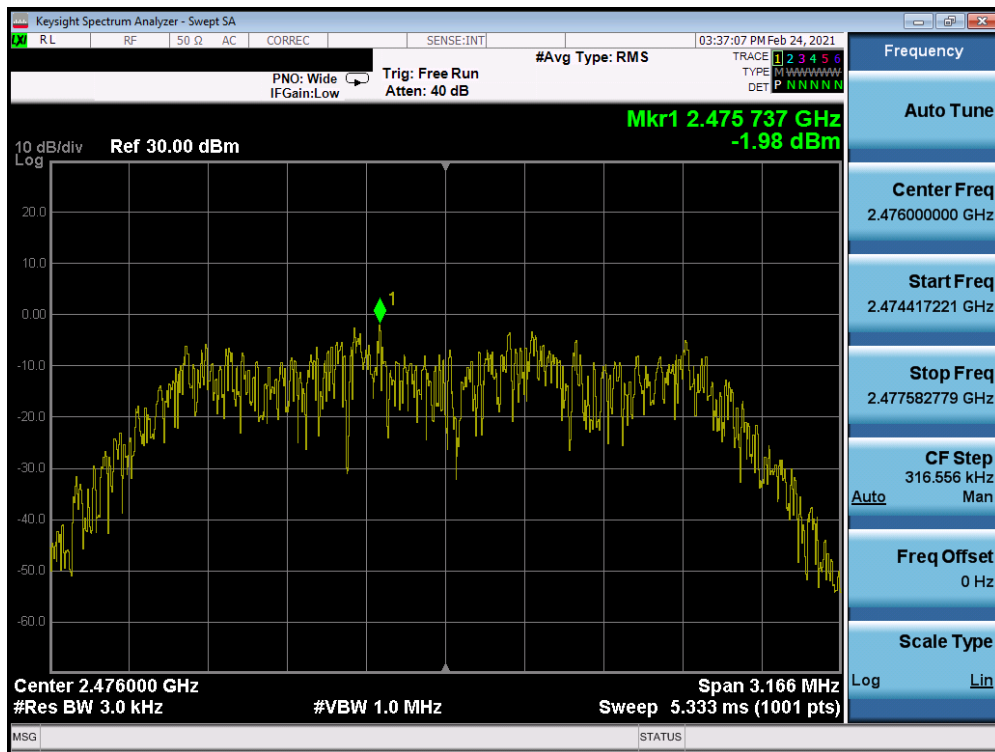
Plot 7-42. Power Spectral Density Plot TxBF Antenna WF7 (Bluetooth (HDR4), 4Mbps, ePA – Ch. 73)
