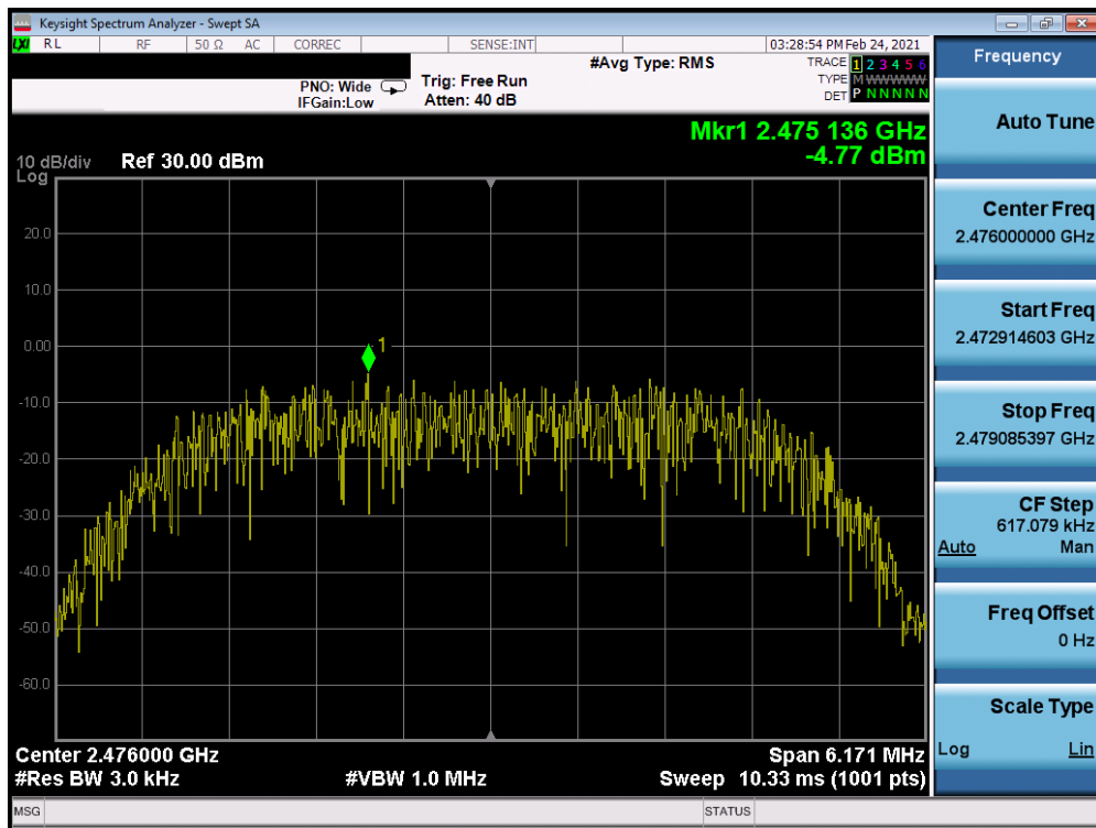
Plot 7-54. Power Spectral Density Plot TxBF Antenna WF7 (Bluetooth (HDR8), 8Mbps, ePA – Ch. 73)
