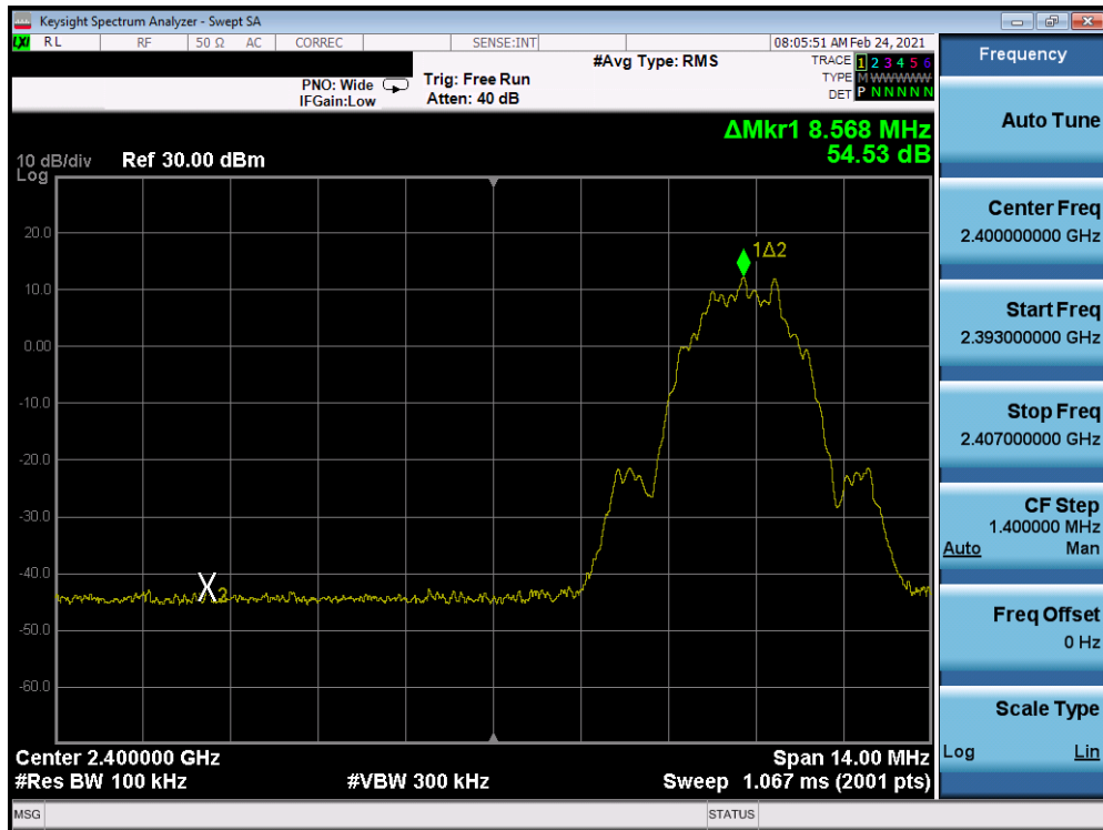
Plot 7-67. Band Edge Plot Antenna WF7 (Bluetooth (LE), 2Mbps, ePA – Ch. 1)
