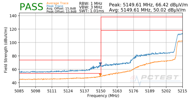
Plot 7-872. Antenna 5B (Pk & Avg, Ch.46, 80.11ax(SU), MCS0)
