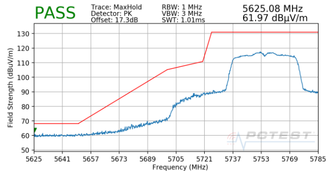
Plot 7-863. Antenna 5B (Pk, Ch.151, 802.11n, MCS0)
