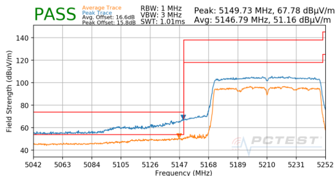
Plot 7-907. Antenna 5B (Pk & Avg, Ch.42, 802.11ac, MCS5)
