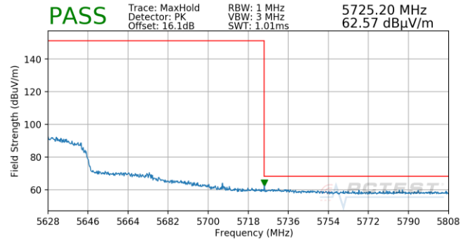
Plot 7-890. (FCC Only) Antenna 5B (Pk, Ch.118, 80.11ax(SU), MCS0)
