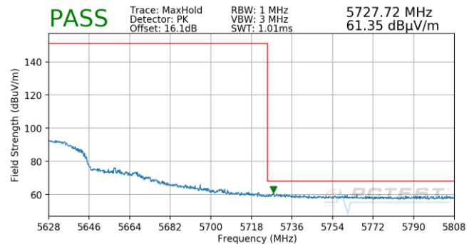
Plot 7-891. (FCC Only) Antenna 5B (Pk, Ch.118, 80.11ax(SU), MCS3)
