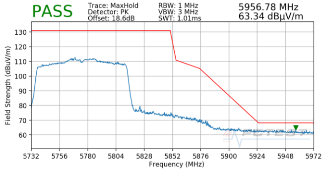
Plot 7-923. Antenna 5B (Pk, Ch.155, 802.11ac, MCS0)
