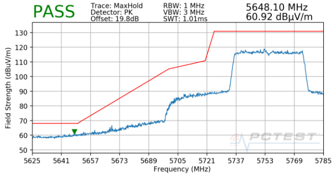
Plot 7-899. Antenna 5B (Pk, Ch.151, 80.11ax(SU), MCS0)
