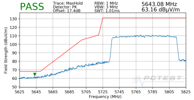
Plot 7-941. Antenna 5B (Pk, Ch.155, 802.11ax(SU), MCS0)
