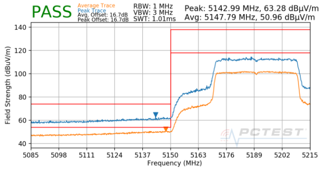
Plot 7-869. Antenna 5B (Pk & Avg, Ch.38, 80.11ax(SU), MCS0)
