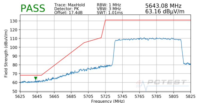
Plot 7-943. Antenna 5B (Pk, Ch.155, 802.11ax(SU), MCS11)
