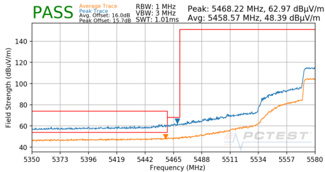
Plot 7-888. (FCC Only) Antenna 5B (Pk & Avg, Ch.118, 80.11ax(SU), MCS3)
