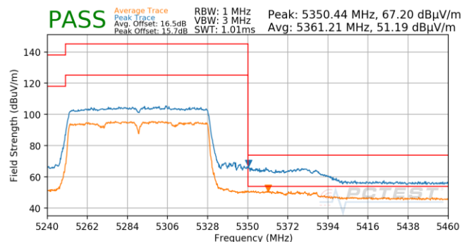
Plot 7-910. Antenna 5B (Pk & Avg, Ch.58, 802.11ac, MCS5)
