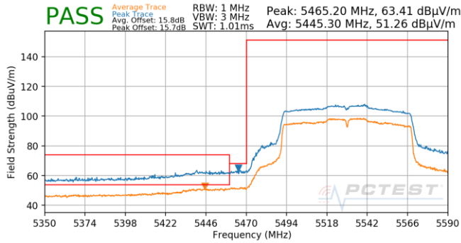
Plot 7-911. Antenna 5B (Pk & Avg, Ch.106, 802.11ac, MCS0)
