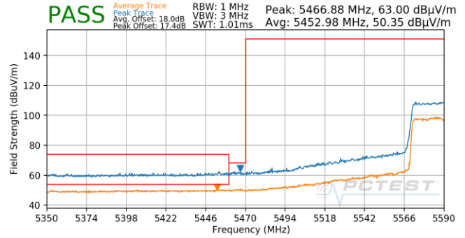
Plot 7-936. (FCC Only) Antenna 5B (Pk & Avg, Ch.122, 802.11ax(SU), MCS3)
