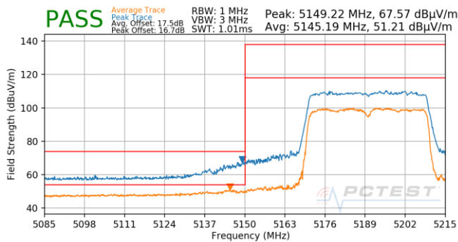
Plot 7-871. Antenna 5B (Pk & Avg, Ch.38, 80.11ax(SU), MCS11)
