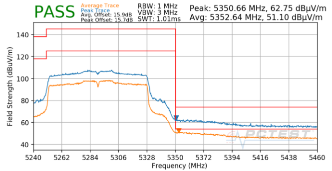
Plot 7-908. Antenna 5B (Pk & Avg, Ch.58, 802.11ac, MCS0)
