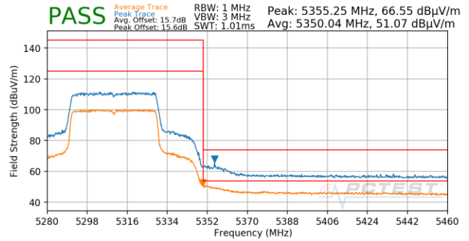
Plot 7-878. Antenna 5B (Pk & Avg, Ch.62, 80.11ax(SU), MCS0)
