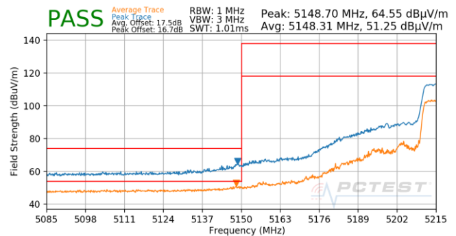
Plot 7-874. Antenna 5B (Pk & Avg, Ch.46, 80.11ax(SU), MCS11)
