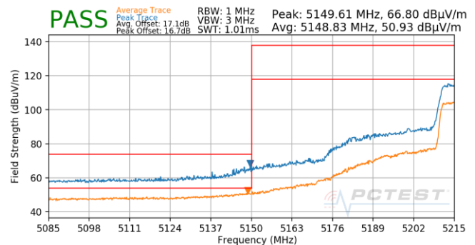
Plot 7-873. Antenna 5B (Pk & Avg, Ch.46, 80.11ax(SU), MCS3)
