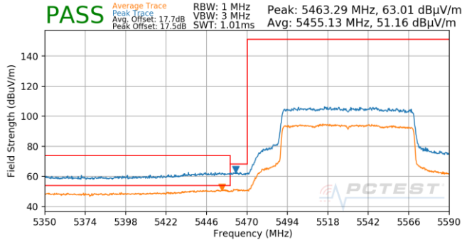
Plot 7-932. Antenna 5B (Pk & Avg, Ch.106, 802.11ax(SU), MCS0)
