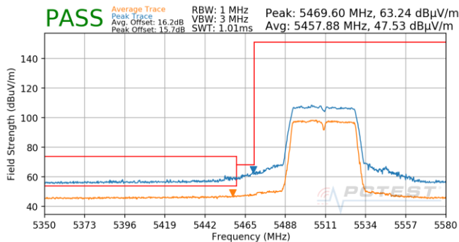
Plot 7-849. Antenna 5B (Pk & Avg, Ch.102, 802.11n, MCS5)
