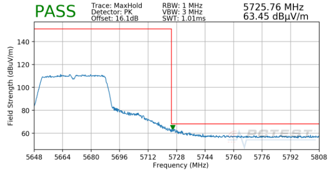
Plot 7-862. Antenna 5B (Pk, Ch.134, 802.11n, MCS5)
