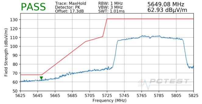
Plot 7-920. Antenna 5B (Pk, Ch.155, 802.11ac, MCS0)
