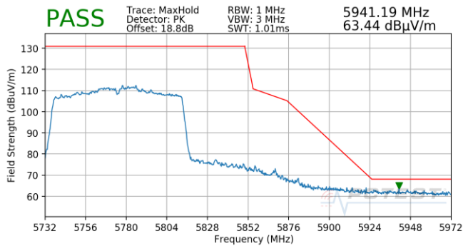
Plot 7-924. Antenna 5B (Pk, Ch.155, 802.11ac, MCS3)
