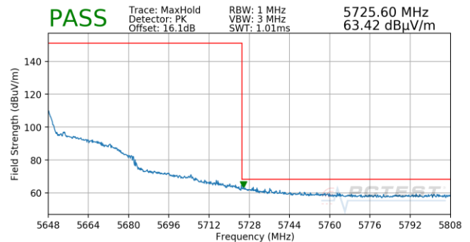
Plot 7-858. (FCC Only) Antenna 5B (Pk, Ch.126, 802.11n, MCS3)
