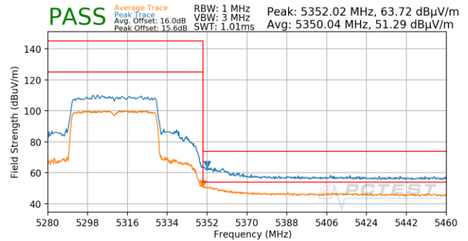
Plot 7-879. Antenna 5B (Pk & Avg, Ch.62, 80.11ax(SU), MCS3)
