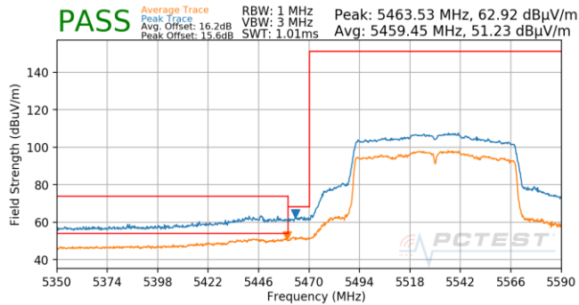
Plot 7-912. Antenna 5B (Pk & Avg, Ch.106, 802.11ac, MCS3)
