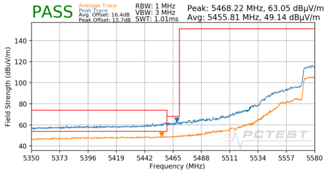
Plot 7-889. (FCC Only) Antenna 5B (Pk & Avg, Ch.118, 80.11ax(SU), MCS11)
