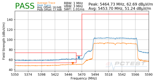
Plot 7-933. Antenna 5B (Pk & Avg, Ch.106, 802.11ax(SU), MCS3)
