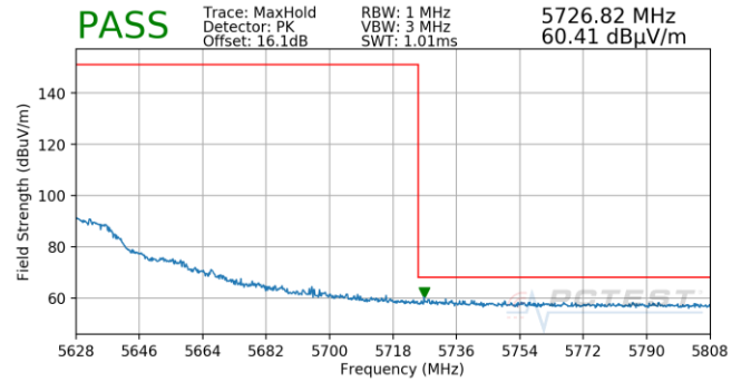
Plot 7-856. (FCC Only) Antenna 5B (Pk, Ch.118, 802.11n, MCS5)
