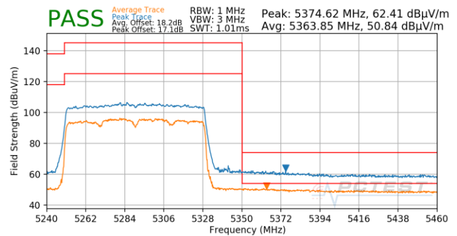
Plot 7-931. Antenna 5B (Pk & Avg, Ch.58, 802.11ax(SU), MCS11)
