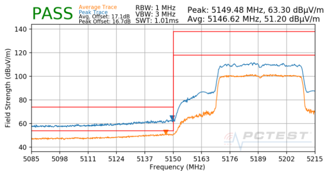
Plot 7-870. Antenna 5B (Pk & Avg, Ch.38, 80.11ax(SU), MCS3)
