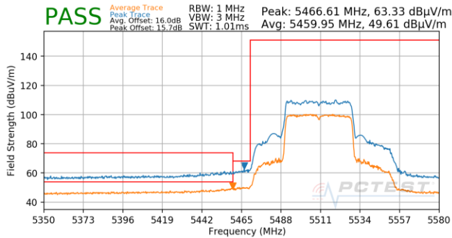
Plot 7-882. Antenna 5B (Pk & Avg, Ch.102, 80.11ax(SU), MCS3)
