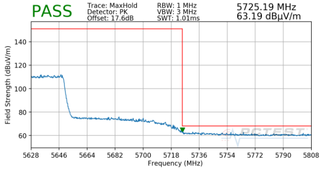
Plot 7-938. (FCC Only) Antenna 5B (Pk, Ch.122, 802.11ax(SU), MCS0)
