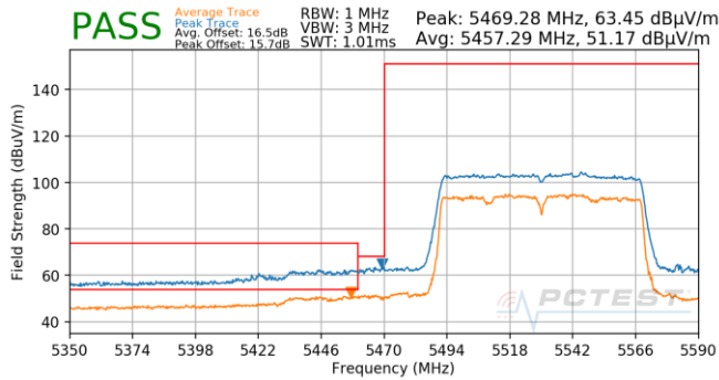
Plot 7-913. Antenna 5B (Pk & Avg, Ch.106, 802.11ac, MCS5)
