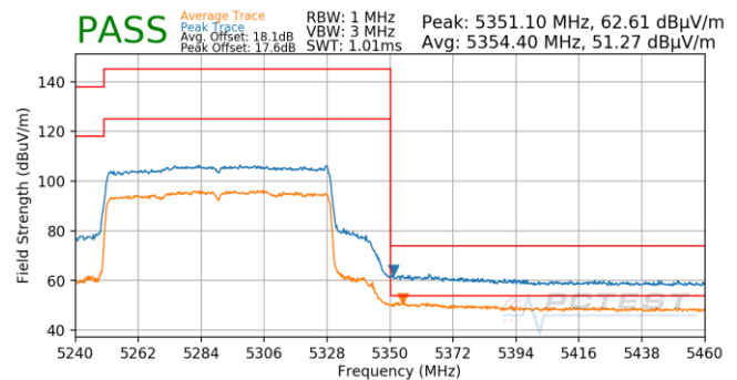
Plot 7-930. Antenna 5B (Pk & Avg, Ch.58, 802.11ax(SU), MCS3)
