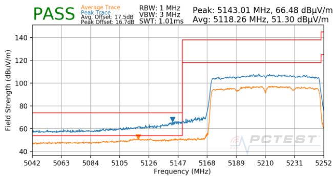
Plot 7-928. Antenna 5B (Pk & Avg, Ch.42, 802.11ax(SU), MCS11)
