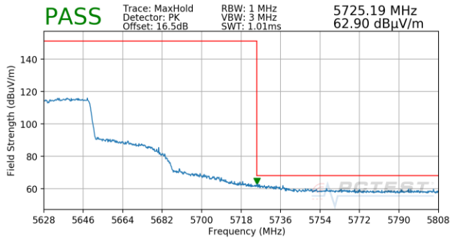
Plot 7-894. (FCC Only) Antenna 5B (Pk, Ch.126, 80.11ax(SU), MCS3)
