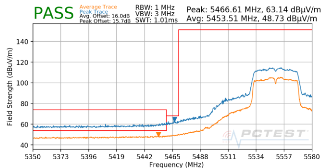
Plot 7-851. Antenna 5B (Pk & Avg, Ch.110, 802.11n, MCS3)
