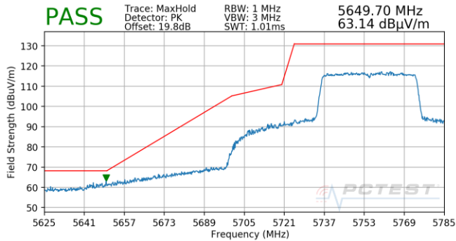
Plot 7-900. Antenna 5B (Pk, Ch.151, 80.11ax(SU), MCS3)
