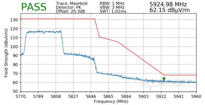
Plot 7-902. Antenna 5B (Pk, Ch.159, 80.11ax(SU), MCS0)
