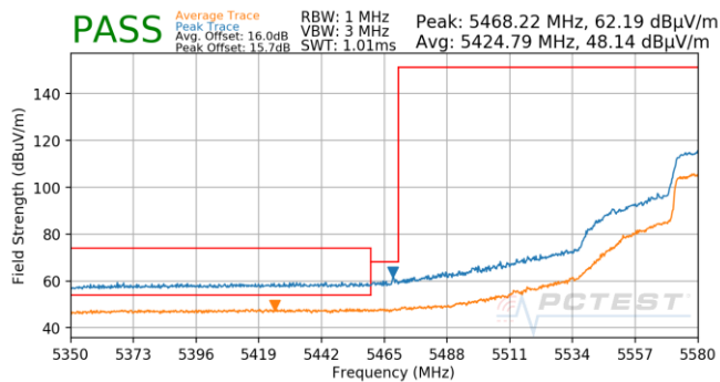
Plot 7-854. (FCC Only) Antenna 5B (Pk, Ch.118, 802.11n, MCS3)
