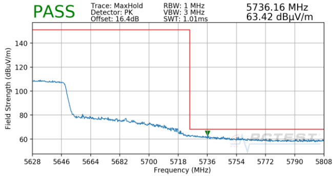
Plot 7-917. (FCC Only) Antenna 5B (Pk, Ch.122, 802.11ac, MCS0)
