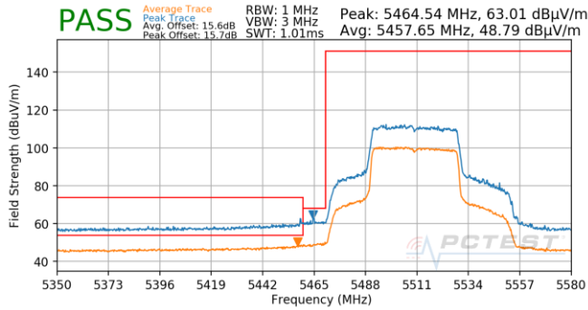
Plot 7-881. Antenna 5B (Pk & Avg, Ch.102, 80.11ax(SU), MCS0)
