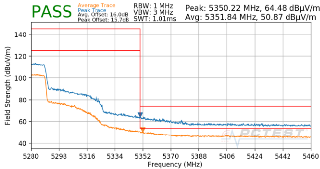
Plot 7-876. Antenna 5B (Pk & Avg, Ch.54, 80.11ax(SU), MCS3)
