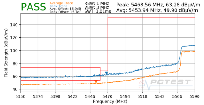
Plot 7-914. (FCC Only) Antenna 5B (Pk & Avg, Ch.122, 802.11ac, MCS0)
