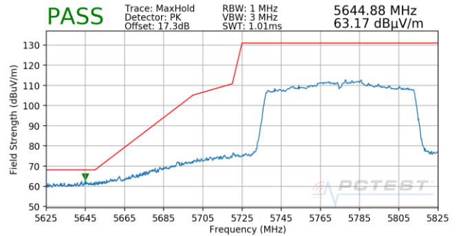
Plot 7-921. Antenna 5B (Pk, Ch.155, 802.11ac, MCS3)
