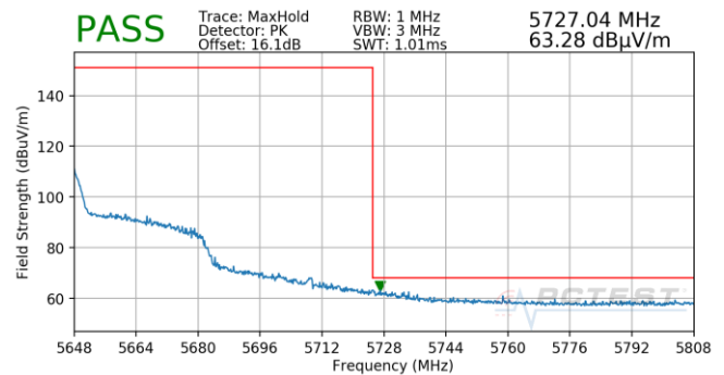
Plot 7-857. (FCC Only) Antenna 5B (Pk, Ch.126, 802.11n, MCS0)
