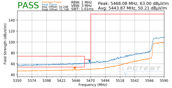
Plot 7-915. (FCC Only) Antenna 5B (Pk & Avg, Ch.122, 802.11ac, MCS3)
