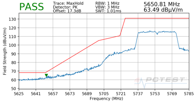
Plot 7-865. Antenna 5B (Pk, Ch.151, 802.11n, MCS5)
