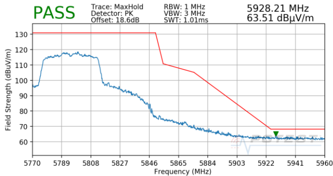
Plot 7-867. Antenna 5B (Pk, Ch.159, 802.11n, MCS3)
