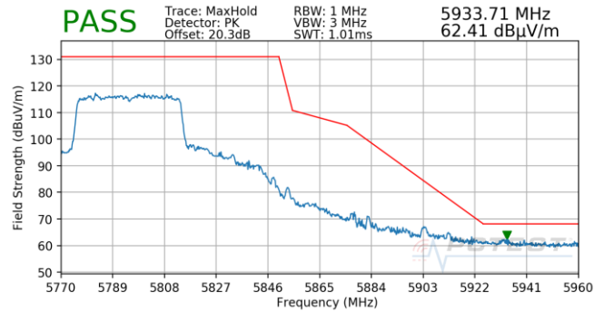
Plot 7-904. Antenna 5B (Pk, Ch.159, 80.11ax(SU), MCS11)
