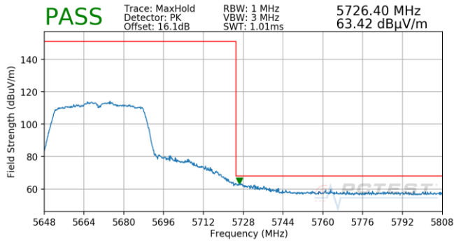
Plot 7-861. Antenna 5B (Pk, Ch.134, 802.11n, MCS3)
