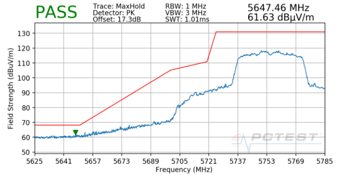
Plot 7-864. Antenna 5B (Pk, Ch.151, 802.11n, MCS3)
