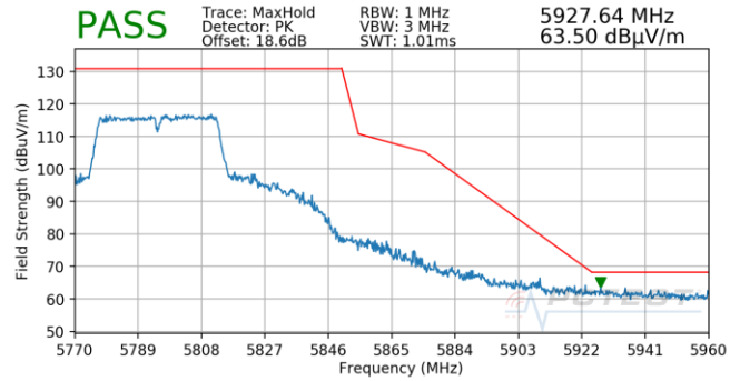
Plot 7-868. Antenna 5B (Pk, Ch.159, 802.11n, MCS5)
