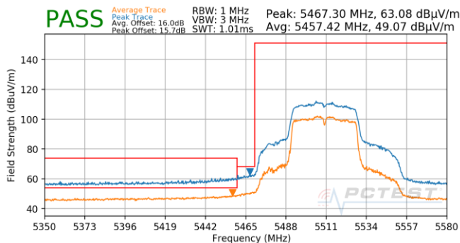
Plot 7-848. Antenna 5B (Pk & Avg, Ch.102, 802.11n, MCS3)
