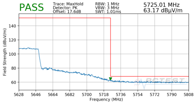
Plot 7-940. (FCC Only) Antenna 5B (Pk, Ch.122, 802.11ax(SU), MCS11)
