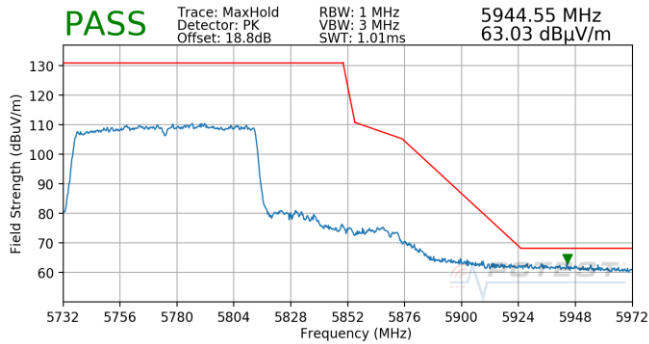
Plot 7-925. Antenna 5B (Pk, Ch.155, 802.11ac, MCS5)
