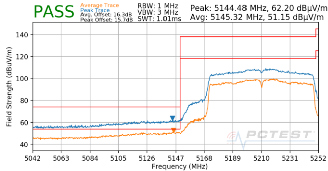
Plot 7-906. Antenna 5B (Pk & Avg, Ch.42, 802.11ac, MCS3)
