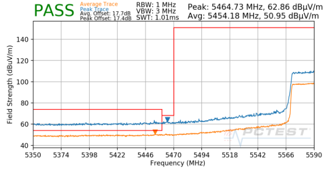
Plot 7-935. (FCC Only) Antenna 5B (Pk & Avg, Ch.122, 802.11ax(SU), MCS0)
