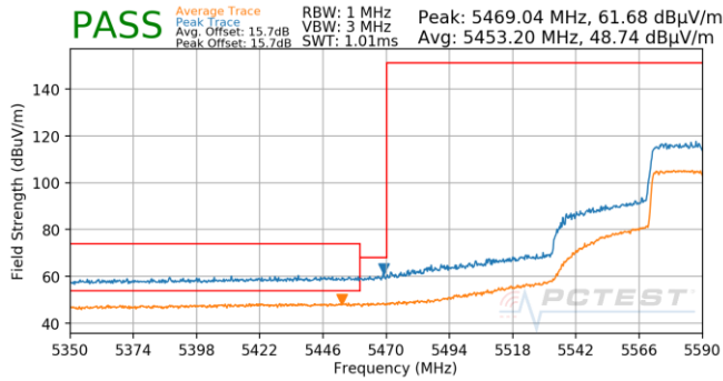
Plot 7-887. (FCC Only) Antenna 5B (Pk & Avg, Ch.118, 80.11ax(SU), MCS0)
