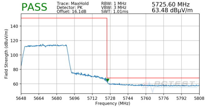
Plot 7-896. Antenna 5B (Pk, Ch.134, 80.11ax(SU), MCS0)
