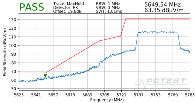
Plot 7-901. Antenna 5B (Pk, Ch.151, 80.11ax(SU), MCS11)
