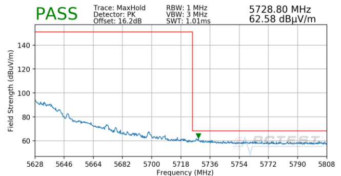
Plot 7-892. (FCC Only) Antenna 5B (Pk, Ch.118, 80.11ax(SU), MCS11)
