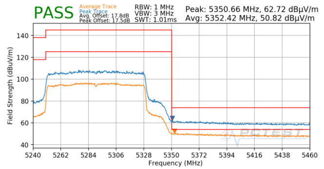
Plot 7-929. Antenna 5B (Pk & Avg, Ch.58, 802.11ax(SU), MCS0)
