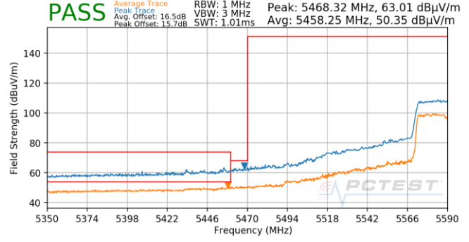
Plot 7-916. (FCC Only) Antenna 5B (Pk & Avg, Ch.122, 802.11ac, MCS5)
