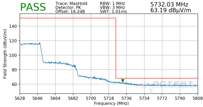
Plot 7-893. (FCC Only) Antenna 5B (Pk, Ch.126, 80.11ax(SU), MCS0)
