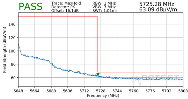
Plot 7-859. (FCC Only) Antenna 5B (Pk, Ch.126, 802.11n, MCS5)
