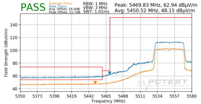
Plot 7-885. Antenna 5B (Pk & Avg, Ch.110, 80.11ax(SU), MCS3)
