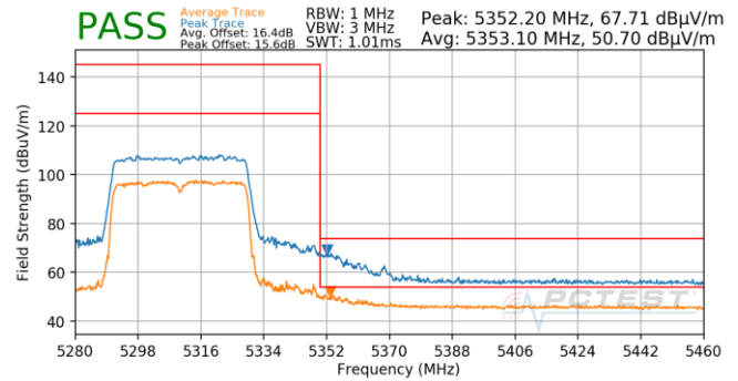
Plot 7-880. Antenna 5B (Pk & Avg, Ch.62, 80.11ax(SU), MCS11)
