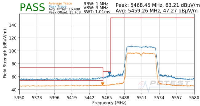
Plot 7-883. Antenna 5B (Pk & Avg, Ch.102, 80.11ax(SU), MCS11)
