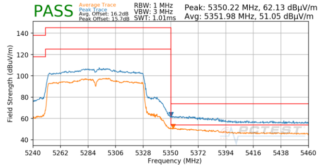
Plot 7-909. Antenna 5B (Pk & Avg, Ch.58, 802.11ac, MCS3)
