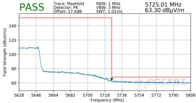
Plot 7-939. (FCC Only) Antenna 5B (Pk, Ch.122, 802.11ax(SU), MCS3)
