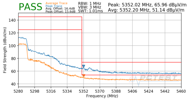
Plot 7-877. Antenna 5B (Pk & Avg, Ch.54, 80.11ax(SU), MCS11)
