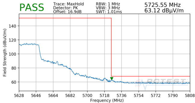
Plot 7-895. (FCC Only) Antenna 5B (Pk, Ch.126, 80.11ax(SU), MCS11)
