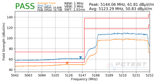
Plot 7-926. Antenna 5B (Pk & Avg, Ch.42, 802.11ax(SU), MCS0)
