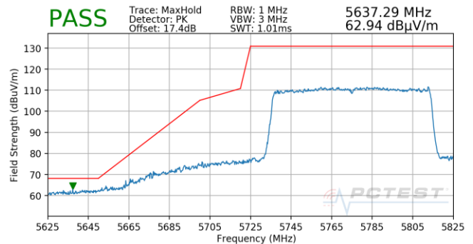
Plot 7-942. Antenna 5B (Pk, Ch.155, 802.11ax(SU), MCS3)
