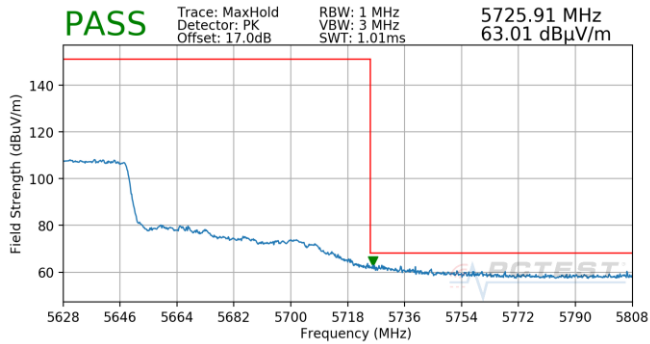
Plot 7-919. (FCC Only) Antenna 5B (Pk, Ch.122, 802.11ac, MCS5)
