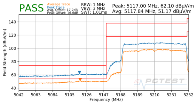
Plot 7-927. Antenna 5B (Pk & Avg, Ch.42, 802.11ax(SU), MCS3)
