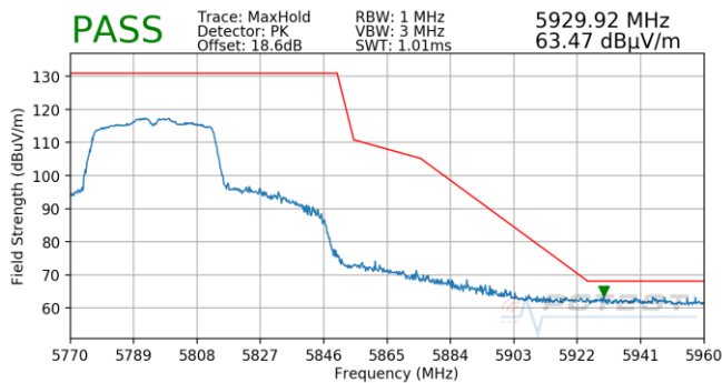
Plot 7-866. Antenna 5B (Pk, Ch.159, 802.11n, MCS0)
