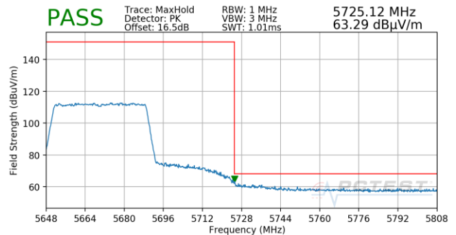
Plot 7-897. Antenna 5B (Pk, Ch.134, 80.11ax(SU), MCS3)
