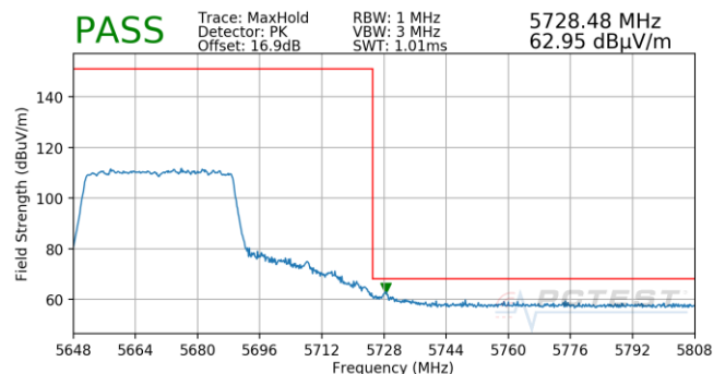
Plot 7-898. Antenna 5B (Pk, Ch.134, 80.11ax(SU), MCS11)
