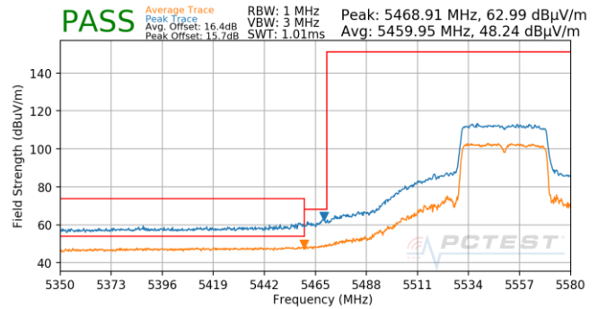
Plot 7-886. Antenna 5B (Pk & Avg, Ch.110, 80.11ax(SU), MCS11)
