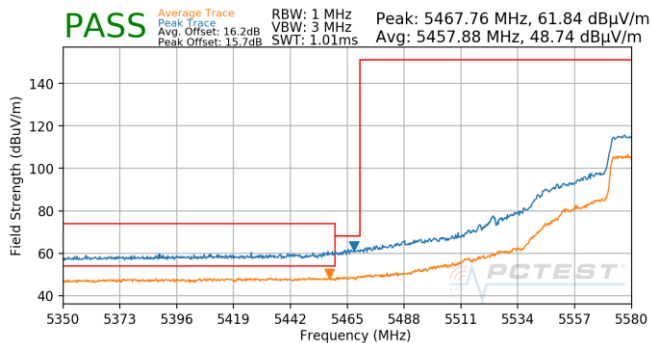
Plot 7-855. (FCC Only) Antenna 5B (Pk, Ch.118, 802.11n, MCS5)
