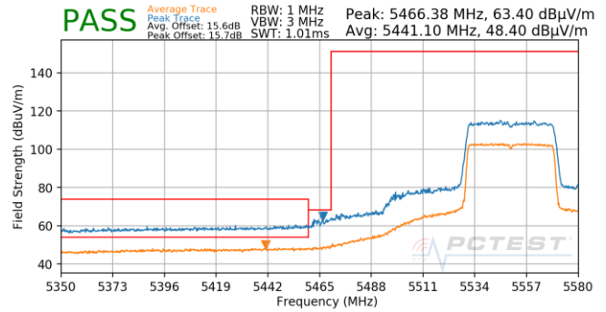
Plot 7-884. Antenna 5B (Pk & Avg, Ch.110, 80.11ax(SU), MCS0)
