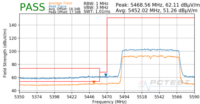
Plot 7-934. Antenna 5B (Pk & Avg, Ch.106, 802.11ax(SU), MCS11)
