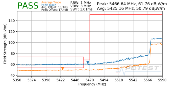
Plot 7-937. (FCC Only) Antenna 5B (Pk & Avg, Ch.122, 802.11ax(SU), MCS11)
