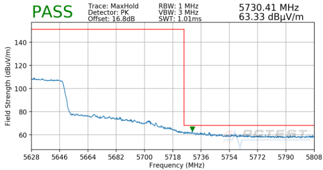
Plot 7-918. (FCC Only) Antenna 5B (Pk, Ch.122, 802.11ac, MCS3)
