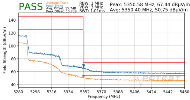
Plot 7-875. Antenna 5B (Pk & Avg, Ch.54, 80.11ax(SU), MCS0)
