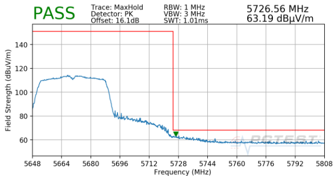
Plot 7-860. Antenna 5B (Pk, Ch.134, 802.11n, MCS0)
