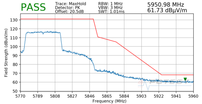
Plot 7-903. Antenna 5B (Pk, Ch.159, 80.11ax(SU), MCS3)
