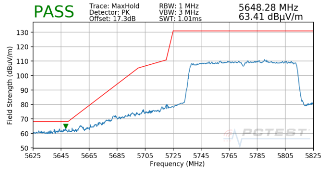
Plot 7-922. Antenna 5B (Pk, Ch.155, 802.11ac, MCS5)
