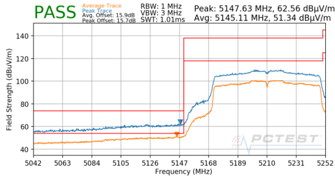
Plot 7-905. Antenna 5B (Pk & Avg, Ch.42, 802.11ac, MCS0)
