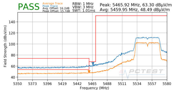
Plot 7-852. Antenna 5B (Pk & Avg, Ch.110, 802.11n, MCS5)
