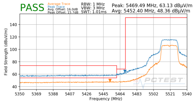
Plot 7-787. Antenna 5B (Pk & Avg, Ch.104, 802.11n, MCS5)
