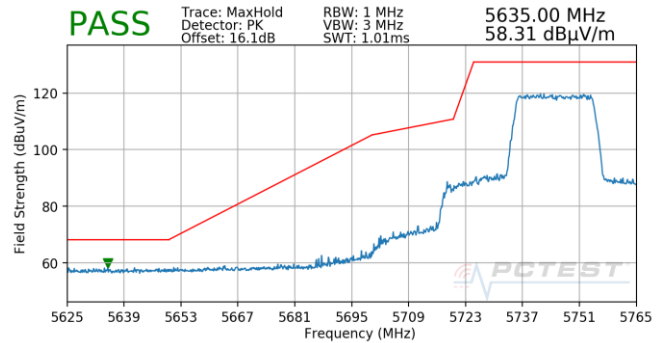
Plot 7-829. Antenna 5B (Pk, Ch.149, 802.11ax(SU), MCS0)
