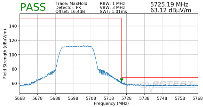
Plot 7-794. Antenna 5B (Pk, Ch.140, 802.11n, MCS5)
