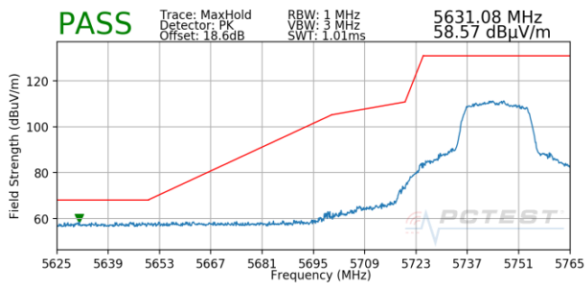
Plot 7-796. Antenna 5B (Pk, Ch.149, 802.11n, MCS3)
