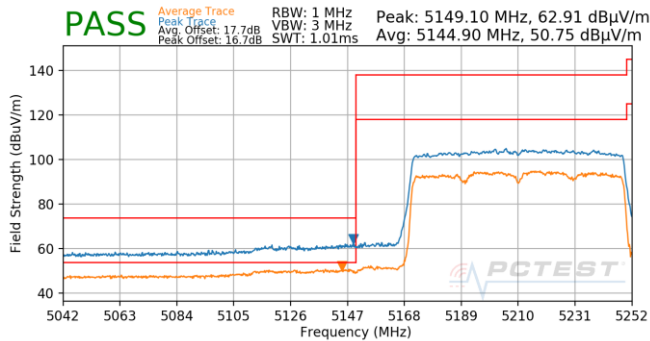
Plot 7-751. Antenna 5T (Pk & Avg, Ch.42, 802.11ax(SU), MCS11)
