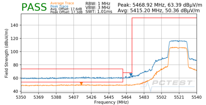
Plot 7-817. Antenna 5B (Pk & Avg, Ch.104, 802.11ax(SU), MCS3)
