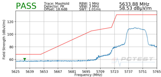
Plot 7-795. Antenna 5B (Pk, Ch.149, 802.11n, MCS0)
