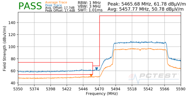
Plot 7-755. Antenna 5T (Pk & Avg, Ch.106, 802.11ax(SU), MCS0)
