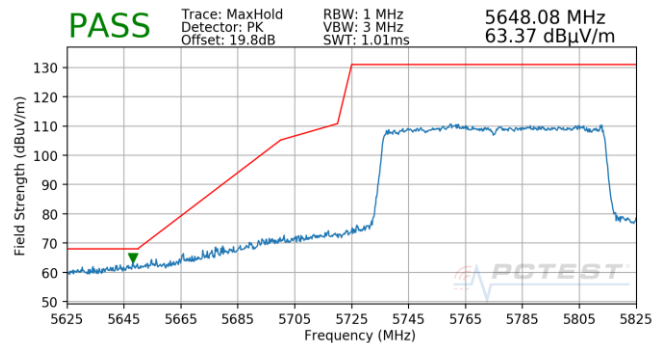
Plot 7-765. Antenna 5T (Pk, Ch.155, 802.11ax(SU), MCS3)
