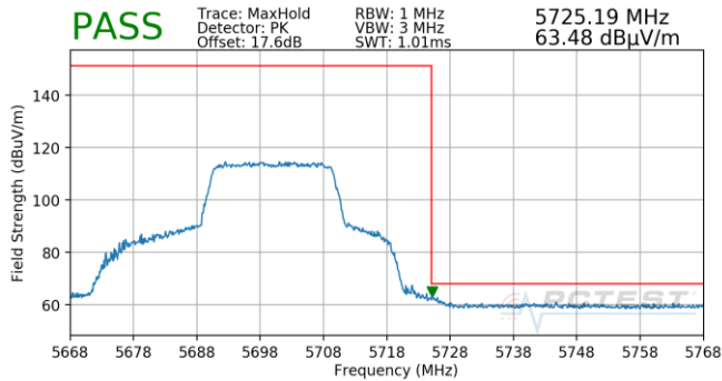
Plot 7-826. Antenna 5B (Pk, Ch.140, 802.11ax(SU), MCS0)
