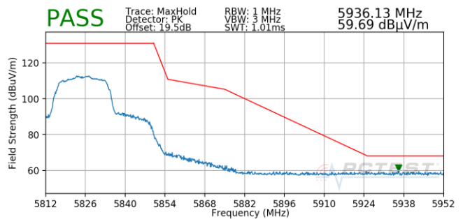
Plot 7-798. Antenna 5B (Pk, Ch.165, 802.11n, MCS0)
