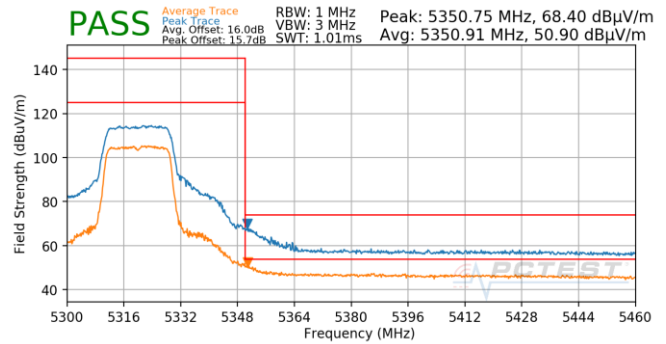
Plot 7-781. Antenna 5B (Pk & Avg, Ch.64, 802.11n, MCS5)
