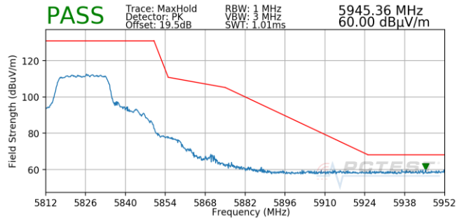
Plot 7-800. Antenna 5B (Pk, Ch.165, 802.11n, MCS5)
