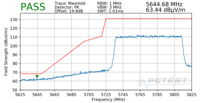
Plot 7-764. Antenna 5T (Pk, Ch.155, 802.11ax(SU), MCS0)
