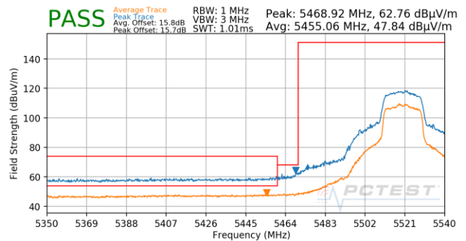
Plot 7-786. Antenna 5B (Pk & Avg, Ch.104, 802.11n, MCS3)
