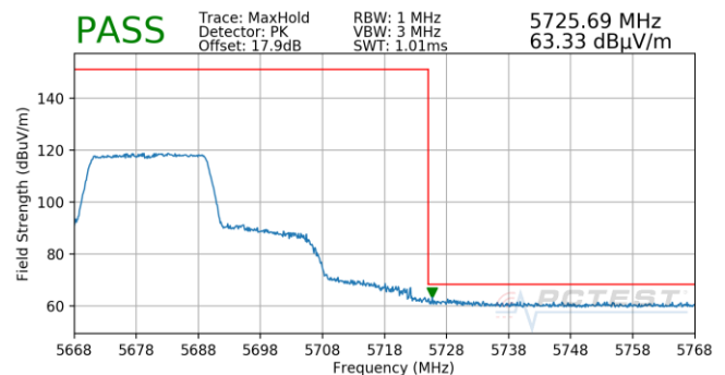
Plot 7-824. Antenna 5B (Pk, Ch.136, 802.11ax(SU), MCS3)
