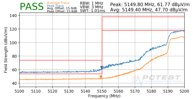
Plot 7-774. Antenna 5B (Pk & Avg, Ch.40, 802.11n, MCS3)
