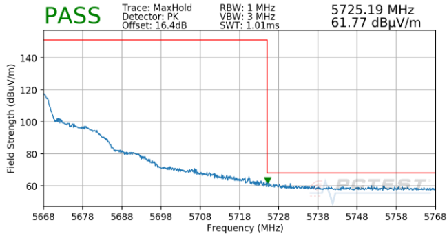
Plot 7-788. Antenna 5B (Pk, Ch.132, 802.11n, MCS5)
