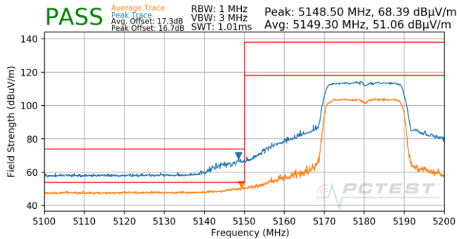
Plot 7-803. Antenna 5B (Pk & Avg, Ch.36, 802.11ax(SU), MCS11)
