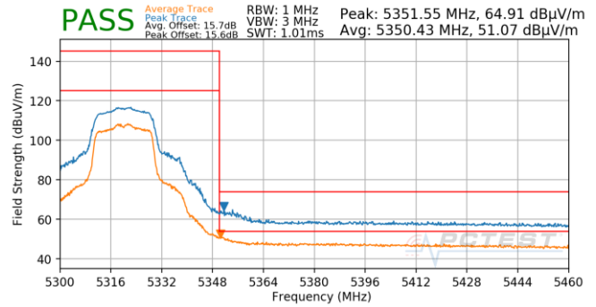
Plot 7-779. Antenna 5B (Pk & Avg, Ch.64, 802.11n, MCS0)
