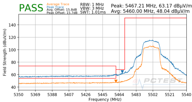
Plot 7-783. Antenna 5B (Pk & Avg, Ch.100, 802.11n, MCS3)
