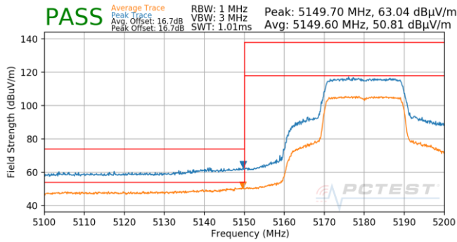
Plot 7-801. Antenna 5B (Pk & Avg, Ch.36, 802.11ax(SU), MCS0)
