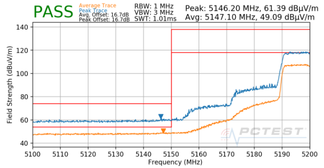
Plot 7-804. Antenna 5B (Pk & Avg, Ch.40, 802.11ax(SU), MCS0)
