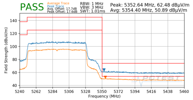
Plot 7-752. Antenna 5T (Pk & Avg, Ch.58, 802.11ax(SU), MCS0)
