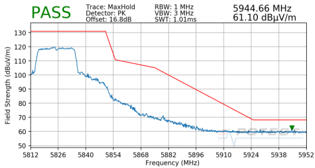
Plot 7-833. Antenna 5B (Pk, Ch.165, 802.11ax(SU), MCS3)
