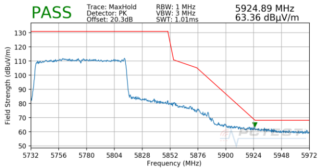
Plot 7-768. Antenna 5T (Pk, Ch.155, 802.11ax(SU), MCS3)
