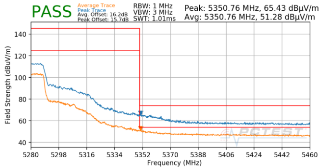
Plot 7-843. Antenna 5B (Pk & Avg, Ch.54, 802.11n, MCS5)
