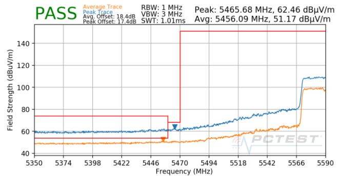
Plot 7-760. (FCC Only) Antenna 5T (Pk & Avg, Ch.122, 802.11ax(SU), MCS11)
