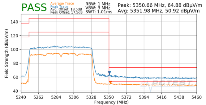
Plot 7-754. Antenna 5T (Pk & Avg, Ch.58, 802.11ax(SU), MCS11)
