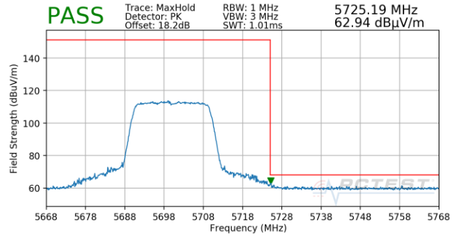
Plot 7-828. Antenna 5B (Pk, Ch.140, 802.11ax(SU), MCS11)
