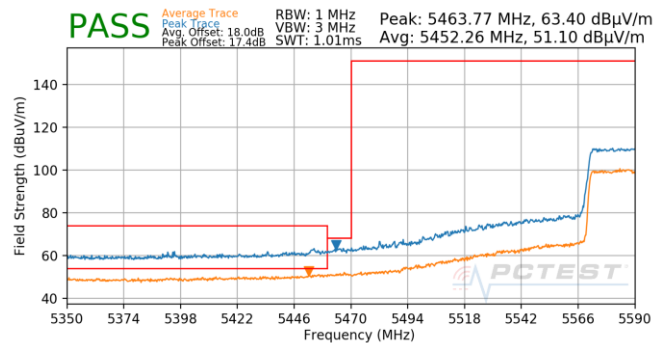
Plot 7-759. (FCC Only) Antenna 5T (Pk & Avg, Ch.122, 802.11ax(SU), MCS3)
