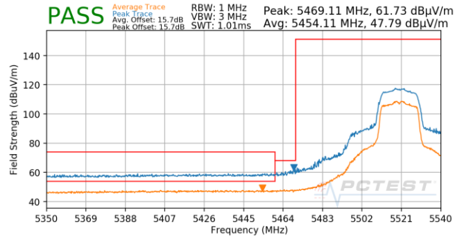
Plot 7-785. Antenna 5B (Pk & Avg, Ch.104, 802.11n, MCS0)
