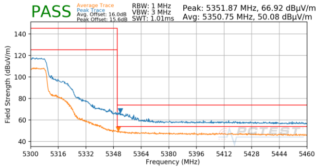
Plot 7-778. Antenna 5B (Pk & Avg, Ch.60, 802.11n, MCS5)
