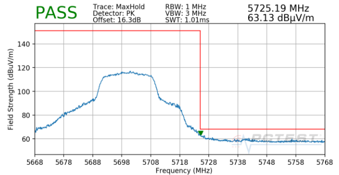
Plot 7-793. Antenna 5B (Pk, Ch.140, 802.11n, MCS3)
