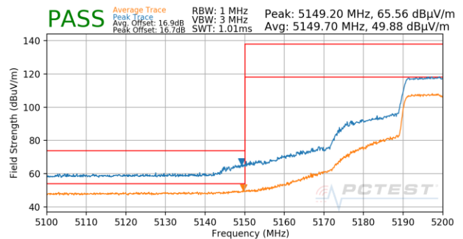
Plot 7-805. Antenna 5B (Pk & Avg, Ch.40, 802.11ax(SU), MCS3)
