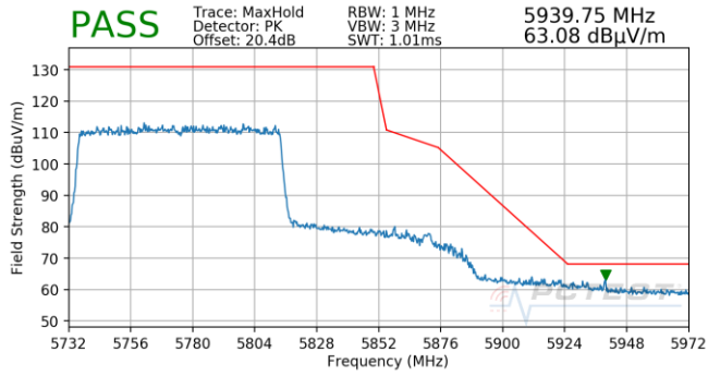
Plot 7-767. Antenna 5T (Pk, Ch.155, 802.11ax(SU), MCS0)
