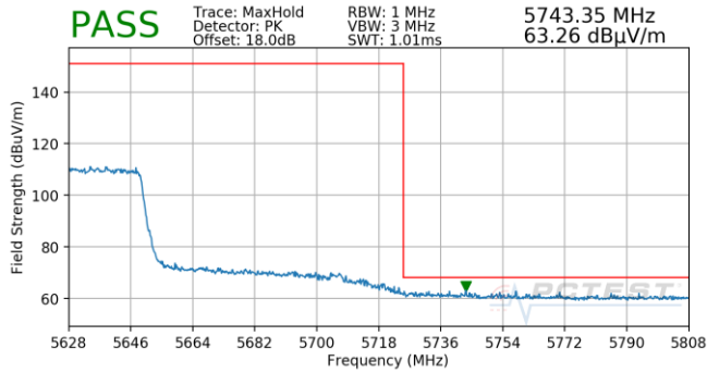
Plot 7-761. (FCC Only) Antenna 5T (Pk, Ch.122, 802.11ax(SU), MCS0)
