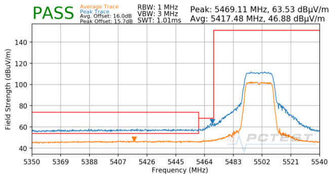
Plot 7-784. Antenna 5B (Pk & Avg, Ch.100, 802.11n, MCS5)
