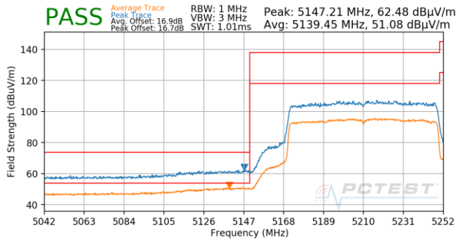
Plot 7-749. Antenna 5T (Pk & Avg, Ch.42, 802.11ax(SU), MCS0)
