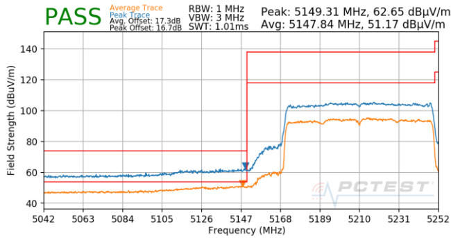
Plot 7-750. Antenna 5T (Pk & Avg, Ch.42, 802.11ax(SU), MCS3)
