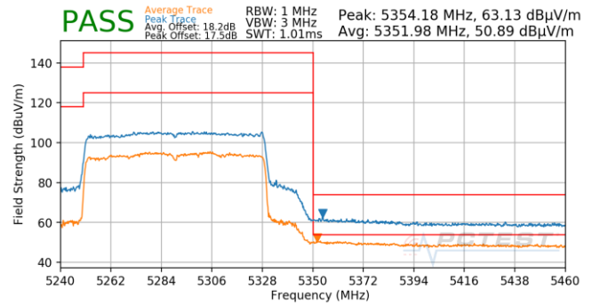
Plot 7-753. Antenna 5T (Pk & Avg, Ch.58, 802.11ax(SU), MCS3)
