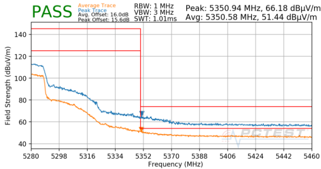
Plot 7-842. Antenna 5B (Pk & Avg, Ch.54, 802.11n, MCS3)
