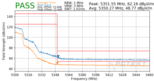
Plot 7-777. Antenna 5B (Pk & Avg, Ch.60, 802.11n, MCS3)
