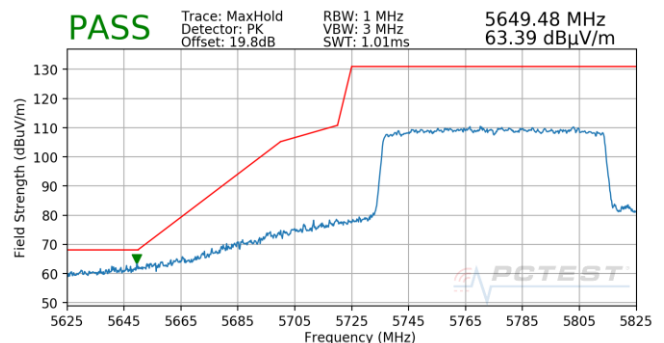
Plot 7-766. Antenna 5T (Pk, Ch.155, 802.11ax(SU), MCS11)
