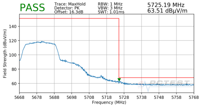
Plot 7-790. Antenna 5B (Pk, Ch.136, 802.11n, MCS3)
