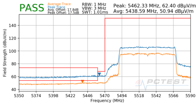
Plot 7-756. Antenna 5T (Pk & Avg, Ch.106, 802.11ax(SU), MCS3)
