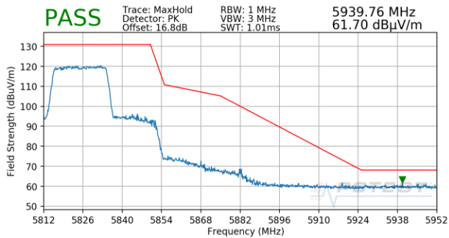
Plot 7-832. Antenna 5B (Pk, Ch.165, 802.11ax(SU), MCS0)
