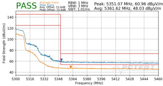
Plot 7-776. Antenna 5B (Pk & Avg, Ch.60, 802.11n, MCS0)
