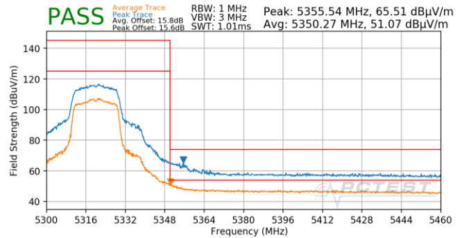
Plot 7-780. Antenna 5B (Pk & Avg, Ch.64, 802.11n, MCS3)
