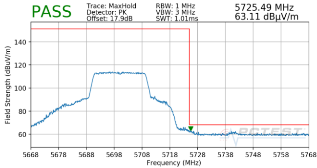
Plot 7-827. Antenna 5B (Pk, Ch.140, 802.11ax(SU), MCS3)
