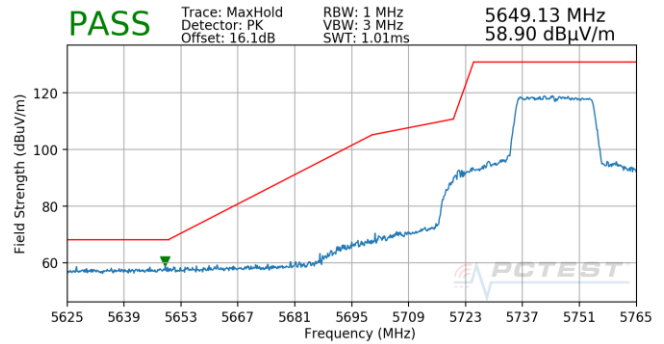
Plot 7-830. Antenna 5B (Pk, Ch.149, 802.11ax(SU), MCS3)
