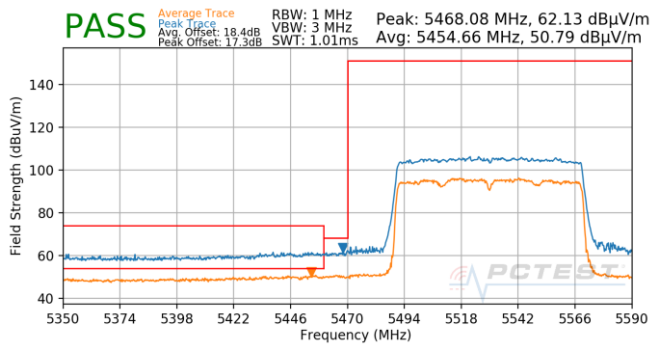
Plot 7-757. Antenna 5T (Pk & Avg, Ch.106, 802.11ax(SU), MCS11)
