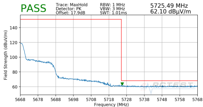
Plot 7-821. Antenna 5B (Pk, Ch.132, 802.11ax(SU), MCS3)
