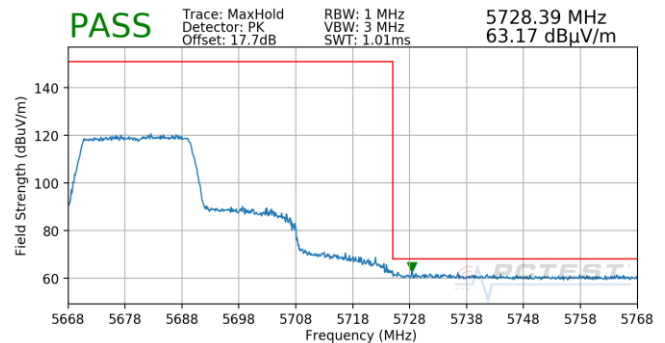
Plot 7-823. Antenna 5B (Pk, Ch.136, 802.11ax(SU), MCS0)
