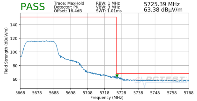
Plot 7-791. Antenna 5B (Pk, Ch.136, 802.11n, MCS5)
