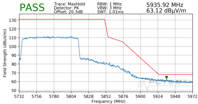
Plot 7-769. Antenna 5T (Pk, Ch.155, 802.11ax(SU), MCS11)
