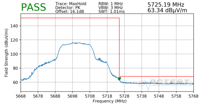
Plot 7-792. Antenna 5B (Pk, Ch.140, 802.11n, MCS0)
