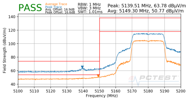
Plot 7-802. Antenna 5B (Pk & Avg, Ch.36, 802.11ax(SU), MCS3)
