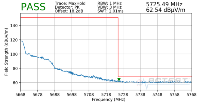
Plot 7-822. Antenna 5B (Pk, Ch.132, 802.11ax(SU), MCS11)
