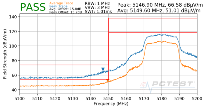
Plot 7-771. Antenna 5B (Pk & Avg, Ch.36, 802.11n, MCS3)
