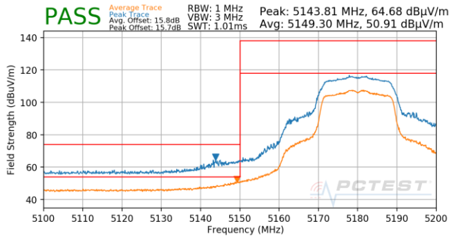
Plot 7-770. Antenna 5B (Pk & Avg, Ch.36, 802.11n, MCS0)
