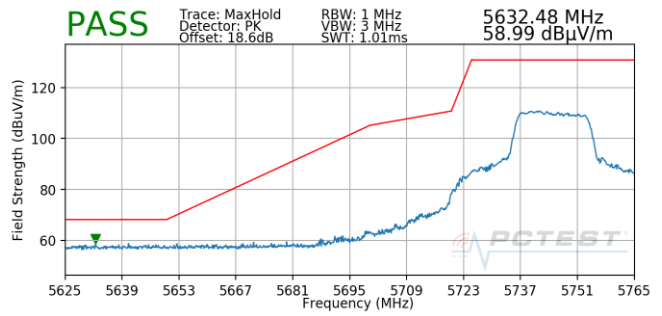
Plot 7-797. Antenna 5B (Pk, Ch.149, 802.11n, MCS5)
