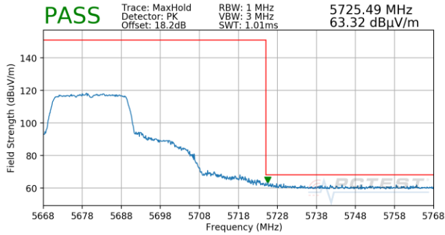
Plot 7-825. Antenna 5B (Pk, Ch.136, 802.11ax(SU), MCS11)
