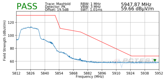
Plot 7-799. Antenna 5B (Pk, Ch.165, 802.11n, MCS3)
