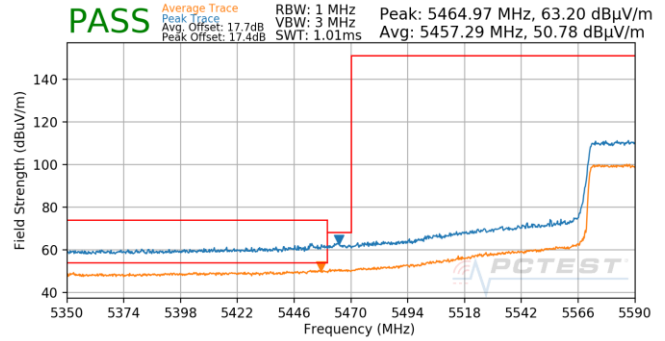
Plot 7-758. (FCC Only) Antenna 5T (Pk & Avg, Ch.122, 802.11ax(SU), MCS0)
