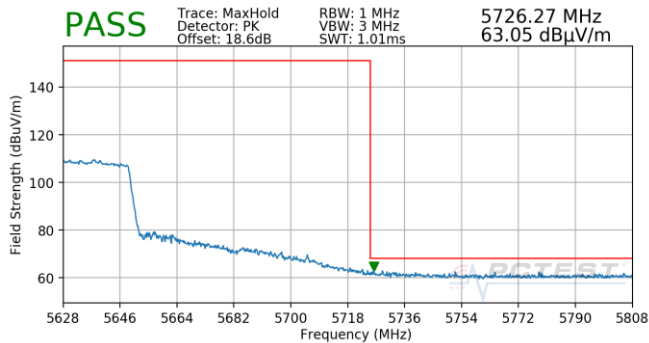
Plot 7-763. (FCC Only) Antenna 5T (Pk, Ch.122, 802.11ax(SU), MCS11)
