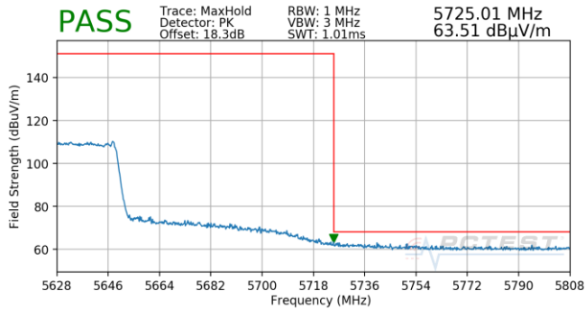
Plot 7-762. (FCC Only) Antenna 5T (Pk, Ch.122, 802.11ax(SU), MCS3)
