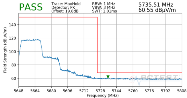
Plot 7-820. Antenna 5B (Pk, Ch.132, 802.11ax(SU), MCS0)
