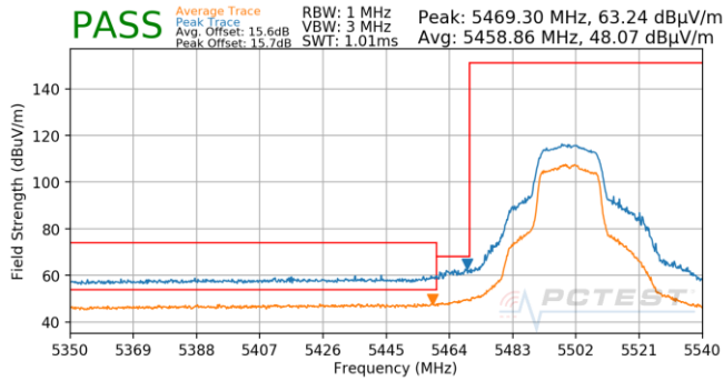
Plot 7-782. Antenna 5B (Pk & Avg, Ch.100, 802.11n, MCS0)
