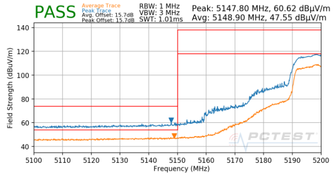
Plot 7-773. Antenna 5B (Pk & Avg, Ch.40, 802.11n, MCS0)
