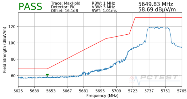
Plot 7-831. Antenna 5B (Pk, Ch.149, 802.11ax(SU), MCS11)
