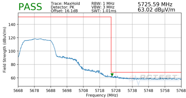
Plot 7-789. Antenna 5B (Pk, Ch.136, 802.11n, MCS0)
