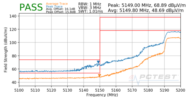
Plot 7-775. Antenna 5B (Pk & Avg, Ch.40, 802.11n, MCS5)
