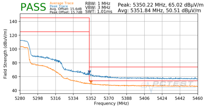
Plot 7-841. Antenna 5B (Pk & Avg, Ch.54, 802.11n, MCS0)
