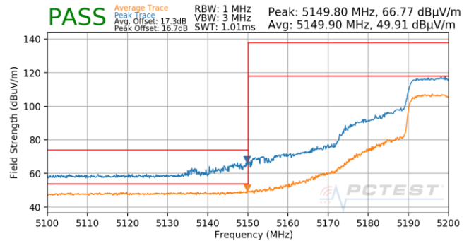
Plot 7-806. Antenna 5B (Pk & Avg, Ch.40, 802.11ax(SU), MCS11)
