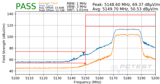
Plot 7-772. Antenna 5B (Pk & Avg, Ch.36, 802.11n, MCS5)
