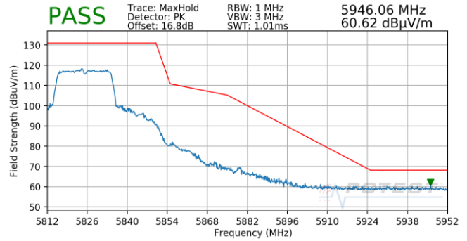
Plot 7-834. Antenna 5B (Pk, Ch.165, 802.11ax(SU), MCS11)
