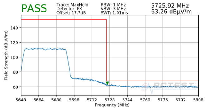
Plot 7-720. Antenna 5T (Pk, Ch.134, 80.11ax(SU), MCS3)
