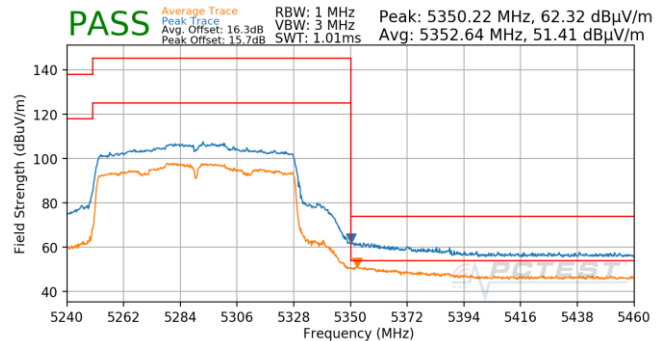
Plot 7-732. Antenna 5T (Pk & Avg, Ch.58, 802.11ac, MCS3)
