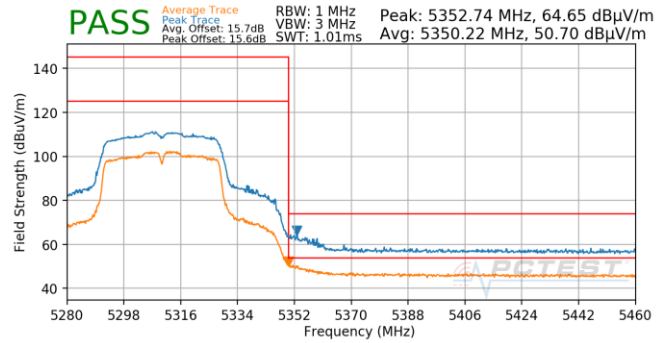
Plot 7-667. Antenna 5T (Pk & Avg, Ch.62, 802.11n, MCS0)
