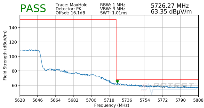
Plot 7-742. (FCC Only) Antenna 5T (Pk, Ch.122, 802.11ac, MCS5)
