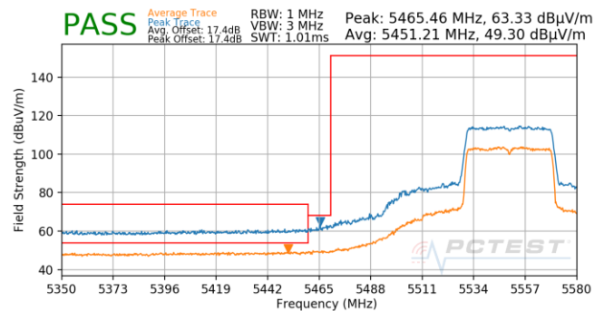
Plot 7-708. Antenna 5T (Pk & Avg, Ch.110, 80.11ax(SU), MCS3)
