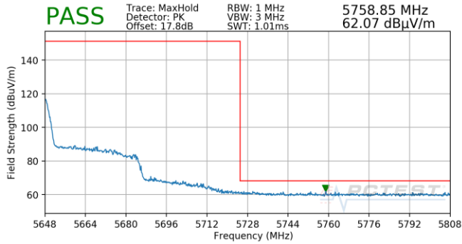
Plot 7-716. (FCC Only) Antenna 5T (Pk, Ch.126, 80.11ax(SU), MCS0)
