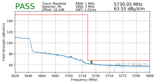
Plot 7-741. (FCC Only) Antenna 5T (Pk, Ch.122, 802.11ac, MCS3)
