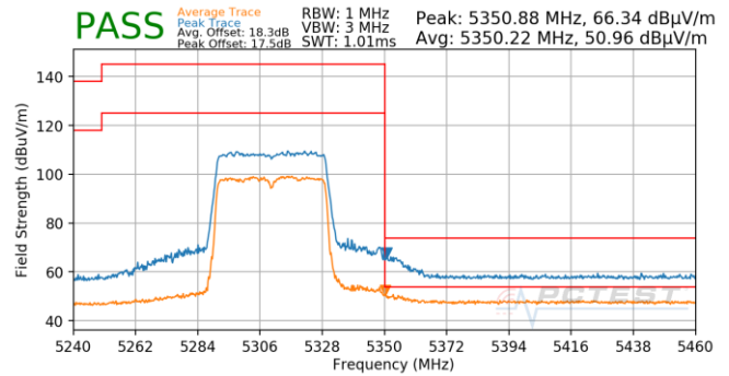
Plot 7-703. Antenna 5T (Pk & Avg, Ch.62, 80.11ax(SU), MCS11)
