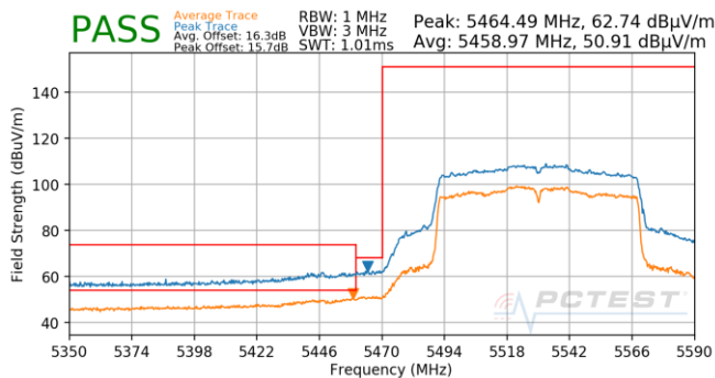
Plot 7-735. Antenna 5T (Pk & Avg, Ch.106, 802.11ac, MCS3)
