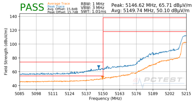
Plot 7-662. Antenna 5T (Pk & Avg, Ch.46, 802.11n, MCS3)
