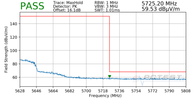
Plot 7-713. (FCC Only) Antenna 5T (Pk, Ch.118, 80.11ax(SU), MCS0)
