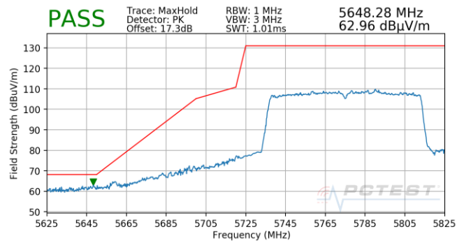
Plot 7-745. Antenna 5T (Pk, Ch.155, 802.11ac, MCS5)
