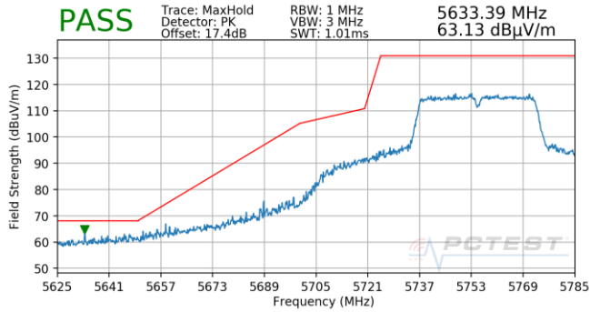
Plot 7-688. Antenna 5T (Pk, Ch.151, 802.11n, MCS5)
