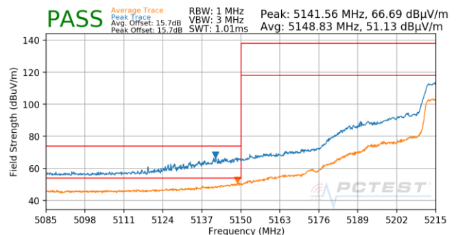
Plot 7-663. Antenna 5T (Pk & Avg, Ch.46, 802.11n, MCS5)
