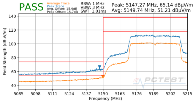
Plot 7-692. Antenna 5T (Pk & Avg, Ch.38, 80.11ax(SU), MCS0)
