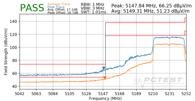
Plot 7-696. Antenna 5T (Pk & Avg, Ch.46, 80.11ax(SU), MCS3)
