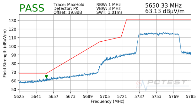
Plot 7-723. Antenna 5T (Pk, Ch.151, 80.11ax(SU), MCS3)
