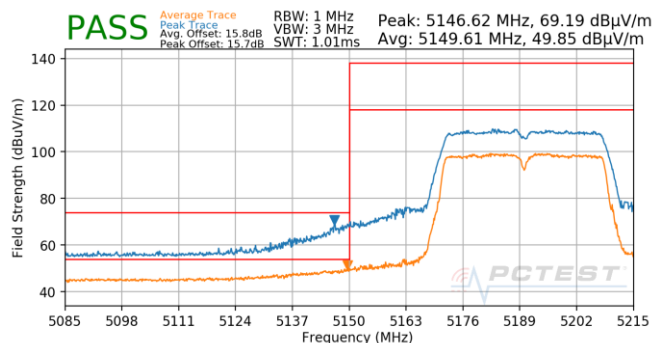
Plot 7-660. Antenna 5T (Pk & Avg, Ch.38, 802.11n, MCS5)
