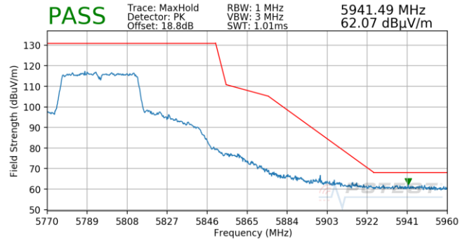
Plot 7-691. Antenna 5T (Pk, Ch.159, 802.11n, MCS5)
