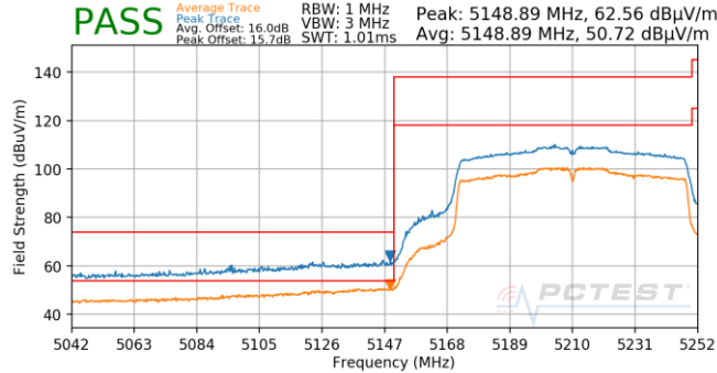
Plot 7-728. Antenna 5T (Pk & Avg, Ch.42, 802.11ac, MCS0)
