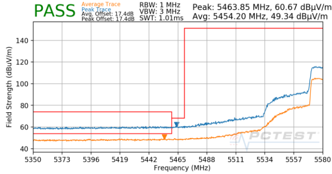
Plot 7-710. (FCC Only) Antenna 5T (Pk & Avg, Ch.118, 80.11ax(SU), MCS0)
