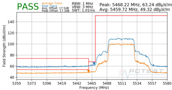
Plot 7-705. Antenna 5T (Pk & Avg, Ch.102, 80.11ax(SU), MCS3)
