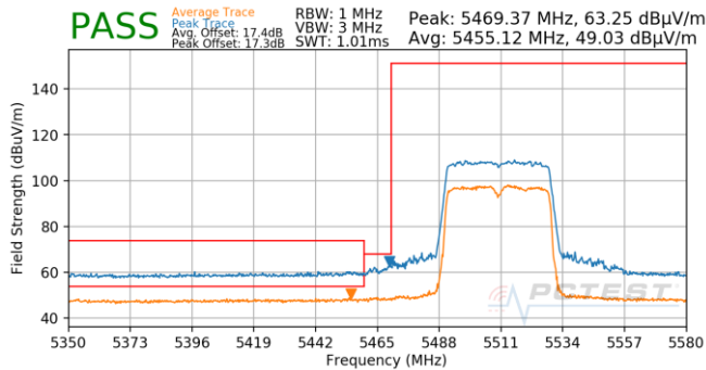
Plot 7-706. Antenna 5T (Pk & Avg, Ch.102, 80.11ax(SU), MCS11)
