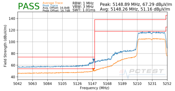
Plot 7-695. Antenna 5T (Pk & Avg, Ch.46, 80.11ax(SU), MCS0)
