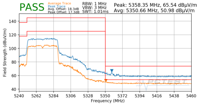
Plot 7-700. Antenna 5T (Pk & Avg, Ch.54, 80.11ax(SU), MCS11)
