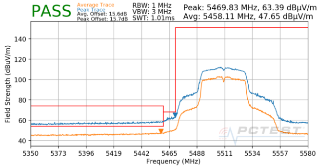
Plot 7-670. Antenna 5T (Pk & Avg, Ch.102, 802.11n, MCS0)
