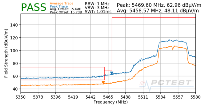
Plot 7-674. Antenna 5T (Pk & Avg, Ch.110, 802.11n, MCS3)
