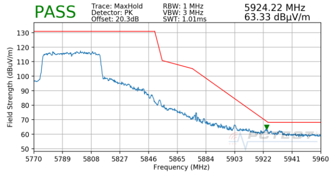
Plot 7-727. Antenna 5T (Pk, Ch.159, 80.11ax(SU), MCS11)
