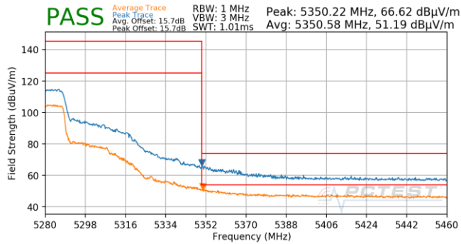
Plot 7-666. Antenna 5T (Pk & Avg, Ch.54, 802.11n, MCS5)
