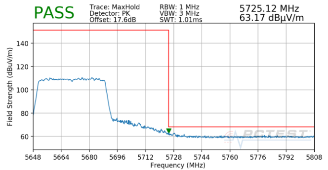
Plot 7-721. Antenna 5T (Pk, Ch.134, 80.11ax(SU), MCS11)
