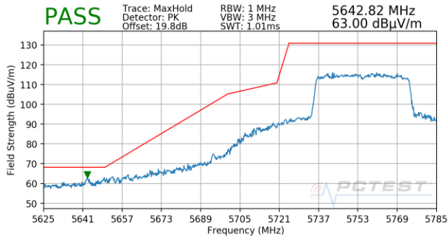
Plot 7-724. Antenna 5T (Pk, Ch.151, 80.11ax(SU), MCS11)
