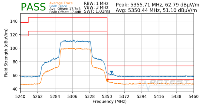
Plot 7-701. Antenna 5T (Pk & Avg, Ch.62, 80.11ax(SU), MCS0)
