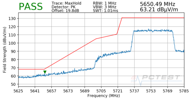
Plot 7-722. Antenna 5T (Pk, Ch.151, 80.11ax(SU), MCS0)
