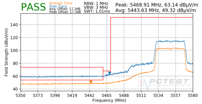
Plot 7-707. Antenna 5T (Pk & Avg, Ch.110, 80.11ax(SU), MCS0)
