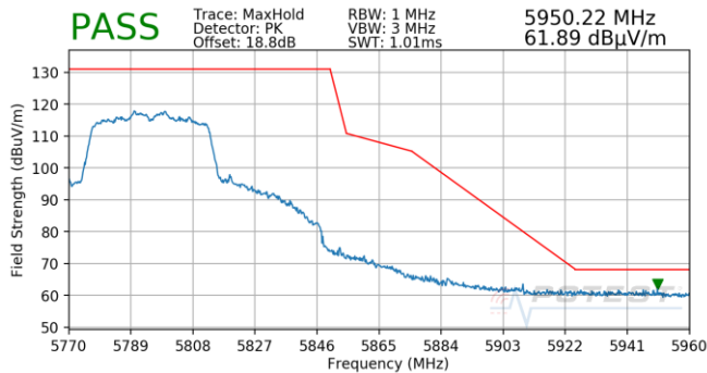
Plot 7-690. Antenna 5T (Pk, Ch.159, 802.11n, MCS3)
