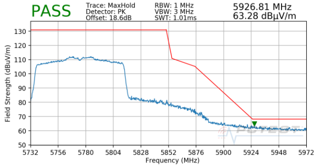
Plot 7-746. Antenna 5T (Pk, Ch.155, 802.11ac, MCS0)
