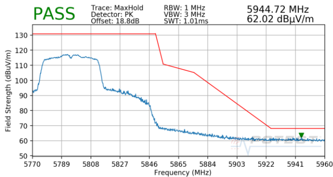
Plot 7-689. Antenna 5T (Pk, Ch.159, 802.11n, MCS0)
