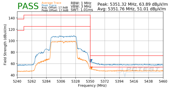
Plot 7-702. Antenna 5T (Pk & Avg, Ch.62, 80.11ax(SU), MCS3)
