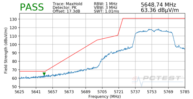
Plot 7-687. Antenna 5T (Pk, Ch.151, 802.11n, MCS3)
