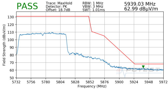
Plot 7-748. Antenna 5T (Pk, Ch.155, 802.11ac, MCS5)
