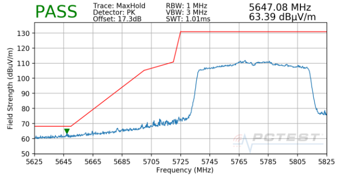
Plot 7-743. Antenna 5T (Pk, Ch.155, 802.11ac, MCS0)
