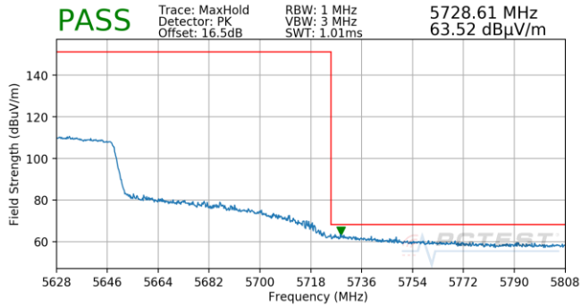
Plot 7-740. (FCC Only) Antenna 5T (Pk, Ch.122, 802.11ac, MCS0)
