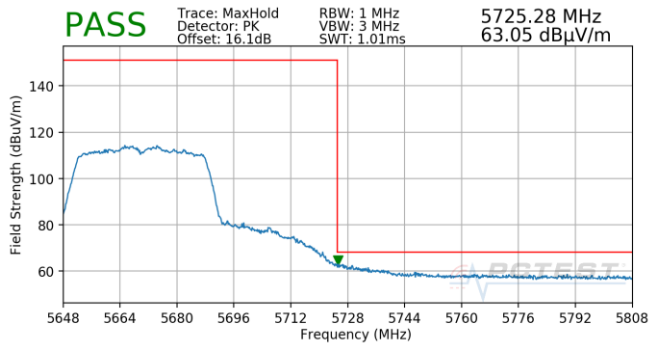
Plot 7-684. Antenna 5T (Pk, Ch.134, 802.11n, MCS3)
