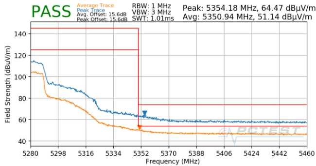
Plot 7-665. Antenna 5T (Pk & Avg, Ch.54, 802.11n, MCS3)
