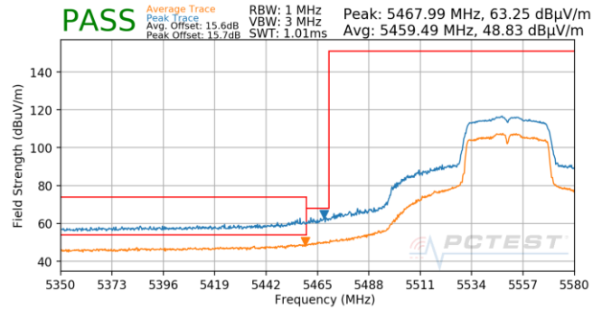
Plot 7-673. Antenna 5T (Pk & Avg, Ch.110, 802.11n, MCS0)
