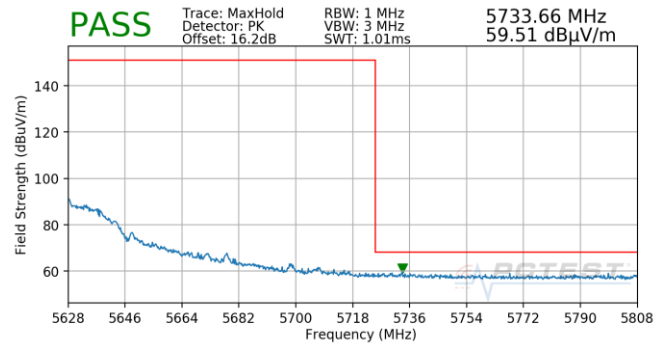
Plot 7-715. (FCC Only) Antenna 5T (Pk, Ch.118, 80.11ax(SU), MCS11)
