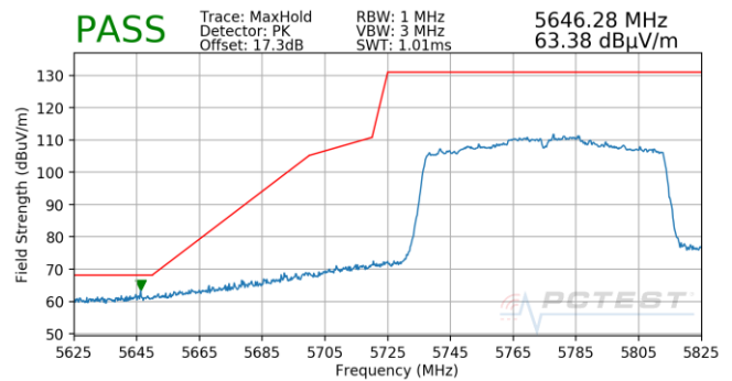
Plot 7-744. Antenna 5T (Pk, Ch.155, 802.11ac, MCS3)
