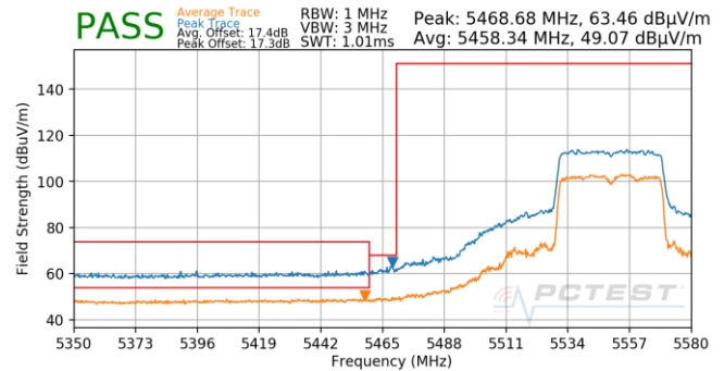
Plot 7-709. Antenna 5T (Pk & Avg, Ch.110, 80.11ax(SU), MCS11)
