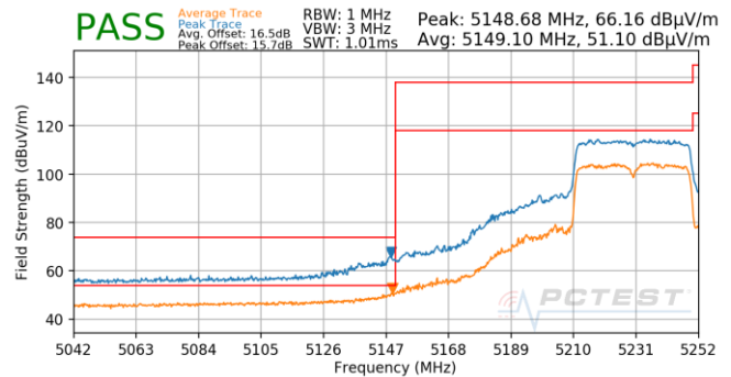
Plot 7-697. Antenna 5T (Pk & Avg, Ch.46, 80.11ax(SU), MCS11)
