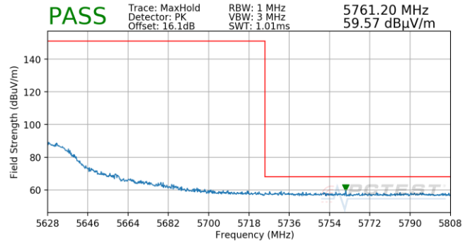
Plot 7-679. (FCC Only) Antenna 5T (Pk, Ch.118, 802.11n, MCS5)
