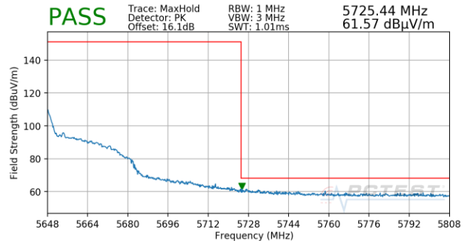
Plot 7-681. (FCC Only) Antenna 5T (Pk, Ch.126, 802.11n, MCS3)
