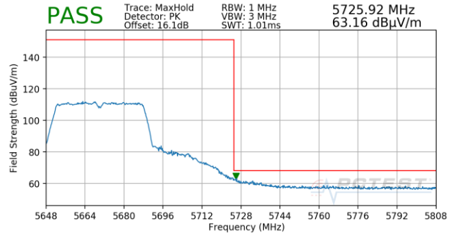
Plot 7-685. Antenna 5T (Pk, Ch.134, 802.11n, MCS5)
