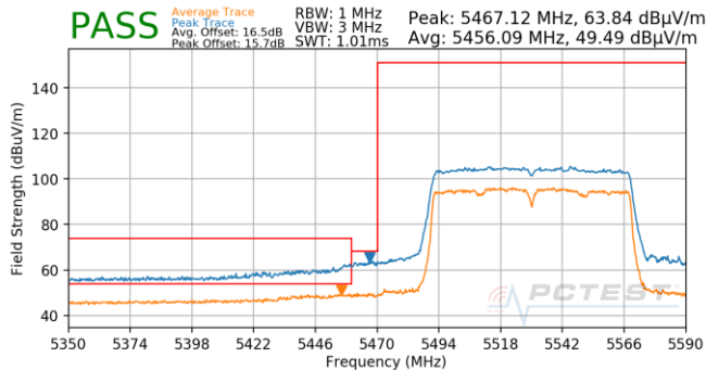
Plot 7-736. Antenna 5T (Pk & Avg, Ch.106, 802.11ac, MCS5)
