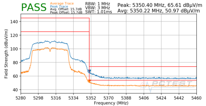
Plot 7-668. Antenna 5T (Pk & Avg, Ch.62, 802.11n, MCS3)
