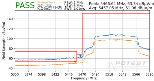
Plot 7-734. Antenna 5T (Pk & Avg, Ch.106, 802.11ac, MCS0)
