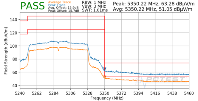
Plot 7-731. Antenna 5T (Pk & Avg, Ch.58, 802.11ac, MCS0)
