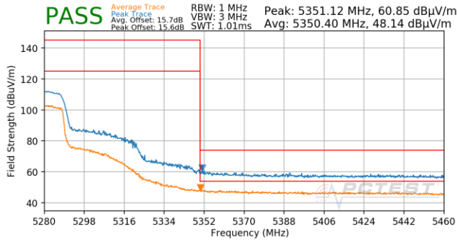
Plot 7-664. Antenna 5T (Pk & Avg, Ch.54, 802.11n, MCS0)
