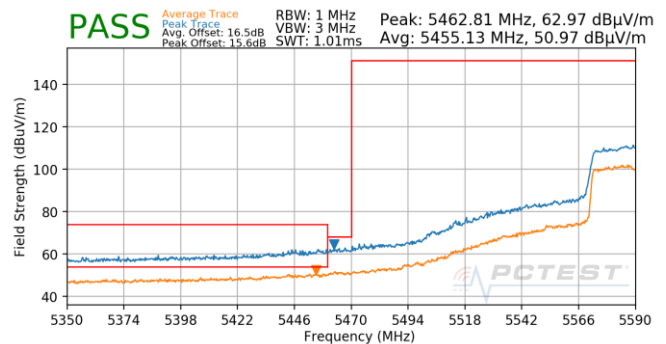
Plot 7-738. (FCC Only) Antenna 5T (Pk & Avg, Ch.122, 802.11ac, MCS3)
