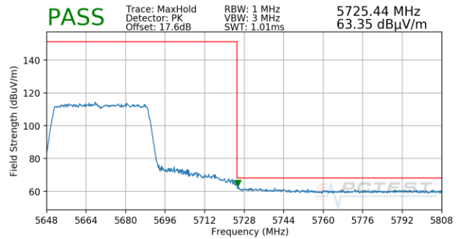
Plot 7-719. Antenna 5T (Pk, Ch.134, 80.11ax(SU), MCS0)
