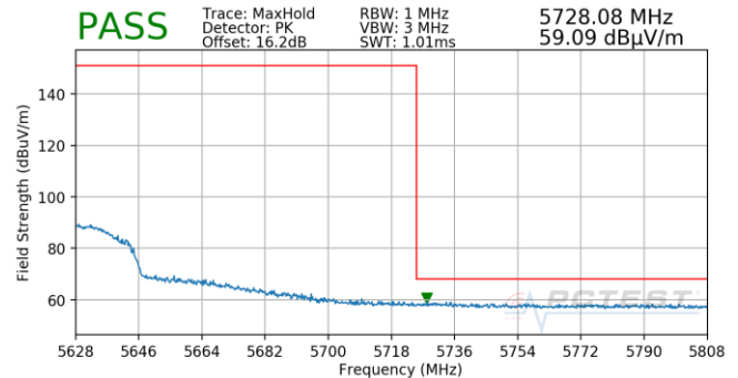
Plot 7-714. (FCC Only) Antenna 5T (Pk, Ch.118, 80.11ax(SU), MCS3)
