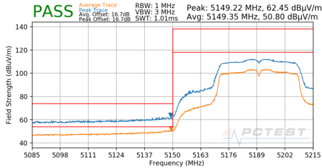
Plot 7-658. Antenna 5T (Pk & Avg, Ch.38, 802.11n, MCS0)
