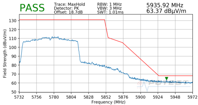
Plot 7-747. Antenna 5T (Pk, Ch.155, 802.11ac, MCS3)
