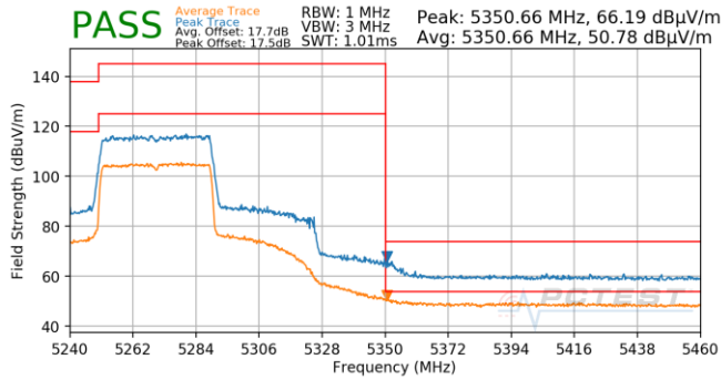
Plot 7-698. Antenna 5T (Pk & Avg, Ch.54, 80.11ax(SU), MCS0)
