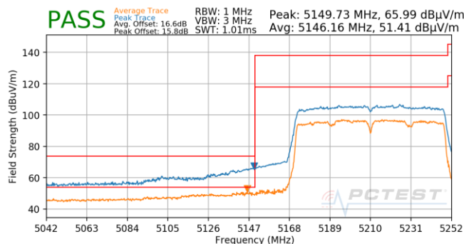
Plot 7-730. Antenna 5T (Pk & Avg, Ch.42, 802.11ac, MCS5)
