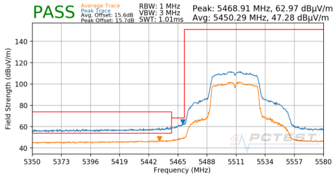
Plot 7-671. Antenna 5T (Pk & Avg, Ch.102, 802.11n, MCS3)
