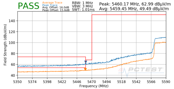
Plot 7-737. (FCC Only) Antenna 5T (Pk & Avg, Ch.122, 802.11ac, MCS0)
