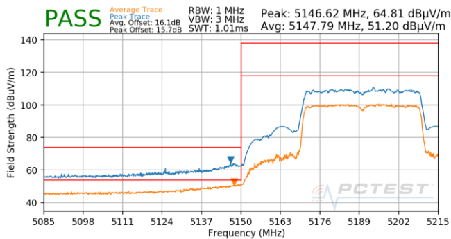
Plot 7-693. Antenna 5T (Pk & Avg, Ch.38, 80.11ax(SU), MCS3)
