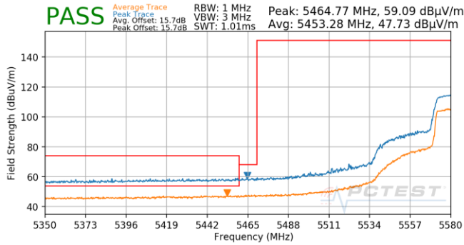
Plot 7-676. (FCC Only) Antenna 5T (Pk & Avg, Ch.118, 802.11n, MCS0)
