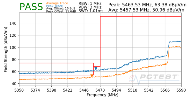
Plot 7-739. (FCC Only) Antenna 5T (Pk & Avg, Ch.122, 802.11ac, MCS5)
