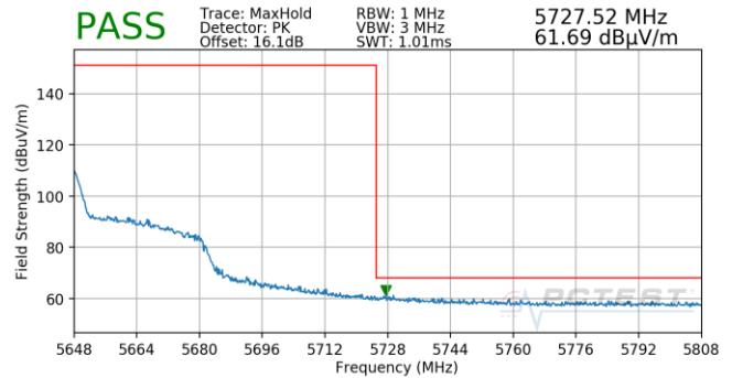
Plot 7-680. (FCC Only) Antenna 5T (Pk, Ch.126, 802.11n, MCS0)
