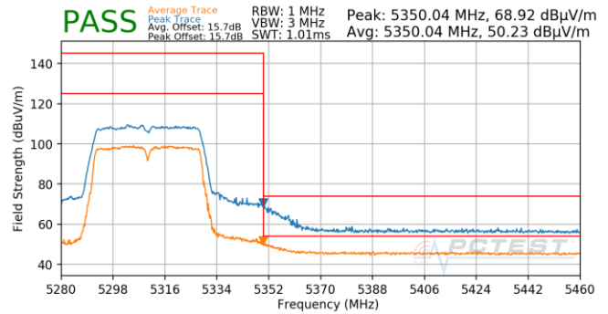
Plot 7-669. Antenna 5T (Pk & Avg, Ch.62, 802.11n, MCS5)
