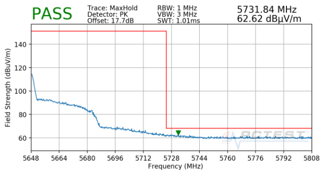
Plot 7-717. (FCC Only) Antenna 5T (Pk, Ch.126, 80.11ax(SU), MCS3)
