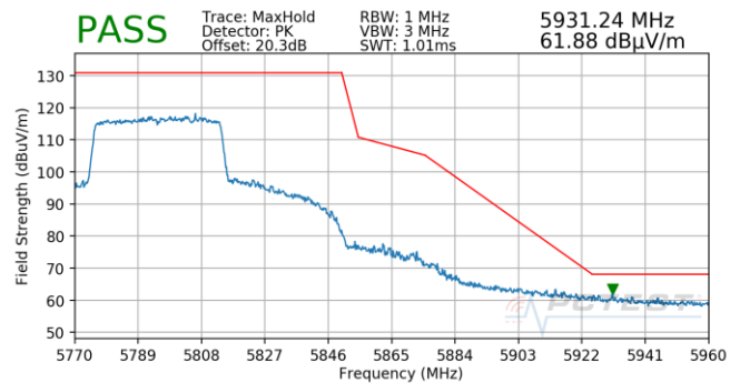
Plot 7-726. Antenna 5T (Pk, Ch.159, 80.11ax(SU), MCS3)
