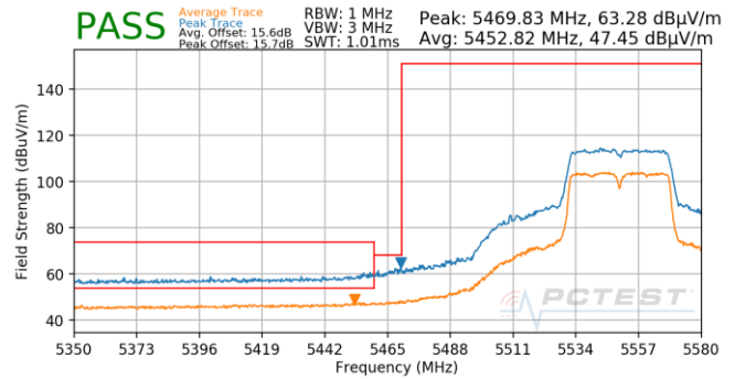
Plot 7-675. Antenna 5T (Pk & Avg, Ch.110, 802.11n, MCS5)
