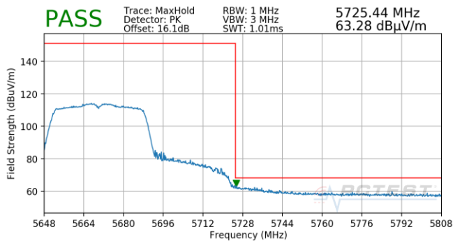
Plot 7-683. Antenna 5T (Pk, Ch.134, 802.11n, MCS0)
