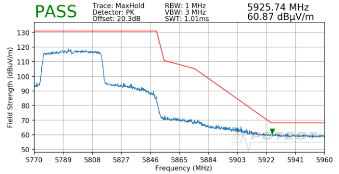
Plot 7-725. Antenna 5T (Pk, Ch.159, 80.11ax(SU), MCS0)
