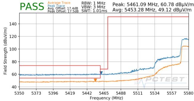
Plot 7-711. (FCC Only) Antenna 5T (Pk & Avg, Ch.118, 80.11ax(SU), MCS3)
