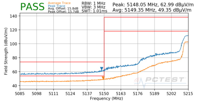
Plot 7-661. Antenna 5T (Pk & Avg, Ch.46, 802.11n, MCS0)
