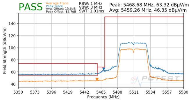
Plot 7-672. Antenna 5T (Pk & Avg, Ch.102, 802.11n, MCS5)
