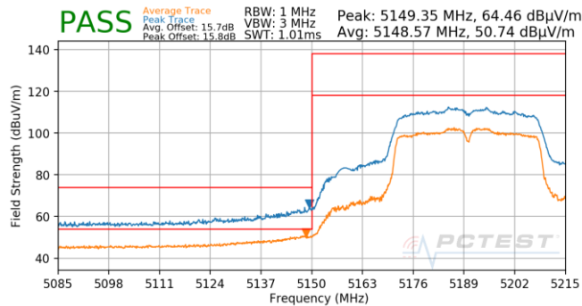
Plot 7-659. Antenna 5T (Pk & Avg, Ch.38, 802.11n, MCS3)
