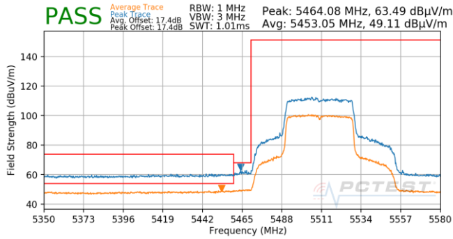
Plot 7-704. Antenna 5T (Pk & Avg, Ch.102, 80.11ax(SU), MCS0)
