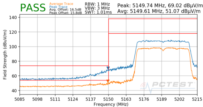
Plot 7-694. Antenna 5T (Pk & Avg, Ch.38, 80.11ax(SU), MCS11)
