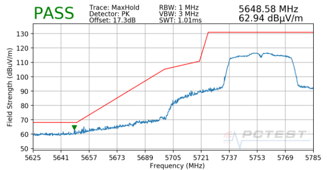
Plot 7-686. Antenna 5T (Pk, Ch.151, 802.11n, MCS0)
