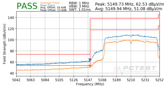
Plot 7-729. Antenna 5T (Pk & Avg, Ch.42, 802.11ac, MCS3)
