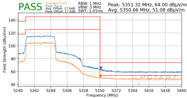
Plot 7-699. Antenna 5T (Pk & Avg, Ch.54, 80.11ax(SU), MCS3)
