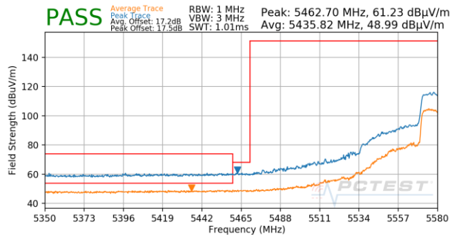
Plot 7-712. (FCC Only) Antenna 5T (Pk & Avg, Ch.118, 80.11ax(SU), MCS11)
