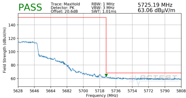
Plot 7-718. (FCC Only) Antenna 5T (Pk, Ch.126, 80.11ax(SU), MCS11)
