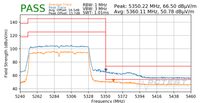
Plot 7-733. Antenna 5T (Pk & Avg, Ch.58, 802.11ac, MCS5)
