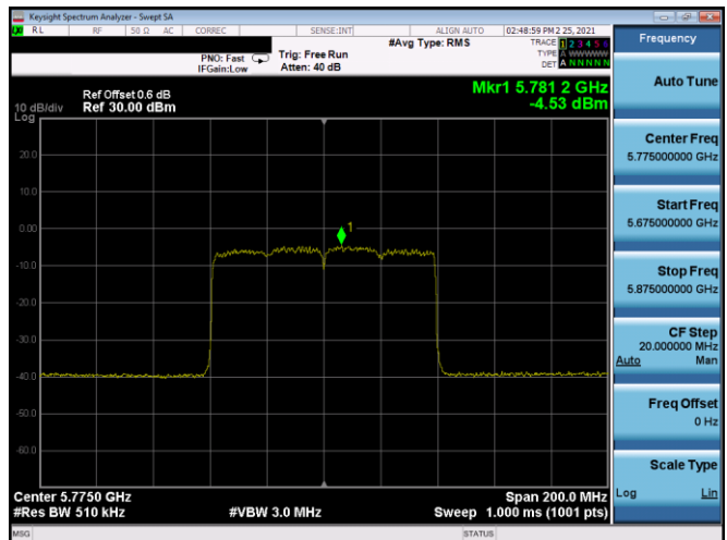
Plot 7-455. PSD CDD Antenna 5T (80MHz BW 802.11ax(SU) – Ch. 155, MCS3)
