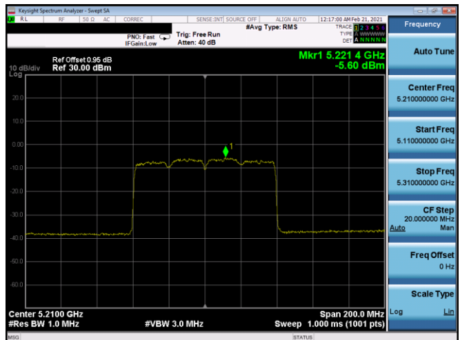
Plot 7-503. ISED PSD SDM Antenna 5T (80MHz BW 11ax(SU) – Ch.42, MCS11)
