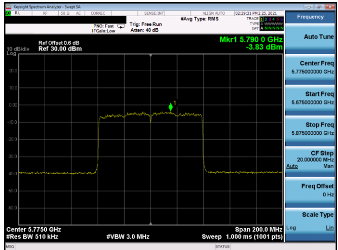
Plot 7-456. PSD CDD Antenna 5B (80MHz BW 802.11ax(SU) – Ch. 155, MCS3)
