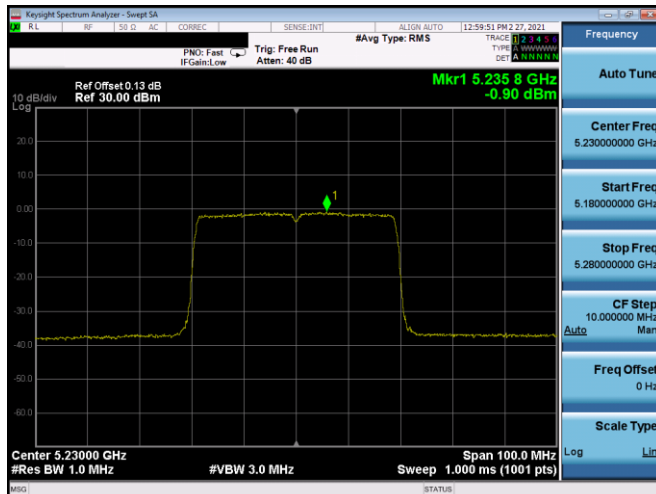
Plot 7-476. ISED PSD SDM Antenna 5B (40MHz BW 11ax(SU) – Ch.46, MCS0)
