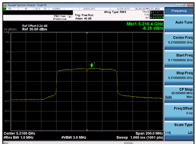
Plot 7-480. ISED PSD SDM Antenna 5B (80MHz BW 11ax (SU) – Ch.42, MCS0)
