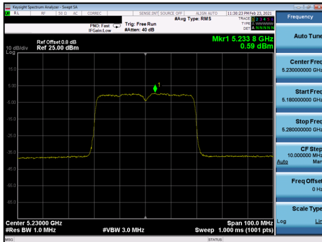
Plot 7-500. ISED PSD SDM Antenna 5B (40MHz BW 11ax(SU) – Ch.46, MCS11)
