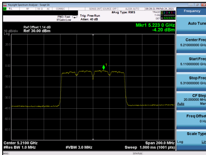
Plot 7-501. ISED PSD SDM Antenna 5T (80MHz BW 11ac – Ch.42, MCS5)
