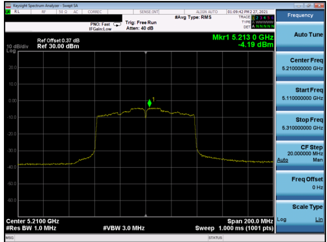
Plot 7-478. ISED PSD SDM Antenna 5B (80MHz BW 11ac – Ch.42, MCS0)
