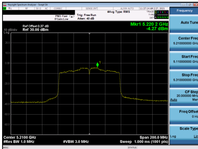
Plot 7-477. ISED PSD SDM Antenna 5T (80MHz BW 11ac – Ch.42, MCS0)
