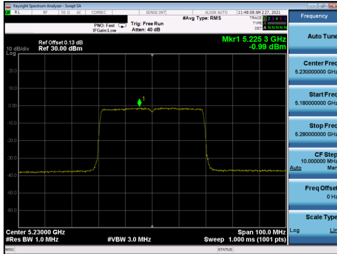
Plot 7-475. ISED PSD SDM Antenna 5T (40MHz BW 11ax(SU) – Ch.46, MCS0)
