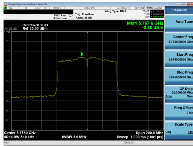
Plot 7-453. PSD CDD Antenna 5T (80MHz BW 802.11ac – Ch. 155, MCS3)
