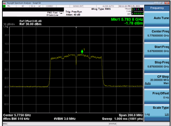
Plot 7-454. PSD CDD Antenna 5B (80MHz BW 802.11ac – Ch. 155, MCS3)
