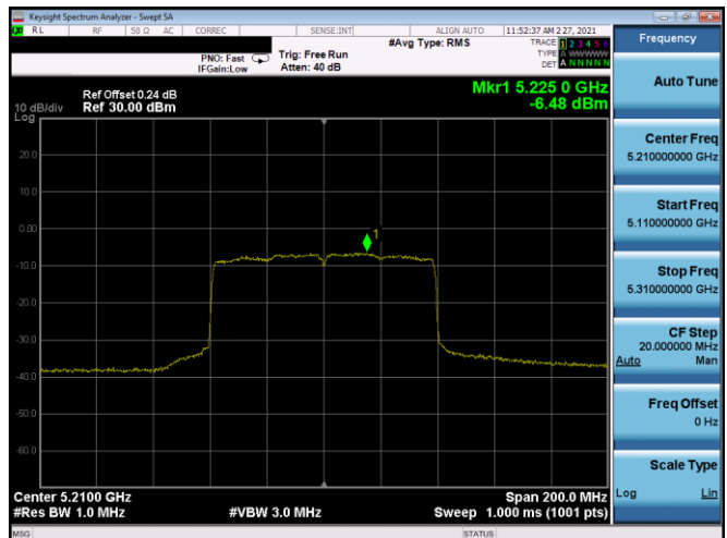
Plot 7-479. ISED PSD SDM Antenna 5T (80MHz BW 11ax (SU) – Ch.42, MCS0)
