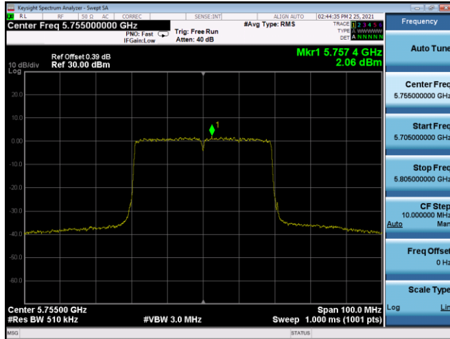
Plot 7-451. PSD CDD Antenna 5T (40MHz BW 802.11ax(SU) – Ch. 151, MCS3)
