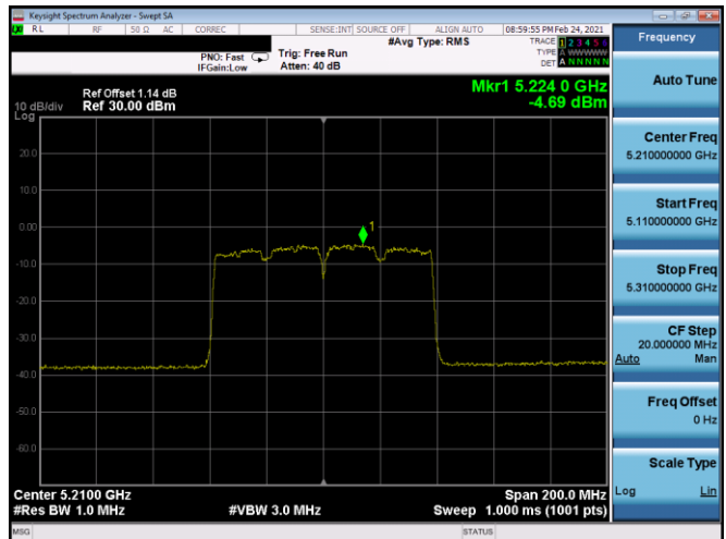
Plot 7-502. ISED PSD SDM Antenna 5B (80MHz BW 11ac – Ch.42, MCS5)
