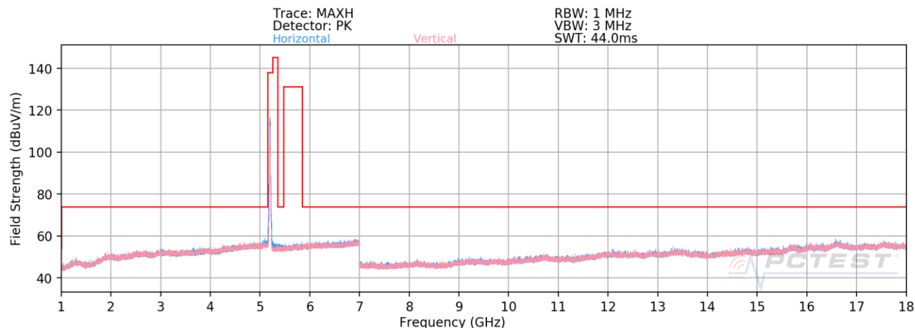
Plot 7-506. Radiated Spurious Emissions above 1GHz Antenna 5T (802.11n – Ch. 40)
