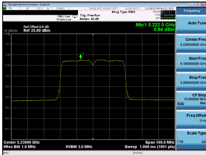
Plot 7-499. ISED PSD SDM Antenna 5T (40MHz BW 11ax(SU) – Ch.46, MCS11)
