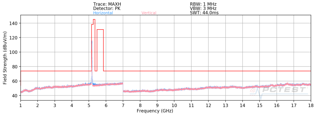
Plot 7-505. Radiated Spurious Emissions above 1GHz Antenna 5T (802.11n – Ch. 36)
