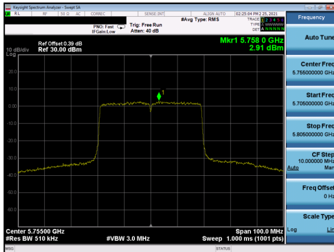
Plot 7-452. PSD CDD Antenna 5B (40MHz BW 802.11ax(SU) – Ch. 151, MCS3)
