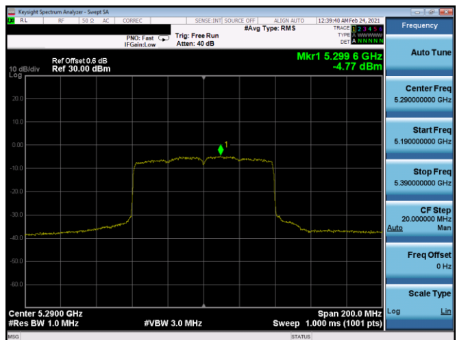
Plot 7-348. PSD CDD Antenna 5B (80MHz BW 802.11ax(SU) – Ch. 58, MCS0)
