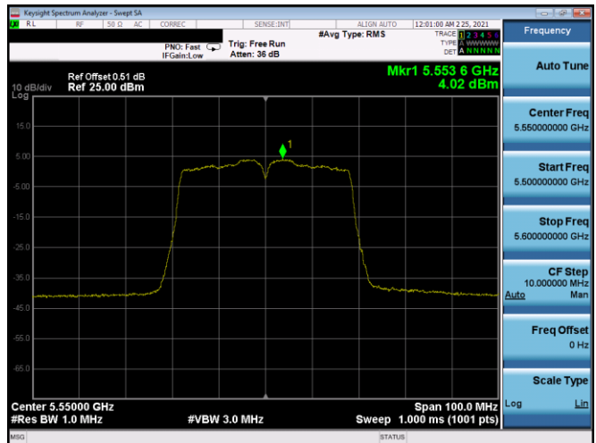
Plot 7-389. PSD SDM Antenna 5T (40MHz BW 802.11n – Ch. 110, MCS11)
