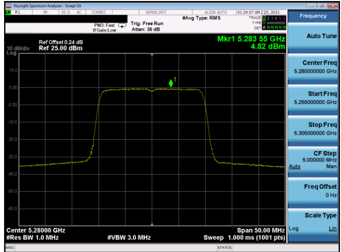
Plot 7-376. PSD SDM Antenna 5B (20MHz BW 802.11ax(SU) – Ch. 56, MCS3)
