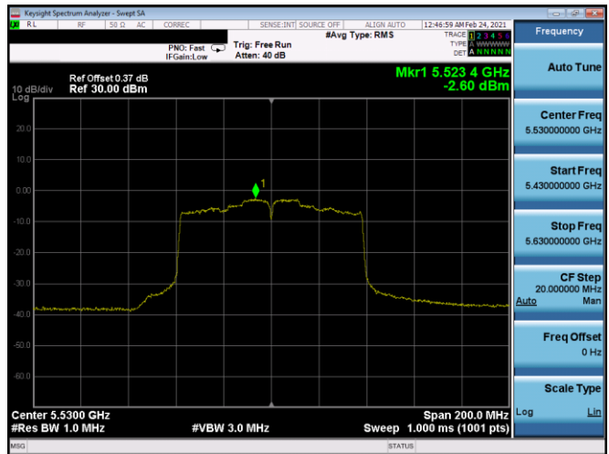
Plot 7-358. PSD CDD Antenna 5B (80MHz BW 802.11ac – Ch. 106, MCS0)
