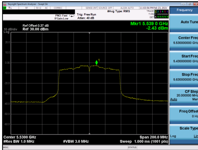
Plot 7-357. PSD CDD Antenna 5T (80MHz BW 802.11ac – Ch. 106, MCS0)
