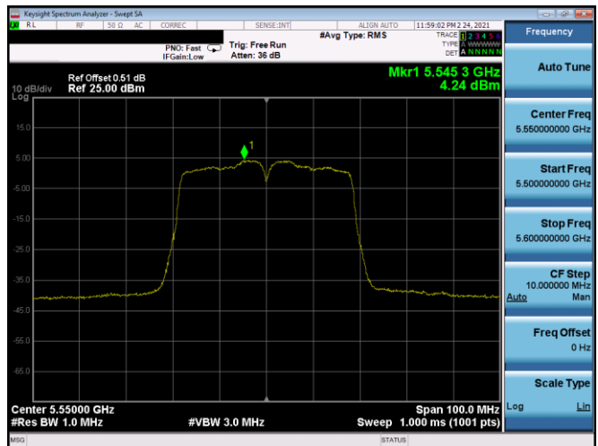
Plot 7-390. PSD SDM Antenna 5B (40MHz BW 802.11n – Ch. 110, MCS11)
