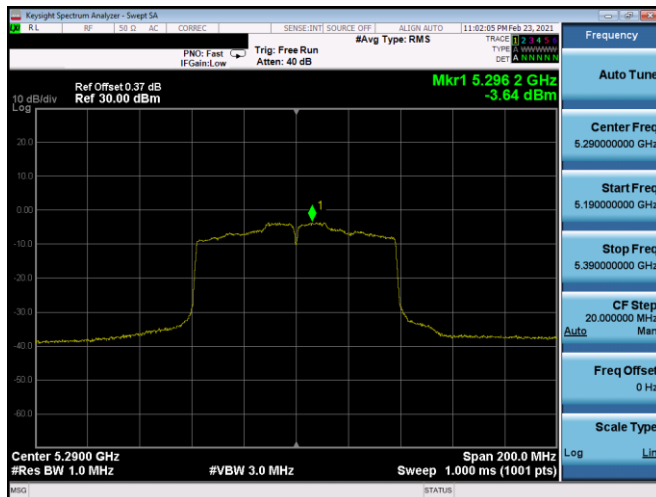
Plot 7-345. PSD CDD Antenna 5T (80MHz BW 802.11ac – Ch. 58, MCS0)
