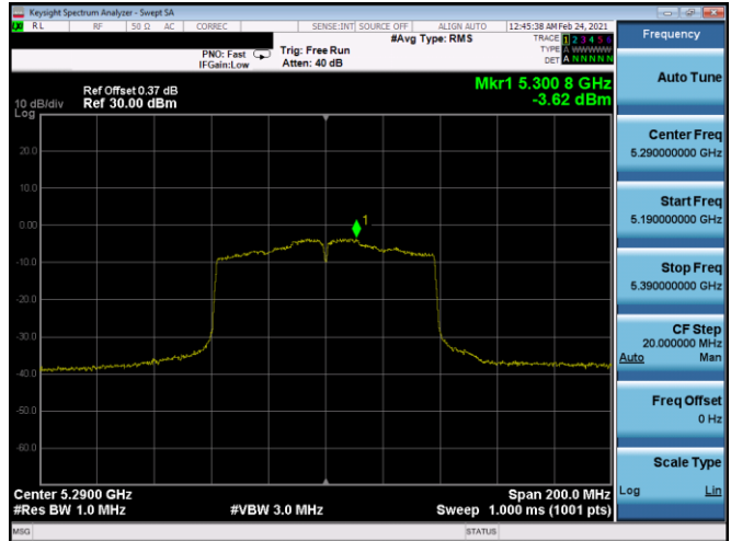
Plot 7-346. PSD CDD Antenna 5B (80MHz BW 802.11ac – Ch. 58, MCS0)
