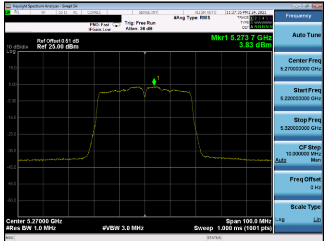
Plot 7-377. PSD SDM Antenna 5T (40MHz BW 802.11n – Ch. 54, MCS11)
