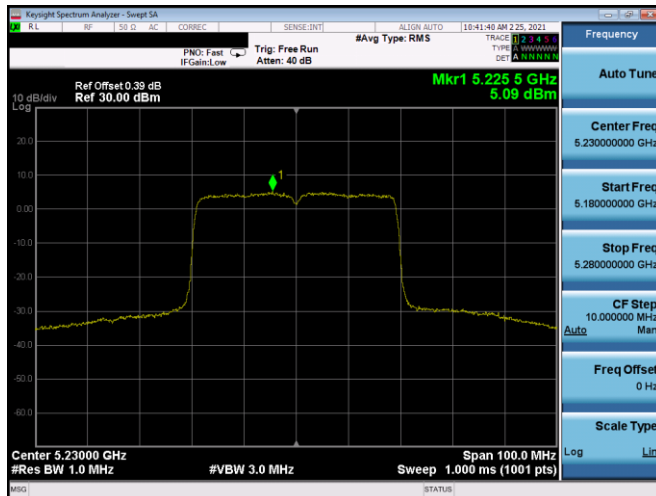
Plot 7-368. PSD SDM Antenna 5B (40MHz BW 802.11ax(SU) – Ch. 46, MCS3)
