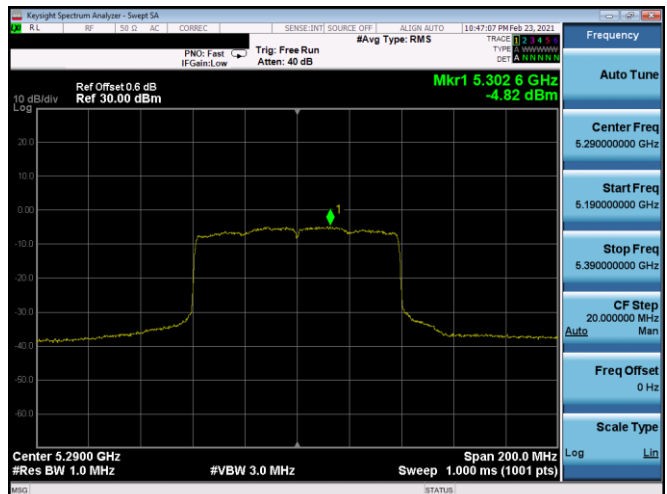
Plot 7-347. PSD CDD Antenna 5T (80MHz BW 802.11ax(SU) – Ch. 58, MCS0)
