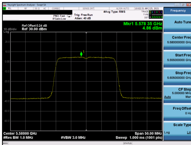
Plot 7-387. PSD SDM Antenna 5T (20MHz BW 802.11ax(SU) – Ch. 116, MCS3)
