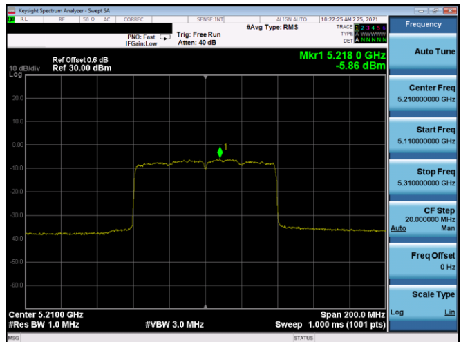
Plot 7-371. PSD CDD Antenna 5T (80MHz BW 802.11ax(SU) – Ch. 42, MCS3)
