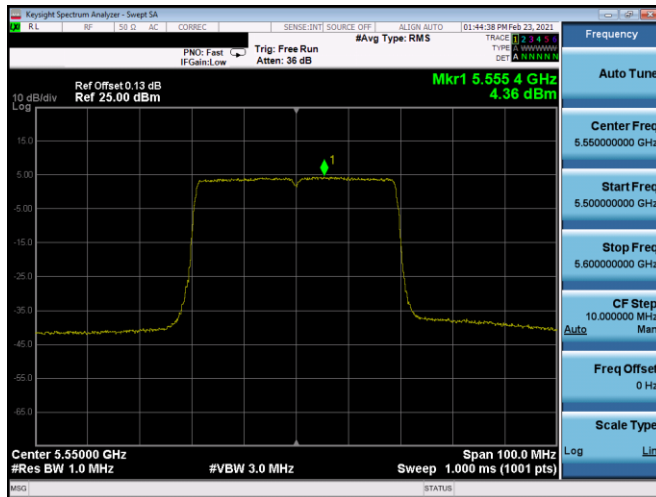
Plot 7-355. PSD SDM Antenna 5T (40MHz BW 802.11ax(SU) – Ch. 110, MCS0)
