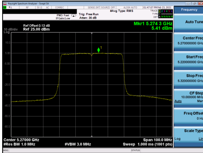
Plot 7-343. PSD SDM Antenna 5T (40MHz BW 802.11ax(SU) – Ch. 54, MCS0)
