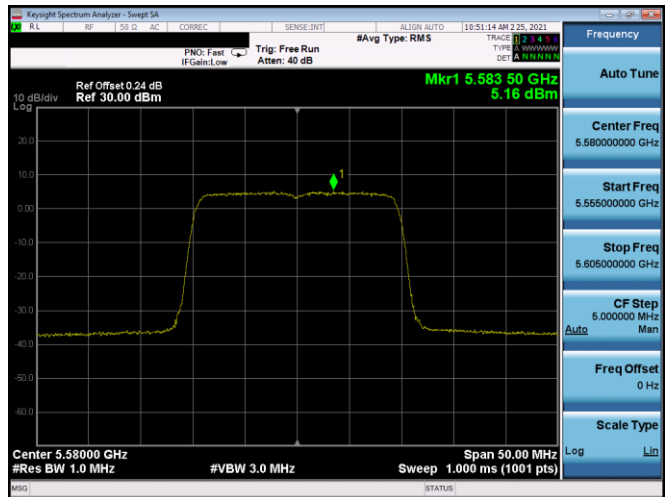
Plot 7-388. PSD SDM Antenna 5B (20MHz BW 802.11ax(SU) – Ch. 116, MCS3)
