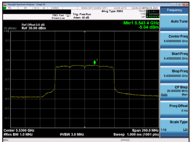
Plot 7-360. PSD CDD Antenna 5B (80MHz BW 802.11ax(SU) – Ch. 106, MCS0)
