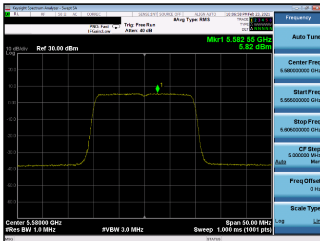
Plot 7-351. PSD SDM Antenna 5T (20MHz BW 802.11ax(SU) – Ch. 116, MCS0)
