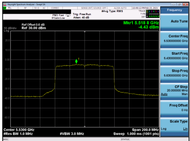
Plot 7-359. PSD CDD Antenna 5T (80MHz BW 802.11ax(SU) – Ch. 106, MCS0)
