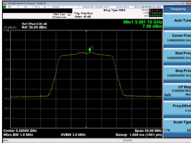
Plot 7-349. PSD SDM Antenna 5T (20MHz BW 802.11n – Ch. 116, MCS8)
