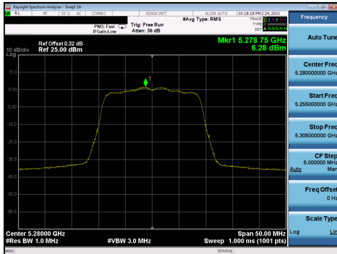
Plot 7-374. PSD SDM Antenna 5B (20MHz BW 802.11n – Ch. 56, MCS11)
