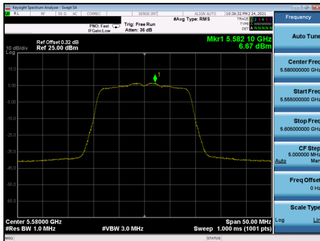
Plot 7-386. PSD SDM Antenna 5B (20MHz BW 802.11n – Ch. 116, MCS11)
