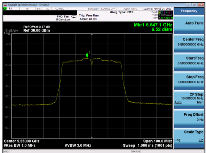
Plot 7-354. PSD SDM Antenna 5B (40MHz BW 802.11n – Ch. 110, MCS8)
