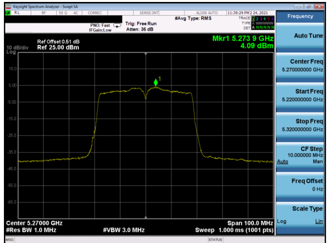
Plot 7-378. PSD SDM Antenna 5B (40MHz BW 802.11n – Ch. 54, MCS11)
