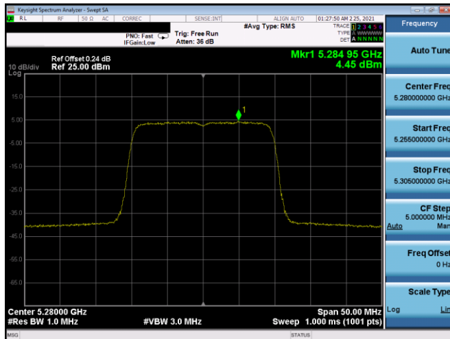
Plot 7-375. PSD SDM Antenna 5T (20MHz BW 802.11ax(SU) – Ch. 56, MCS3)
