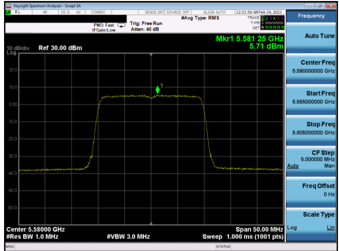
Plot 7-352. PSD SDM Antenna 5B (20MHz BW 802.11ax(SU) – Ch. 116, MCS0)
