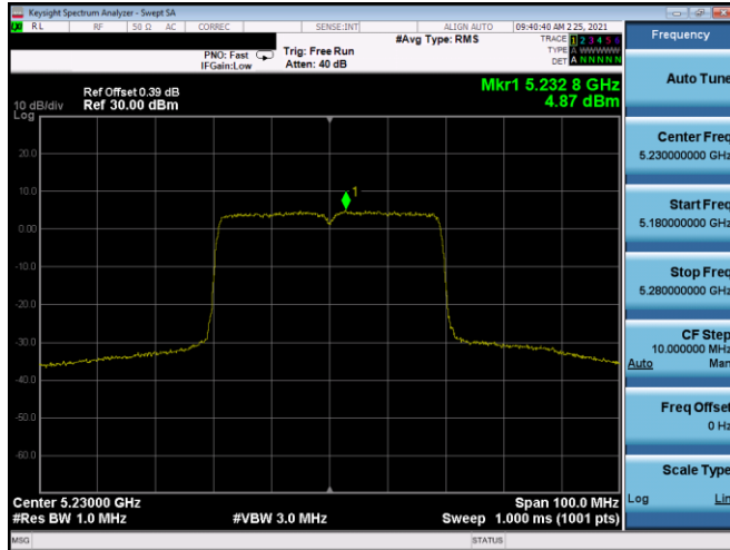
Plot 7-367. PSD SDM Antenna 5T (40MHz BW 802.11ax(SU) – Ch. 46, MCS3)
