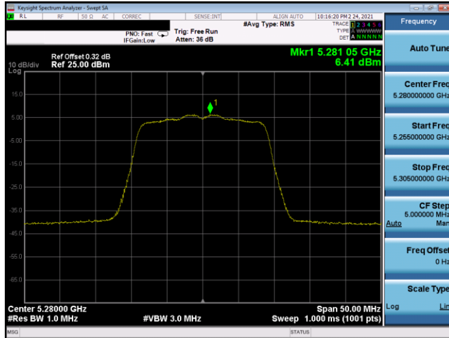
Plot 7-373. PSD SDM Antenna 5T (20MHz BW 802.11n – Ch. 56, MCS11)
