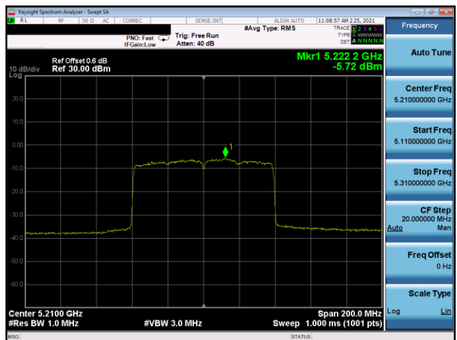
Plot 7-372. PSD CDD Antenna 5B (80MHz BW 802.11ax(SU) – Ch. 42, MCS3)
