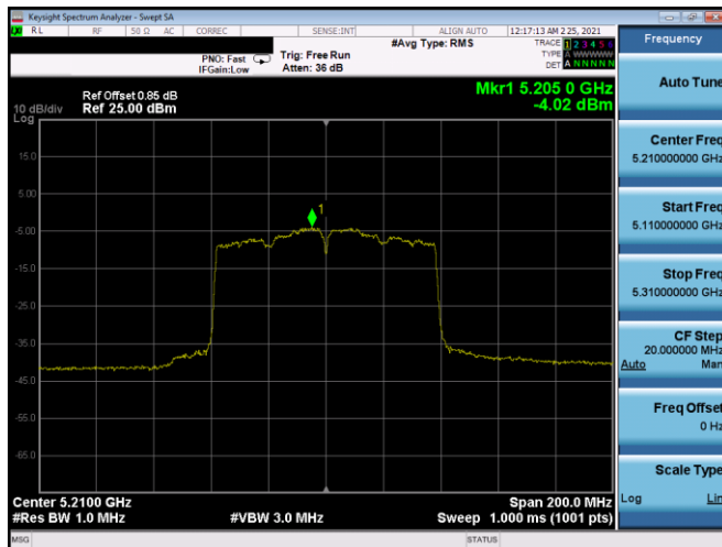
Plot 7-369. PSD CDD Antenna 5T (80MHz BW 802.11ac – Ch. 42, MCS3)
