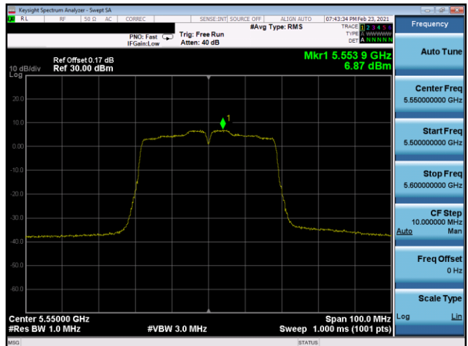
Plot 7-353. PSD SDM Antenna 5T (40MHz BW 802.11n – Ch. 110, MCS8)
