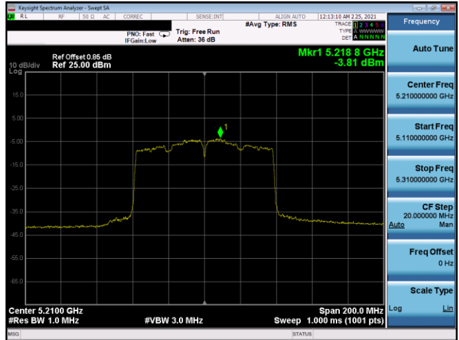
Plot 7-370. PSD CDD Antenna 5B (80MHz BW 802.11ac – Ch. 42, MCS3)
