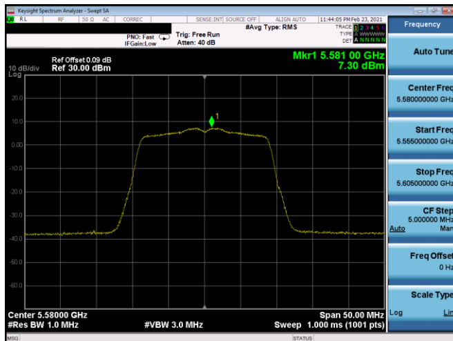
Plot 7-350. PSD SDM Antenna 5B (20MHz BW 802.11n – Ch. 116, MCS8)
