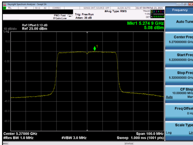
Plot 7-344. PSD SDM Antenna 5B (40MHz BW 802.11ax(SU) – Ch. 54, MCS0)
