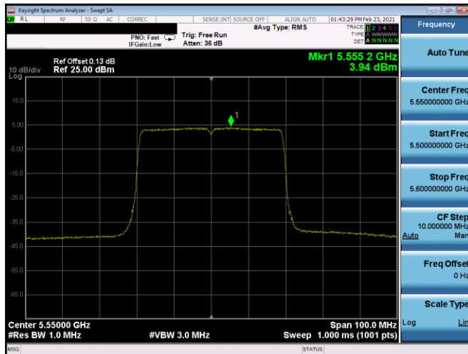
Plot 7-356. PSD SDM Antenna 5B (40MHz BW 802.11ax(SU) – Ch. 110, MCS0)
