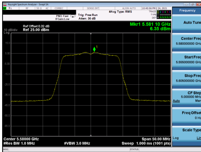
Plot 7-385. PSD SDM Antenna 5T (20MHz BW 802.11n – Ch. 116, MCS11)
