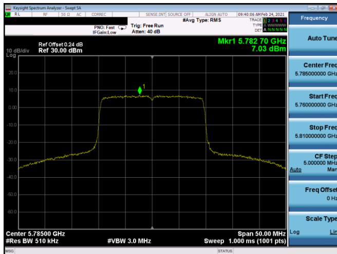
Plot 7-206. PSD Antenna 5T (20MHz BW 802.11ax(SU) – Ch. 157, MCS3)
