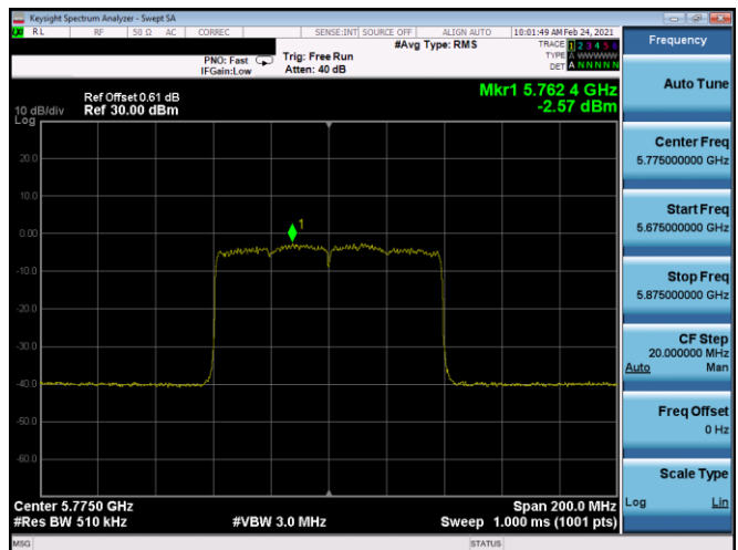
Plot 7-210. PSD Antenna 5T (80MHz BW 802.11ax(SU) – Ch. 155, MCS3)
