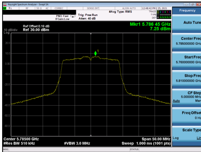
Plot 7-205. PSD Antenna 5T (20MHz BW 802.11n – Ch. 157, MCS3)
