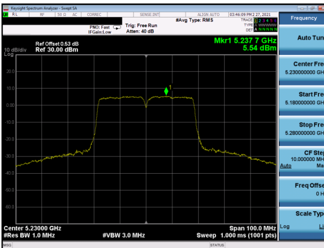
Plot 7-183. PSD Antenna 5T (40MHz BW 802.11n – Ch. 46, MCS5)
