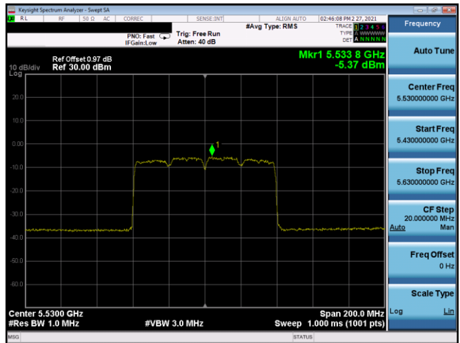
Plot 7-198. PSD Antenna 5T (80MHz BW 802.11ax(SU) – Ch. 106, MCS11)
