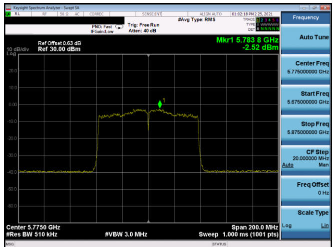
Plot 7-209. PSD Antenna 5T (80MHz BW 802.11ac – Ch. 155, MCS3)
