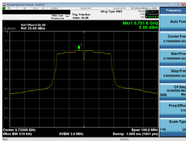
Plot 7-201. PSD Antenna 5T (40MHz BW 802.11n – Ch. 151, MCS0)
