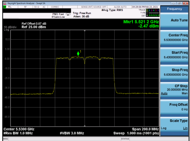
Plot 7-197. PSD Antenna 5T (80MHz BW 802.11ac – Ch. 106, MCS5)
