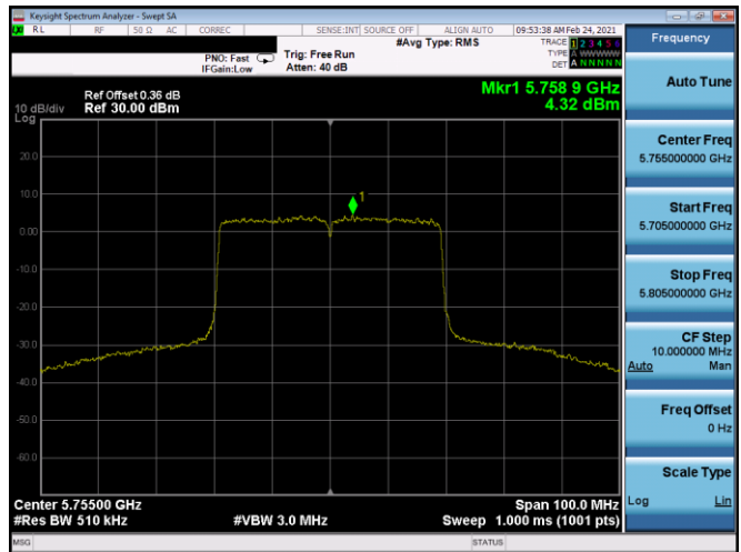
Plot 7-208. PSD Antenna 5T (40MHz BW 802.11ax(SU) – Ch. 151, MCS3)
