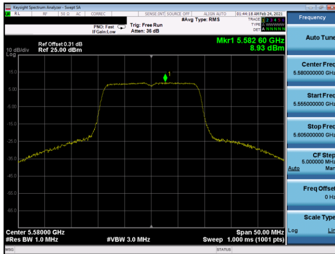
Plot 7-193. PSD Antenna 5T (20MHz BW 802.11n – Ch. 116, MCS5)
