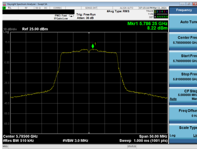
Plot 7-199. PSD Antenna 5T (20MHz BW 802.11n – Ch. 157, MCS0)
