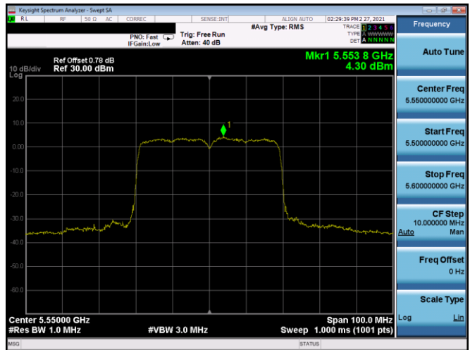
Plot 7-196. PSD Antenna 5T (40MHz BW 802.11ax(SU) – Ch. 110, MCS11)
