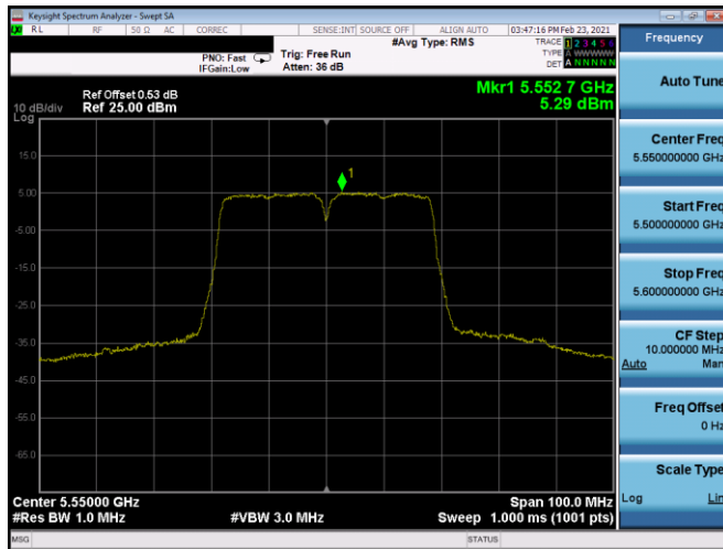
Plot 7-195. PSD Antenna 5T (40MHz BW 802.11n – Ch. 110, MCS5)
