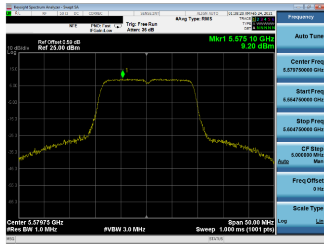
Plot 7-194. PSD Antenna 5T (20MHz BW 802.11ax(SU) – Ch. 116, MCS11)
