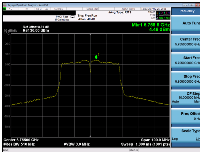
Plot 7-207. PSD Antenna 5T (40MHz BW 802.11n – Ch. 151, MCS3)
