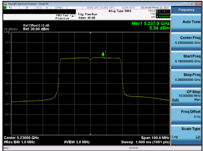
Plot 7-148. PSD Antenna 5T (40MHz BW 802.11ax(SU) – Ch. 46, MCS0)
