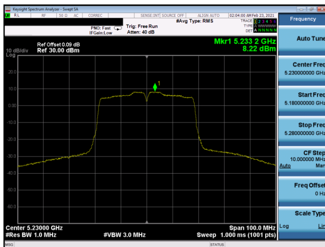
Plot 7-147. PSD Antenna 5T (40MHz BW 802.11n – Ch. 46, MCS0)
