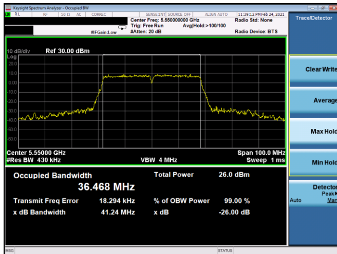
Plot 7-105. 26dB BW & 99% OBW Antenna 5B (40MHz BW 802.11n – Ch. 110, MCS5)
