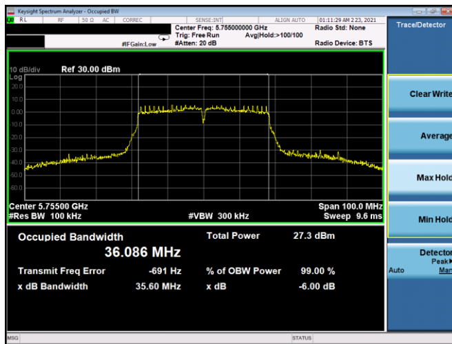
Plot 7-111. 6dB BW & 99% OBW Antenna 5T (40MHz BW 802.11n – Ch. 151, MCS0)
