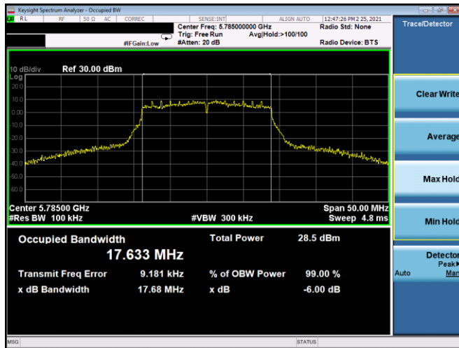
Plot 7-115. 6dB BW & 99% OBW Antenna 5T (20MHz BW 802.11n – Ch. 157, MCS3)
