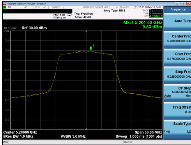
Plot 7-145. PSD Antenna 5T (20MHz BW 802.11n – Ch. 40, MCS0)
