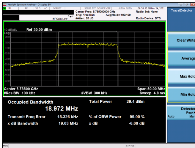
Plot 7-116. 6dB BW & 99% OBW Antenna 5T (20MHz BW 802.11ax(SU) – Ch. 157, MCS3)
