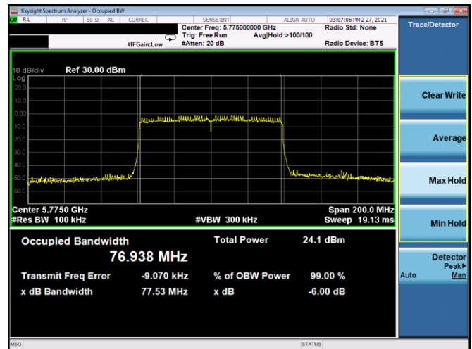
Plot 7-126. 6dB BW & 99% OBW Antenna 5T (80MHz BW 802.11ax(SU) – Ch. 155, MCS11)
