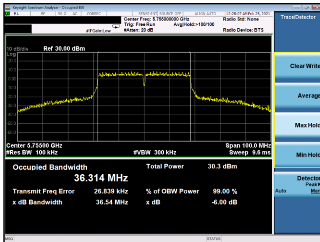
Plot 7-141. 6dB BW & 99% OBW Antenna 5B (40MHz BW 802.11n – Ch. 151, MCS5)
