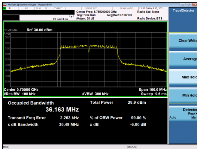
Plot 7-117. 6dB BW & 99% OBW Antenna 5T (40MHz BW 802.11n – Ch. 151, MCS3)
