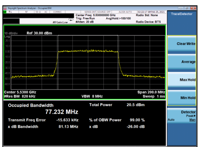
Plot 7-108. 26dB BW & 99% OBW Antenna 5B (80MHz BW 802.11ax(SU) – Ch. 106, MCS11)
