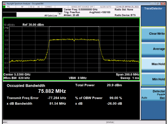
Plot 7-107. 26dB BW & 99% OBW Antenna 5B (80MHz BW 802.11ac – Ch. 106, MCS5)
