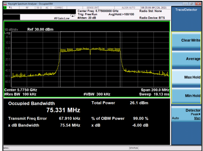
Plot 7-131. 6dB BW & 99% OBW Antenna 5B (80MHz BW 802.11ac – Ch. 155, MCS0)
