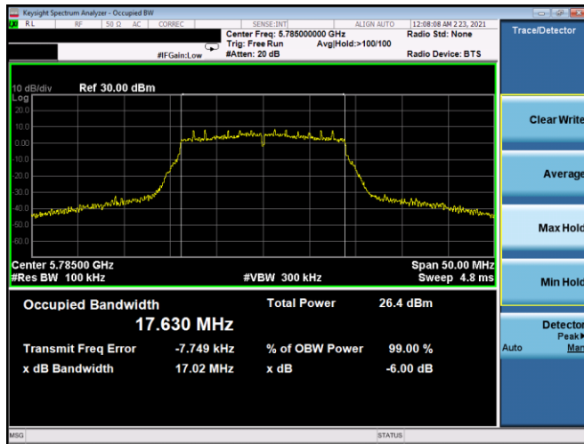
Plot 7-109. 6dB BW & 99% OBW Antenna 5T (20MHz BW 802.11n – Ch. 157, MCS0)
