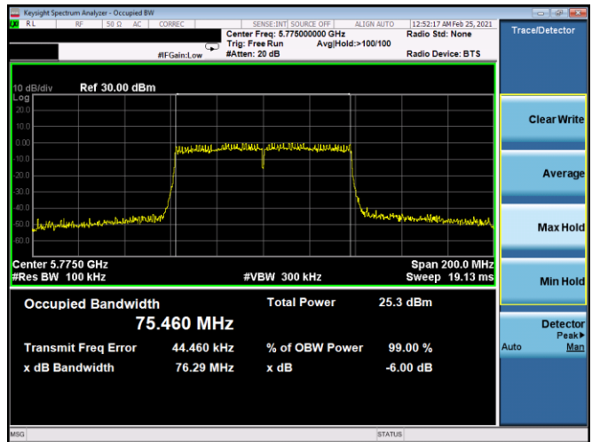
Plot 7-143. 6dB BW & 99% OBW Antenna 5B (80MHz BW 802.11ac – Ch. 155, MCS5)
