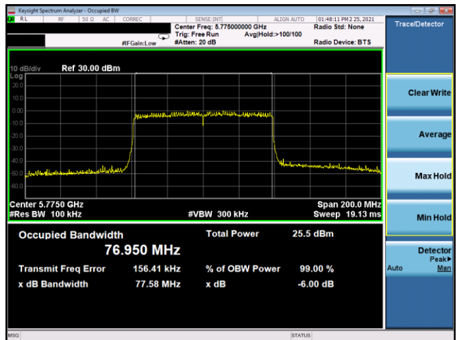
Plot 7-138. 6dB BW & 99% OBW Antenna 5B (80MHz BW 802.11ax(SU) – Ch. 155, MCS3)
