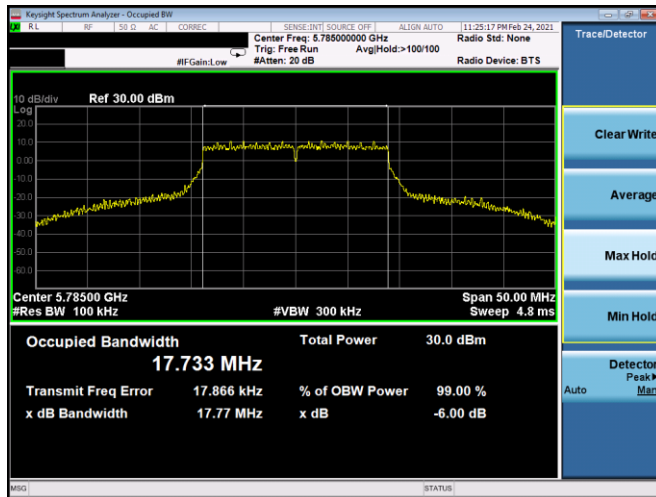
Plot 7-139. 6dB BW & 99% OBW Antenna 5B (20MHz BW 802.11n – Ch. 157, MCS5)
