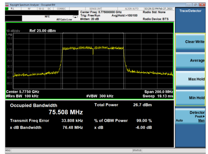
Plot 7-125. 6dB BW & 99% OBW Antenna 5T (80MHz BW 802.11ac – Ch. 155, MCS5)
