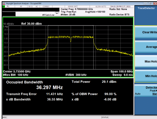
Plot 7-123. 6dB BW & 99% OBW Antenna 5T (40MHz BW 802.11n – Ch. 151, MCS5)
