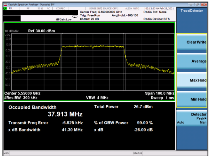
Plot 7-106. 26dB BW & 99% OBW Antenna 5B (40MHz BW 802.11ax(SU) – Ch. 110, MCS11)
