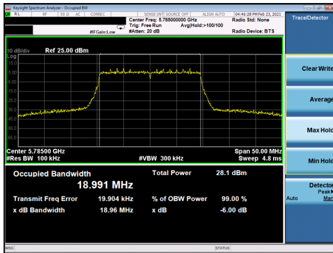
Plot 7-110. 6dB BW & 99% OBW Antenna 5T (20MHz BW 802.11ax(SU) – Ch. 157, MCS0)
