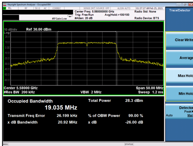
Plot 7-104. 26dB BW & 99% OBW Antenna 5B (20MHz BW 802.11ax(SU) – Ch. 116, MCS11)
