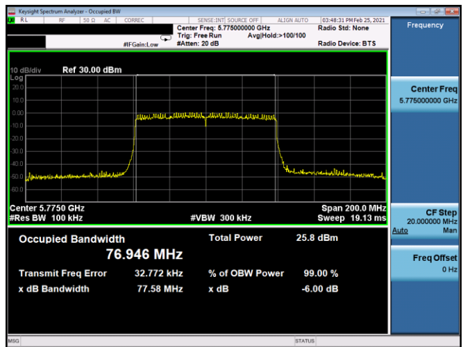
Plot 7-114. 6dB BW & 99% OBW Antenna 5T (80MHz BW 802.11ax(SU) – Ch. 155, MCS0)
