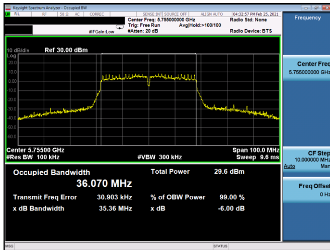
Plot 7-129. 6dB BW & 99% OBW Antenna 5B (40MHz BW 802.11n – Ch. 151, MCS0)
