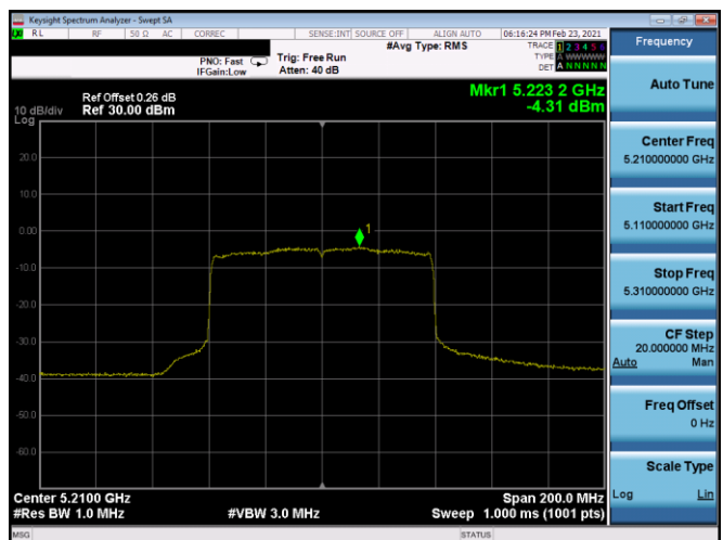
Plot 7-150. PSD Antenna 5T (80MHz BW 802.11ax(SU) – Ch. 42, MCS0)
