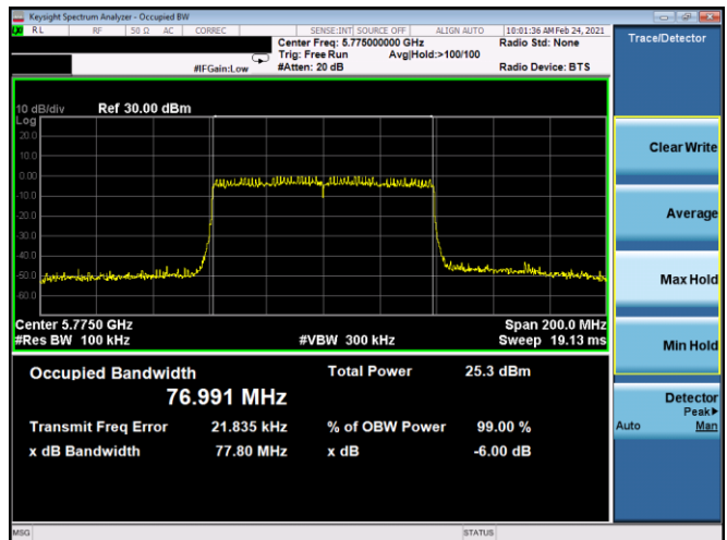
Plot 7-120. 6dB BW & 99% OBW Antenna 5T (80MHz BW 802.11ax(SU) – Ch. 155, MCS3)
