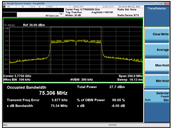
Plot 7-113. 6dB BW & 99% OBW Antenna 5T (80MHz BW 802.11ac – Ch. 155, MCS0)
