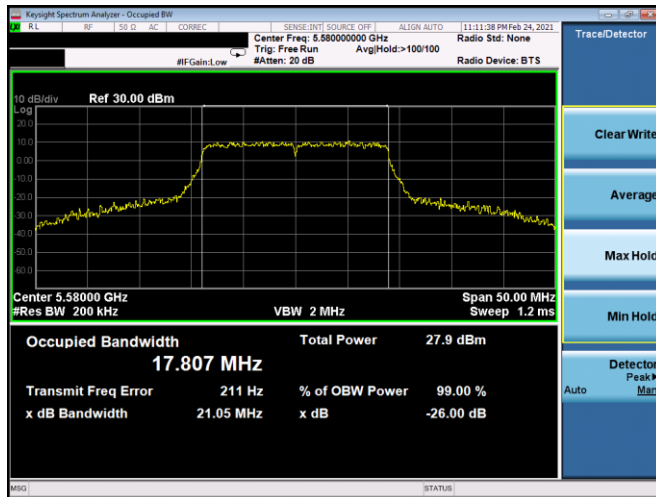
Plot 7-103. 26dB BW & 99% OBW Antenna 5B (20MHz BW 802.11n – Ch. 116, MCS5)
