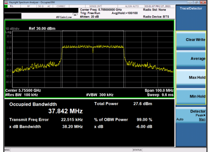
Plot 7-124. 6dB BW & 99% OBW Antenna 5T (40MHz BW 802.11ax(SU) – Ch. 151, MCS11)
