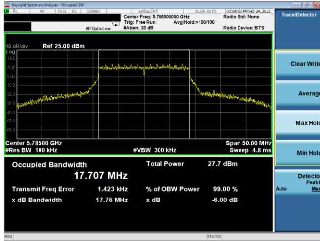
Plot 7-121. 6dB BW & 99% OBW Antenna 5T (20MHz BW 802.11n – Ch. 157, MCS5)
