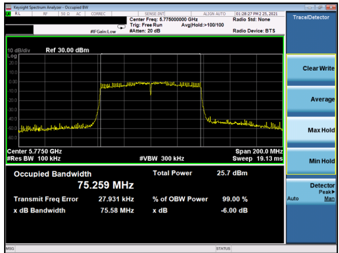
Plot 7-137. 6dB BW & 99% OBW Antenna 5B (80MHz BW 802.11ac – Ch. 155, MCS3)
