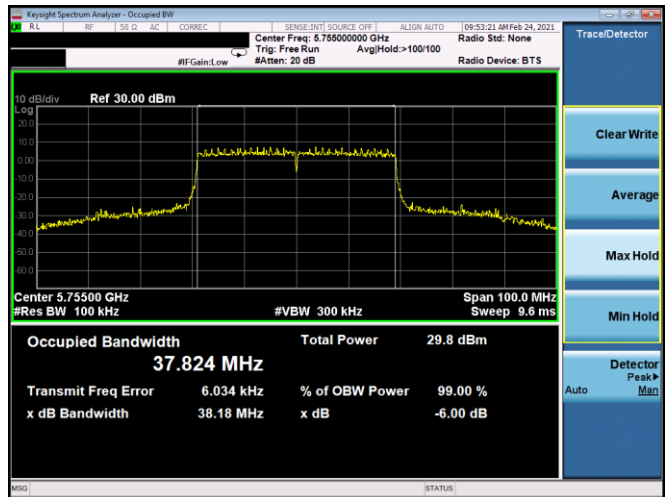
Plot 7-118. 6dB BW & 99% OBW Antenna 5T (40MHz BW 802.11ax(SU) – Ch. 151, MCS3)
