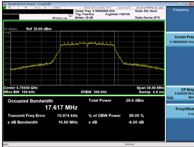
Plot 7-127. 6dB BW & 99% OBW Antenna 5B (20MHz BW 802.11n – Ch. 157, MCS0)
