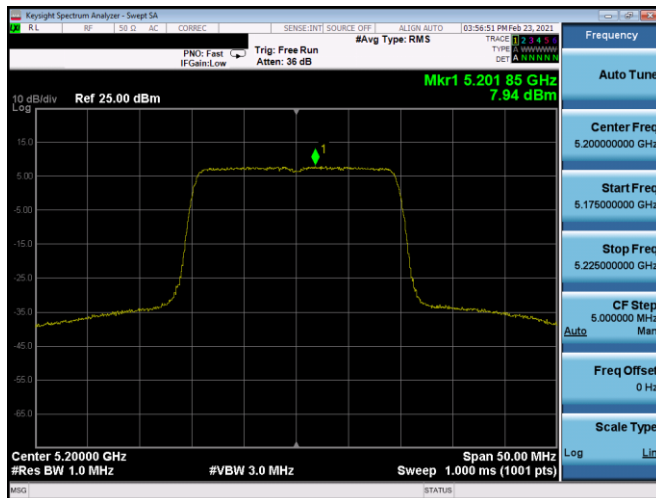
Plot 7-146. PSD Antenna 5T (20MHz BW 802.11ax(SU) – Ch. 40, MCS0)
