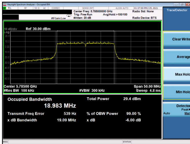
Plot 7-134. 6dB BW & 99% OBW Antenna 5B (20MHz BW 802.11ax(SU) – Ch. 157, MCS3)
