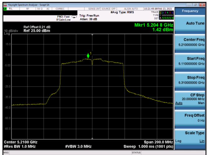
Plot 7-149. PSD Antenna 5T (80MHz BW 802.11ac – Ch. 42, MCS0)
