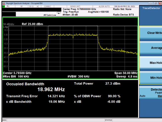
Plot 7-122. 6dB BW & 99% OBW Antenna 5T (20MHz BW 802.11ax(SU) – Ch. 157, MCS11)
