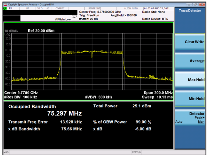
Plot 7-119. 6dB BW & 99% OBW Antenna 5T (80MHz BW 802.11ac – Ch. 155, MCS3)
