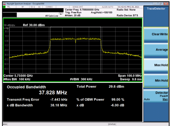
Plot 7-136. 6dB BW & 99% OBW Antenna 5B (40MHz BW 802.11ax (SU) – Ch. 151, MCS3)
