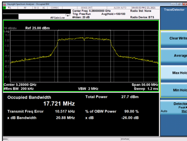
Plot 7-25. 26dB BW & 99% OBW Antenna 5T (20MHz BW 802.11n – Ch. 56, MCS3)
