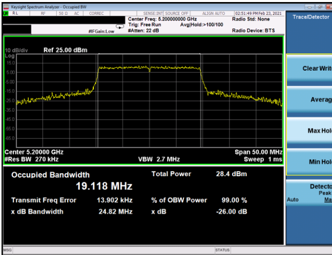
Plot 7-38. 26dB BW & 99% OBW Antenna 5T (20MHz BW 802.11ax(SU) – Ch. 40, MCS11)
