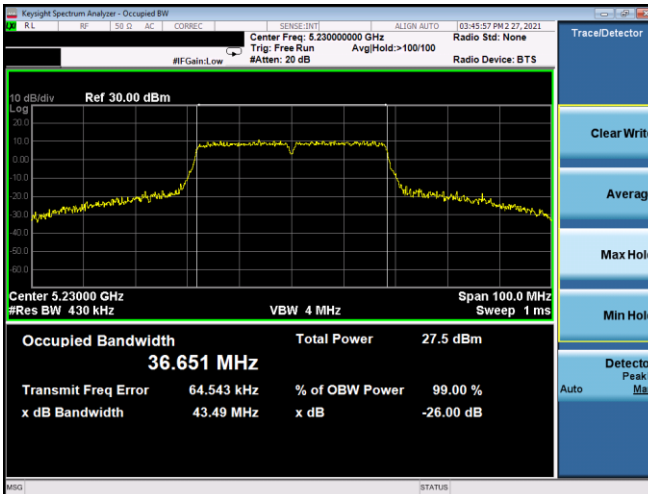
Plot 7-39. 26dB BW & 99% OBW Antenna 5T (40MHz BW 802.11n – Ch. 46, MCS5)
