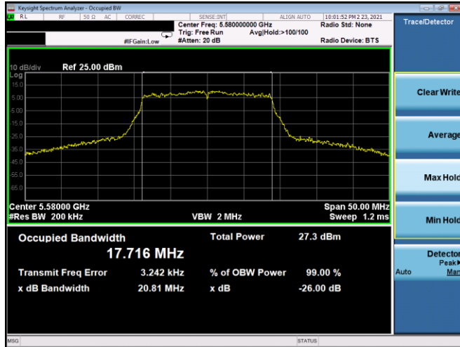
Plot 7-31. 26dB BW & 99% OBW Antenna 5T (20MHz BW 802.11n – Ch. 116, MCS3)
