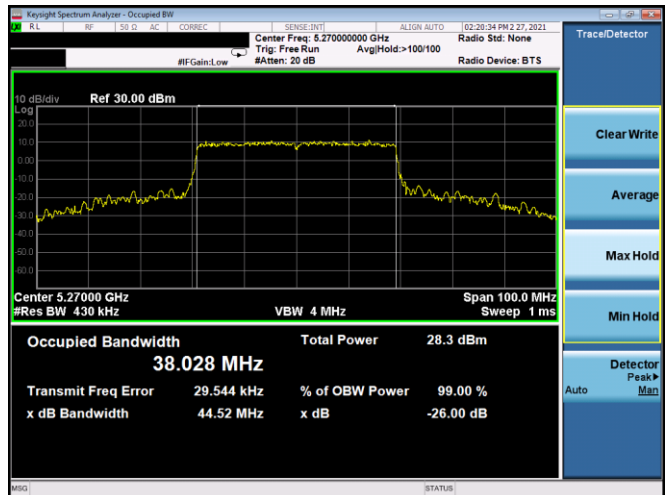
Plot 7-46. 26dB BW & 99% OBW Antenna 5T (40MHz BW 802.11ax(SU) – Ch. 54, MCS11)
