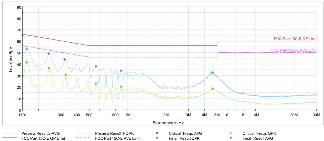
Plot 7-574. AC Line Conducted Plot with SDM 11ax UNII Band 1 – RU26 – Ch.40 (N) with AC/DC Adapter
