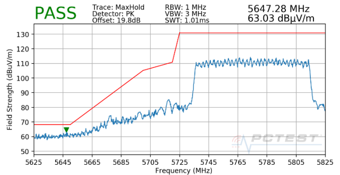
Plot 7-569. CDD (Pk, RU996, Index 67, Ch.155, MCS11)
