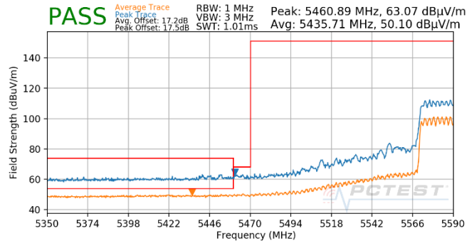
Plot 7-567. (FCC Only) CDD (Pk & Avg, RU996, Index 67, Ch.122, MCS11)
