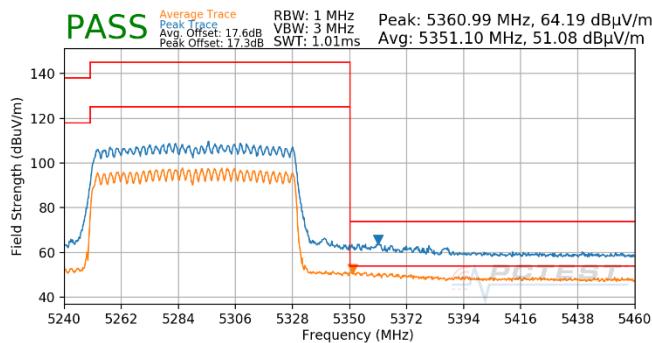
Plot 7-565. CDD (Pk & Avg, RU996, Index 67, Ch.58, MCS11)
