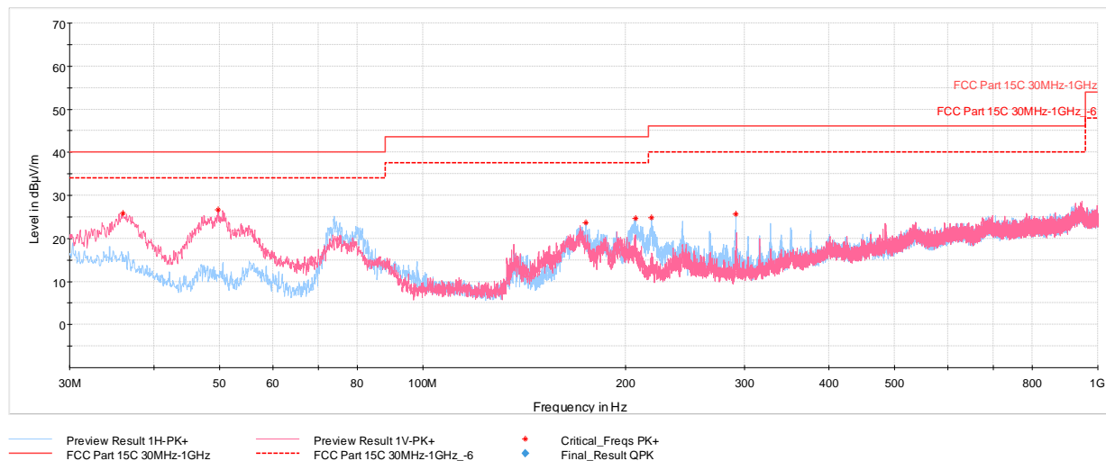
Plot 7-571. RSE below 1GHz SDM (RU26 – Ch.40), with AC/DC Adapter
