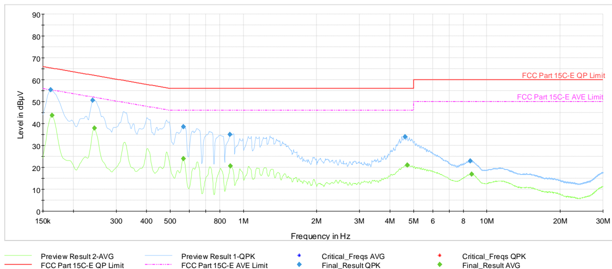
Plot 7-573. AC Line Conducted Plot with SDM 11ax UNII Band 1 – RU26 – Ch.40 (L1) with AC/DC Adapter
