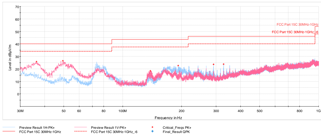
Plot 7-572. RSE below 1GHz SDM (RU242 – Ch.40), with AC/DC Adapter
