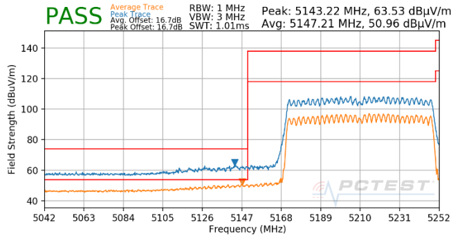
Plot 7-564. CDD (Pk & Avg, RU996, Index 67, Ch.42, MCS11)
