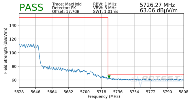
Plot 7-568. (FCC Only) CDD (Pk, RU996, Index 67, Ch.122, MCS11)
