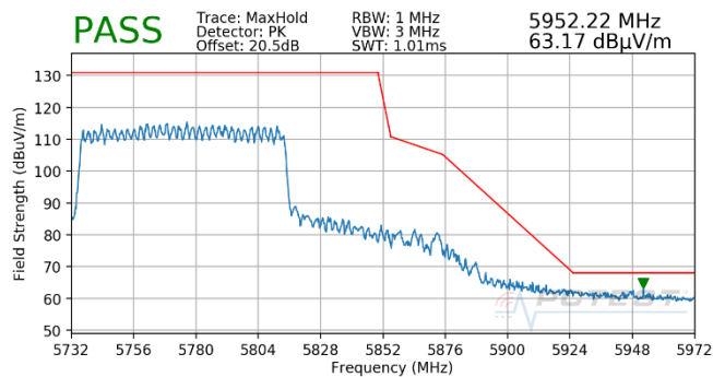
Plot 7-570. CDD (Pk, RU996, Index 67, Ch.155, MCS11)
