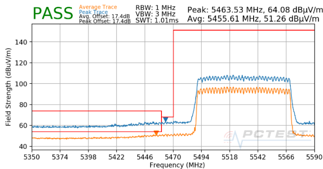
Plot 7-566. CDD (Pk & Avg, RU996, Index 67, Ch.106, MCS11)
