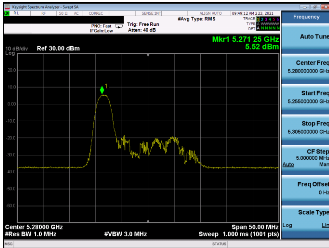
Plot 7-242. PSD SDM Antenna 5B (20MHz BW 11ax Index 0 - RU26 - Ch.56)
