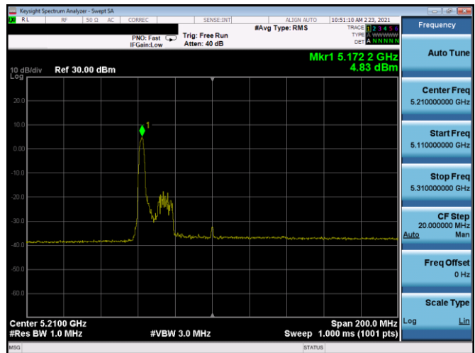
Plot 7-234. PSD SDM Antenna 5B (80MHz BW 11ax Index 0 – RU26 – Ch.42)
