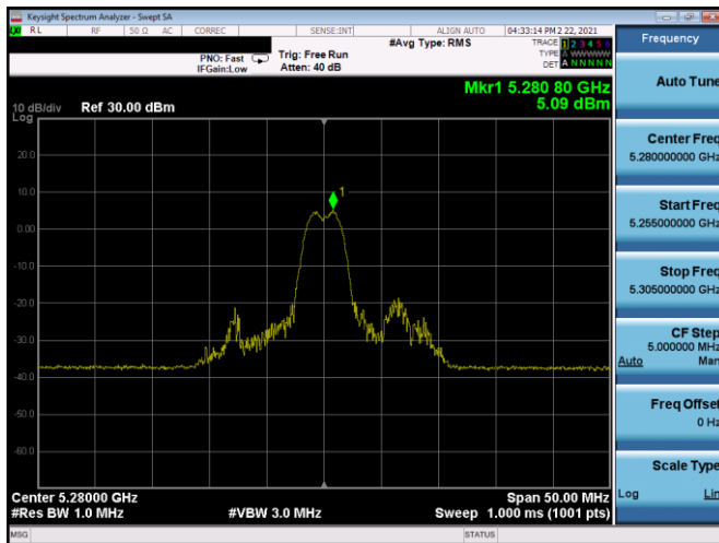
Plot 7-243. PSD SDM Antenna 5T (20MHz BW 11ax Index 4 - RU26 - Ch.56)
