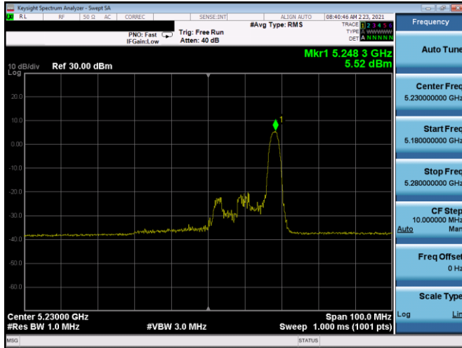
Plot 7-229. PSD SDM Antenna 5T (40MHz BW 11ax Index 17 – RU26 – Ch.46)
