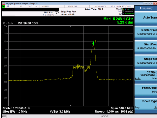
Plot 7-230. PSD SDM Antenna 5B (40MHz BW 11ax Index 17 – RU26 – Ch.46)
