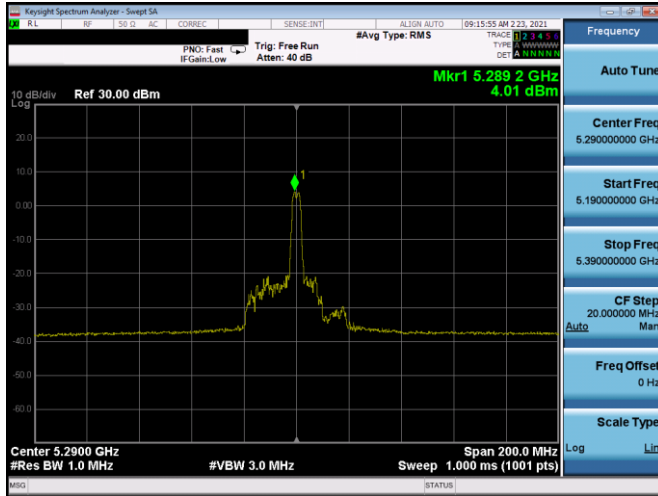
Plot 7-259. PSD SDM Antenna 5T (80MHz BW 11ax Index 18 – RU26 – Ch.58)
