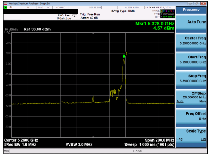
Plot 7-262. PSD SDM Antenna 5B (80MHz BW 11ax Index 36 – RU26 – Ch.58)
