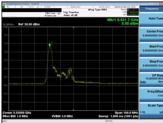
Plot 7-273. PSD SDM Antenna 5T (40MHz BW 11ax Index 0 - RU26 - Ch.110)
