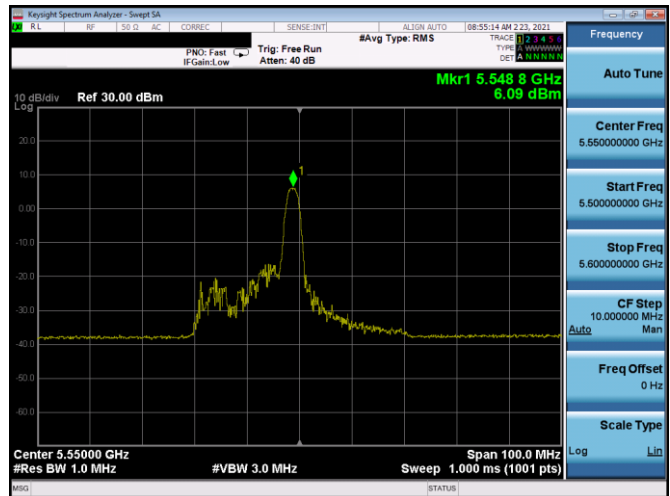
Plot 7-275. PSD SDM Antenna 5T (40MHz BW 11ax Index 8 - RU26 - Ch.110)
