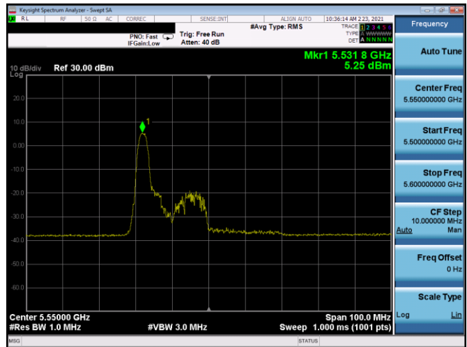
Plot 7-274. PSD SDM Antenna 5B (40MHz BW 11ax Index 0 - RU26 - Ch.110)
