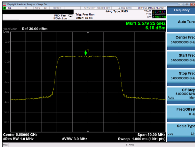
Plot 7-272. PSD SDM Antenna 5B (20MHz BW 11ax- RU242 - Ch.116)
