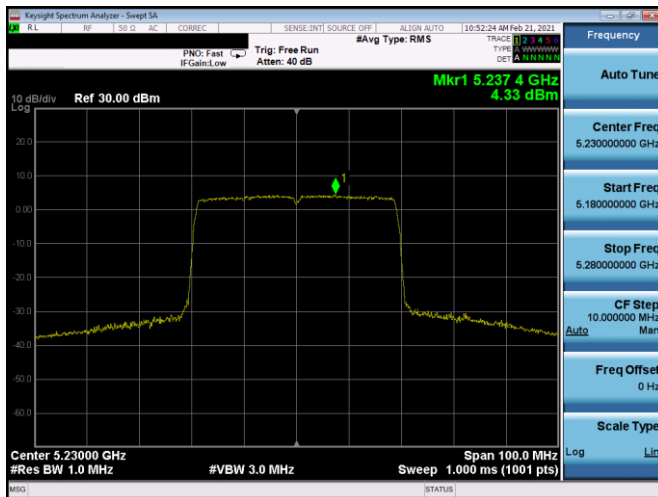
Plot 7-231. PSD CDD Antenna 5T (40MHz BW 11ax – RU484 – Ch.46)
