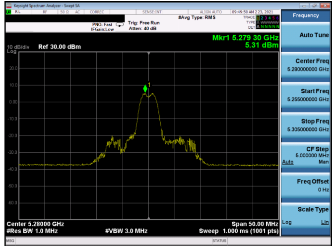
Plot 7-244. PSD SDM Antenna 5B (20MHz BW 11ax Index 4 - RU26 - Ch.56)
