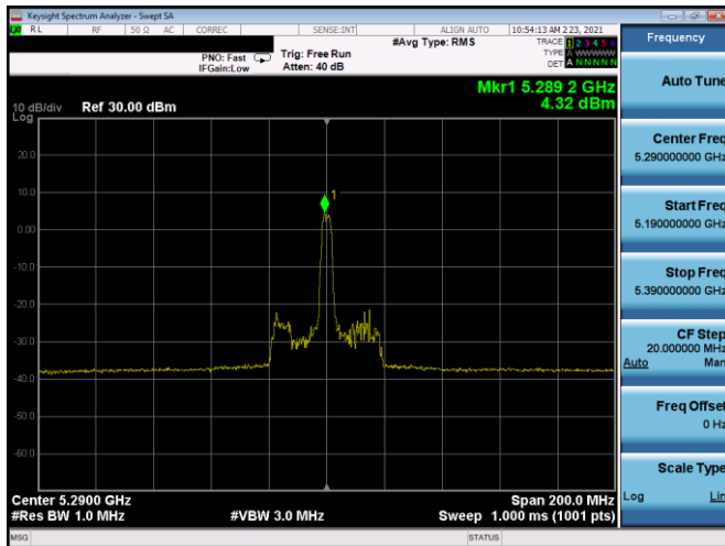
Plot 7-260. PSD SDM Antenna 5B (80MHz BW 11ax Index 18 – RU26 – Ch.58)
