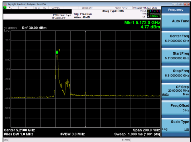
Plot 7-233. PSD SDM Antenna 5T (80MHz BW 11ax Index 0 – RU26 – Ch.42)
