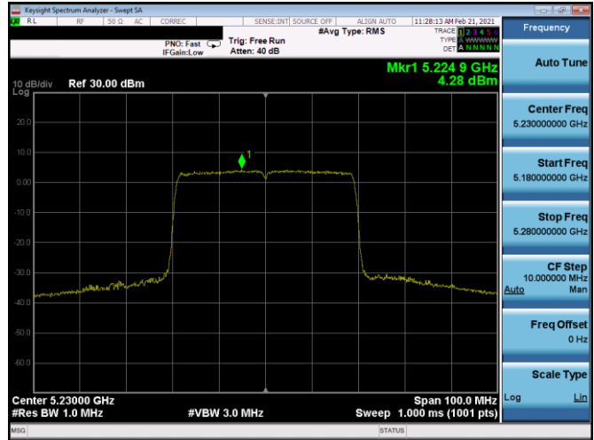
Plot 7-232. PSD CDD Antenna 5B (40MHz BW 11ax – RU484 – Ch.46)
