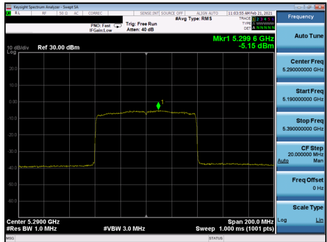
Plot 7-263. PSD CDD Antenna 5T (80MHz BW 11ax – RU996 – Ch.58)
