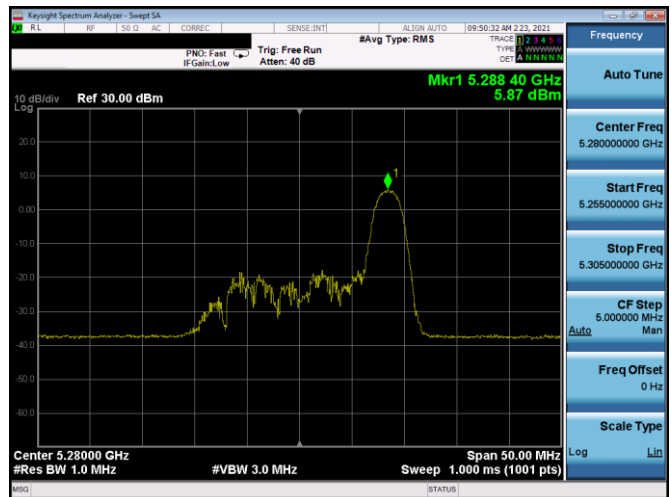
Plot 7-246. PSD SDM Antenna 5B (20MHz BW 11ax Index 8- RU26 - Ch.56)
