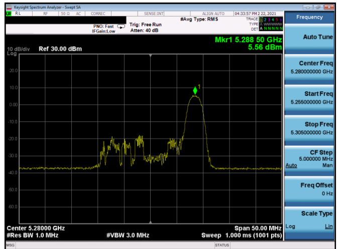
Plot 7-245. PSD SDM Antenna 5T (20MHz BW 11ax Index 8- RU26 - Ch.56)
