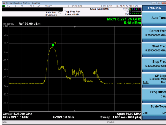
Plot 7-241. PSD SDM Antenna 5T (20MHz BW 11ax Index 0 - RU26 - Ch.56)
