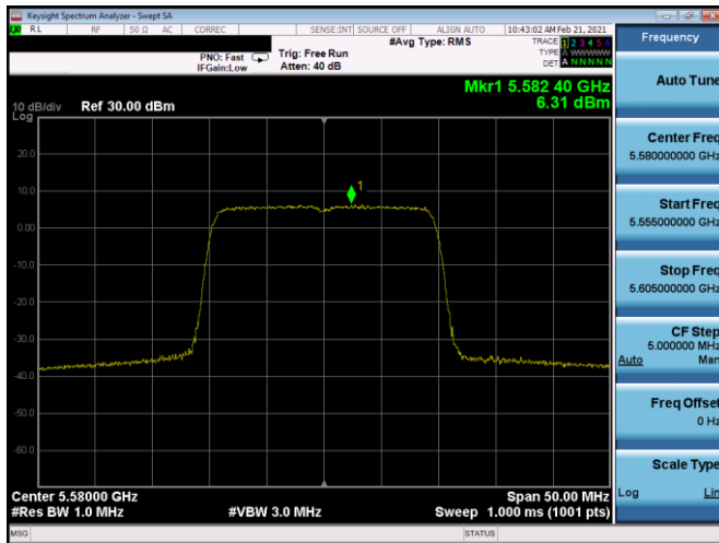
Plot 7-271. PSD SDM Antenna 5T (20MHz BW 11ax- RU242 - Ch.116)
