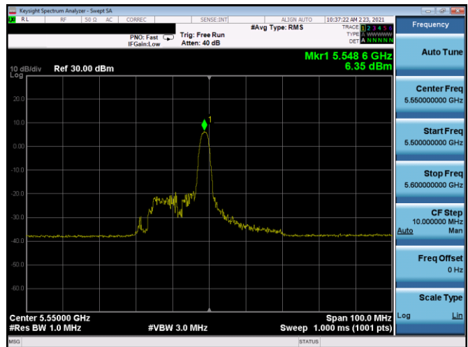
Plot 7-276. PSD SDM Antenna 5B (40MHz BW 11ax Index 8 - RU26 - Ch.110)
