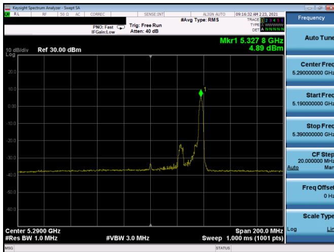
Plot 7-261. PSD SDM Antenna 5T (80MHz BW 11ax Index 36 – RU26 – Ch.58)
