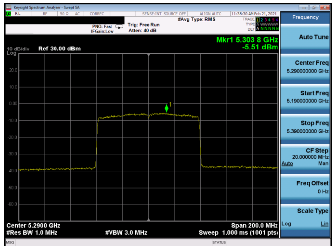
Plot 7-264. PSD CDD Antenna 5B (80MHz BW 11ax – RU996 – Ch.58)
