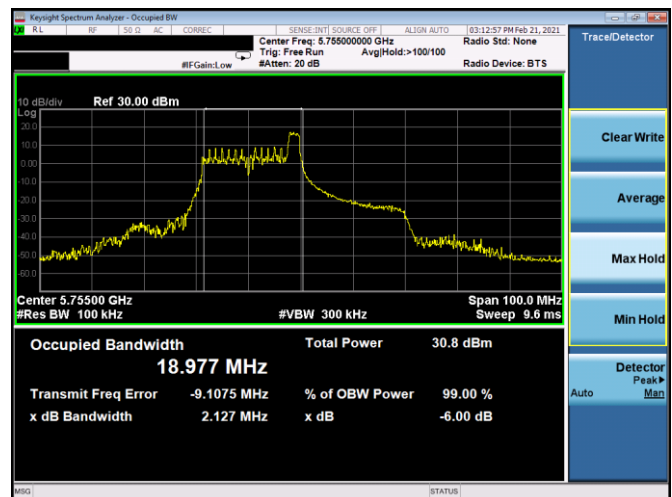
Plot 7-78. 6dB BW & 99% OBW Antenna 5T (40MHz BW 11ax Index 8 – RU26 – Ch.151)
