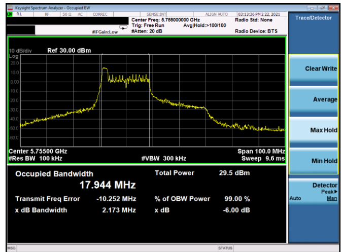
Plot 7-88. 6dB BW & 99% OBW Antenna 5B (40MHz BW 11ax Index 0 – RU26 – Ch.151)
