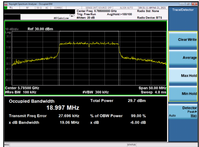
Plot 7-86. 6dB BW & 99% OBW Antenna 5B (20MHz BW 11ax – RU242 – Ch.157)
