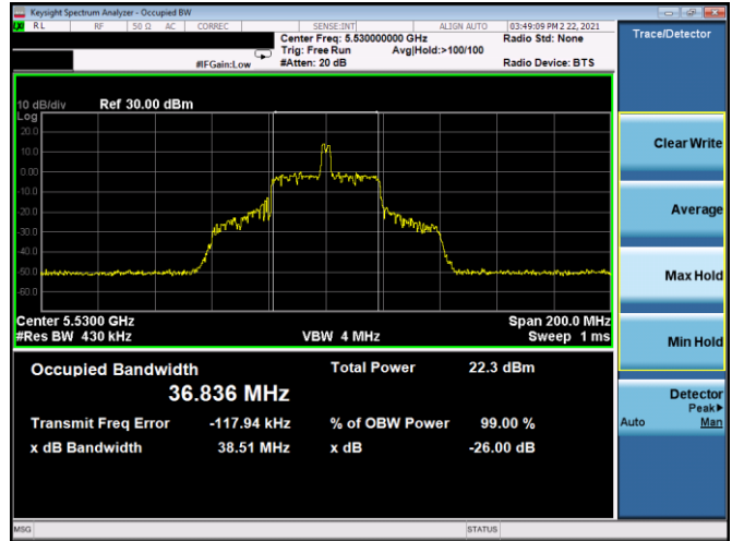
Plot 7-70. 26dB BW & 99% OBW Antenna 5B (80MHz BW 11ax Index 18 – RU26 – Ch.106)
