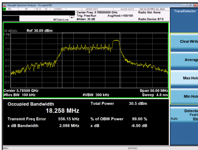
Plot 7-89. 6dB BW & 99% OBW Antenna 5B (20MHz BW 11ax Index 8 – RU26 – Ch.157)
