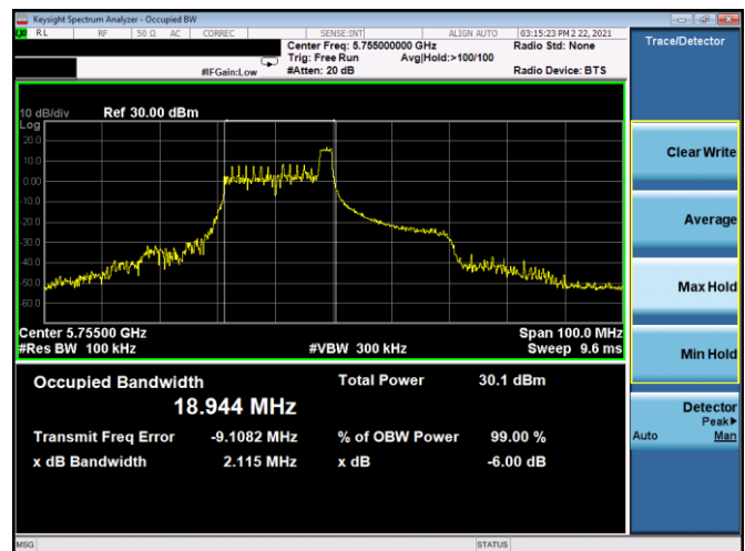
Plot 7-90. 6dB BW & 99% OBW Antenna 5B (40MHz BW 11ax Index 8 – RU26 – Ch.151)
