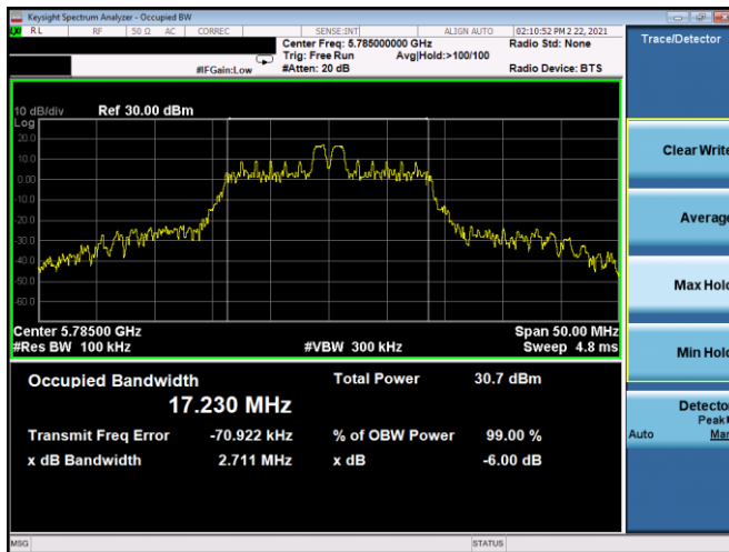
Plot 7-87. 6dB BW & 99% OBW Antenna 5B (20MHz BW 11ax Index 4 – RU26 – Ch.157)
