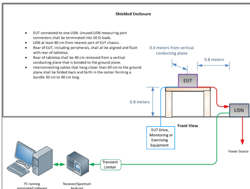
Figure 1 - Conducted Disturbance
