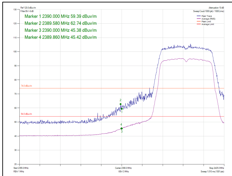
Figure 134 - 802.11n, HT20, Core 1 - 2412 MHz, Band Edge Frequency 2390 MHz
