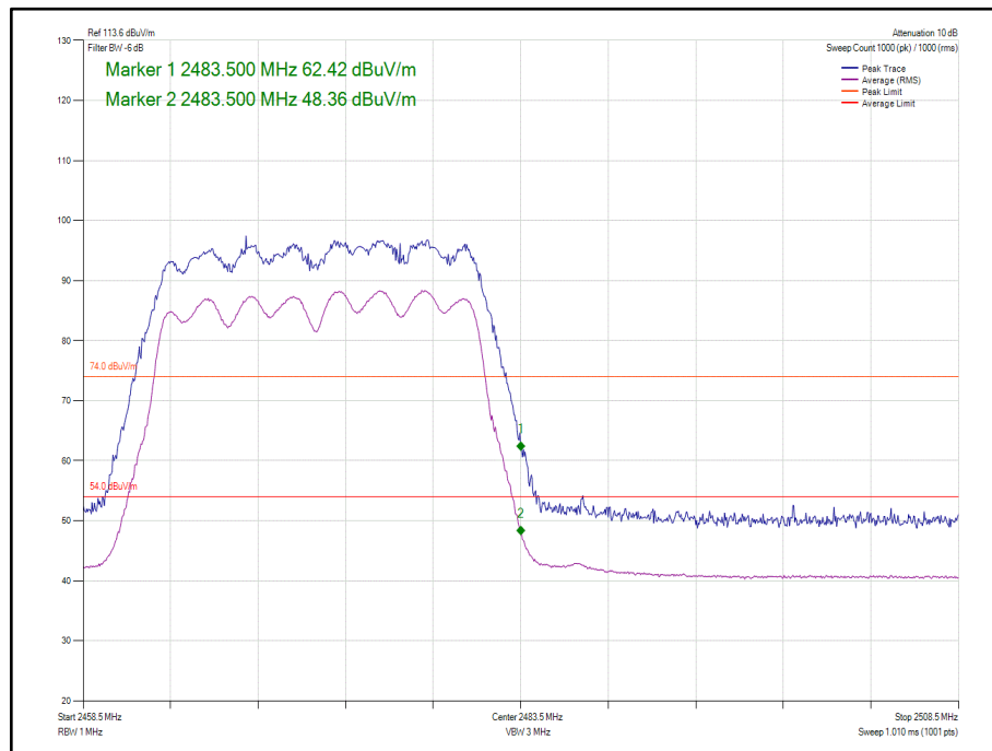
Figure 149 - 802.11n HT20, Core 0-1 - 2472 MHz, Band Edge Frequency 2483.5 MHz
