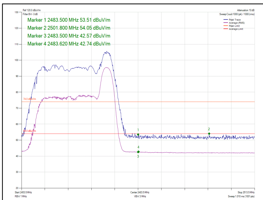
Figure 143 - 802.11ax HE20, Core 1, 26-8 - 2467 MHz, Band Edge Frequency 2483.5 MHz
