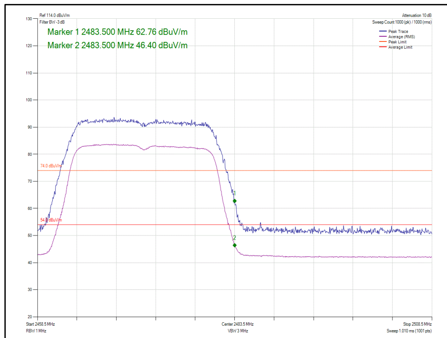
Figure 137 - 802.11n HT20, Core 1 - 2472 MHz, Band Edge Frequency 2483.5 MHz
