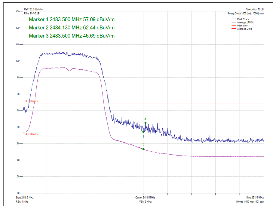
Figure 135 - 802.11n HT20, Core 1 - 2462 MHz, Band Edge Frequency 2483.5 MHz
