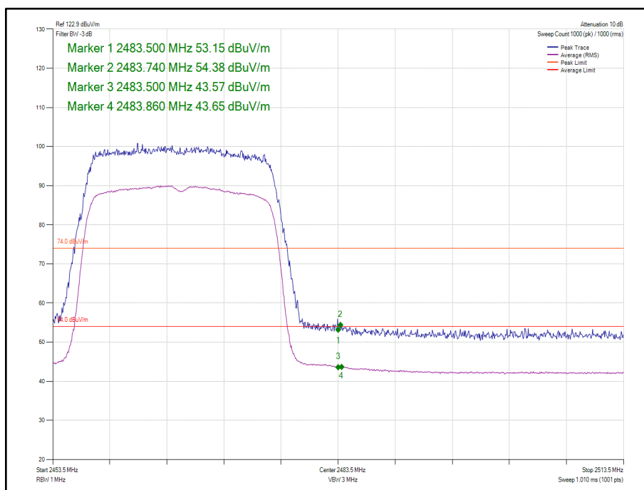
Figure 142 - 802.11ax HE20, Core 1, SU - 2467 MHz, Band Edge Frequency 2483.5 MHz
