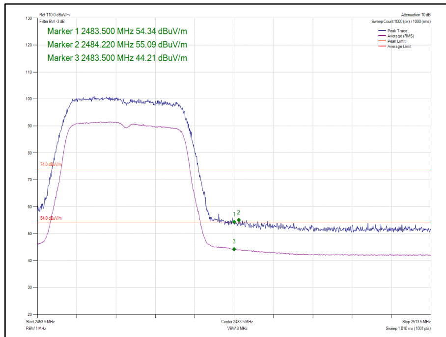
Figure 136 - 802.11n HT20, Core 1 - 2467 MHz, Band Edge Frequency 2483.5 MHz
