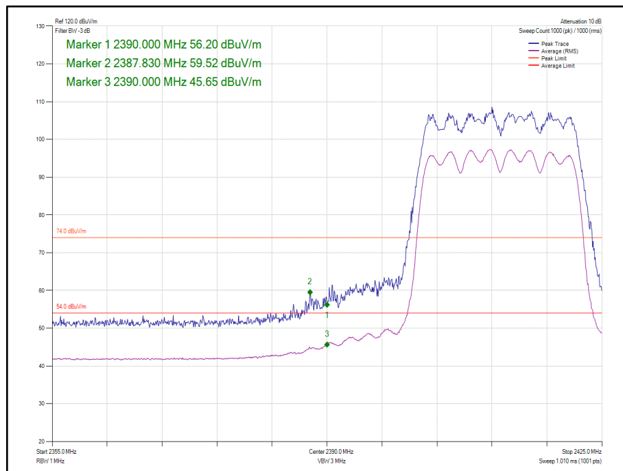
Figure 150 - 802.11ax HE20, Core 0-1, SU - 2412 MHz, Band Edge Frequency 2390 MHz
