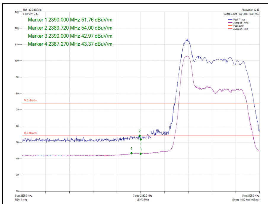
Figure 139 - 802.11ax HE20, Core 1, 26-0 - 2412 MHz, Band Edge Frequency 2390 MHz
