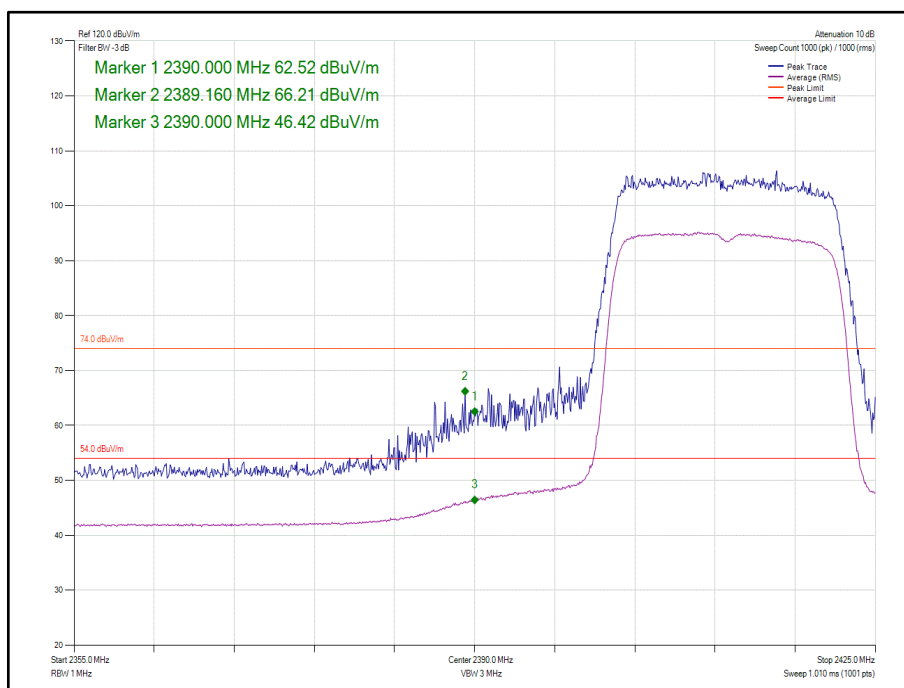
Figure 138 - 802.11ax HE20, Core 1, SU - 2412 MHz, Band Edge Frequency 2390 MHz
