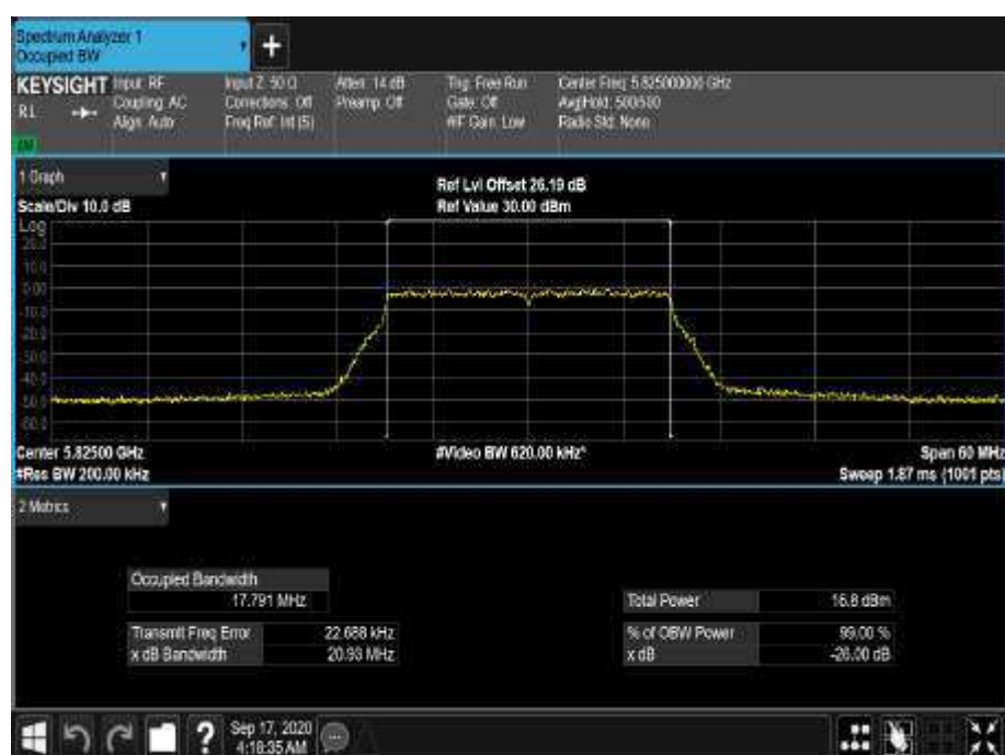
Figure 444 - 5825 MHz - 99% Occupied Bandwidth
