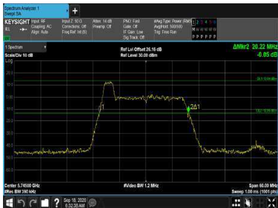
Figure 554 - 5745 MHz - 26 dB Emission Bandwidth
