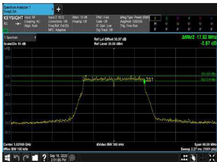
Figure 478 - 5825 MHz - 6 dB DTS Bandwidth
