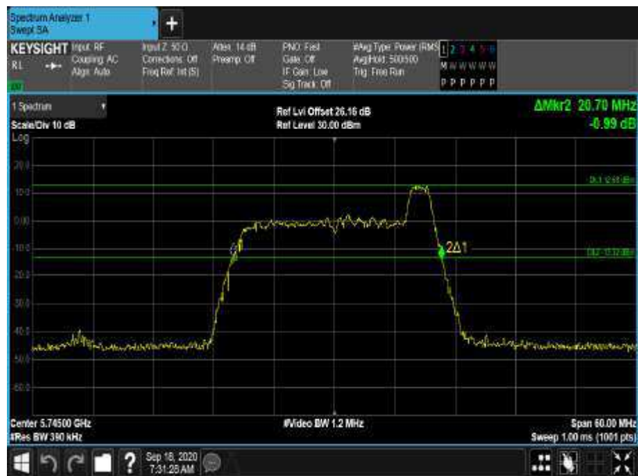
Figure 563 - 5745 MHz - 26 dB Emission Bandwidth
