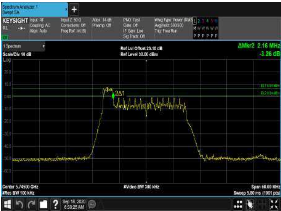
Figure 523 - 5745 MHz - 6 dB DTS Bandwidth
