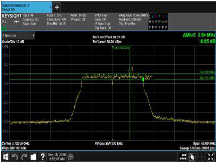
Figure 457 - 5720 MHz - 6 dB DTS Bandwidth
