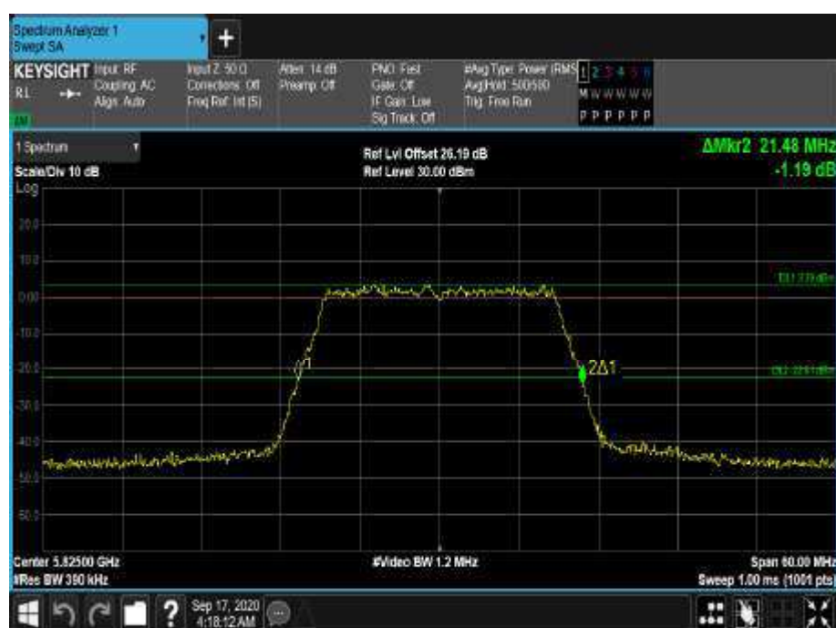
Figure 443 - 5825 MHz - 26 dB Emission Bandwidth
