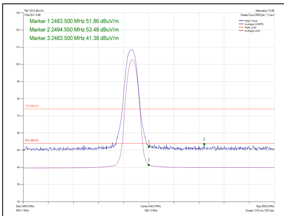
Figure 105 - Core 0 - \pi/4 DQPSK/2DH5 - 2480 MHz - Band Edge Frequency 2483.5 MHz
