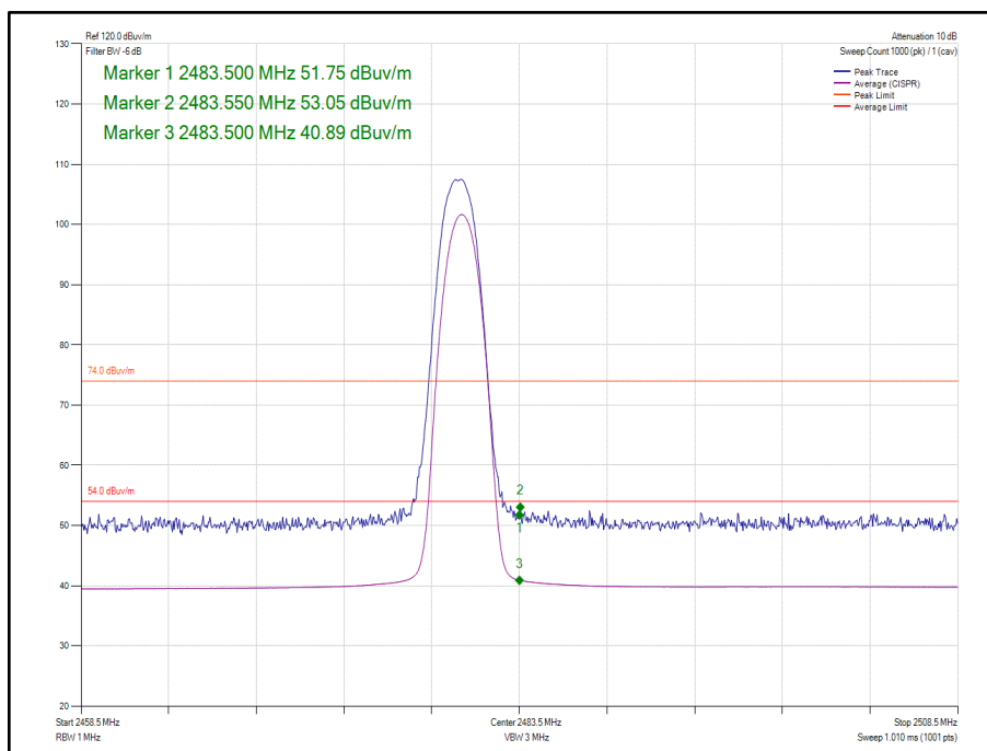
Figure 111 - Core 1 - \pi/4 DQPSK/2DH5 - 2480 MHz - Band Edge Frequency 2483.5 MHz
