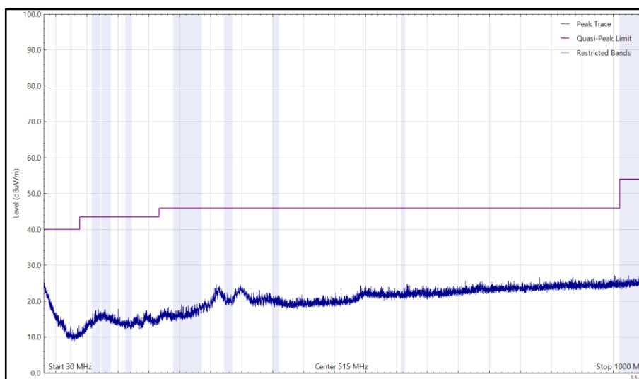
Figure 20 - 2452 MHz (CH9), HT20, CDD, Core 0 + Core 1 and 2402 MHz (CH0), DH5, ePA, Core 0, 30 MHz to 1 GHz, Horizontal (Peak)
