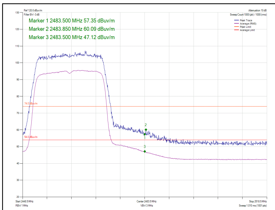
Figure 83 - 802.11ax HE20, Core 0, SU - 2462 MHz, Band Edge Frequency 2483.5 MHz
