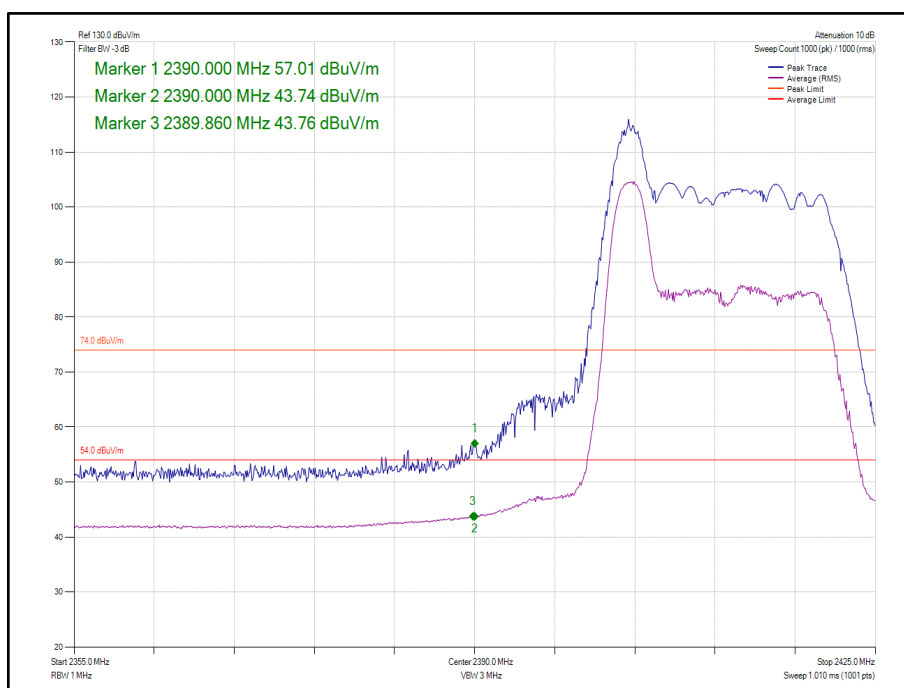
Figure 82 - 802.11ax HE20, Core 0, 26-0 - 2412 MHz, Band Edge Frequency 2390 MHz
