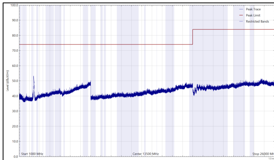
Figure 107 - 2437 MHz (CH6), HT20, CDD, Core 0 + Core 1, 1 GHz to 26 GHz, Horizontal (Peak)
