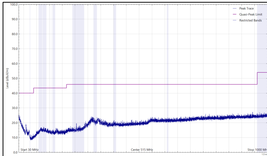
Figure 106 - 2437 MHz (CH6), HT20, CDD, Core 0 + Core 1, 30 MHz to 1 GHz, Horizontal (Peak)
