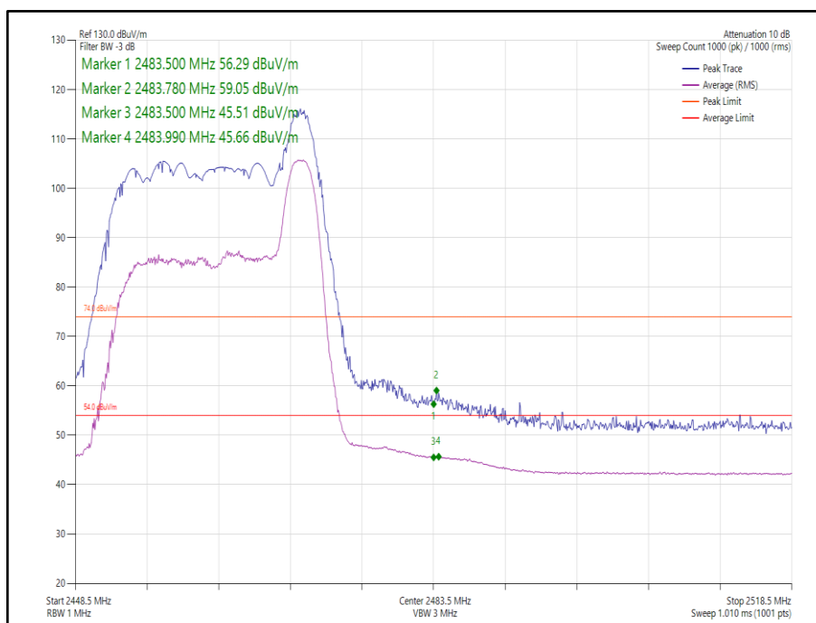
Figure 84 - 802.11ax HE20, Core 0, 26-8 - 2462 MHz, Band Edge Frequency 2483.5 MHz
