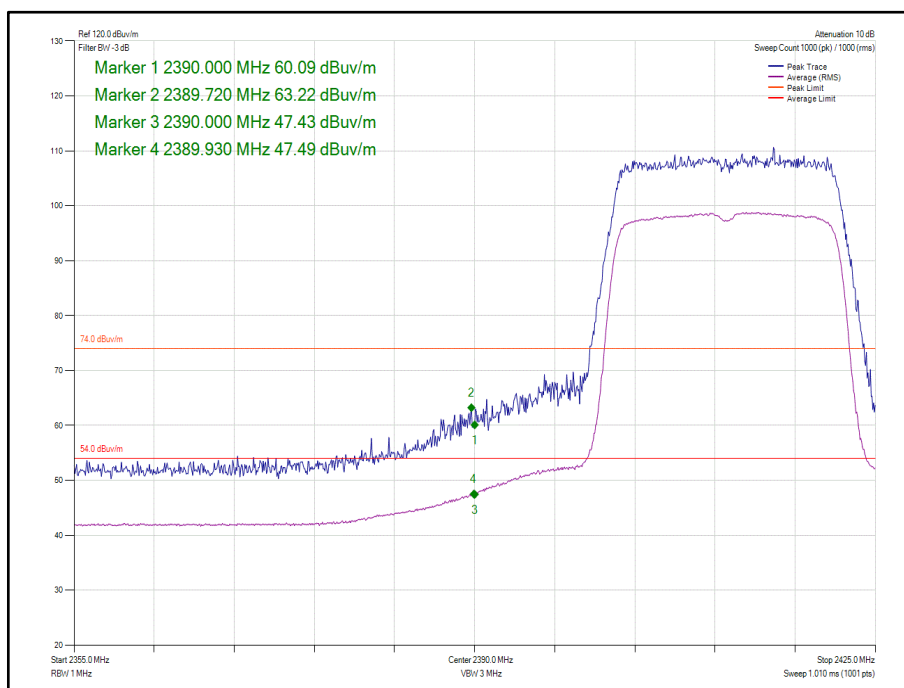
Figure 81 - 802.11ax HE20, Core 0, SU - 2412 MHz, Band Edge Frequency 2390 MHz
