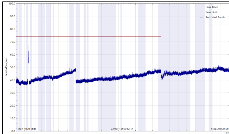
Figure 154 - 2472 MHz (CH13), HE20, RU26-0, Core 0 + Core 1, 1 GHz to 26 GHz, Horizontal (Peak)
