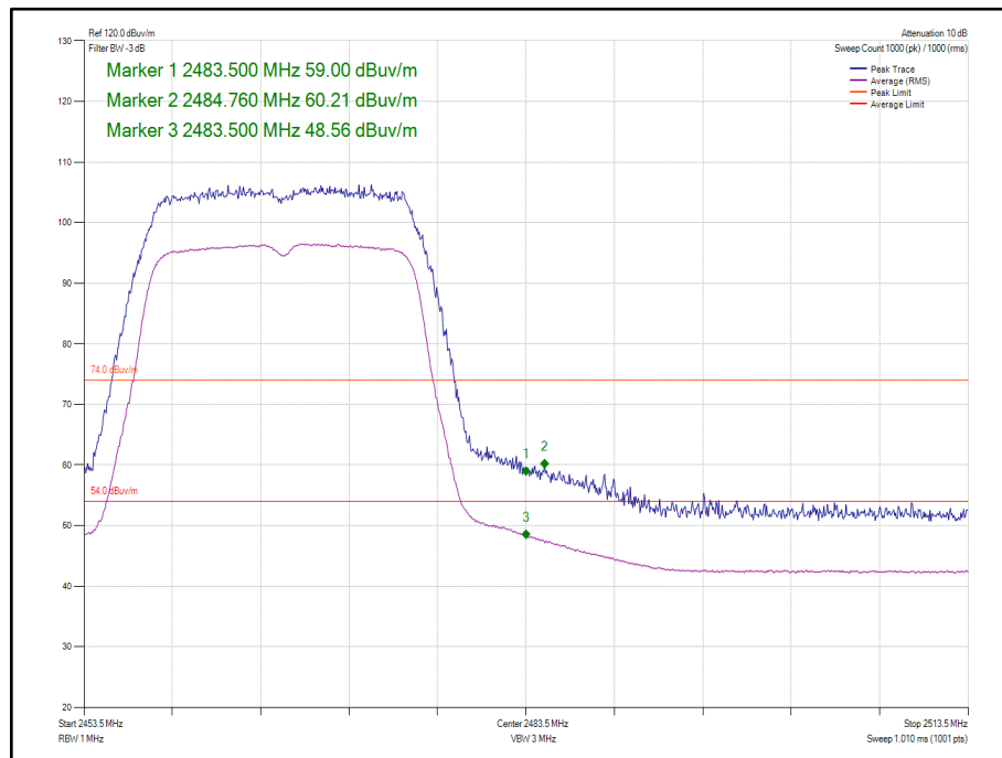
Figure 79 - 802.11n HT20, Core 0 - 2467 MHz, Band Edge Frequency 2483.5 MHz
