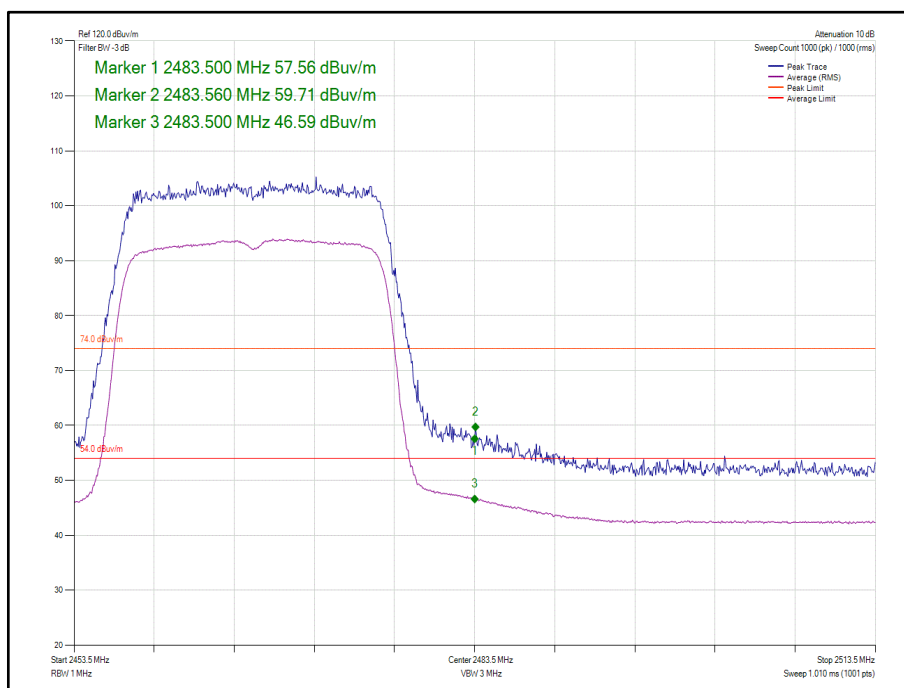
Figure 85 - 802.11ax HE20, Core 0, SU - 2467 MHz, Band Edge Frequency 2483.5 MHz
