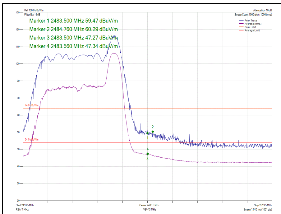
Figure 86 - 802.11ax HE20, Core 0, 26-8 - 2467 MHz, Band Edge Frequency 2483.5 MHz
