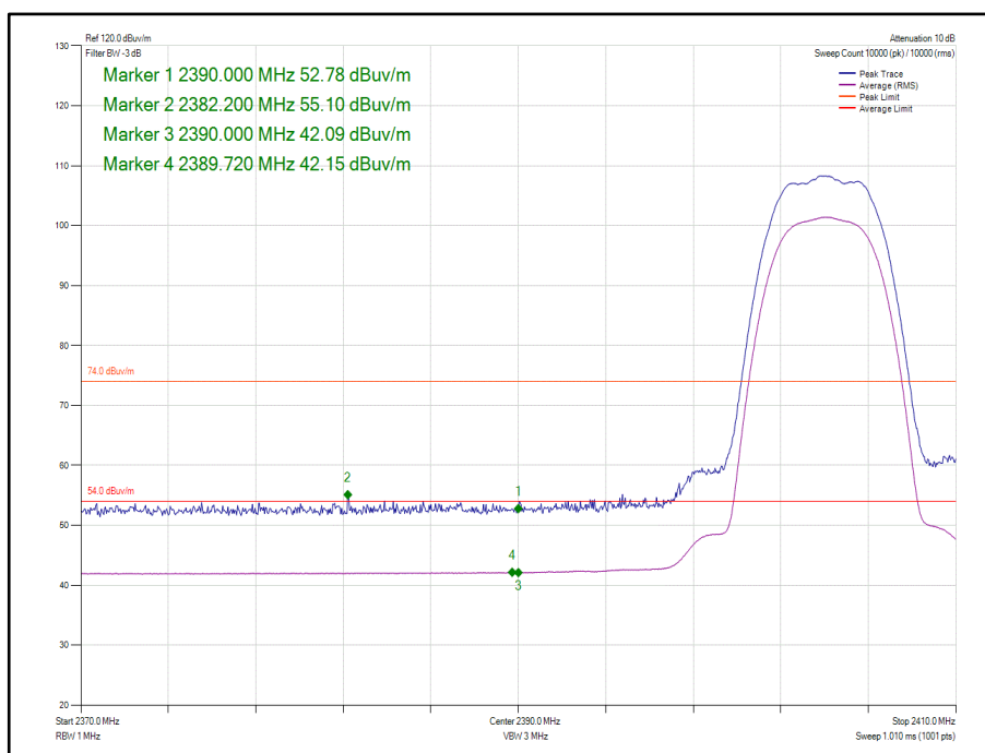
Figure 137- Core 0-1 - Static - \pi/4 DQPSK /HDR8 - 2404 MHz - Band Edge Frequency 2390.0 MHz
