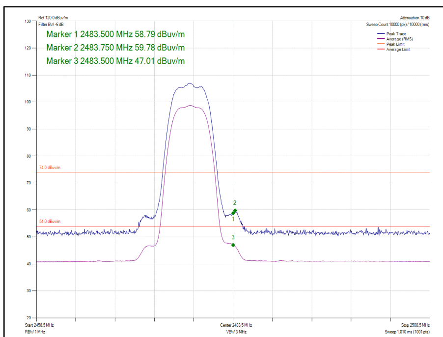
Figure 138 - Core 0-1 - Static - \pi/4 DQPSK /HDR8 - 2478 MHz - Band Edge Frequency 2483.5 MHz
