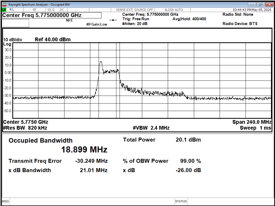
Figure 1042 - 5775 MHz - 99% Occupied Bandwidth
