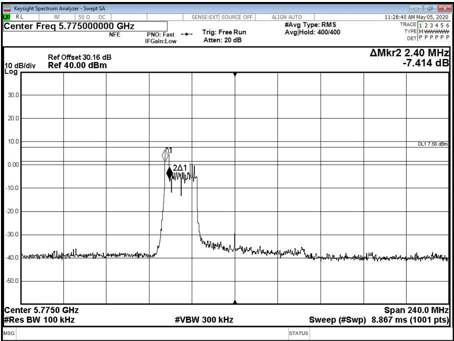
Figure 1016 - 5775 MHz - 6 dB DTS Bandwidth
