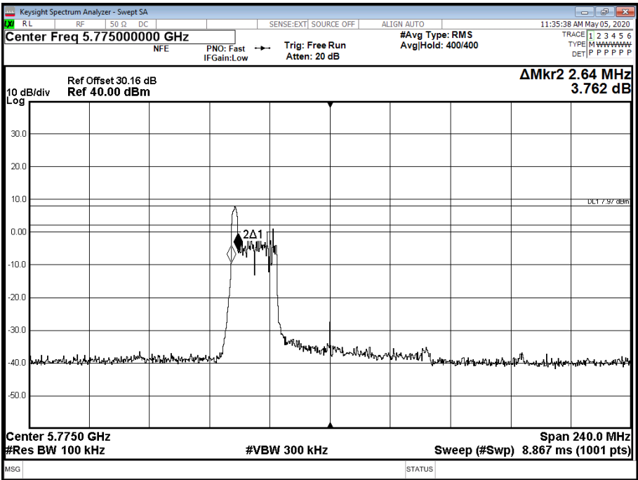
Figure 1028 - 5775 MHz - 6 dB DTS Bandwidth
