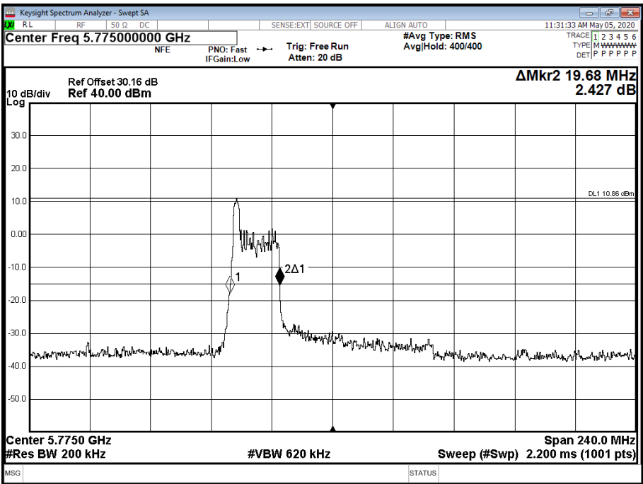
Figure 1017 - 5775 MHz - 26 dB Emission Bandwidth
