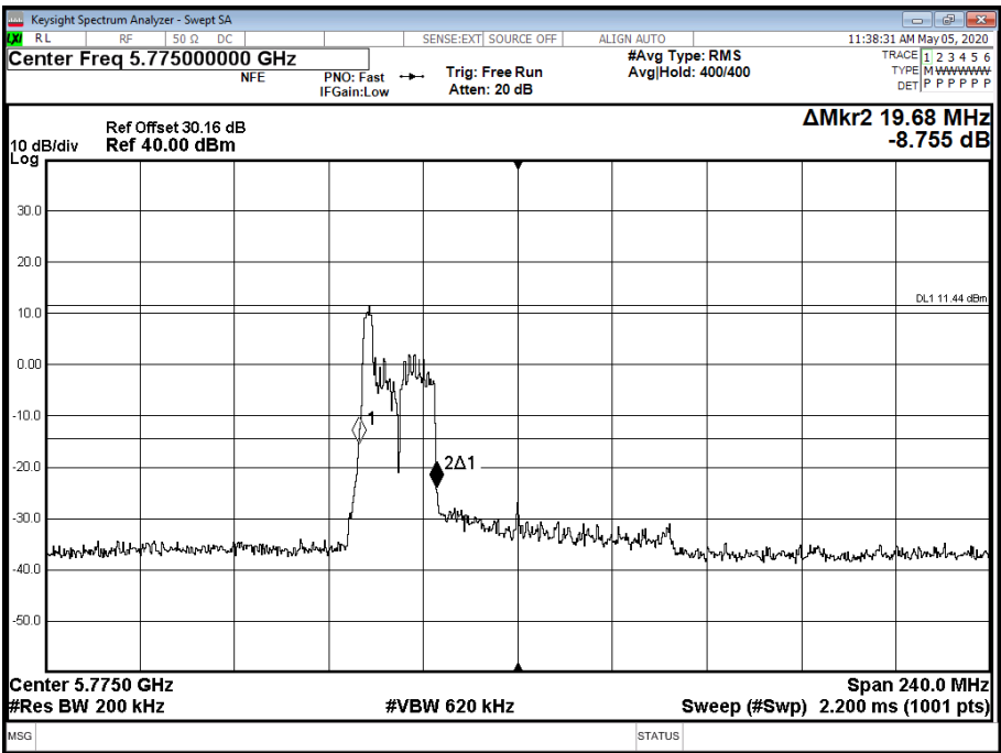
Figure 1029 - 5775 MHz - 26 dB Emission Bandwidth
