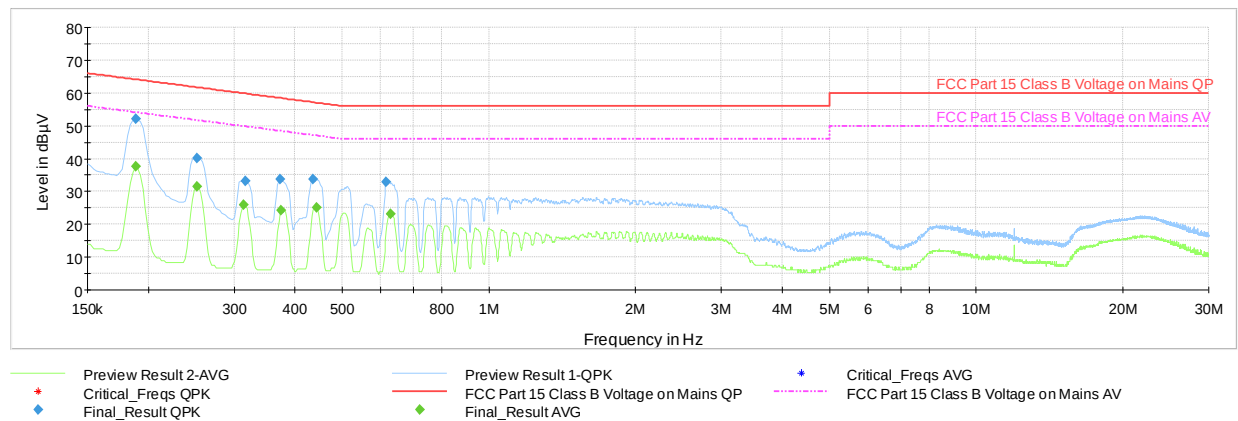
Plot 7-1586. AC Line Conducted Plot with 802.11ax UNII Band 1 – RU242 – Ch. 36 (L1) with Laptop
