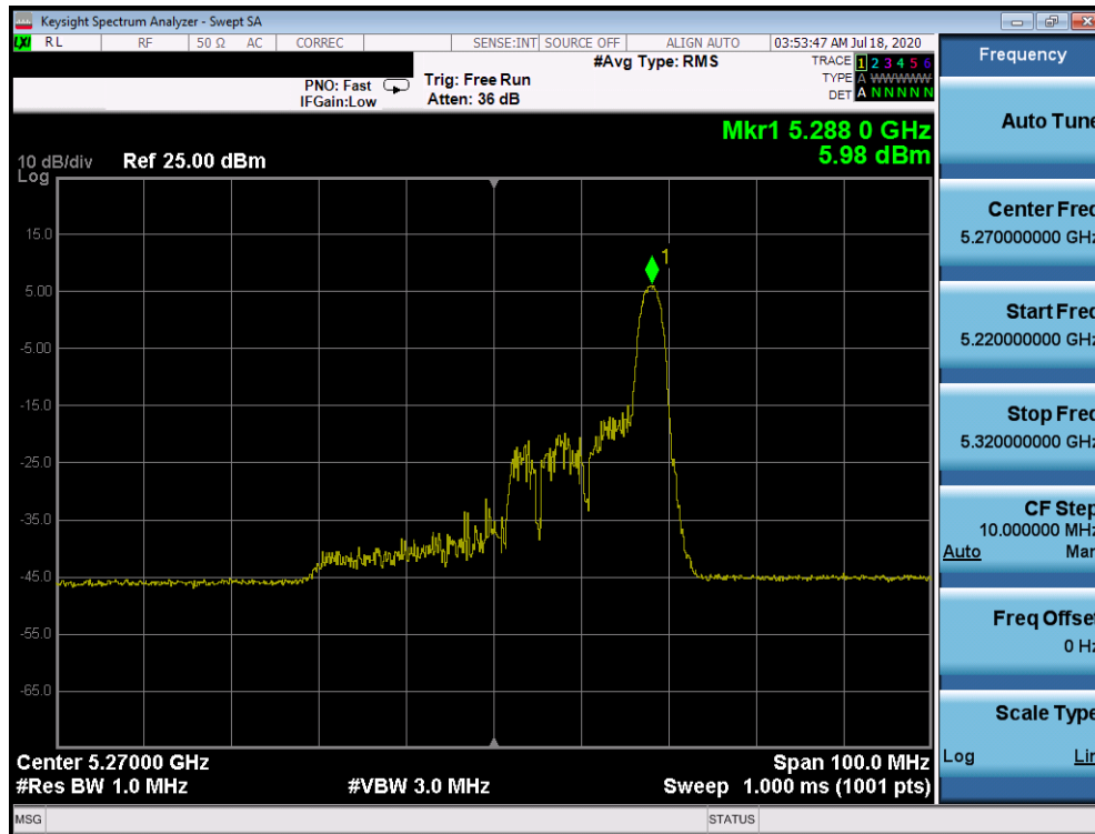
Plot 7-779. Power Spectral Density Plot CDD Primary Antenna 2b (40MHz BW 802.11ax Index 17 – RU26 (UNII Band 2A) – Ch. 54)
