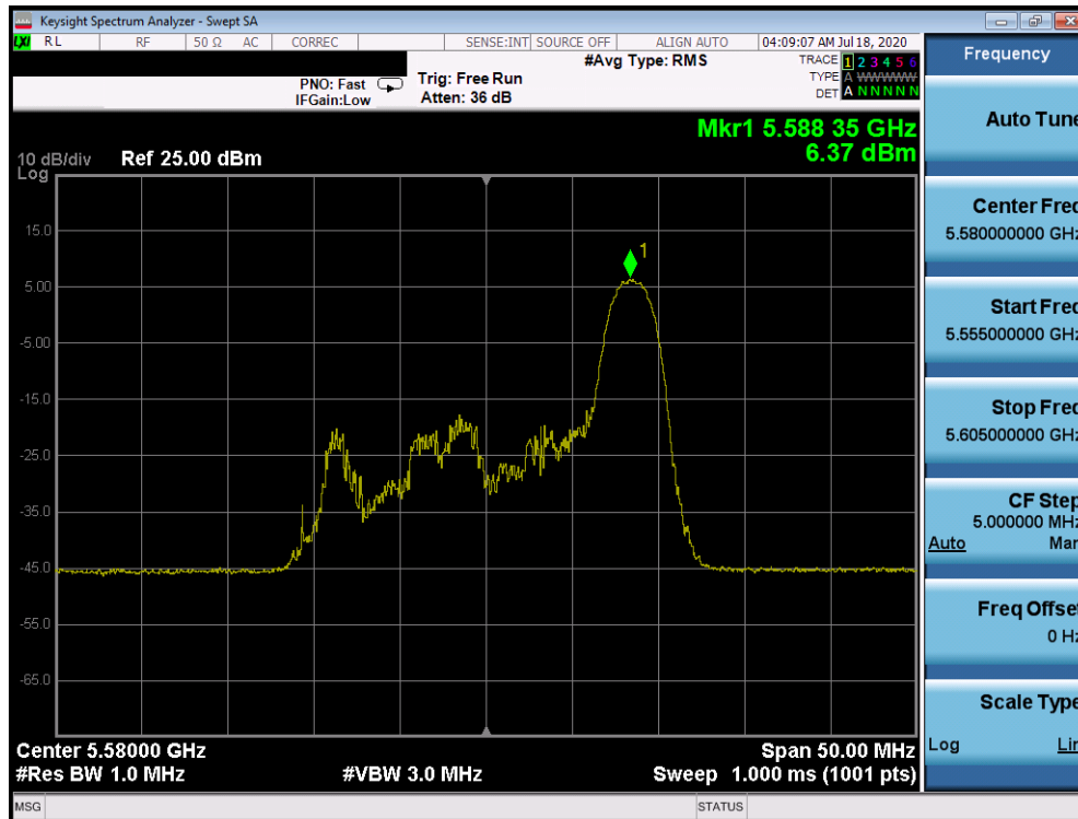
Plot 7-809. Power Spectral Density Plot CDD Primary Antenna 2b (20MHz BW 802.11ax Index 8– RU26 (UNII Band 2C) – Ch. 116)
