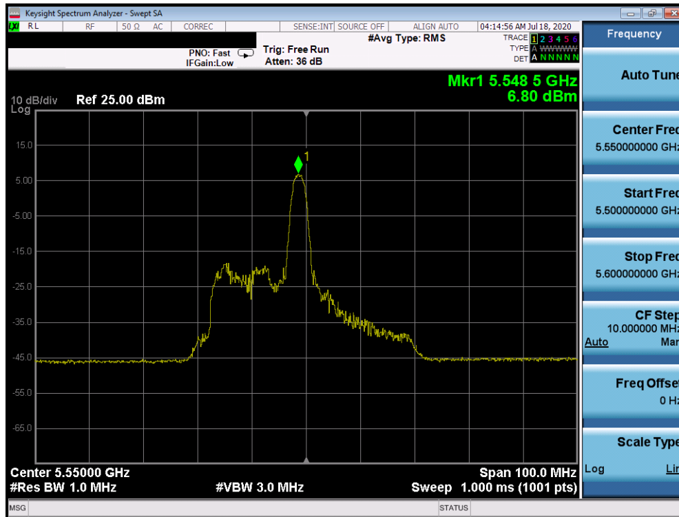
Plot 7-831. Power Spectral Density Plot CDD Primary Antenna 2b (40MHz BW 802.11ax Index 8 – RU26 (UNII Band 2C) – Ch. 110)
