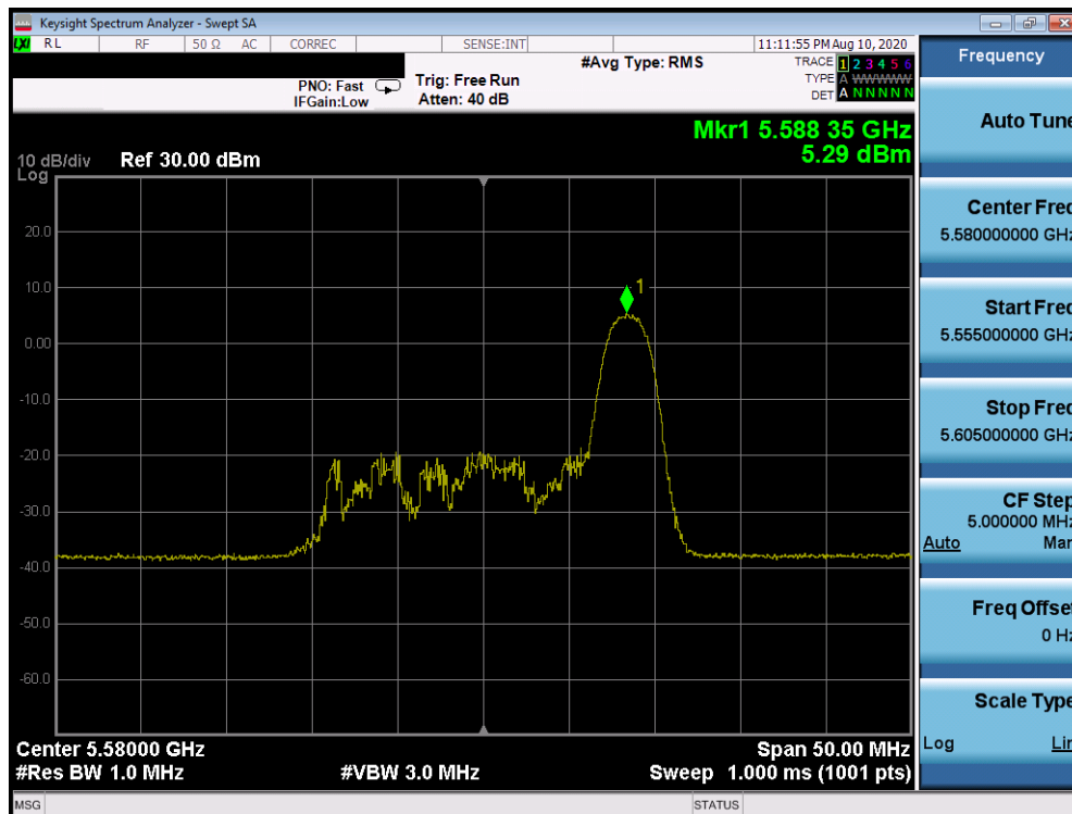
Plot 7-810. Power Spectral Density Plot CDD Primary Antenna 2a (20MHz BW 802.11ax Index 8– RU26 (UNII Band 2C) – Ch. 116)
