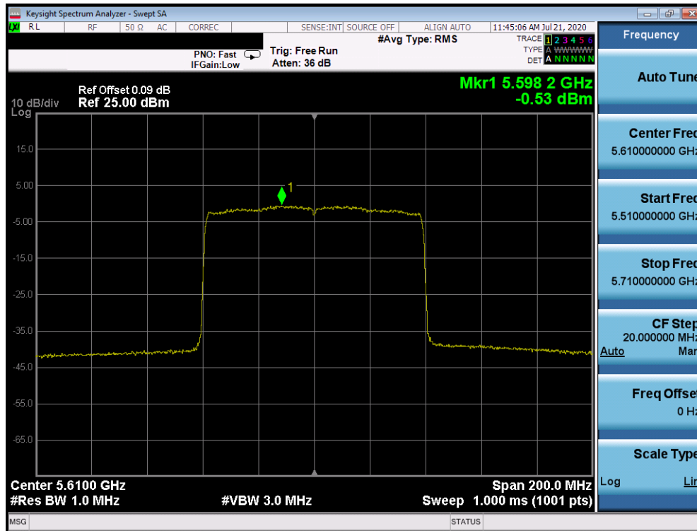
Plot 7-863. Power Spectral Density Plot CDD Primary Antenna 2b (80MHz BW 802.11ax – RU996 (UNII Band 2C) – Ch. 122)
