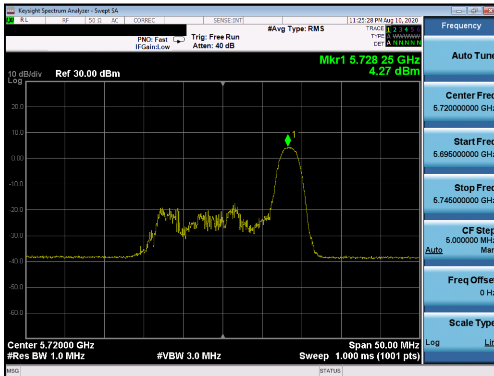
Plot 7-816. Power Spectral Density Plot CDD Primary Antenna 2a (20MHz BW 802.11ax Index 8 – RU26 (UNII Band 2C) – Ch. 144)
