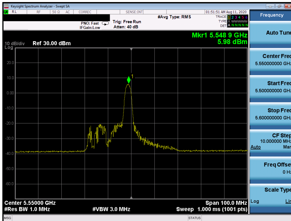
Plot 7-832. Power Spectral Density Plot CDD Primary Antenna 2a (40MHz BW 802.11ax Index 8 – RU26 (UNII Band 2C) – Ch. 110)
