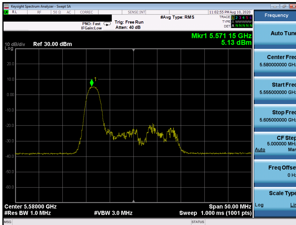
Plot 7-806. Power Spectral Density Plot CDD Primary Antenna 2a (20MHz BW 802.11ax Index 0 – RU26 (UNII Band 2C) – Ch. 116)
