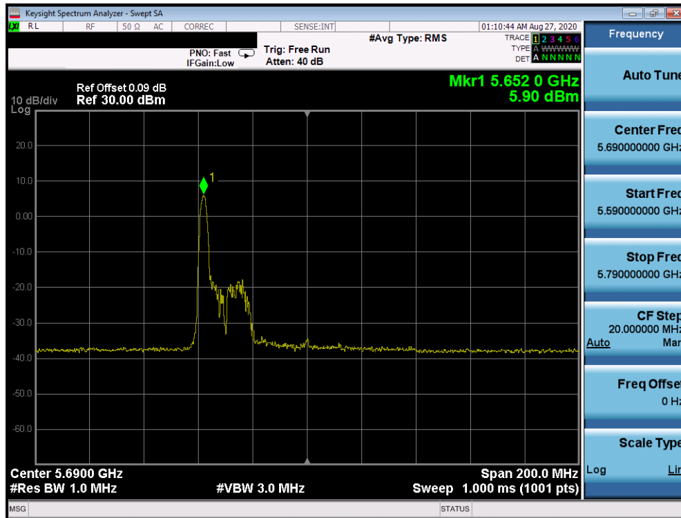
Plot 7-855. Power Spectral Density Plot CDD Primary Antenna 2b (80MHz BW 802.11ax Index 0 – RU26 (UNII Band 2C) – Ch. 138)
