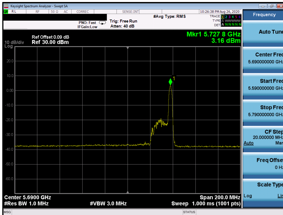
Plot 7-860. Power Spectral Density Plot CDD Primary Antenna 2a (80MHz BW 802.11ax Index 36 – RU26 (UNII Band 2C) – Ch. 138)
