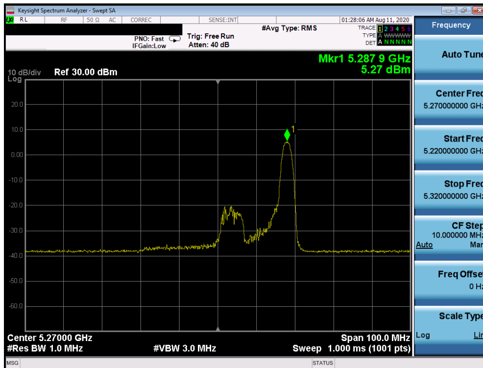
Plot 7-780. Power Spectral Density Plot CDD Primary Antenna 2a (40MHz BW 802.11ax Index 17 – RU26 (UNII Band 2A) – Ch. 54)
