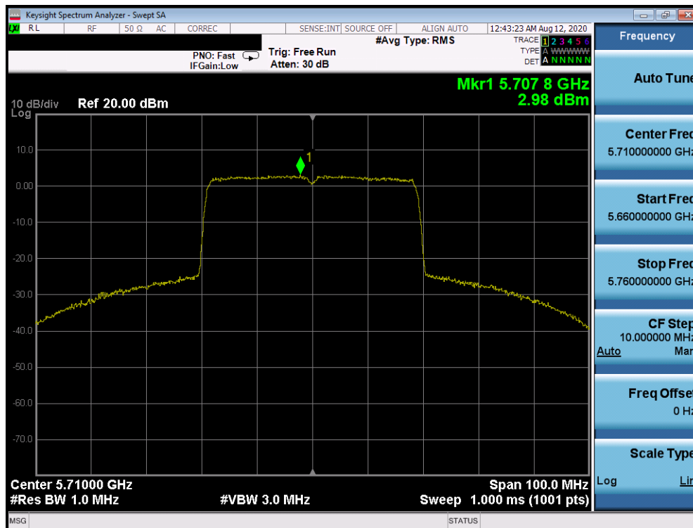
Plot 7-848. Power Spectral Density Plot CDD Primary Antenna 2a (40MHz BW 802.11ax – RU484 (UNII Band 2C) – Ch. 142)
