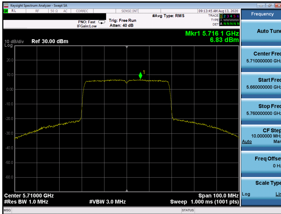
Plot 7-847. Power Spectral Density Plot CDD Primary Antenna 2b (40MHz BW 802.11ax – RU484 (UNII Band 2C) – Ch. 142)
