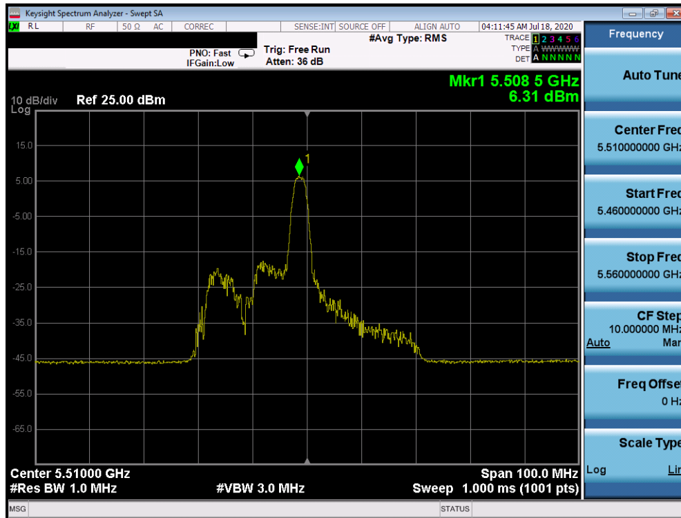
Plot 7-825. Power Spectral Density Plot CDD Primary Antenna 2b (40MHz BW 802.11ax Index 8 – RU26 (UNII Band 2C) – Ch. 102)
