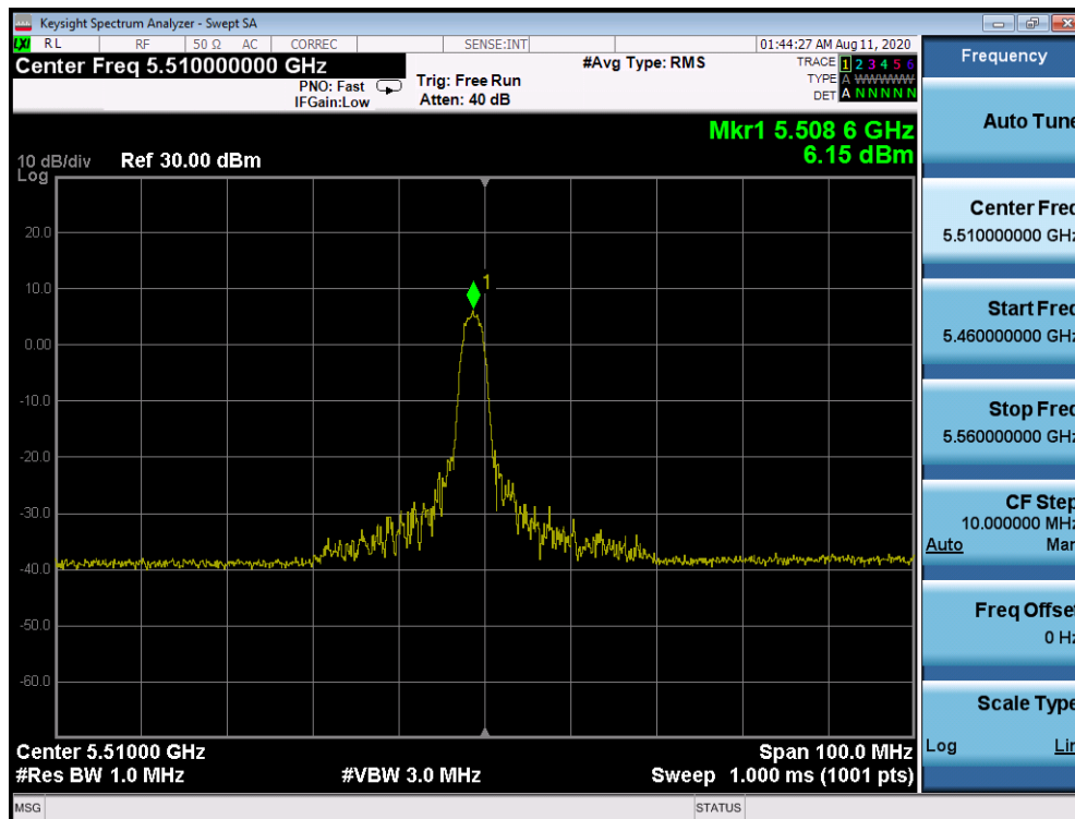
Plot 7-826. Power Spectral Density Plot CDD Primary Antenna 2a (40MHz BW 802.11ax Index 8 – RU26 (UNII Band 2C) – Ch. 102)
