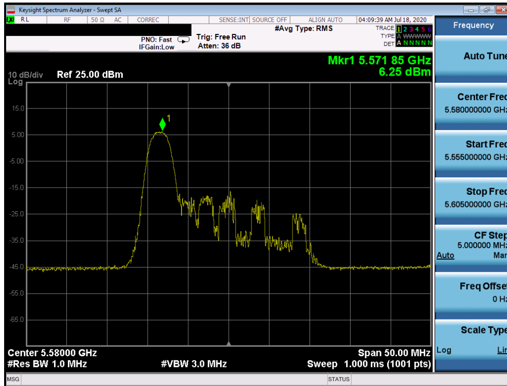
Plot 7-805. Power Spectral Density Plot CDD Primary Antenna 2b (20MHz BW 802.11ax Index 0 – RU26 (UNII Band 2C) – Ch. 116)
