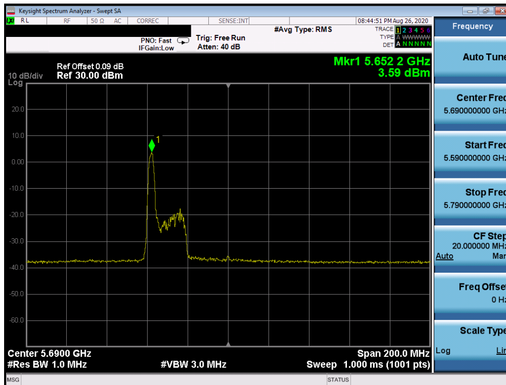
Plot 7-856. Power Spectral Density Plot CDD Primary Antenna 2a (80MHz BW 802.11ax Index 0 – RU26 (UNII Band 2C) – Ch. 138)
