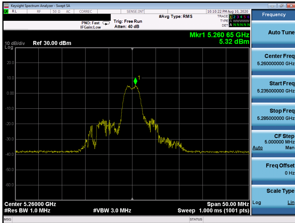
Plot 7-754. Power Spectral Density Plot CDD Primary Antenna 2a (20MHz BW 802.11ax Index 4 – RU26 (UNII Band 2A) – Ch. 52)
