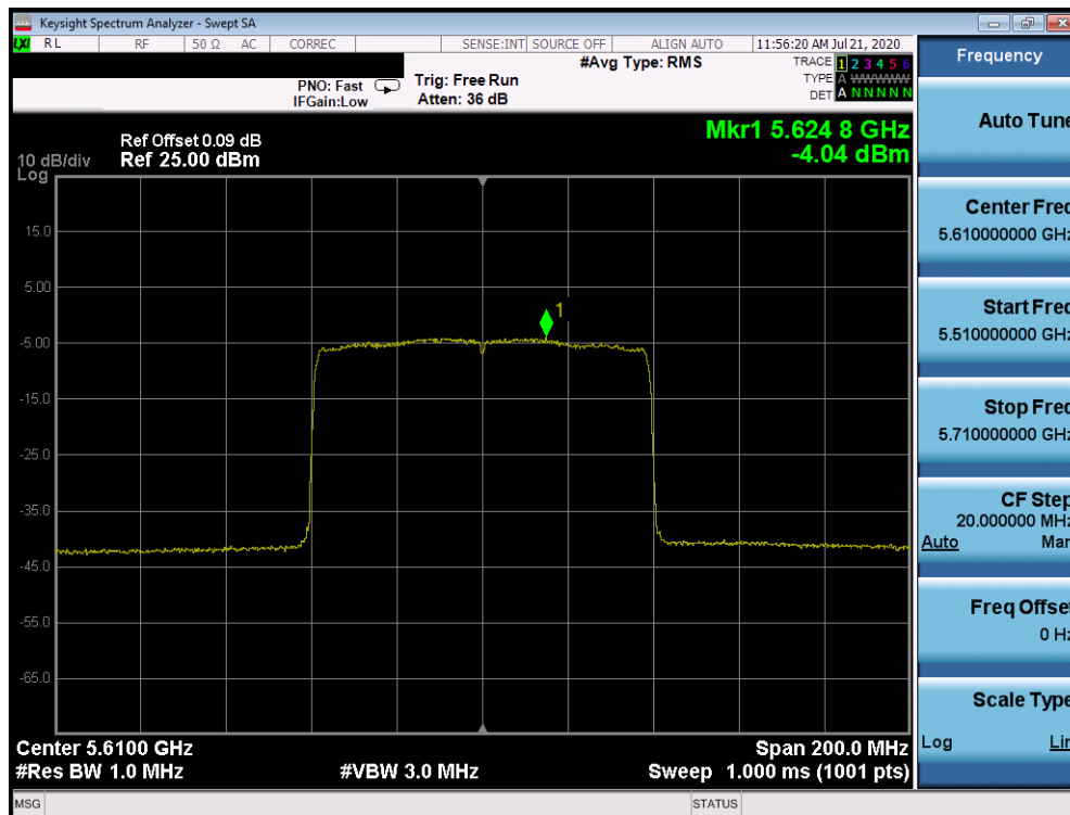
Plot 7-864. Power Spectral Density Plot CDD Primary Antenna 2a (80MHz BW 802.11ax – RU996 (UNII Band 2C) – Ch. 122)
