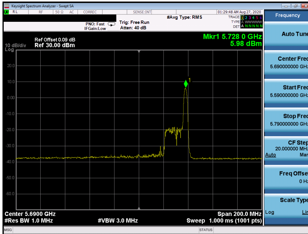
Plot 7-859. Power Spectral Density Plot CDD Primary Antenna 2b (80MHz BW 802.11ax Index 36 – RU26 (UNII Band 2C) – Ch. 138)
