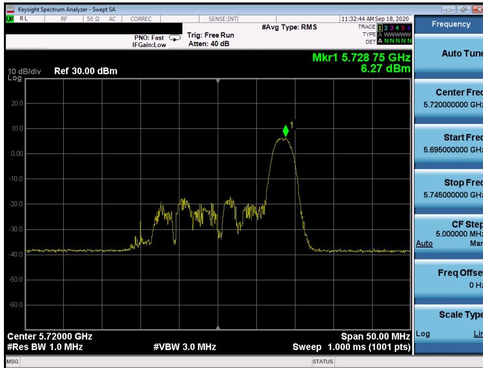
Plot 7-815. Power Spectral Density Plot CDD Primary Antenna 2b (20MHz BW 802.11ax Index 8 – RU26 (UNII Band 2C) – Ch. 144)
