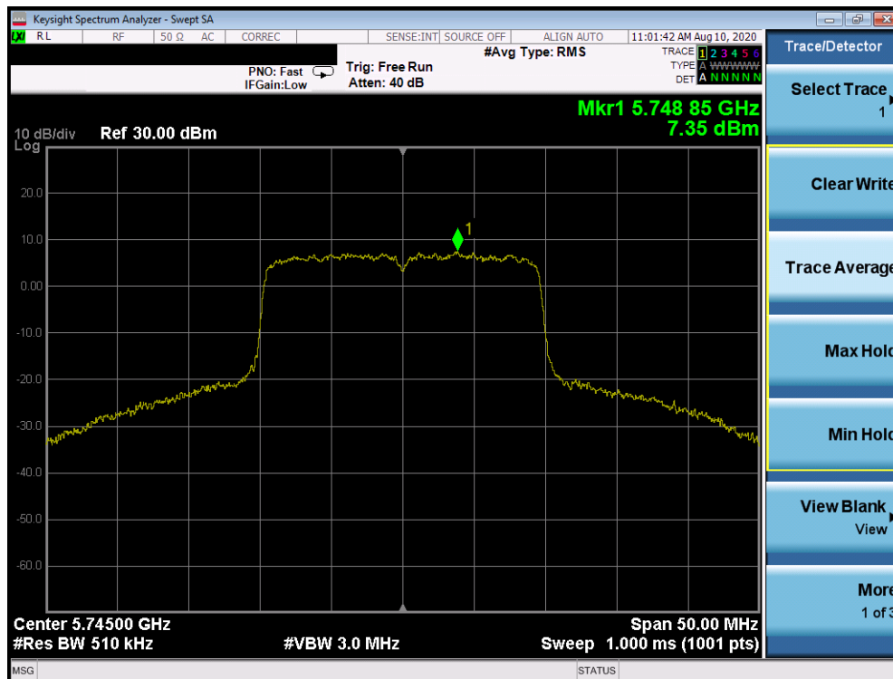
Plot 7-404. Power Spectral Density Plot Antenna 2b (20MHz BW 802.11ax– RU242 (UNII Band 3) – Ch. 149)
