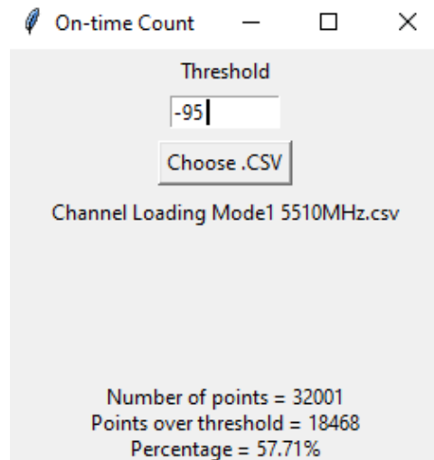
Figure 9-4 5510MHz - Channel Loading Calculation - Mode 1 (40MHz)
