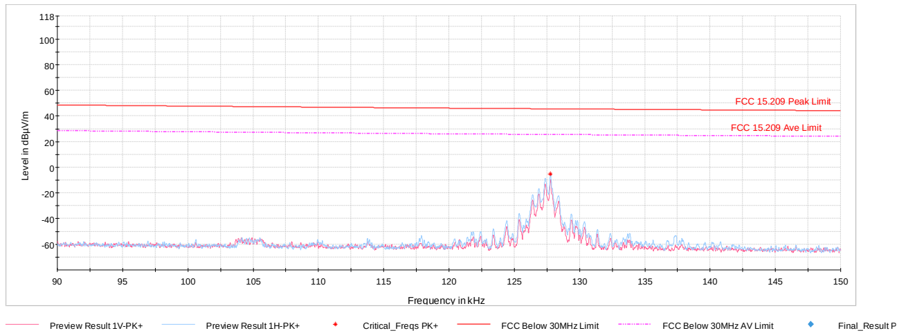
Plot 6-2. Radiated Restricted Lower Band Edge Peak Measurement (Charging Rate 10C)
