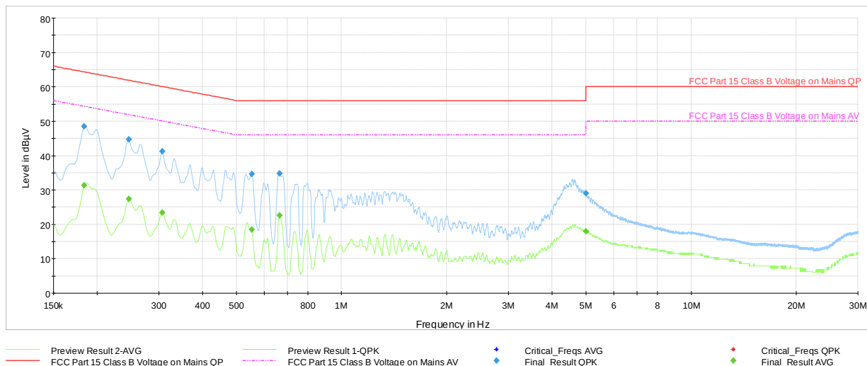
Plot 6-6. AC Line Conducted Plot (N, Charging Rate 10C, with AC/DC Adapter)
