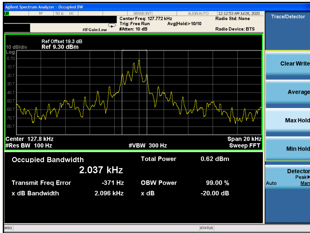
Plot 6-1. Occupied Bandwidth Plot (Charging Rate 10C)
