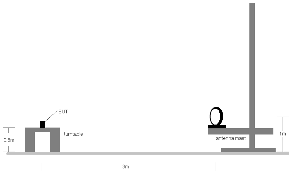
Figure 6-1. Test Setup
