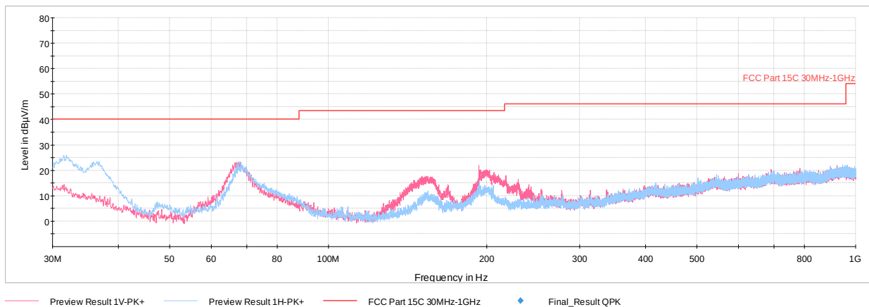
Plot 6-4. Radiated Spurious Emissions 30MHz-1000MHz (Charging Rate 10C, with AC/DC Adapter)
