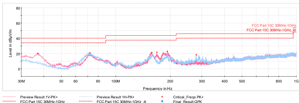
Plot 7-84. Radiated Spurious Emissions below 1GHz Simultaneous Tx, with AC/DC Adapter
