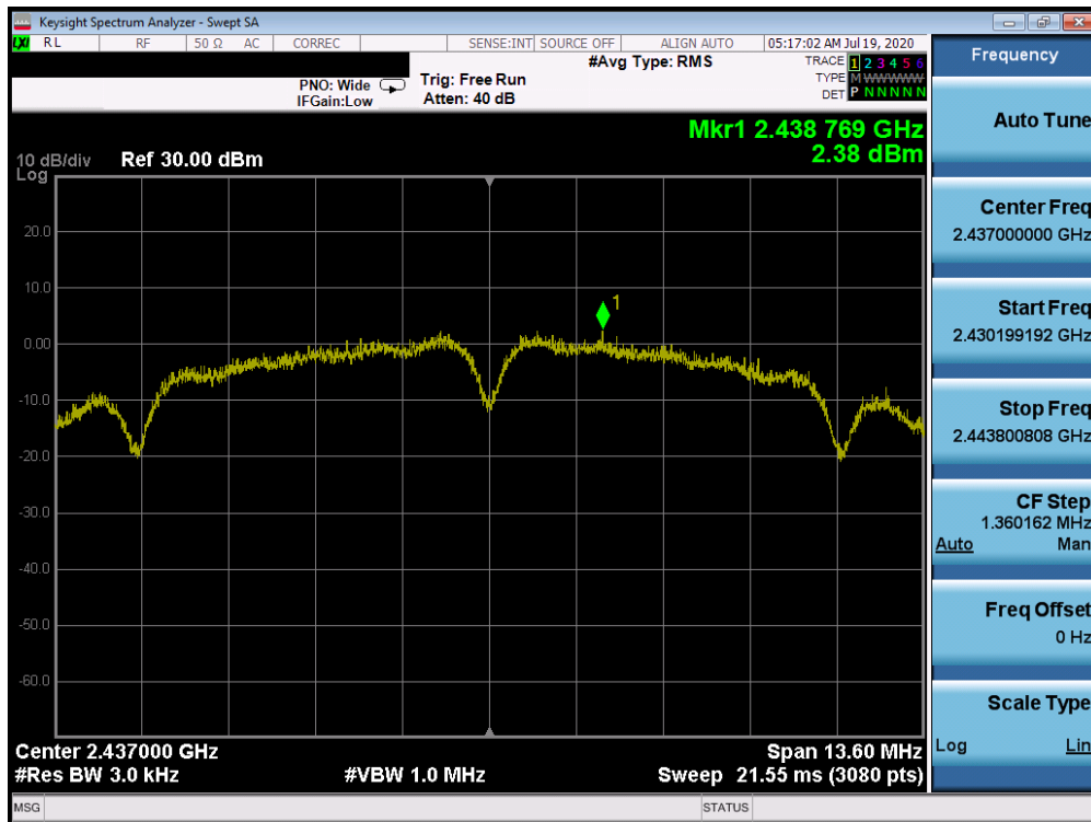
Plot 7-20. Power Spectral Density Plot ANT WF8 (802.11b – Ch. 6)
