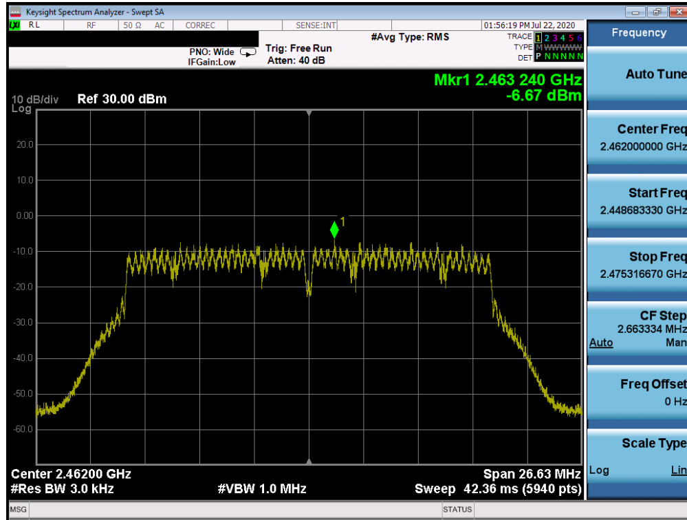
Plot 7-36. Power Spectral Density Plot ANT WF7b (802.11n (2.4GHz) – Ch. 11)
