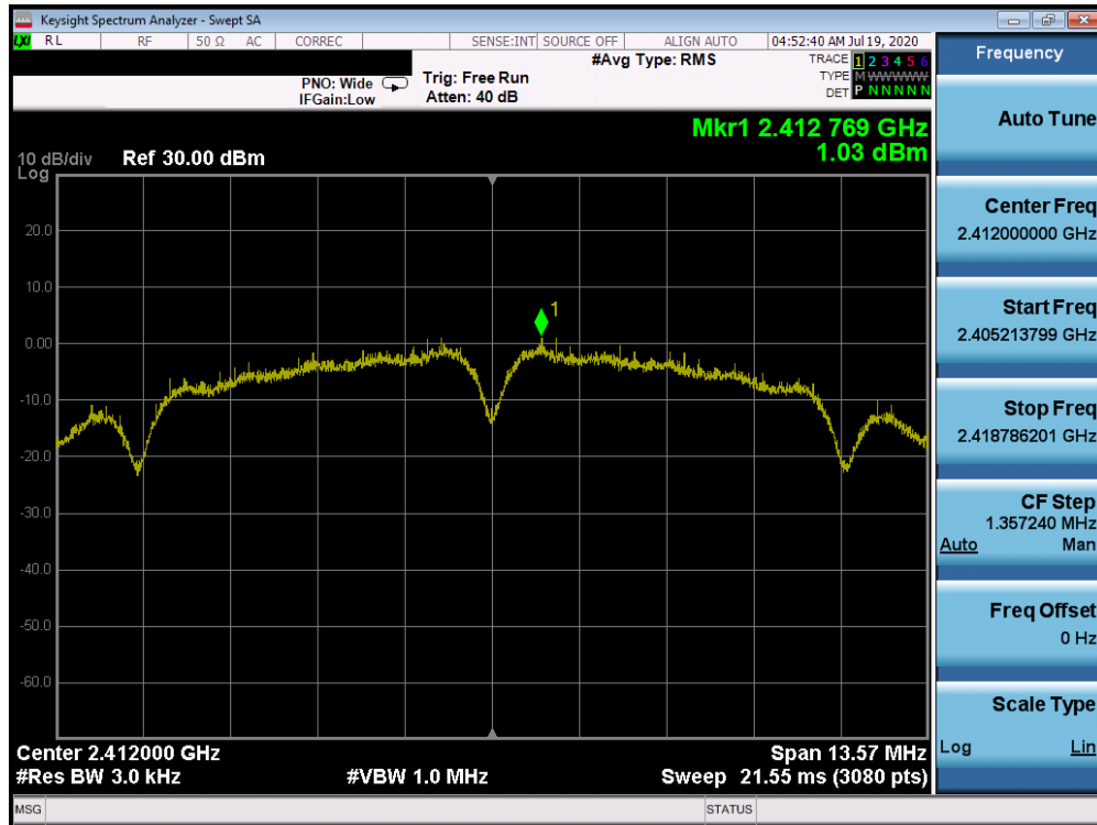
Plot 7-19. Power Spectral Density Plot ANT WF8 (802.11b – Ch. 1)
