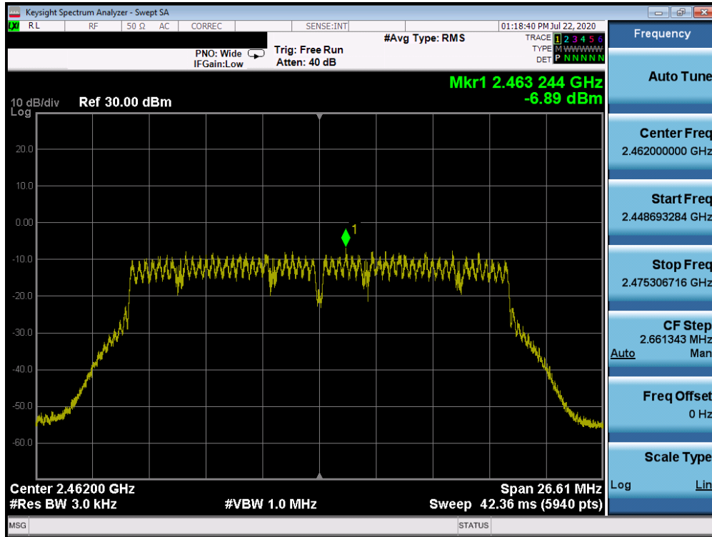
Plot 7-27. Power Spectral Density Plot ANT WF8 (802.11n (2.4GHz) – Ch. 11)
