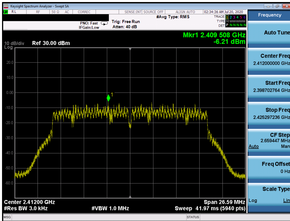
Plot 7-44. Power Spectral Density Plot CDD ANT WF7b (802.11n (2.4GHz) – Ch. 1)
