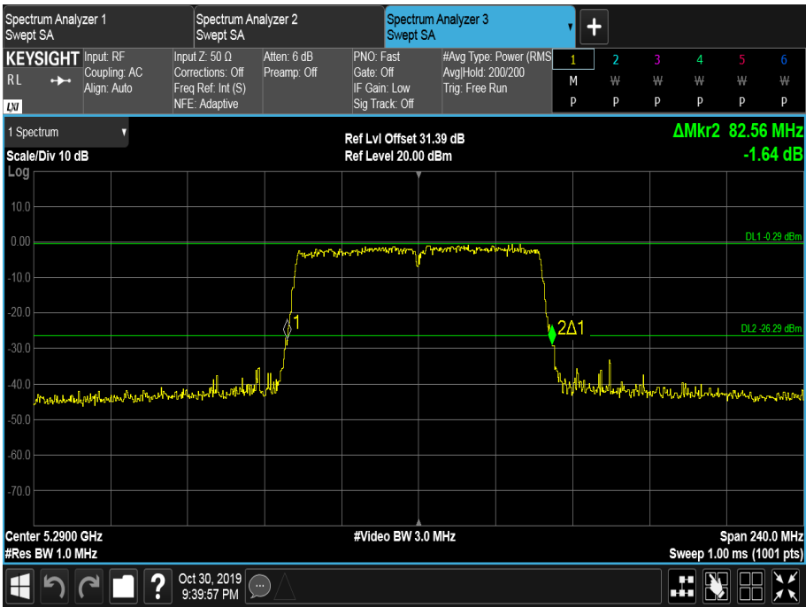
Figure 313 - 5290 MHz - 26 dB Emission Bandwidth
